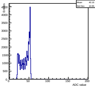
Pedestals ch 12 chip 3000 shift-gain3-shaper0
