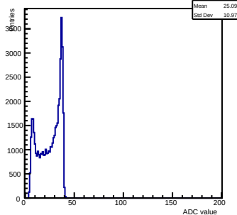
Pedestals ch 14 chip 3000 shift-gain3-shaper0
