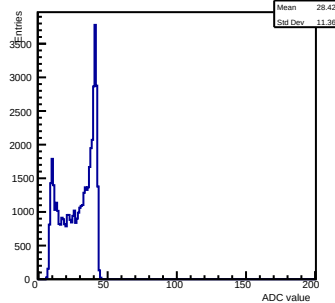
Pedestals ch 11 chip 3000 shift-gain3-shaper0
