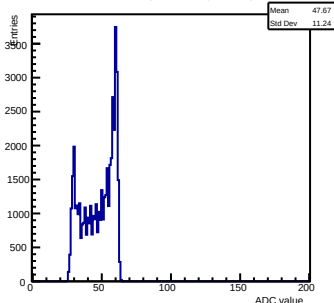
Pedestals ch 4 chip 3000 shift-gain3-shaper0
