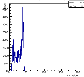
Pedestals ch 3 chip 3000 shift-gain3-shaper0
