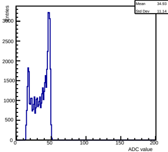
Pedestals ch 8 chip 3000 shift-gain3-shaper0
