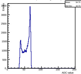
Pedestals ch 0 chip 3000 shift-gain3-shaper0
