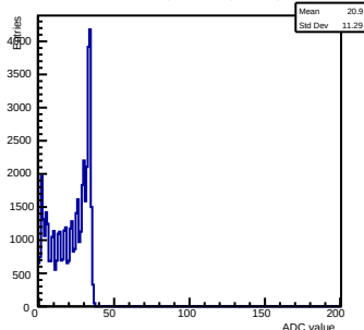
Pedestals ch 5 chip 3000 shift-gain3-shaper0
