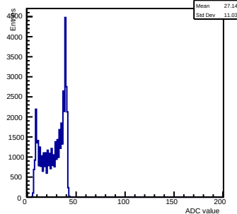
Pedestals ch 15 chip 3000 shift-gain3-shaper0
