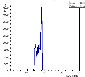
Pedestals ch 7 chip 3001 shift-gain0-shaper7
