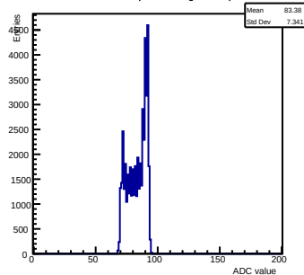
Pedestals ch 6 chip 3001 shift-gain0-shaper7
