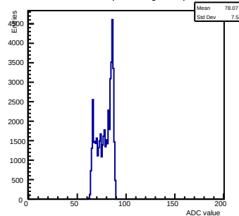
Pedestals ch 15 chip 3001 shift-gain0-shaper7
