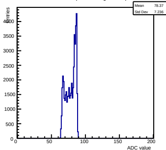
Pedestals ch 13 chip 3001 shift-gain0-shaper7
