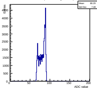
Pedestals ch 5 chip 3001 shift-gain0-shaper7
