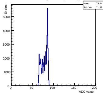
Pedestals ch 14 chip 3001 shift-gain0-shaper7
