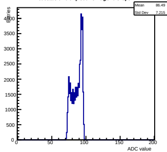
Pedestals ch 0 chip 3001 shift-gain0-shaper7
