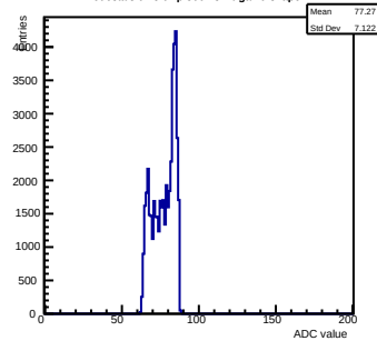
Pedestals ch 3 chip 3001 shift-gain0-shaper7
