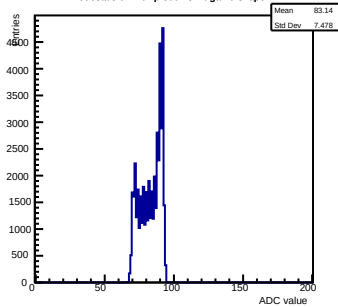
Pedestals ch 1 chip 3001 shift-gain0-shaper7
