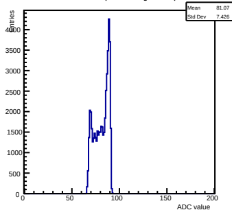
Pedestals ch 12 chip 3001 shift-gain0-shaper7
