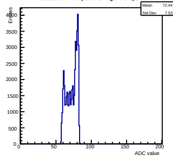
Pedestals ch 11 chip 3001 shift-gain0-shaper7
