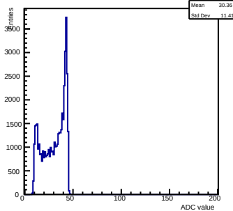
Pedestals ch 11 chip 3002 shift-gain3-shaper0
