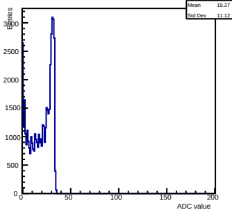
Pedestals ch 8 chip 3002 shift-gain3-shaper0
