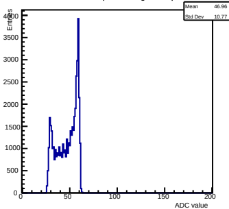
Pedestals ch 0 chip 3002 shift-gain3-shaper0
