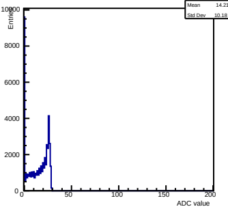
Pedestals ch 9 chip 3002 shift-gain3-shaper0
