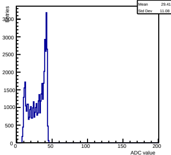
Pedestals ch 12 chip 3002 shift-gain3-shaper0
