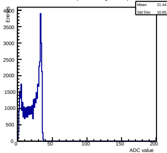
Pedestals ch 1 chip 3002 shift-gain3-shaper0
