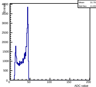
Pedestals ch 15 chip 3002 shift-gain3-shaper0
