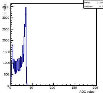
Pedestals ch 14 chip 3002 shift-gain3-shaper0
