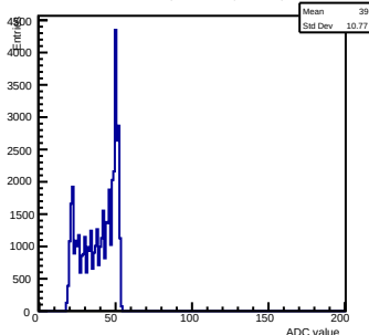
Pedestals ch 7 chip 3002 shift-gain3-shaper0
