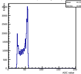
Pedestals ch 2 chip 3002 shift-gain3-shaper0
