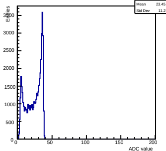
Pedestals ch 13 chip 3002 shift-gain3-shaper0
