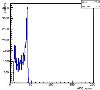
Pedestals ch 10 chip 3002 shift-gain3-shaper0
