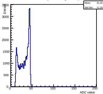
Pedestals ch 3 chip 3002 shift-gain3-shaper0
