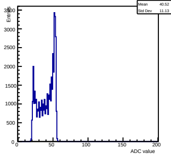
Pedestals ch 4 chip 3003 shift-gain3-shaper0
