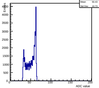
Pedestals ch 9 chip 3003 shift-gain3-shaper0
