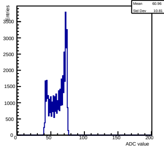
Pedestals ch 1 chip 3003 shift-gain3-shaper0
