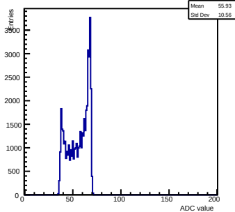
Pedestals ch 5 chip 3003 shift-gain3-shaper0
