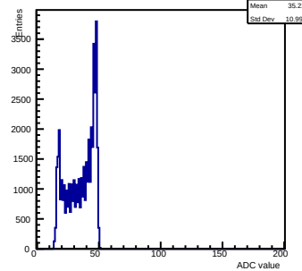
Pedestals ch 11 chip 3003 shift-gain3-shaper0
