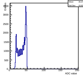
Pedestals ch 3 chip 3003 shift-gain3-shaper0
