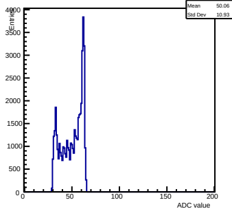
Pedestals ch 12 chip 3003 shift-gain3-shaper0
