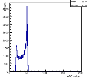
Pedestals ch 10 chip 3003 shift-gain3-shaper0
