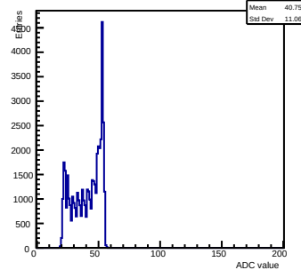
Pedestals ch 15 chip 3003 shift-gain3-shaper0
