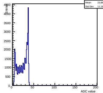
Pedestals ch 7 chip 3003 shift-gain3-shaper0
