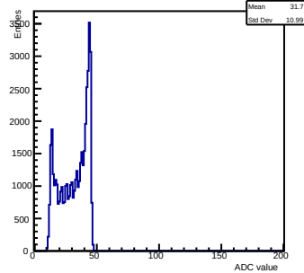
Pedestals ch 2 chip 3003 shift-gain3-shaper0
