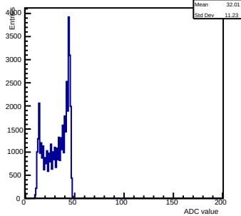
Pedestals ch 8 chip 3003 shift-gain3-shaper0
