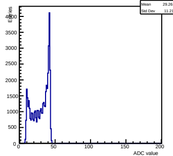
Pedestals ch 6 chip 3003 shift-gain3-shaper0
