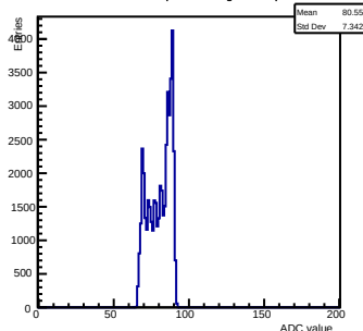
Pedestals ch 6 chip 3003 shift-gain0-shaper7
