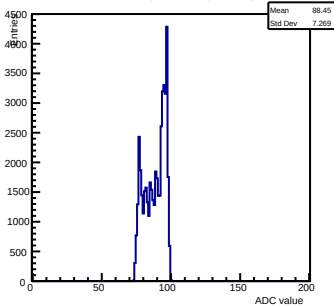
Pedestals ch 12 chip 3003 shift-gain0-shaper7
