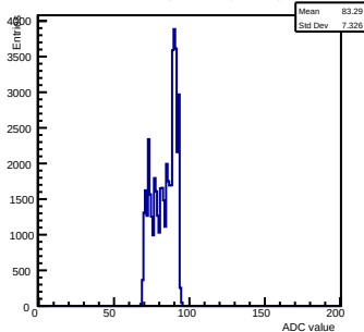
Pedestals ch 15 chip 3003 shift-gain0-shaper7
