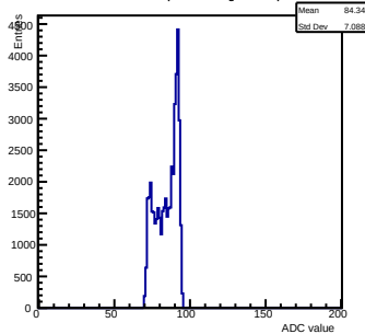
Pedestals ch 10 chip 3003 shift-gain0-shaper7
