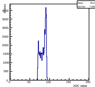
Pedestals ch 14 chip 3003 shift-gain0-shaper7
