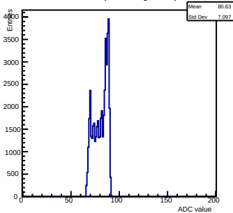
Pedestals ch 0 chip 3003 shift-gain0-shaper7
