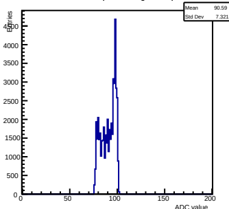
Pedestals ch 4 chip 3003 shift-gain0-shaper7
