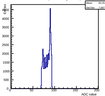
Pedestals ch 3 chip 3003 shift-gain0-shaper7
