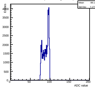
Pedestals ch 9 chip 3003 shift-gain0-shaper7
