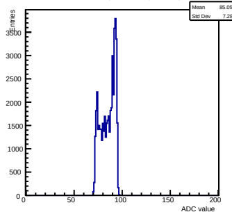
Pedestals ch 13 chip 3003 shift-gain0-shaper7
