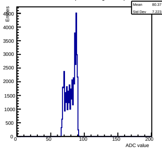
Pedestals ch 11 chip 3003 shift-gain0-shaper7
