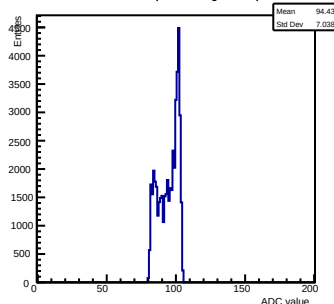
Pedestals ch 5 chip 3003 shift-gain0-shaper7
