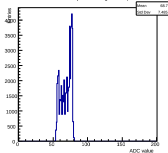
Pedestals ch 6 chip 3004 shift-gain0-shaper7
