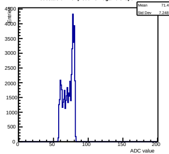
Pedestals ch 2 chip 3004 shift-gain0-shaper7
