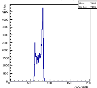
Pedestals ch 13 chip 3004 shift-gain0-shaper7
