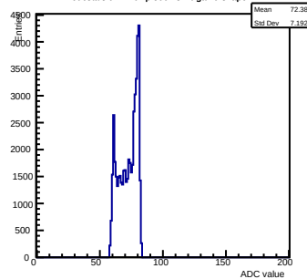
Pedestals ch 11 chip 3004 shift-gain0-shaper7
