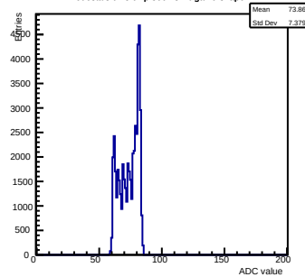
Pedestals ch 3 chip 3004 shift-gain0-shaper7
