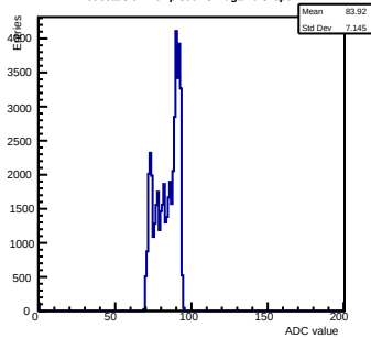
Pedestals ch 1 chip 3004 shift-gain0-shaper7
