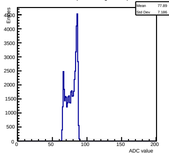
Pedestals ch 12 chip 3004 shift-gain0-shaper7
