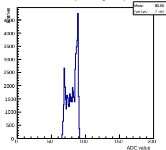
Pedestals ch 4 chip 3004 shift-gain0-shaper7
