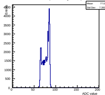
Pedestals ch 7 chip 3004 shift-gain0-shaper7
