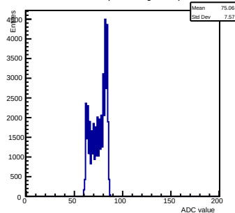
Pedestals ch 14 chip 3004 shift-gain0-shaper7
