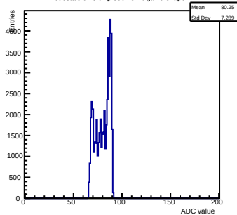
Pedestals ch 8 chip 3004 shift-gain0-shaper7
