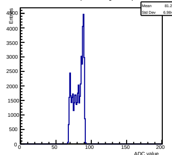
Pedestals ch 6 chip 3005 shift-gain0-shaper7
