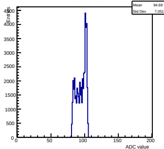
Pedestals ch 12 chip 3005 shift-gain0-shaper7
