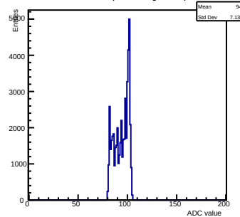
Pedestals ch 10 chip 3005 shift-gain0-shaper7
