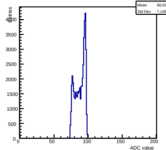
Pedestals ch 15 chip 3005 shift-gain0-shaper7
