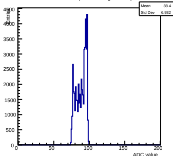
Pedestals ch 5 chip 3005 shift-gain0-shaper7
