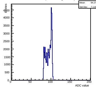
Pedestals ch 11 chip 3005 shift-gain0-shaper7
