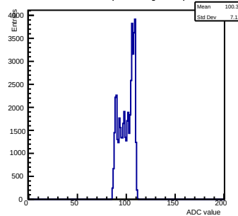
Pedestals ch 3 chip 3005 shift-gain0-shaper7
