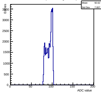
Pedestals ch 0 chip 3005 shift-gain0-shaper7
