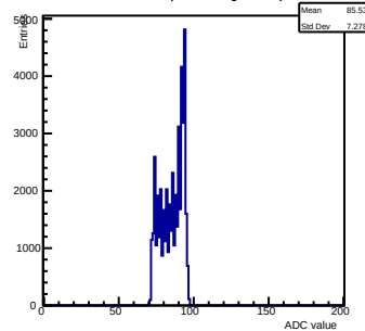
Pedestals ch 2 chip 3005 shift-gain0-shaper7
