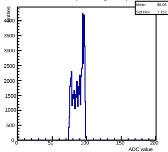
Pedestals ch 8 chip 3005 shift-gain0-shaper7
