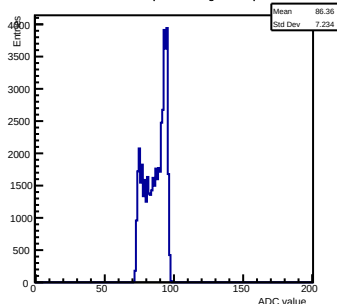
Pedestals ch 4 chip 3005 shift-gain0-shaper7
