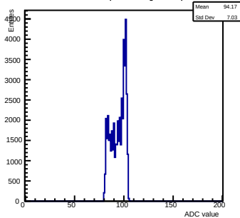
Pedestals ch 1 chip 3005 shift-gain0-shaper7
