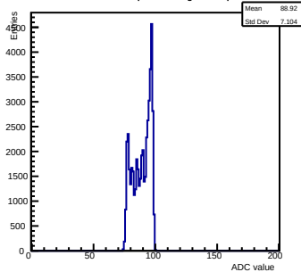
Pedestals ch 9 chip 3005 shift-gain0-shaper7
