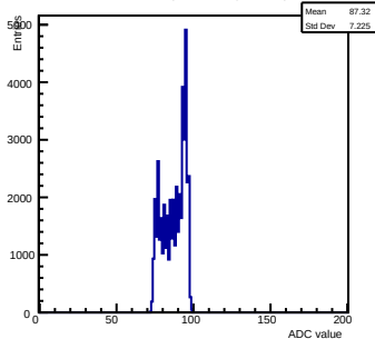
Pedestals ch 13 chip 3005 shift-gain0-shaper7
