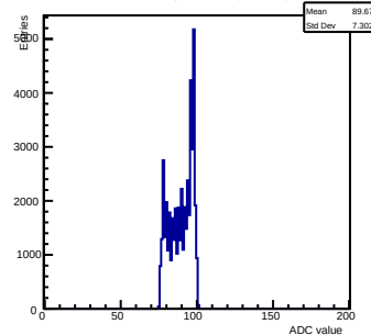
Pedestals ch 14 chip 3005 shift-gain0-shaper7
