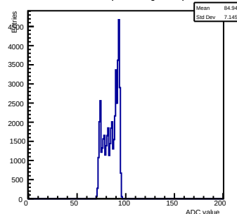
Pedestals ch 7 chip 3005 shift-gain0-shaper7
