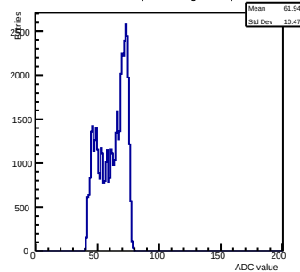
Pedestals ch 3 chip 3005 shift-gain3-shaper7
