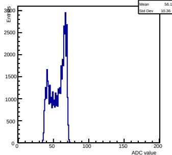
Pedestals ch 12 chip 3005 shift-gain3-shaper7
