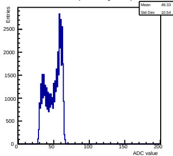
Pedestals ch 1 chip 3005 shift-gain3-shaper7
