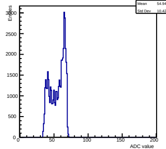
Pedestals ch 11 chip 3005 shift-gain3-shaper7
