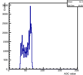
Pedestals ch 10 chip 3005 shift-gain3-shaper7
