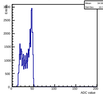
Pedestals ch 7 chip 3005 shift-gain3-shaper7
