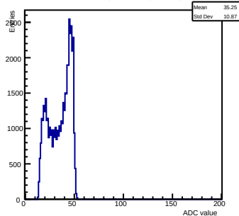
Pedestals ch 4 chip 3005 shift-gain3-shaper7
