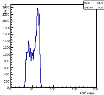
Pedestals ch 0 chip 3005 shift-gain3-shaper7
