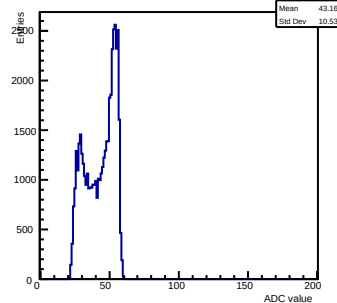
Pedestals ch 15 chip 3005 shift-gain3-shaper7
