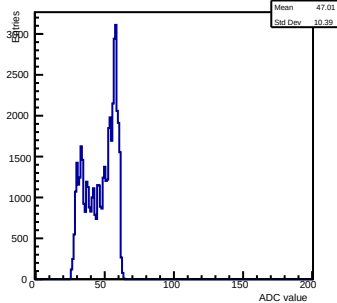
Pedestals ch 9 chip 3005 shift-gain3-shaper7
