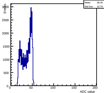
Pedestals ch 13 chip 3005 shift-gain3-shaper7
