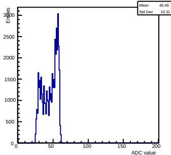
Pedestals ch 5 chip 3005 shift-gain3-shaper7
