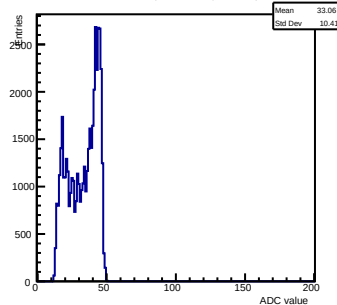
Pedestals ch 6 chip 3005 shift-gain3-shaper7
