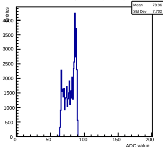
Pedestals ch 7 chip 3006 shift-gain0-shaper7
