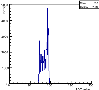
Pedestals ch 4 chip 3006 shift-gain0-shaper7
