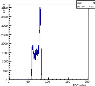
Pedestals ch 12 chip 3006 shift-gain0-shaper7
