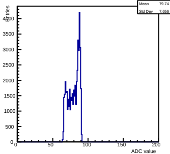
Pedestals ch 9 chip 3006 shift-gain0-shaper7
