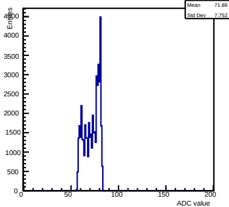
Pedestals ch 11 chip 3006 shift-gain0-shaper7
