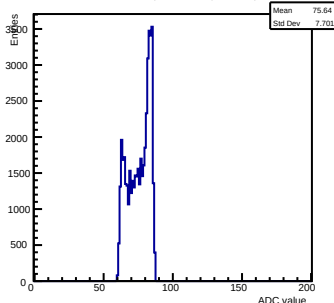
Pedestals ch 15 chip 3006 shift-gain0-shaper7
