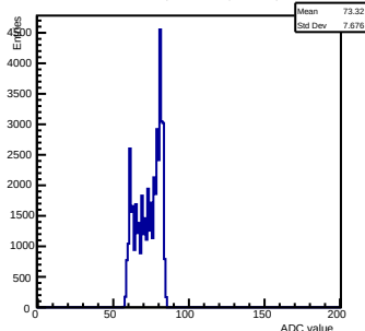
Pedestals ch 6 chip 3006 shift-gain0-shaper7
