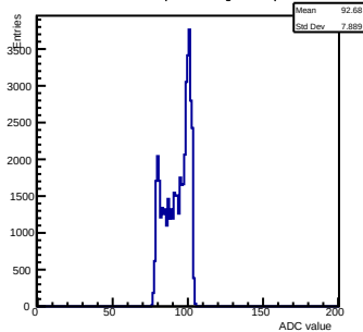
Pedestals ch 2 chip 3006 shift-gain0-shaper7
