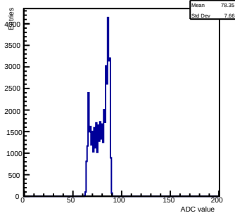
Pedestals ch 10 chip 3006 shift-gain0-shaper7
