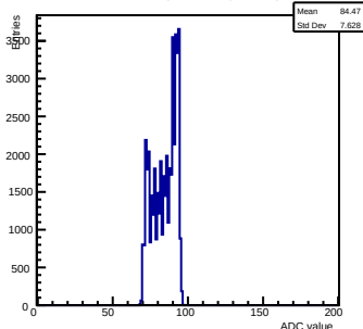
Pedestals ch 13 chip 3006 shift-gain0-shaper7
