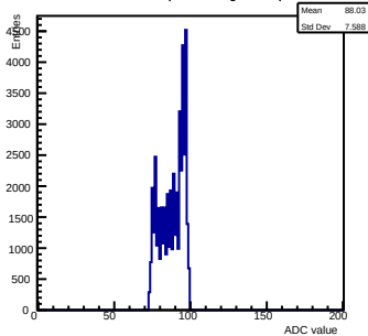
Pedestals ch 1 chip 3006 shift-gain0-shaper7
