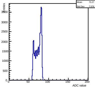
Pedestals ch 8 chip 3006 shift-gain0-shaper7
