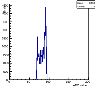
Pedestals ch 14 chip 3006 shift-gain0-shaper7
