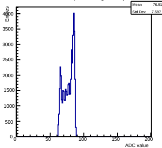
Pedestals ch 3 chip 3006 shift-gain0-shaper7
