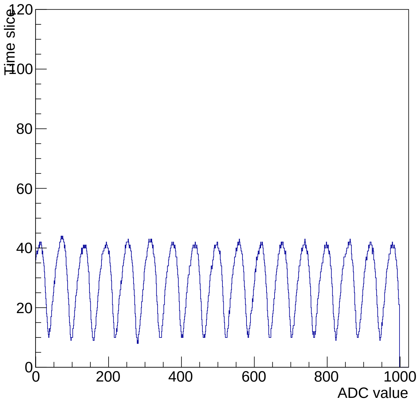
Evt 10 Time mcm 3000 chip 0 chan 9 1000-shift-gain3-shaper0
