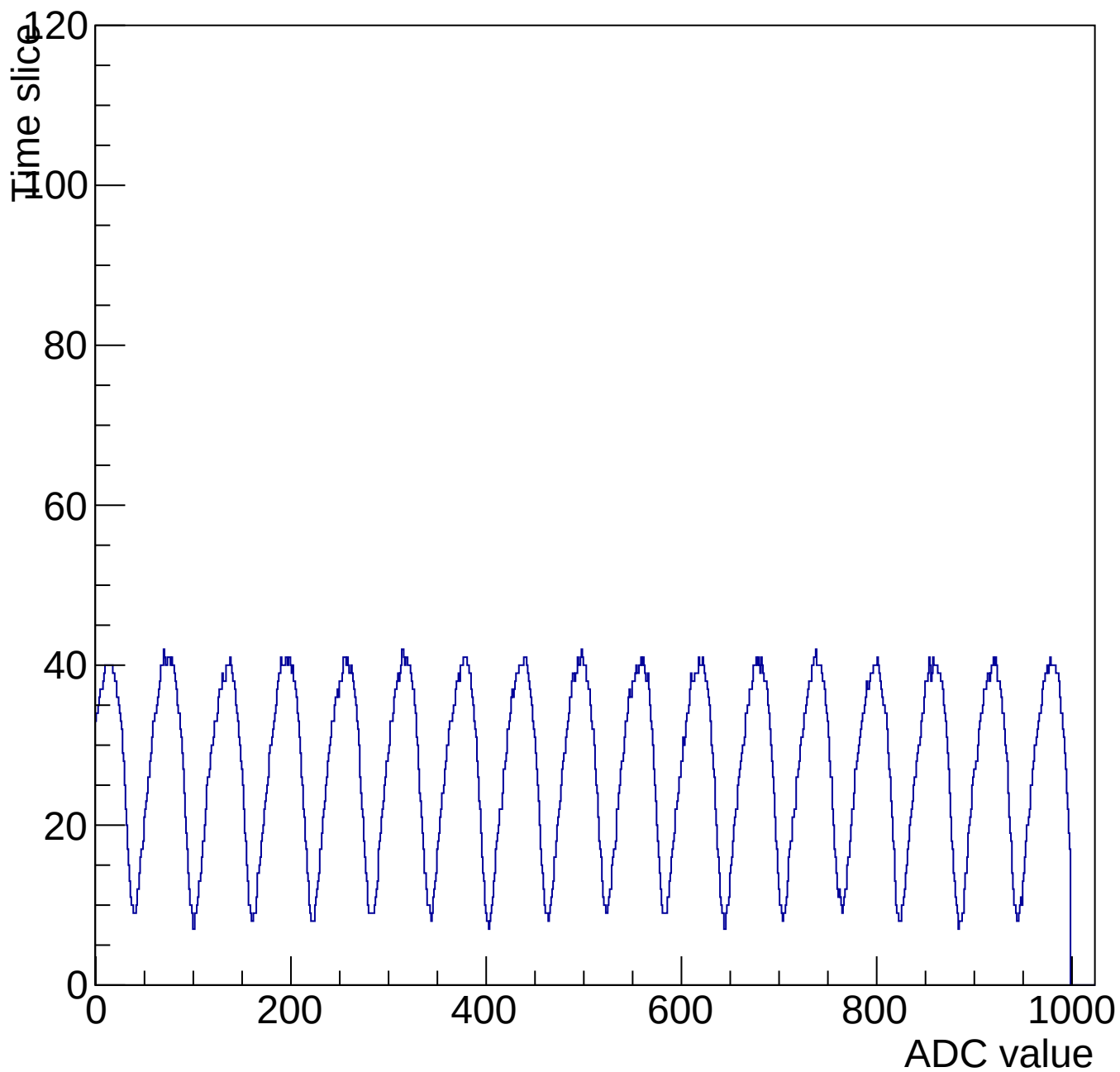
Evt 10 Time mcm 3000 chip 0 chan 7 1000-shift-gain3-shaper0
