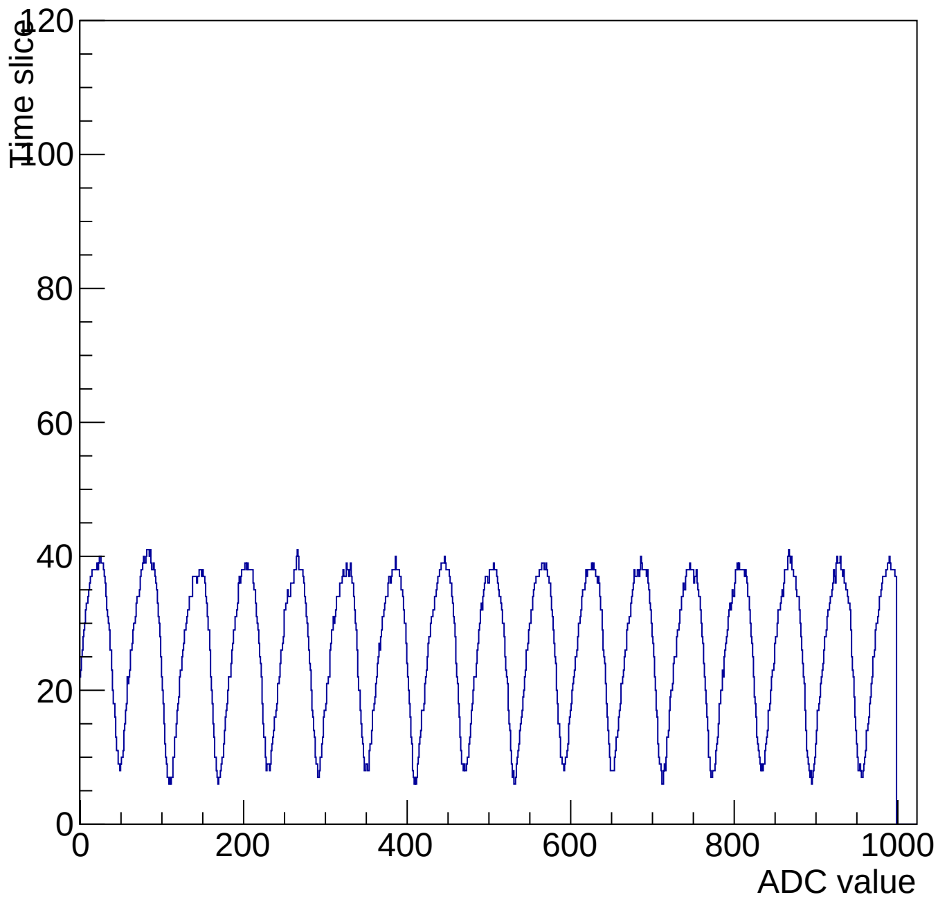
Evt 10 Time mcm 3000 chip 0 chan 3 1000-shift-gain3-shaper0
