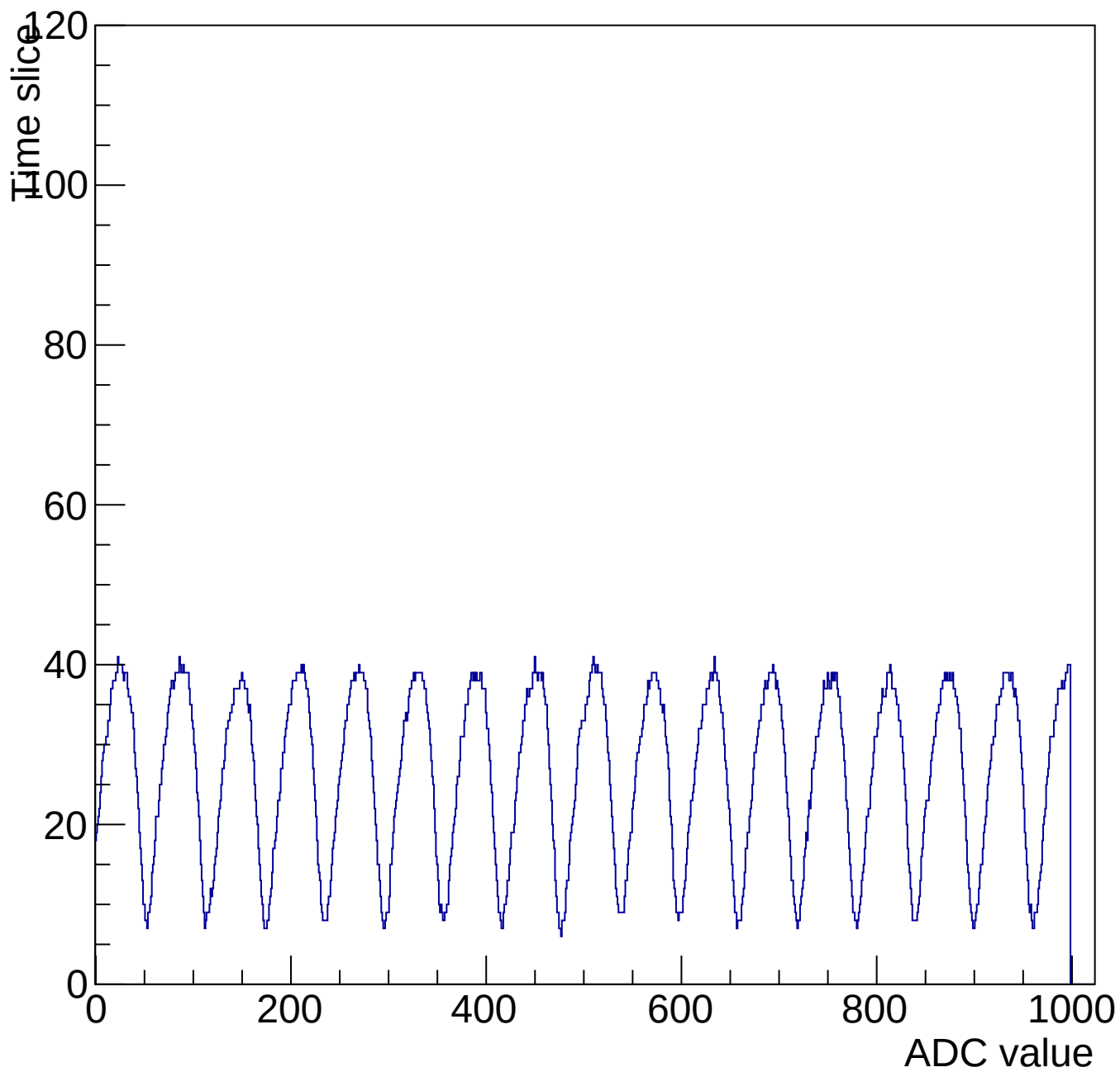
Evt 10 Time mcm 3000 chip 0 chan 15 1000-shift-gain3-shaper0
