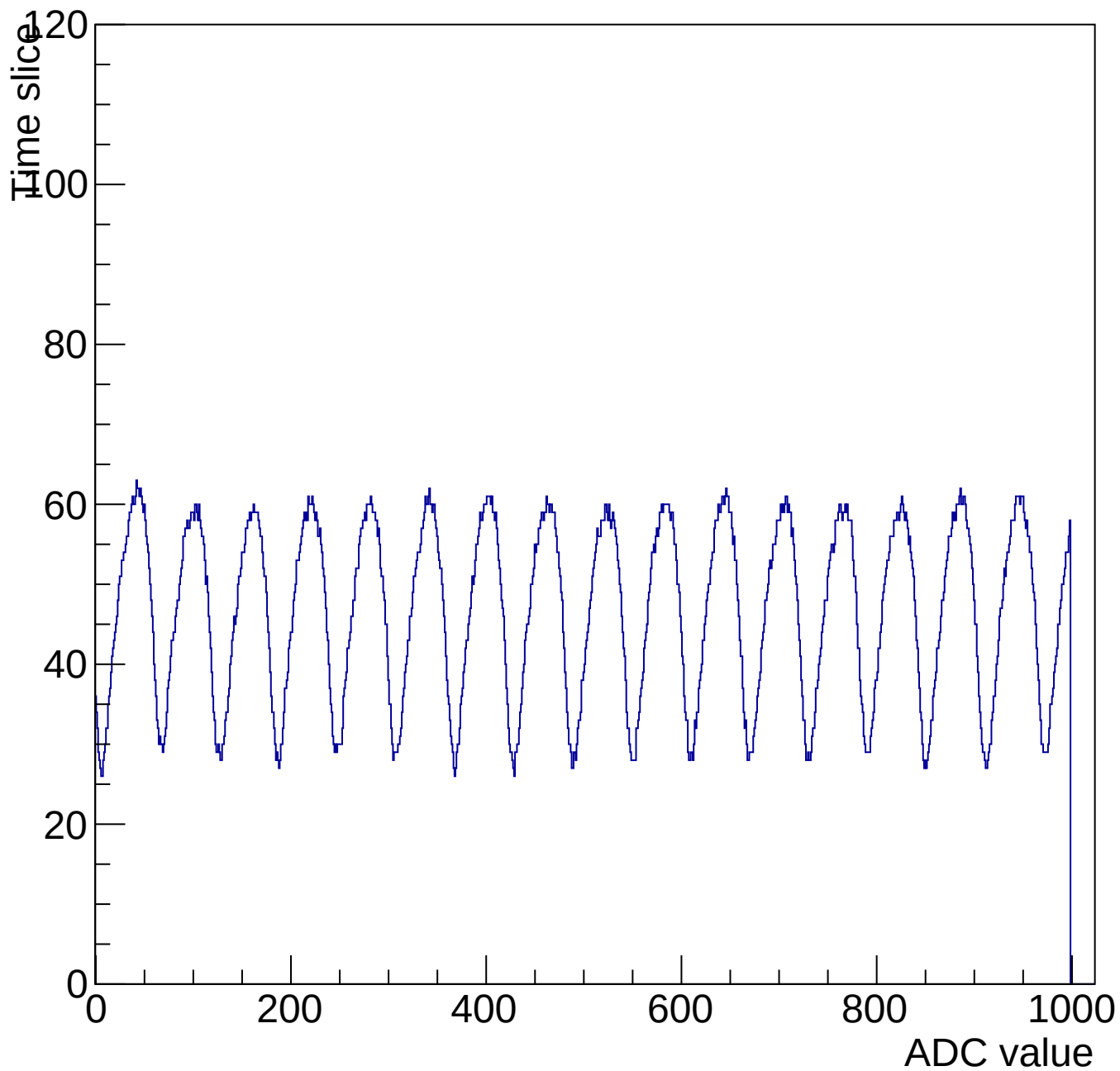
Evt 10 Time mcm 3000 chip 0 chan 4 1000-shift-gain3-shaper0
