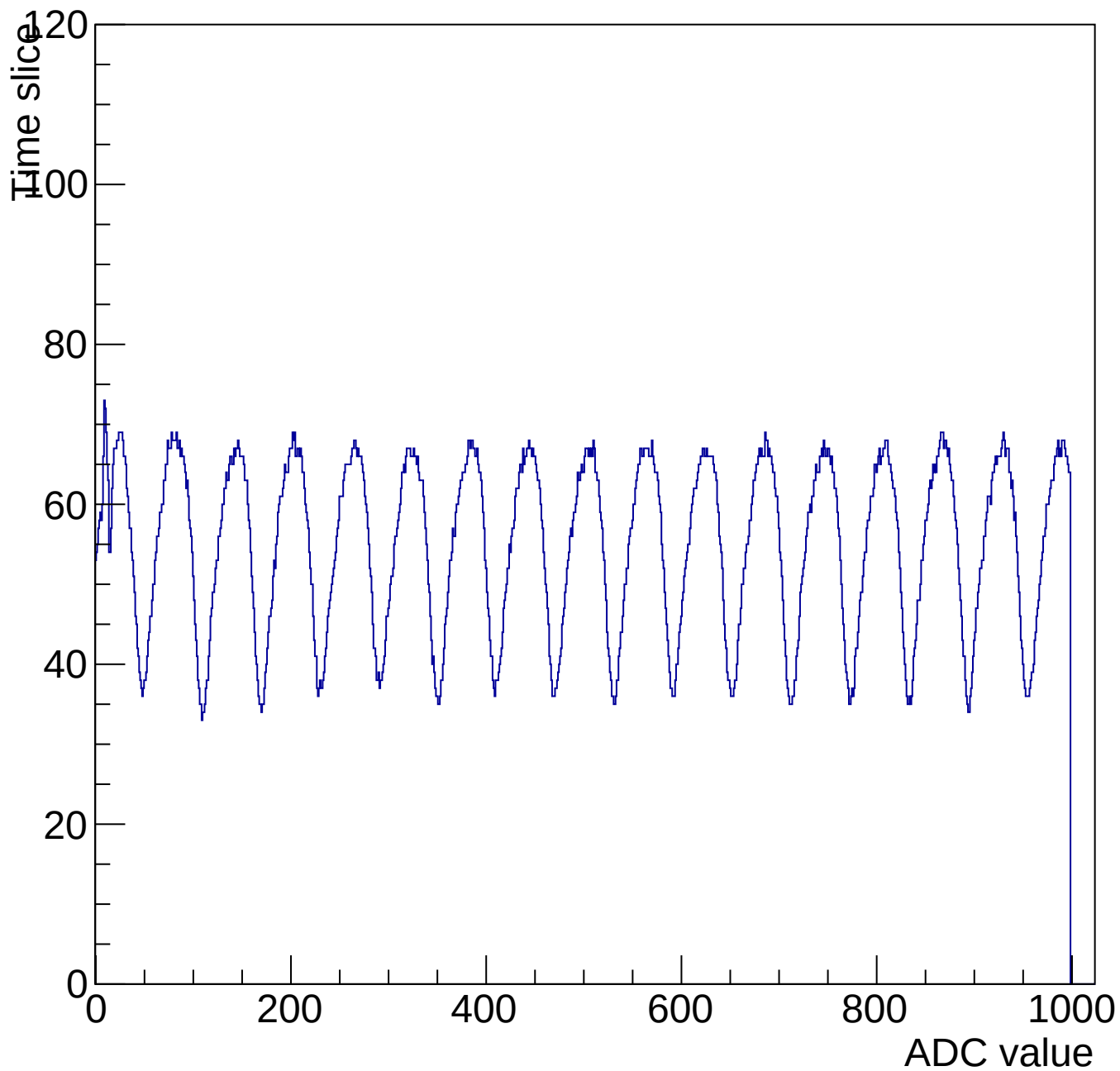
Evt 10 Time mcm 3000 chip 0 chan 2 1000-shift-gain3-shaper0
