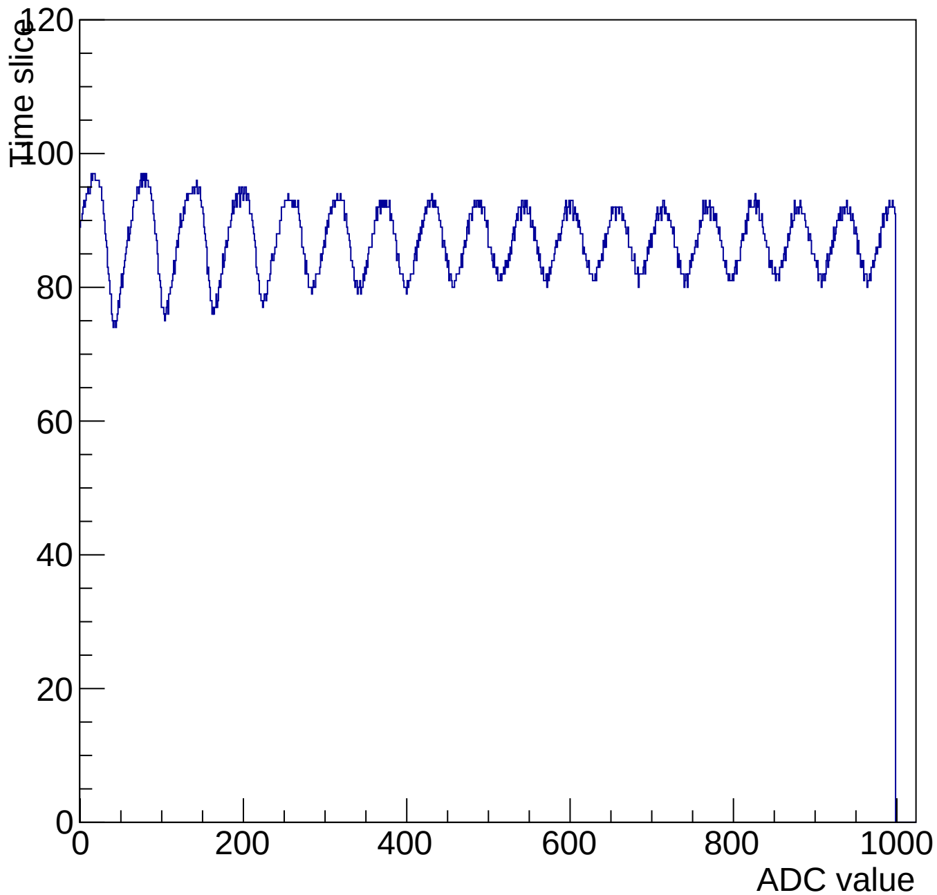
Evt 10 Time mcm 3000 chip 0 chan 0 1000-shift-gain0-shaper7
