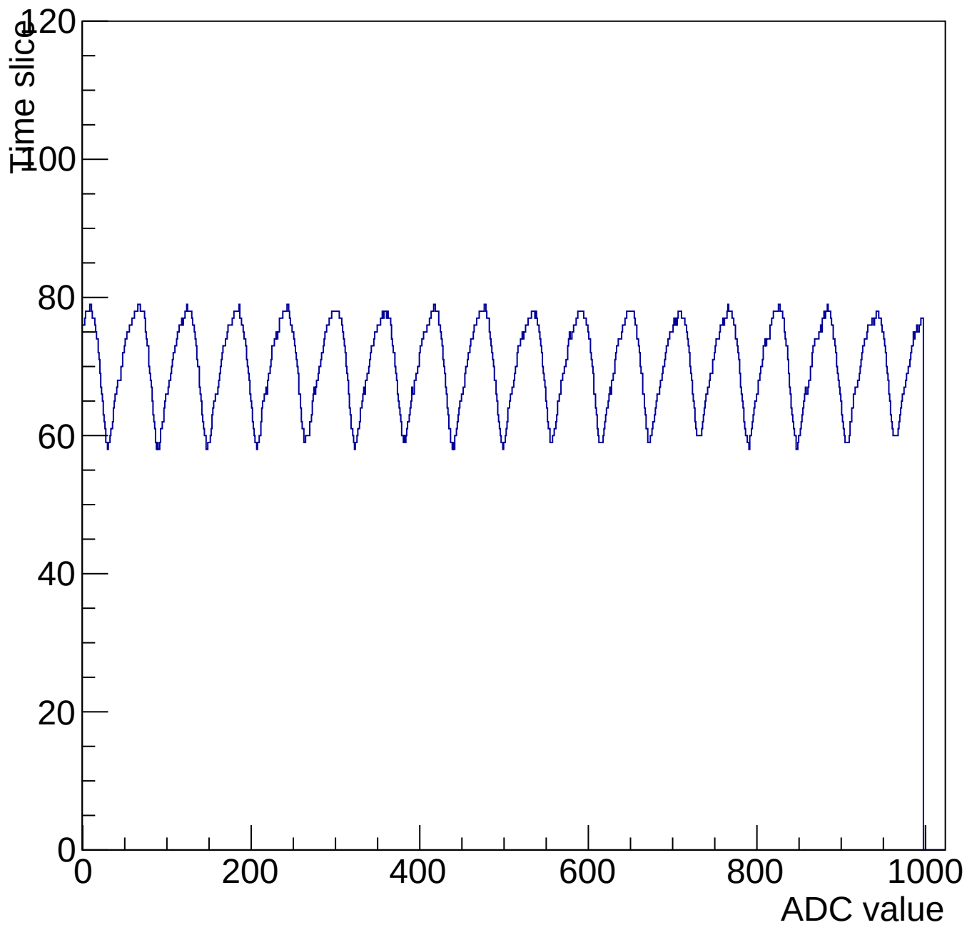
Evt 10 Time mcm 3001 chip 1 chan 11 1000-shift-gain0-shaper0
