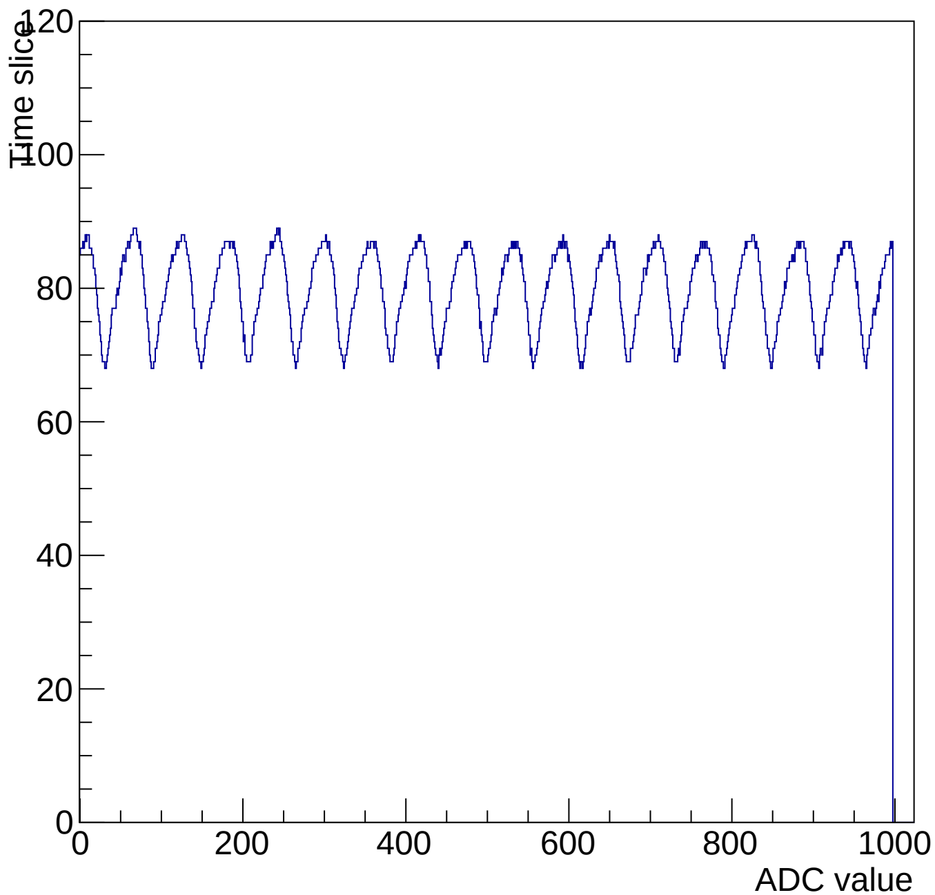
Evt 10 Time mcm 3001 chip 1 chan 10 1000-shift-gain0-shaper0
