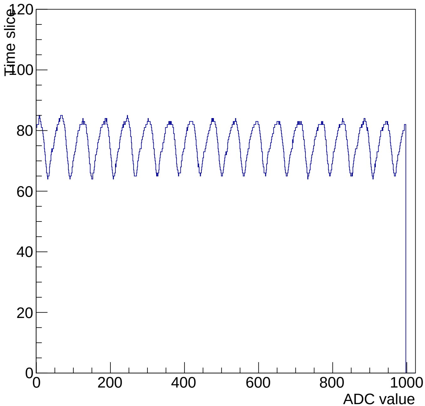
Evt 10 Time mcm 3001 chip 1 chan 14 1000-shift-gain0-shaper0
