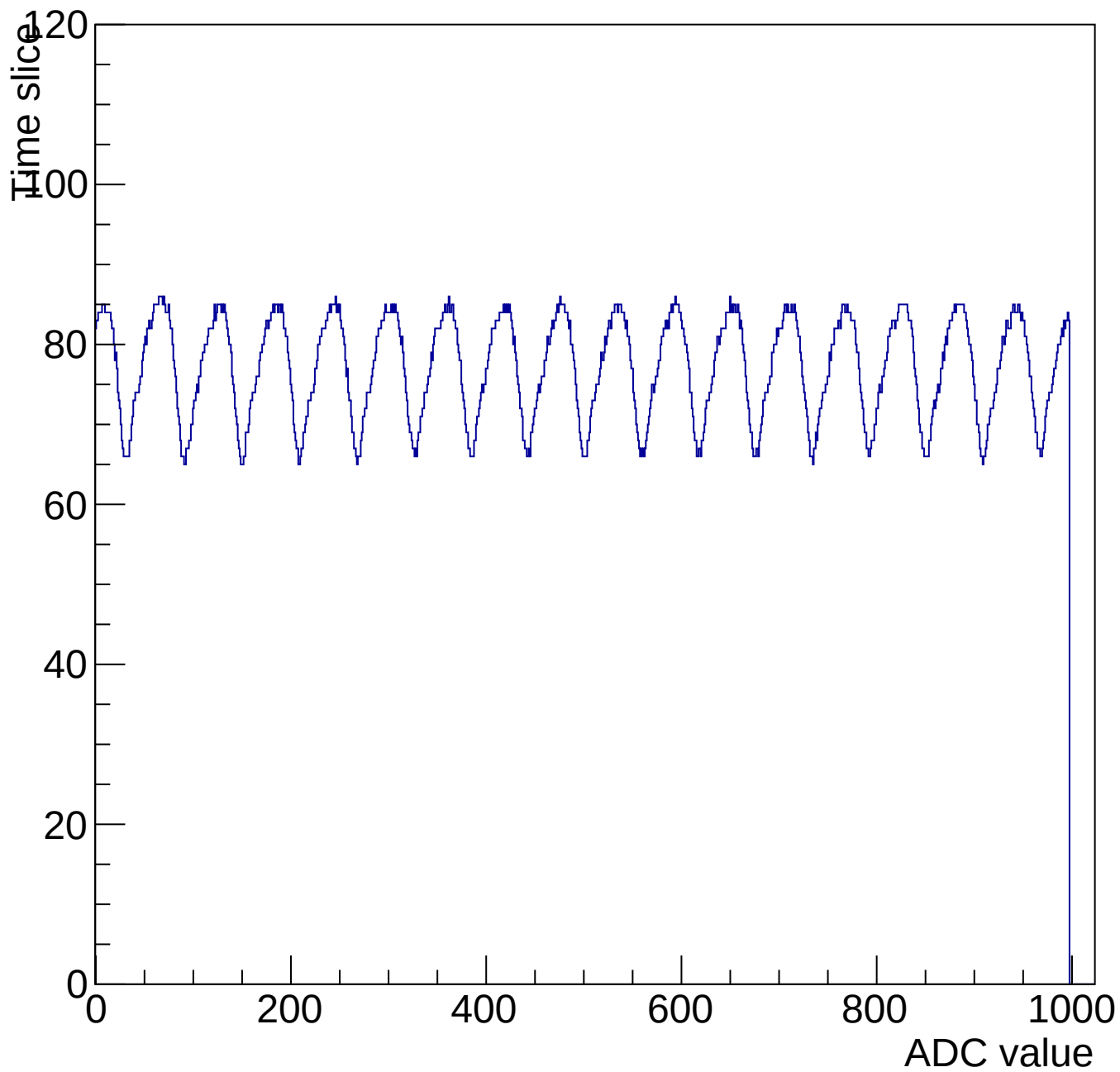
Evt 10 Time mcm 3001 chip 1 chan 15 1000-shift-gain0-shaper0
