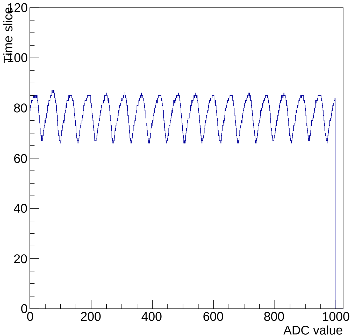
Evt 10 Time mcm 3001 chip 1 chan 5 1000-shift-gain0-shaper0
