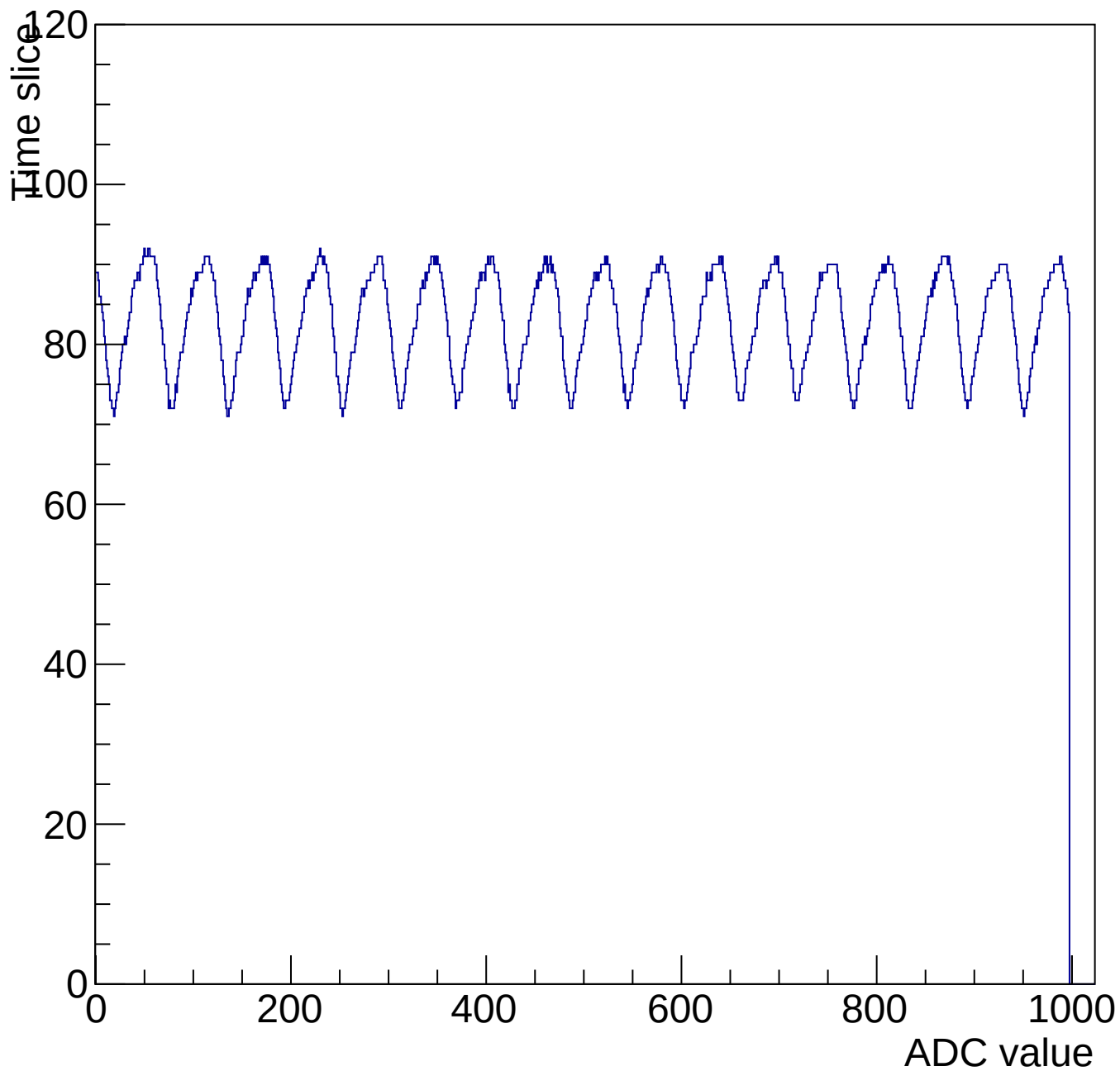
Evt 10 Time mcm 3001 chip 1 chan 0 1000-shift-gain0-shaper0
