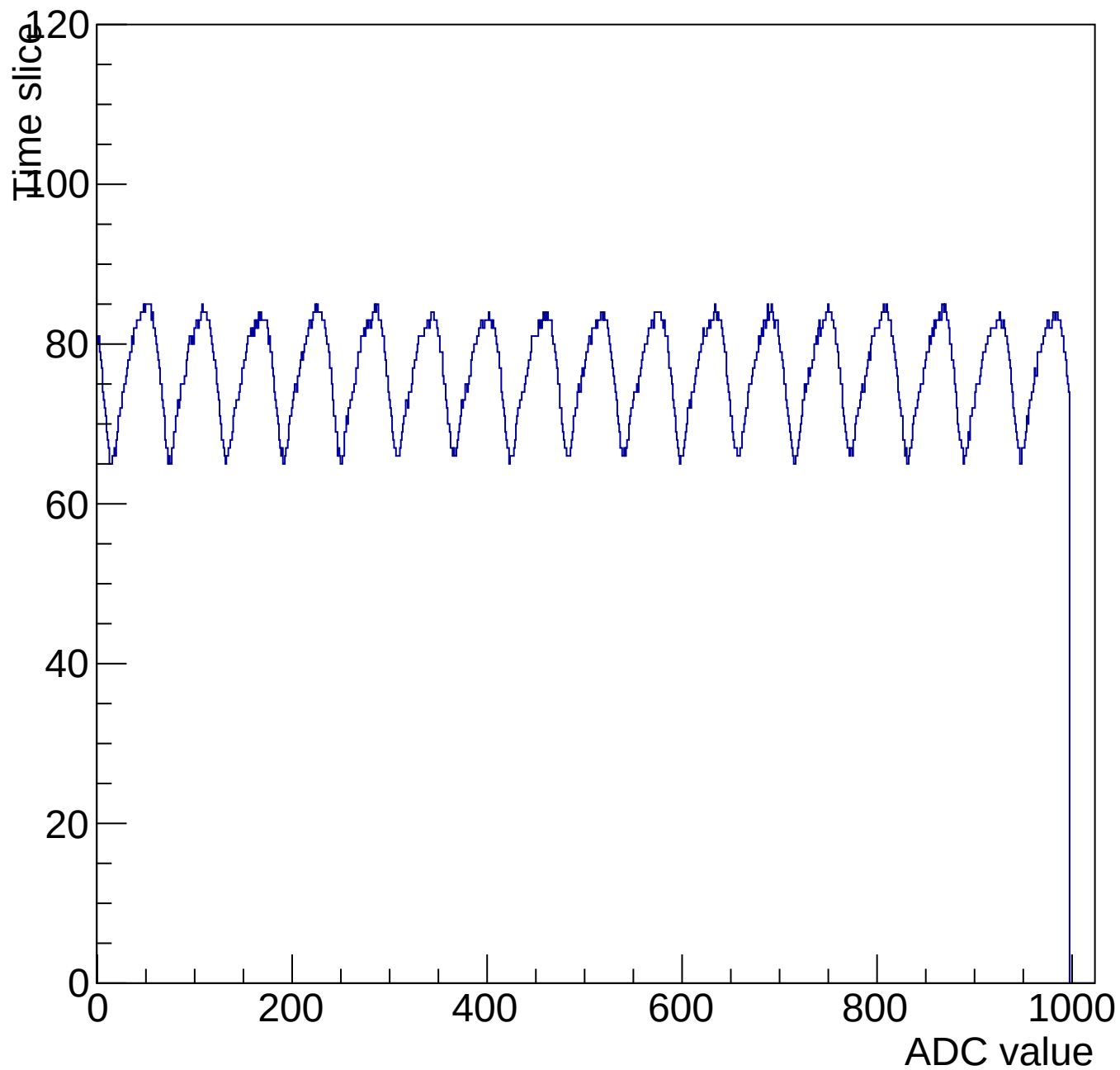
Evt 10 Time mcm 3001 chip 1 chan 3 1000-shift-gain0-shaper0
