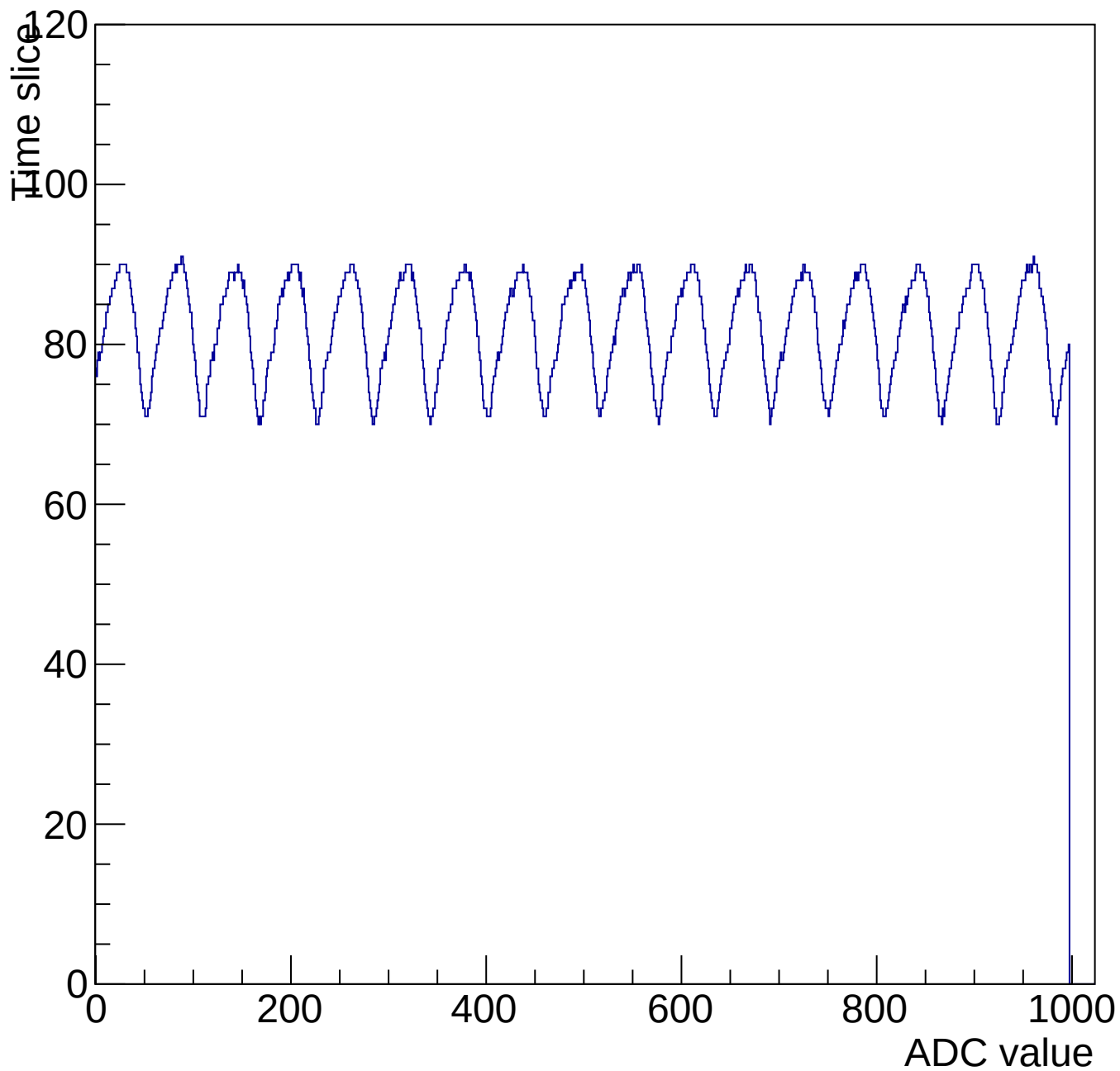
Evt 10 Time mcm 3001 chip 1 chan 12 1000-shift-gain0-shaper0
