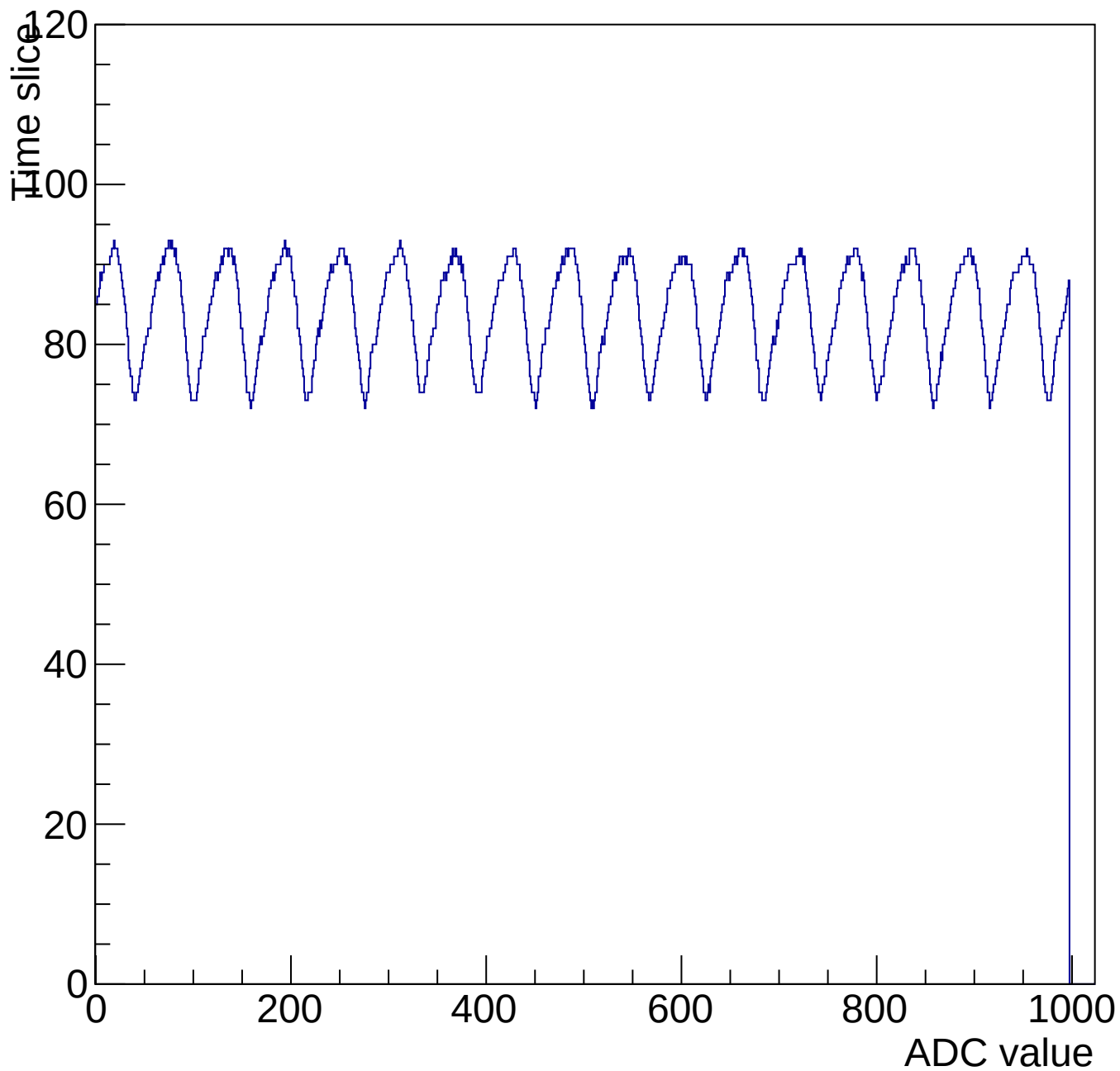
Evt 10 Time mcm 3001 chip 1 chan 7 1000-shift-gain0-shaper0
