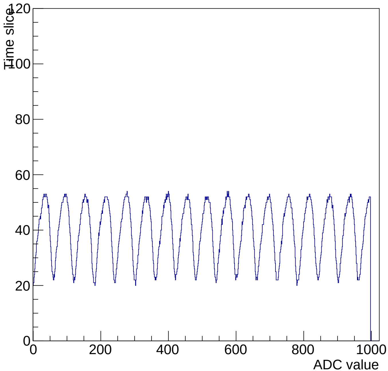
Evt 10 Time mcm 3001 chip 1 chan 6 1000-shift-gain3-shaper0
