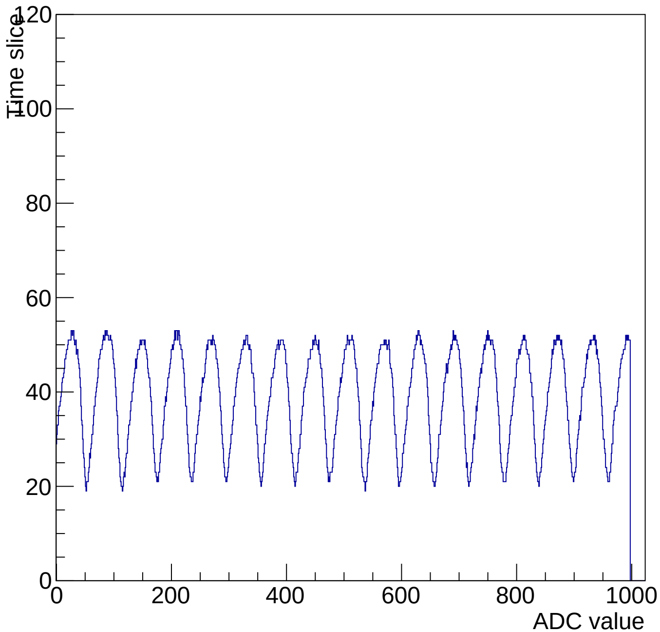
Evt 10 Time mcm 3001 chip 1 chan 10 1000-shift-gain3-shaper0
