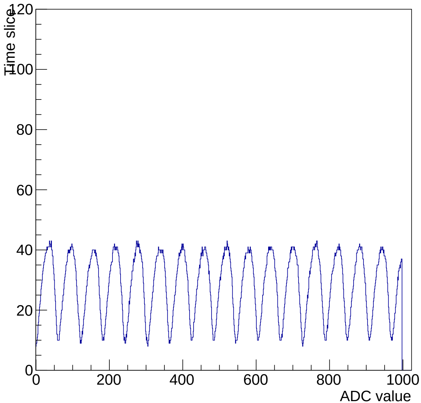
Evt 10 Time mcm 3001 chip 1 chan 4 1000-shift-gain3-shaper0
