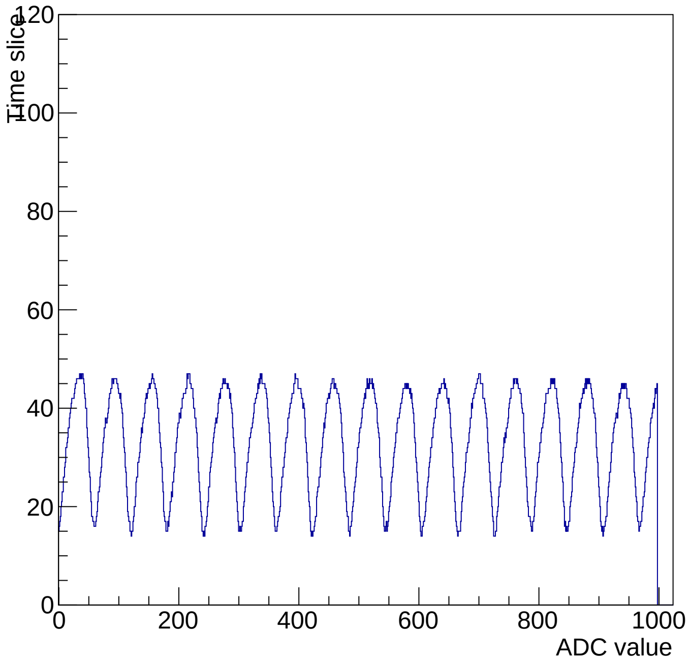
Evt 10 Time mcm 3001 chip 1 chan 9 1000-shift-gain3-shaper0
