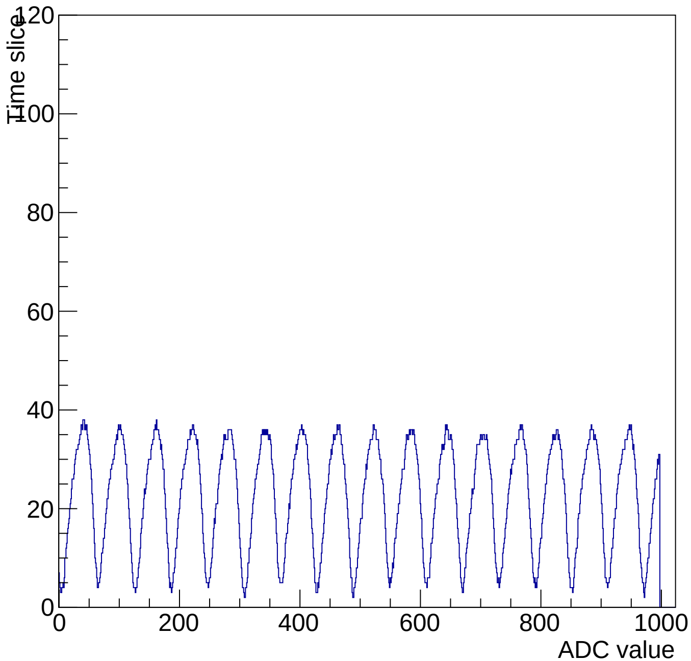
Evt 10 Time mcm 3001 chip 1 chan 2 1000-shift-gain3-shaper0
