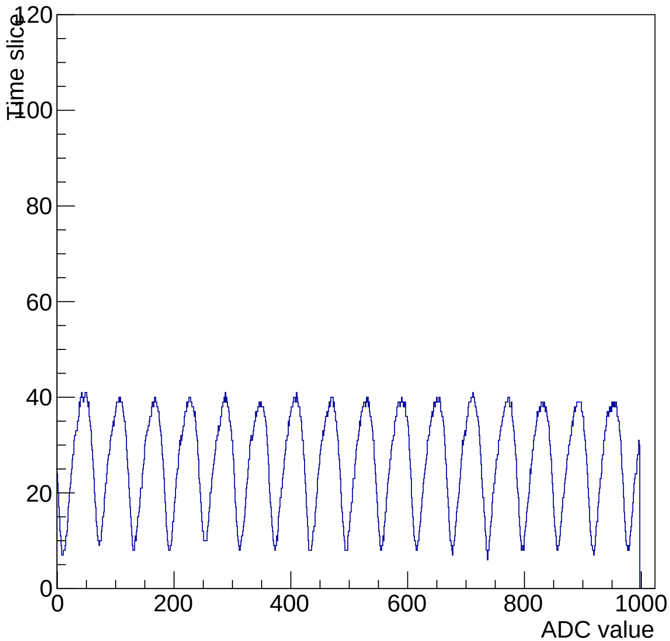
Evt 10 Time mcm 3001 chip 1 chan 13 1000-shift-gain3-shaper0
