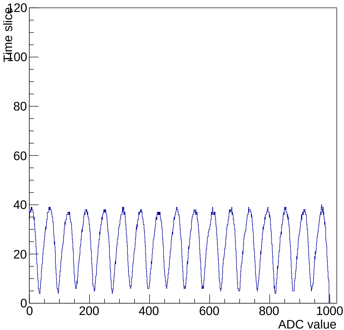
Evt 10 Time mcm 3001 chip 1 chan 15 1000-shift-gain3-shaper0
