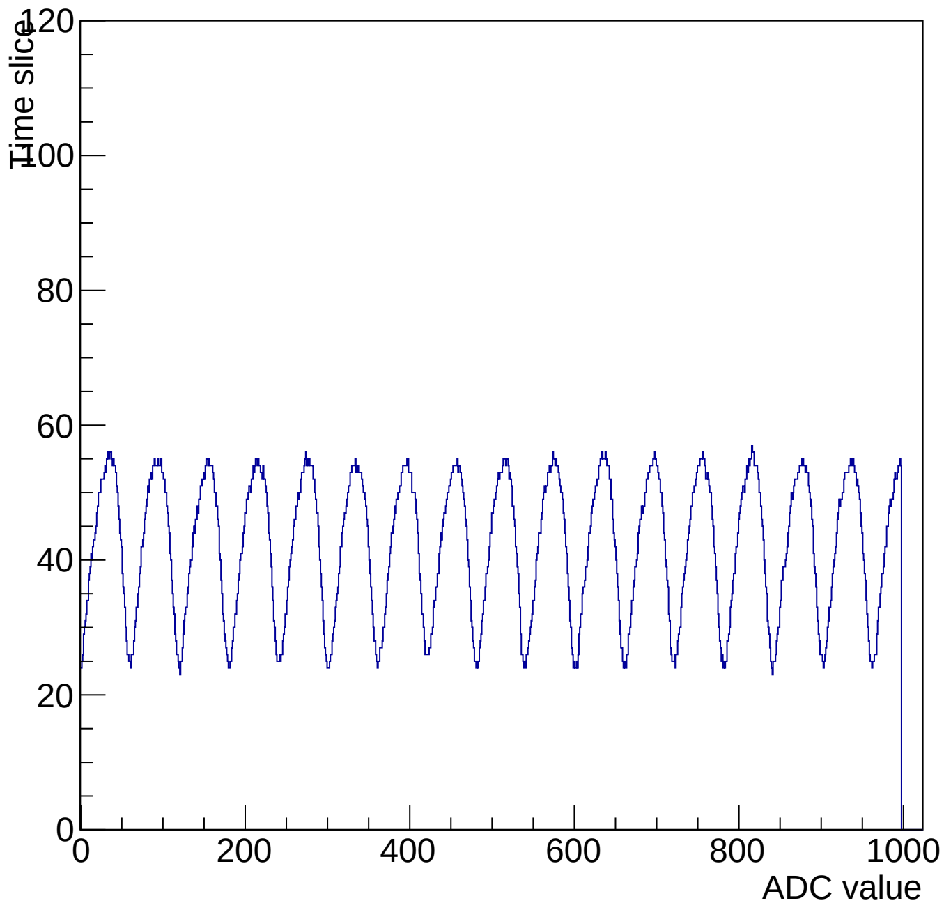
Evt 10 Time mcm 3001 chip 1 chan 7 1000-shift-gain3-shaper0
