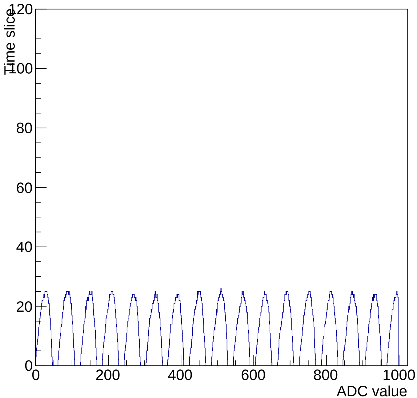
Evt 10 Time mcm 3001 chip 1 chan 11 1000-shift-gain3-shaper0
