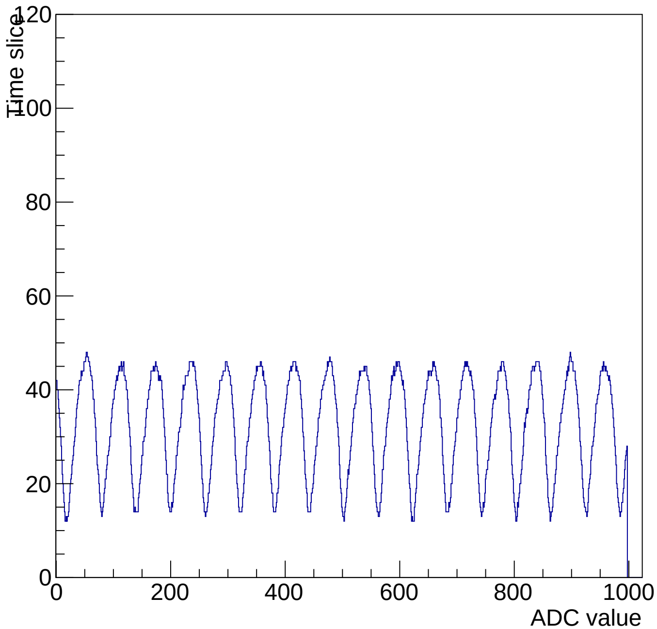
Evt 10 Time mcm 3001 chip 1 chan 1 1000-shift-gain3-shaper0
