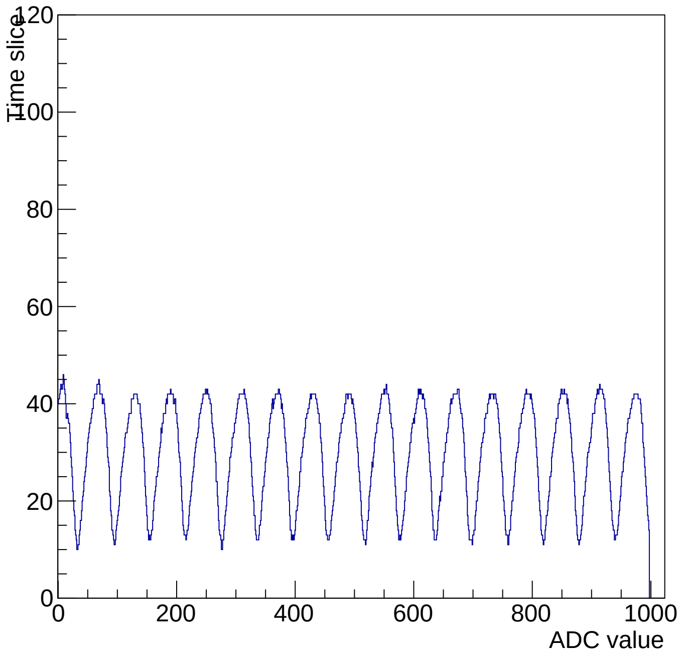
Evt 10 Time mcm 3001 chip 1 chan 14 1000-shift-gain3-shaper0
