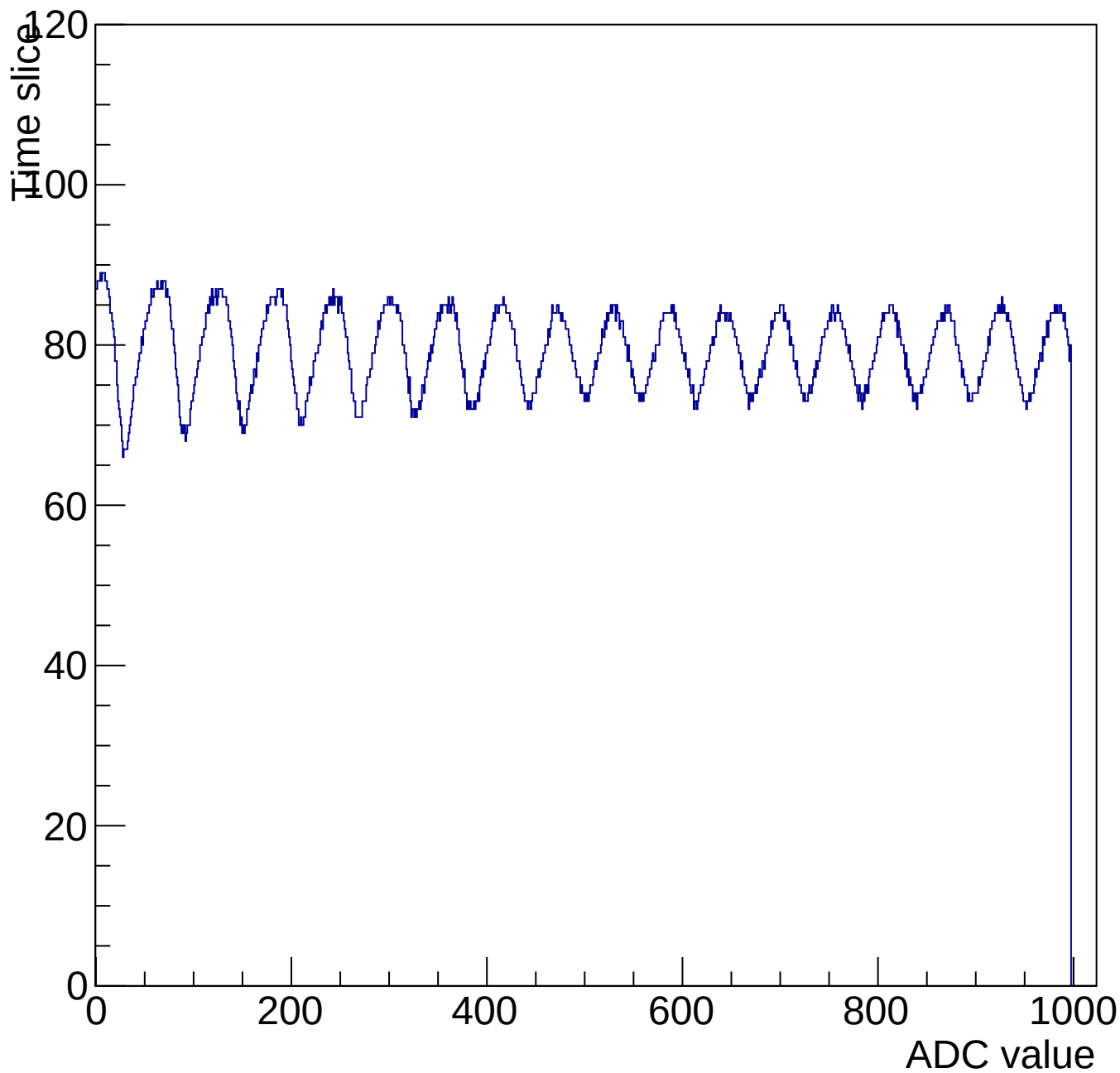
Evt 10 Time mcm 3001 chip 1 chan 9 1000-shift-gain0-shaper7
