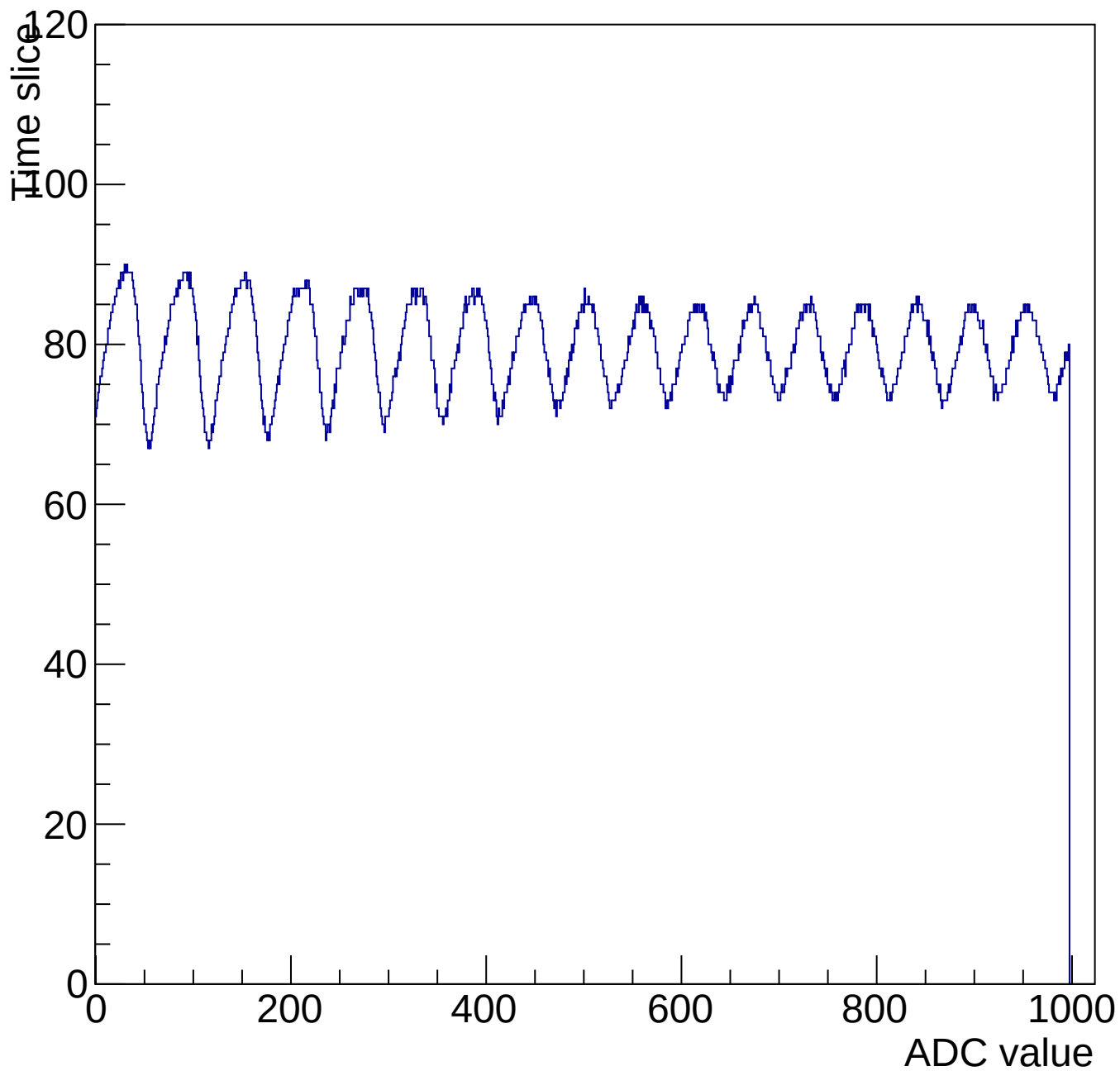
Evt 10 Time mcm 3001 chip 1 chan 5 1000-shift-gain0-shaper7
