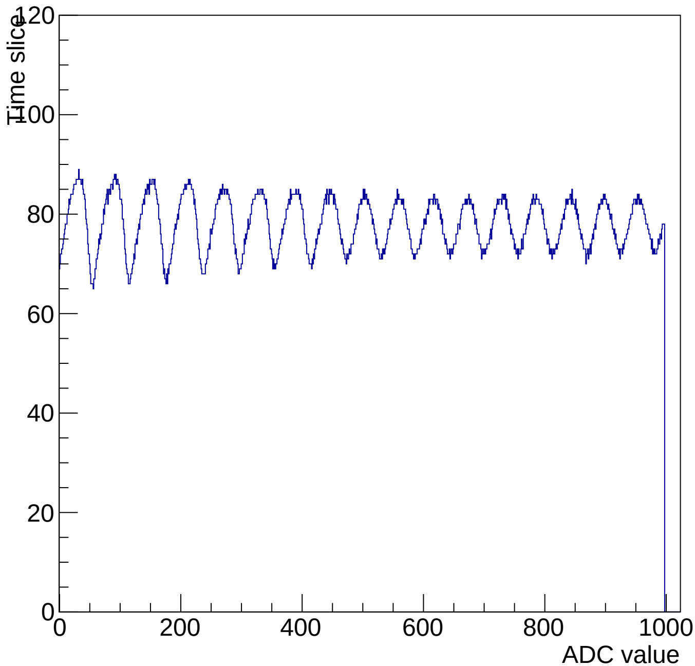
Evt 10 Time mcm 3001 chip 1 chan 4 1000-shift-gain0-shaper7
