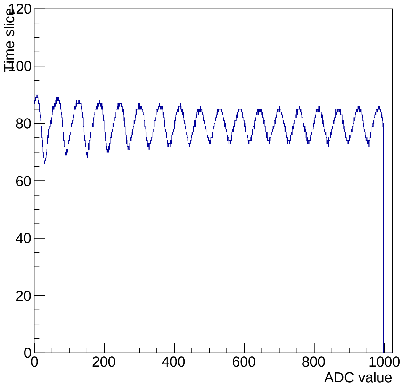
Evt 10 Time mcm 3001 chip 1 chan 8 1000-shift-gain0-shaper7
