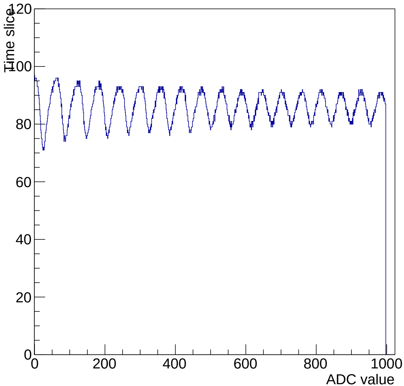
Evt 10 Time mcm 3001 chip 1 chan 0 1000-shift-gain0-shaper7
