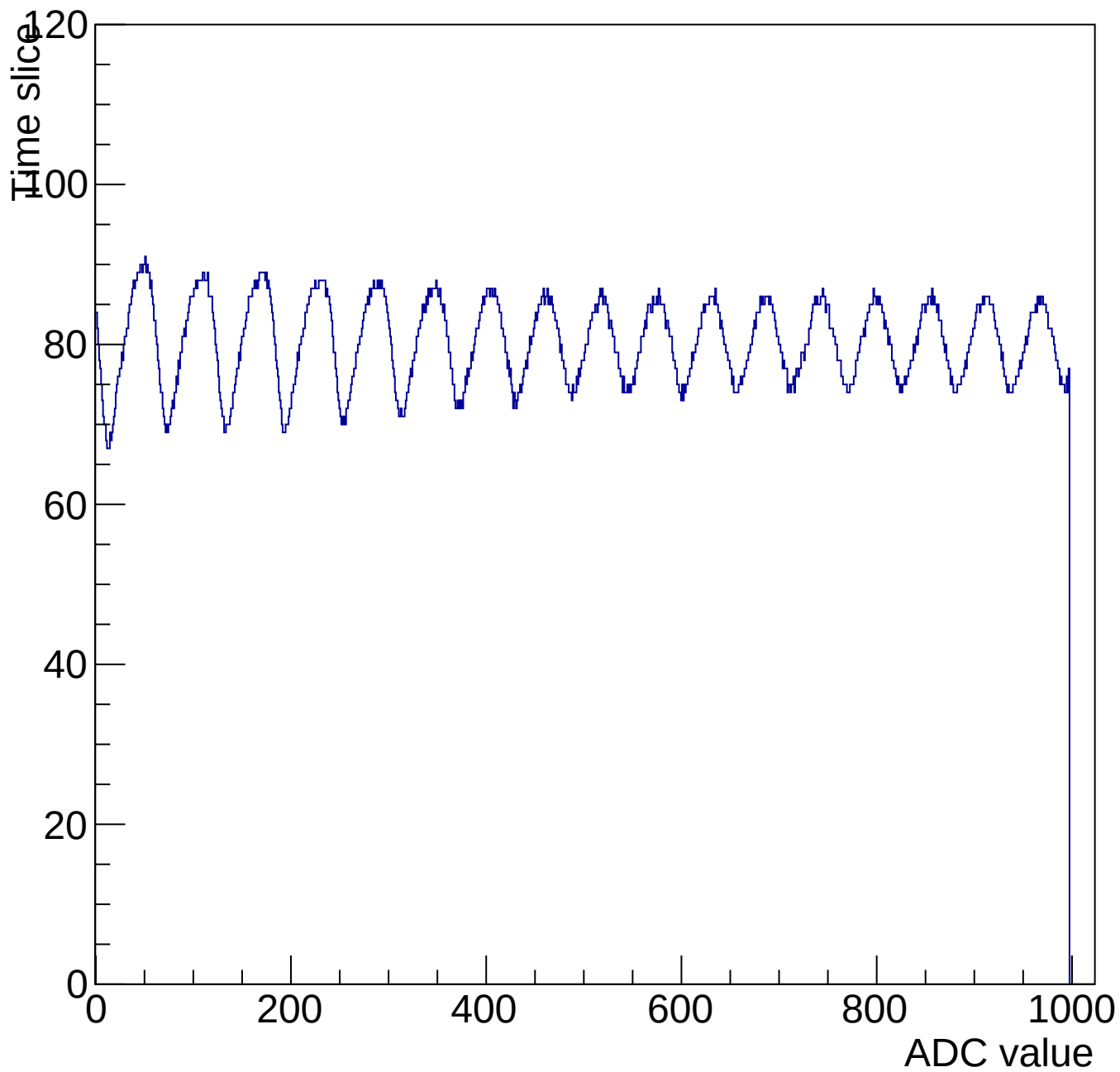
Evt 10 Time mcm 3001 chip 1 chan 12 1000-shift-gain0-shaper7
