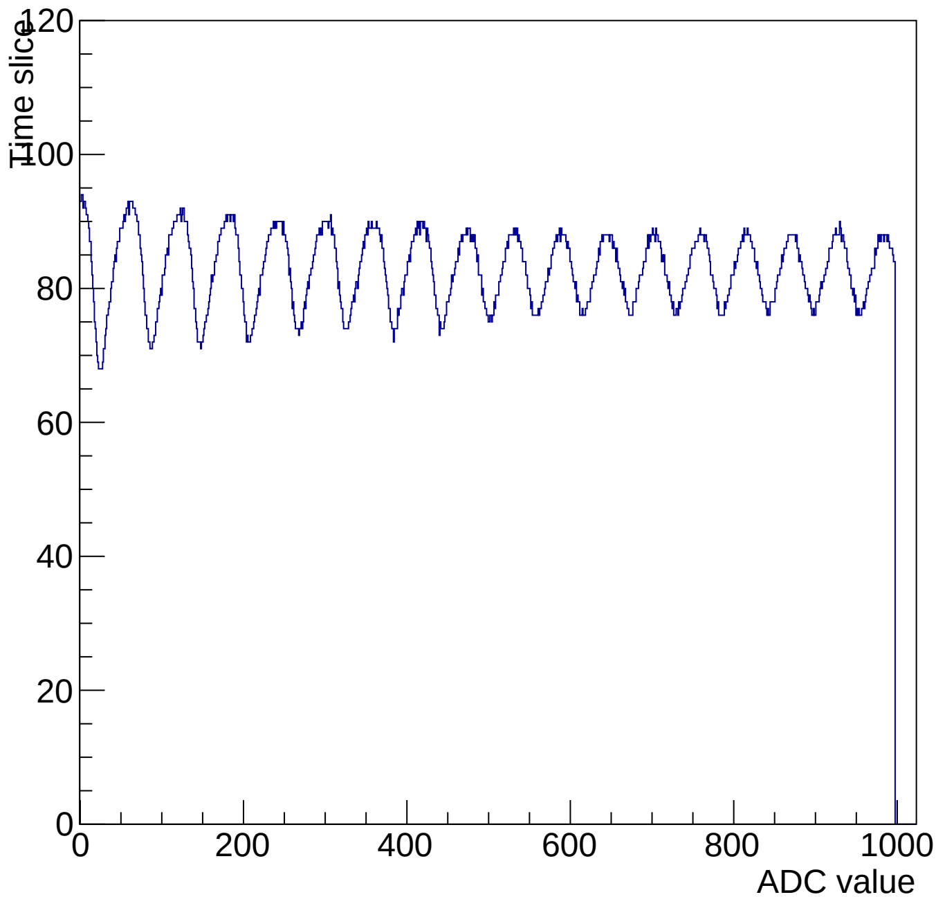
Evt 10 Time mcm 3001 chip 1 chan 1 1000-shift-gain0-shaper7
