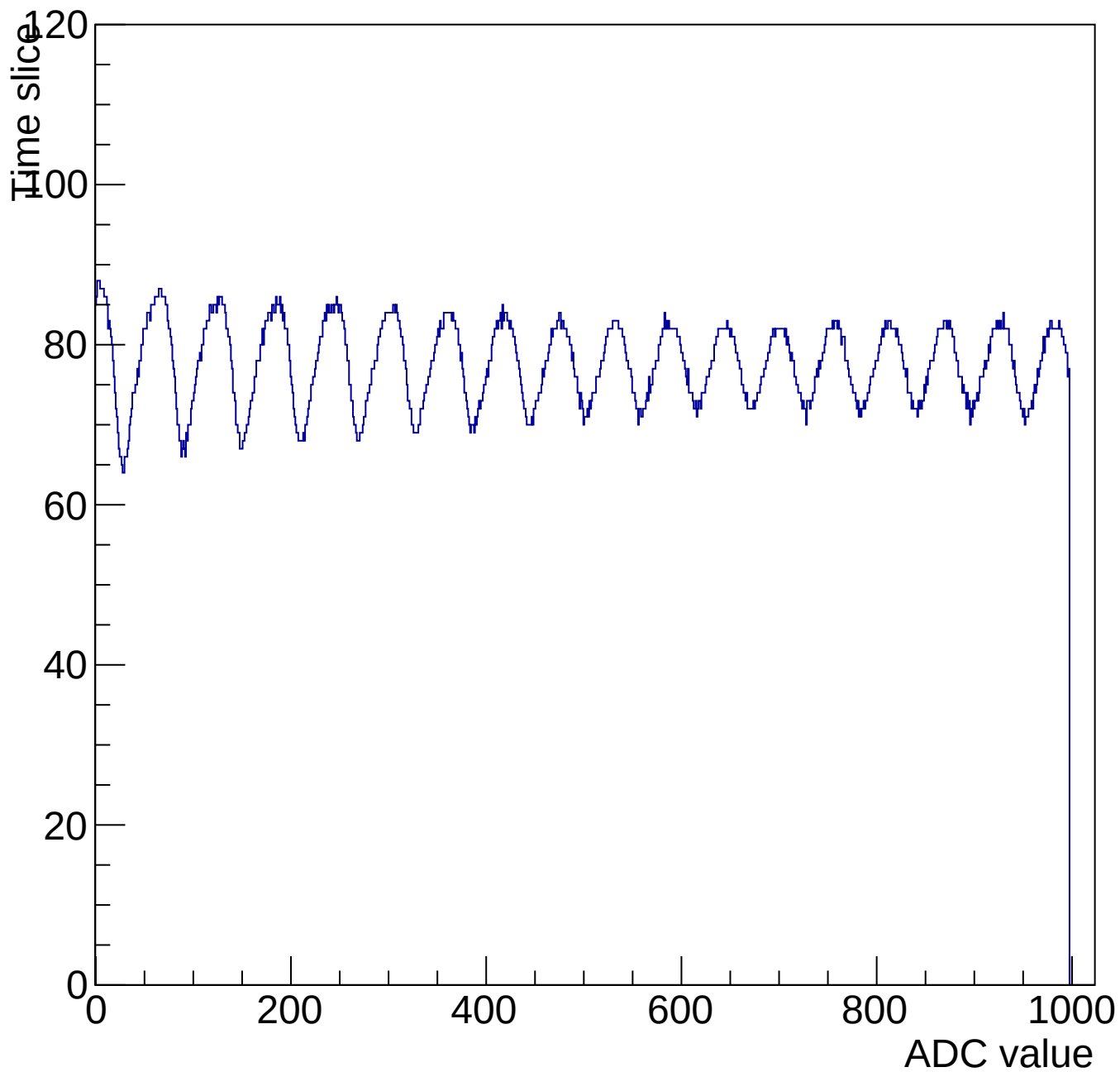
Evt 10 Time mcm 3001 chip 1 chan 14 1000-shift-gain0-shaper7
