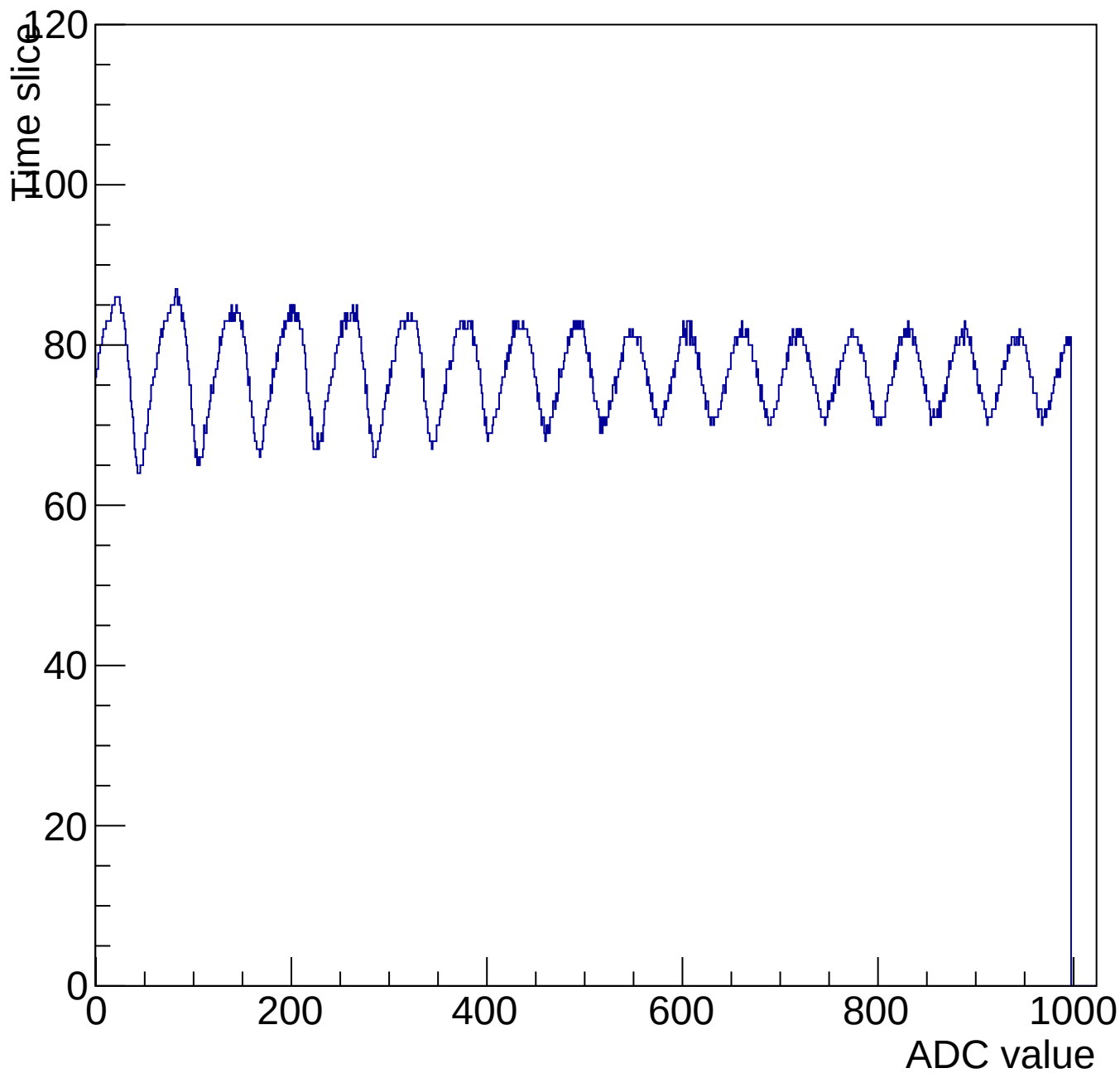
Evt 10 Time mcm 3001 chip 1 chan 3 1000-shift-gain0-shaper7
