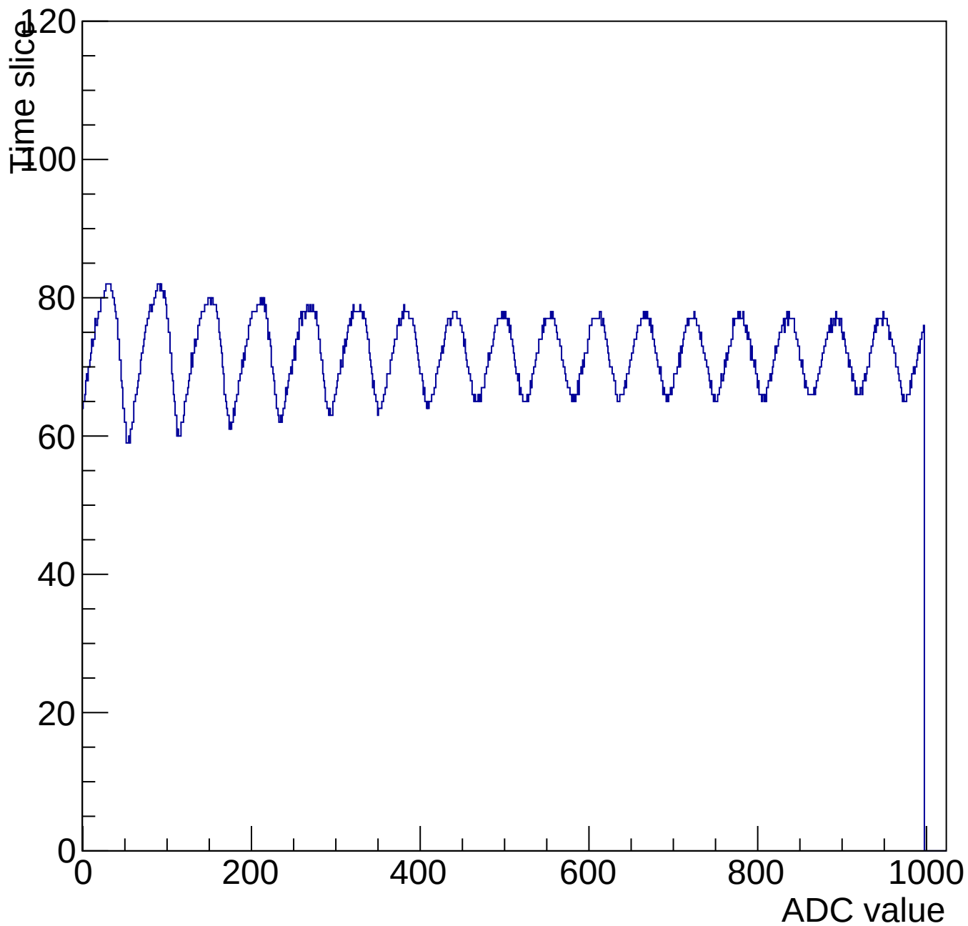
Evt 10 Time mcm 3001 chip 1 chan 11 1000-shift-gain0-shaper7
