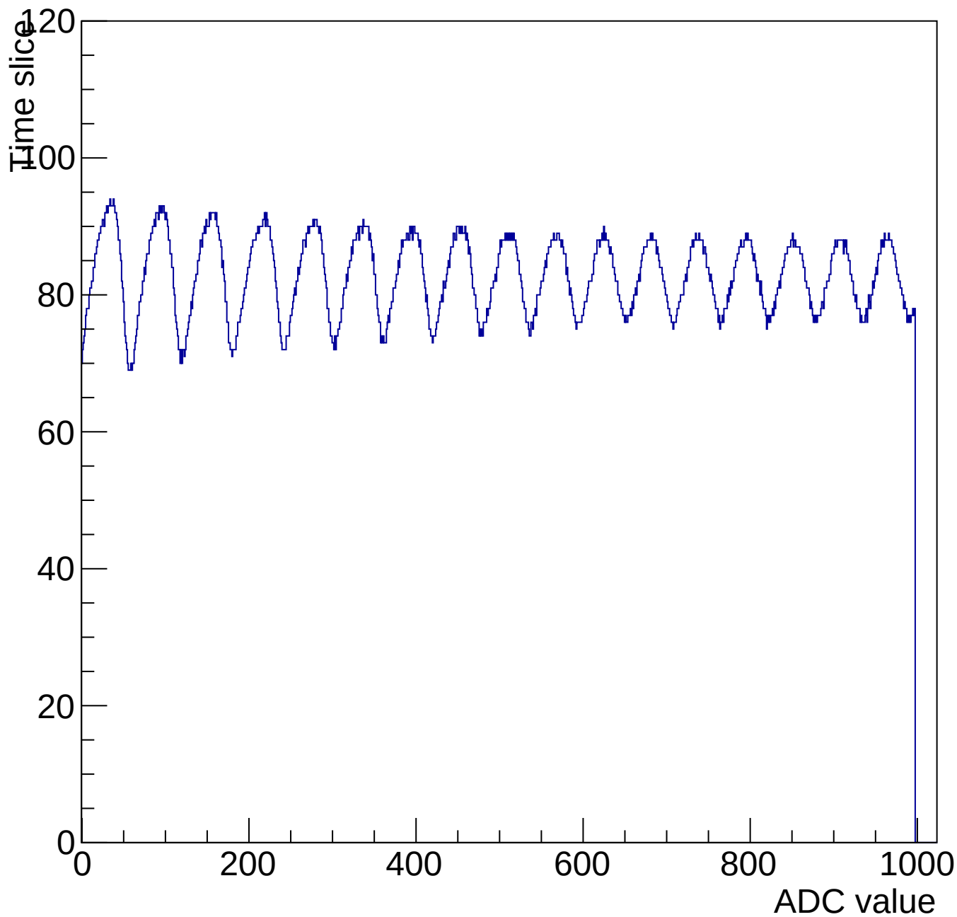
Evt 11 Time mcm 3001 chip 1 chan 1 1000-shift-gain0-shaper7
