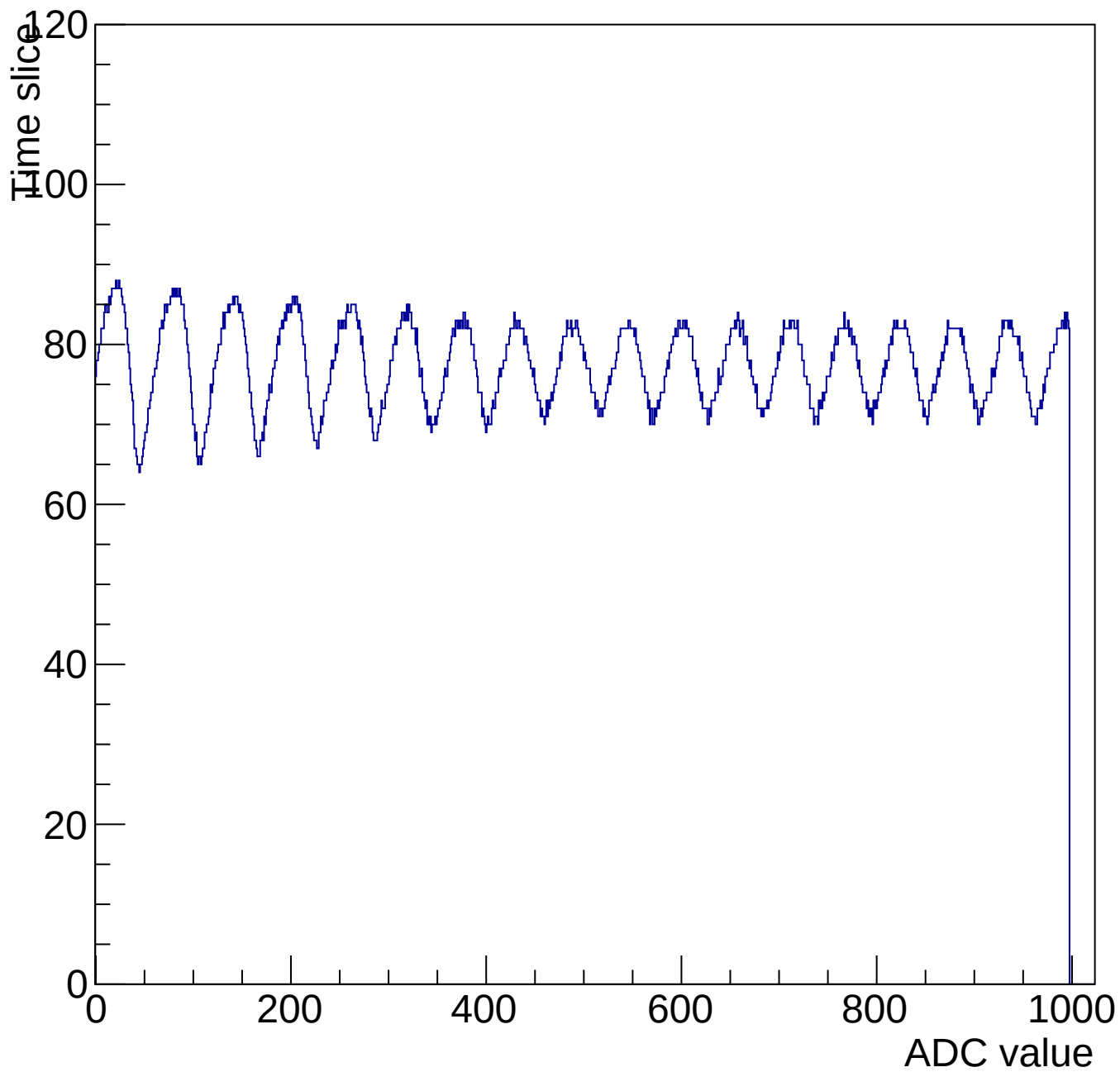
Evt 11 Time mcm 3001 chip 1 chan 15 1000-shift-gain0-shaper7
