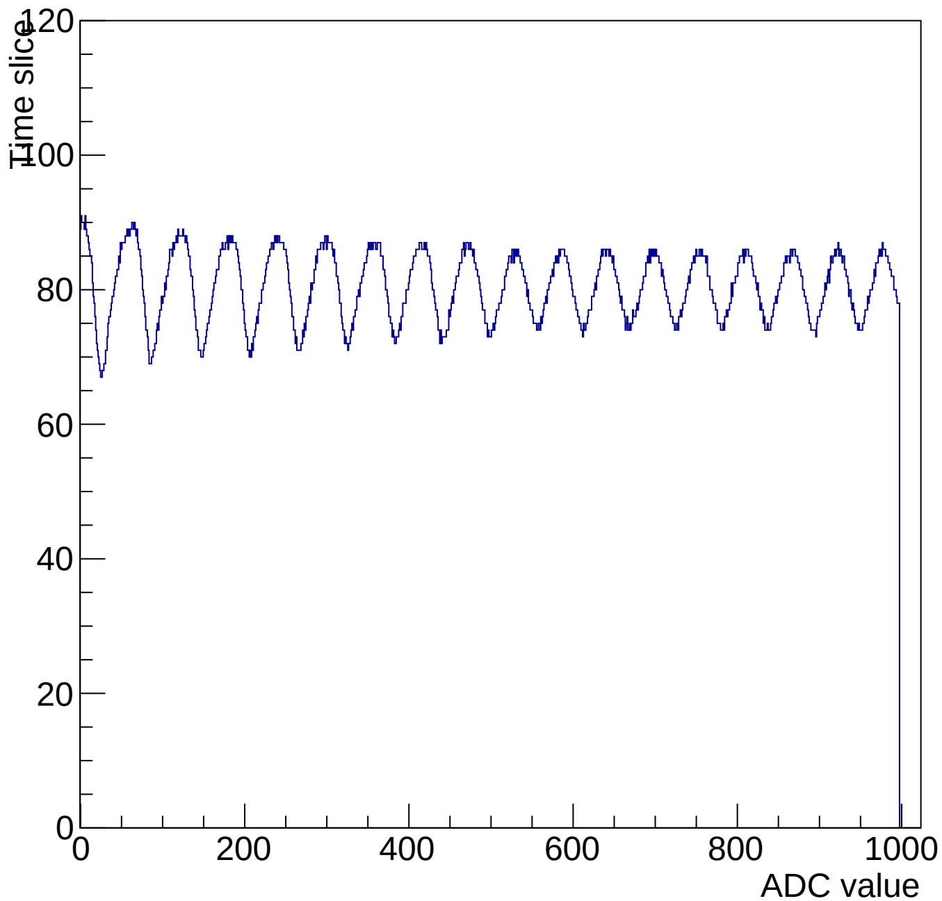
Evt 11 Time mcm 3001 chip 1 chan 12 1000-shift-gain0-shaper7
