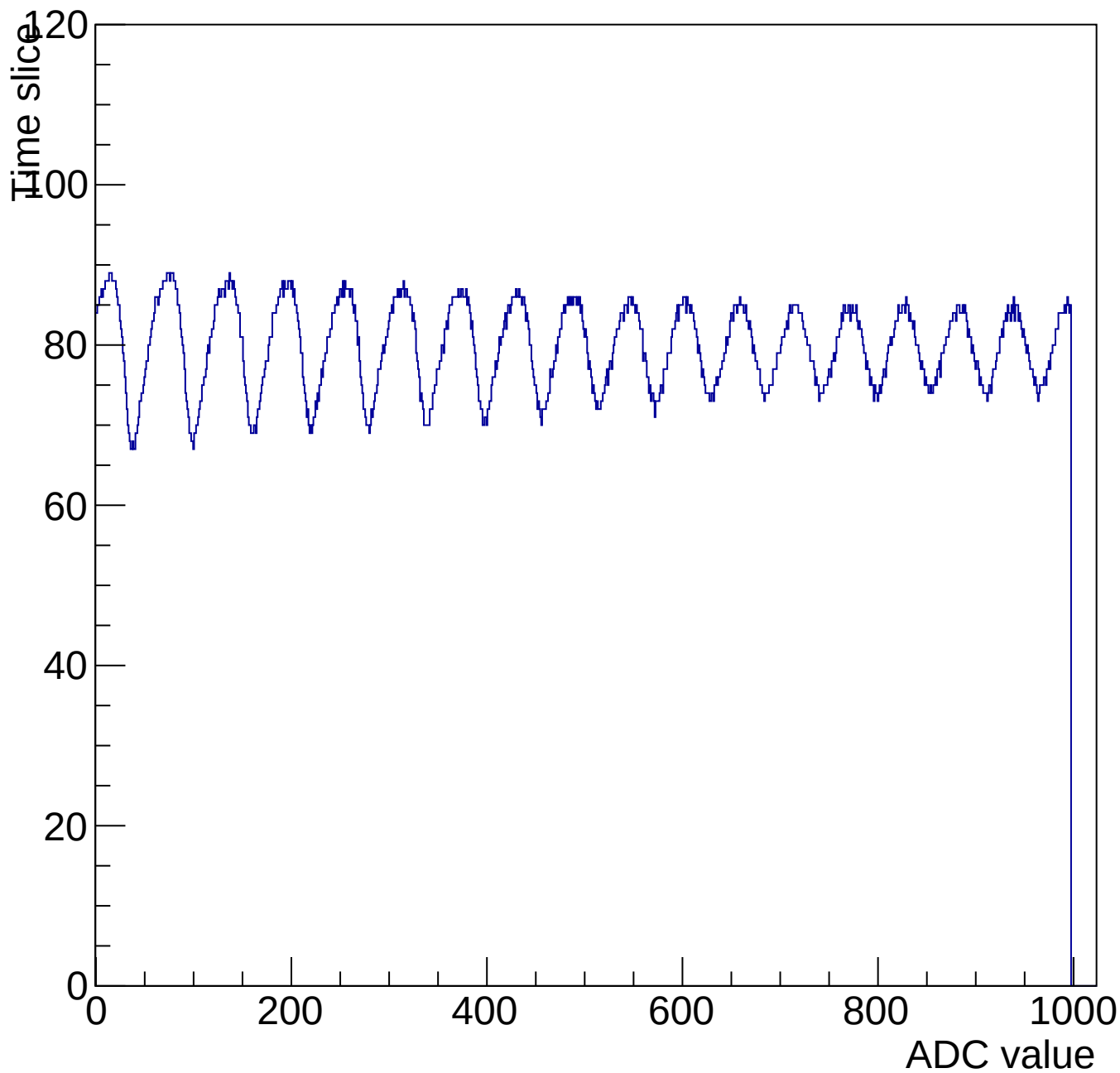
Evt 11 Time mcm 3001 chip 1 chan 8 1000-shift-gain0-shaper7
