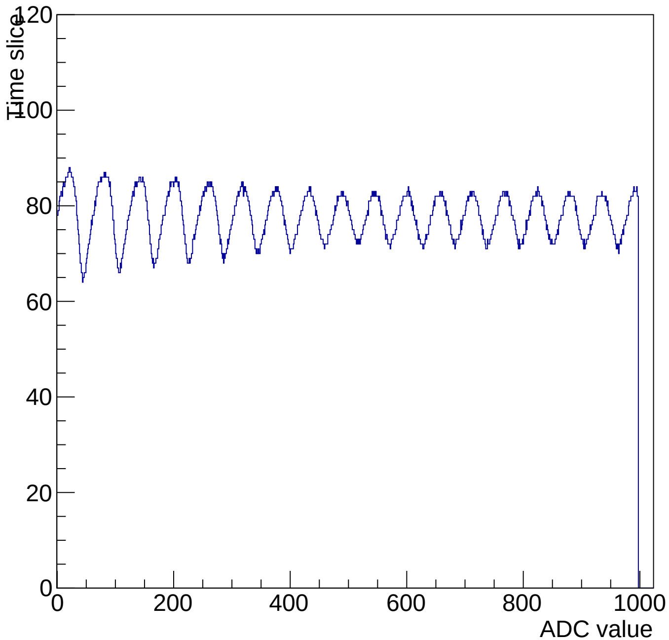
Evt 11 Time mcm 3001 chip 1 chan 14 1000-shift-gain0-shaper7
