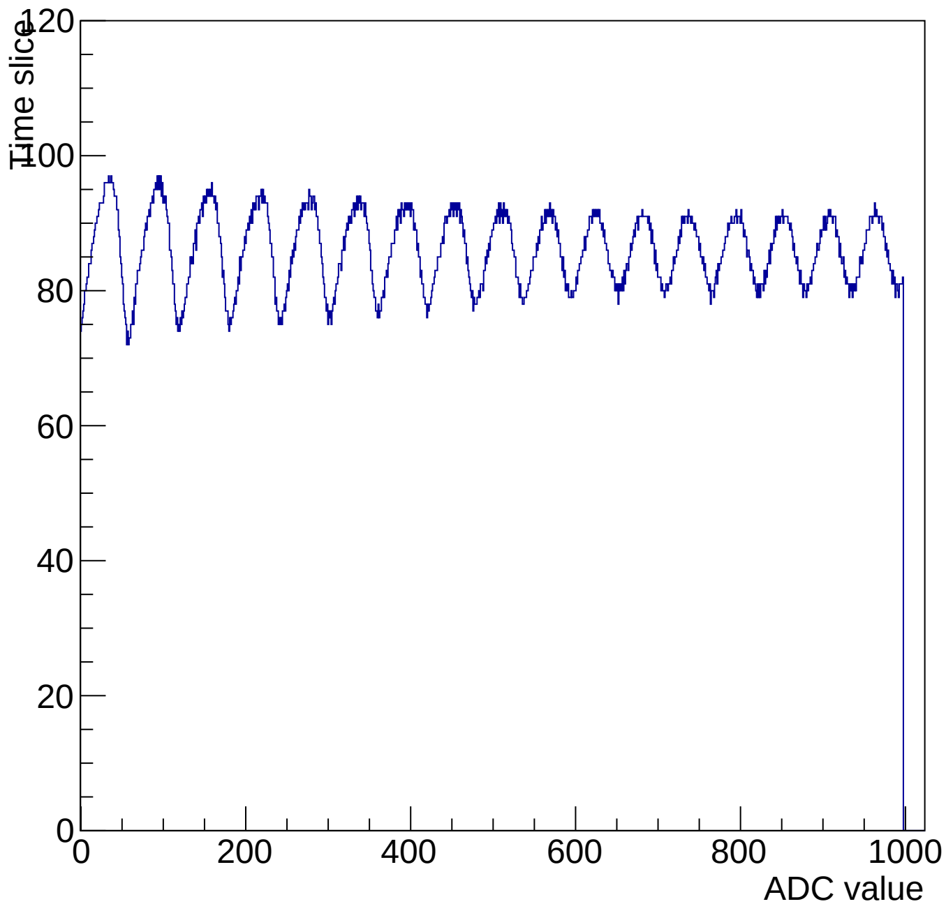
Evt 11 Time mcm 3001 chip 1 chan 0 1000-shift-gain0-shaper7
