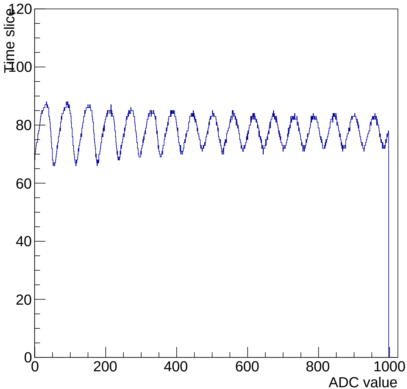
Evt 11 Time mcm 3001 chip 1 chan 4 1000-shift-gain0-shaper7
