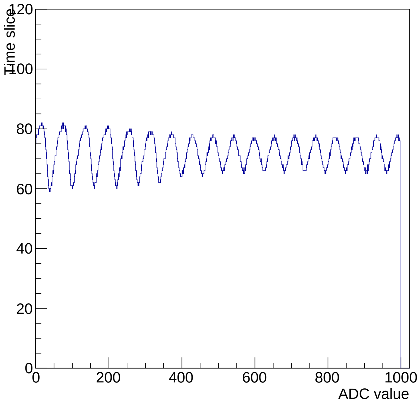
Evt 11 Time mcm 3001 chip 1 chan 11 1000-shift-gain0-shaper7
