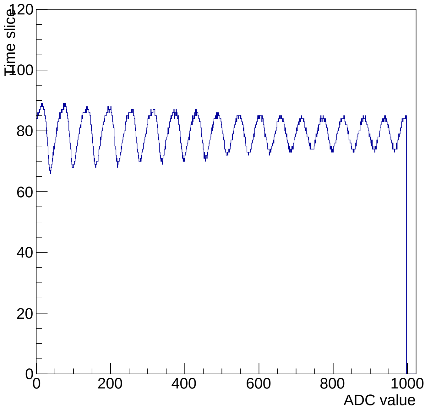
Evt 11 Time mcm 3001 chip 1 chan 9 1000-shift-gain0-shaper7
