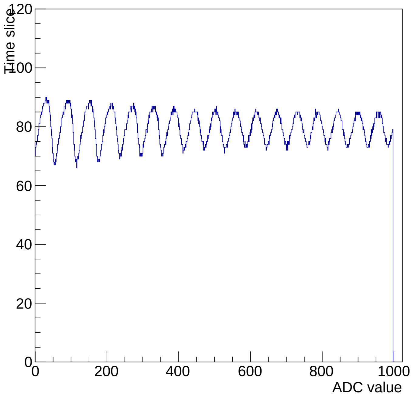
Evt 11 Time mcm 3001 chip 1 chan 5 1000-shift-gain0-shaper7
