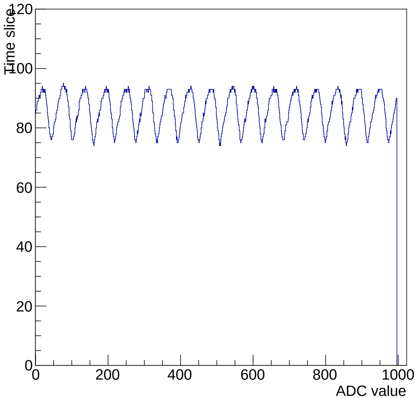
Evt 10 Time mcm 3002 chip 2 chan 2 1000-shift-gain0-shaper0
