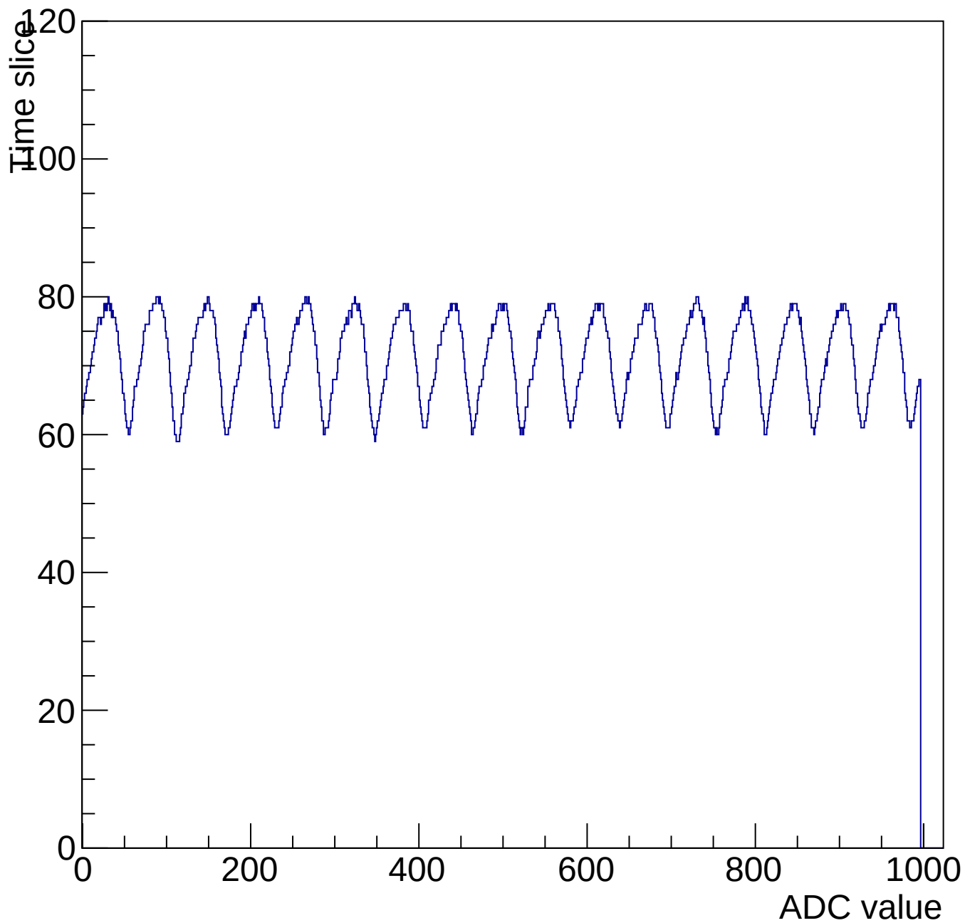
Evt 10 Time mcm 3002 chip 2 chan 5 1000-shift-gain0-shaper0
