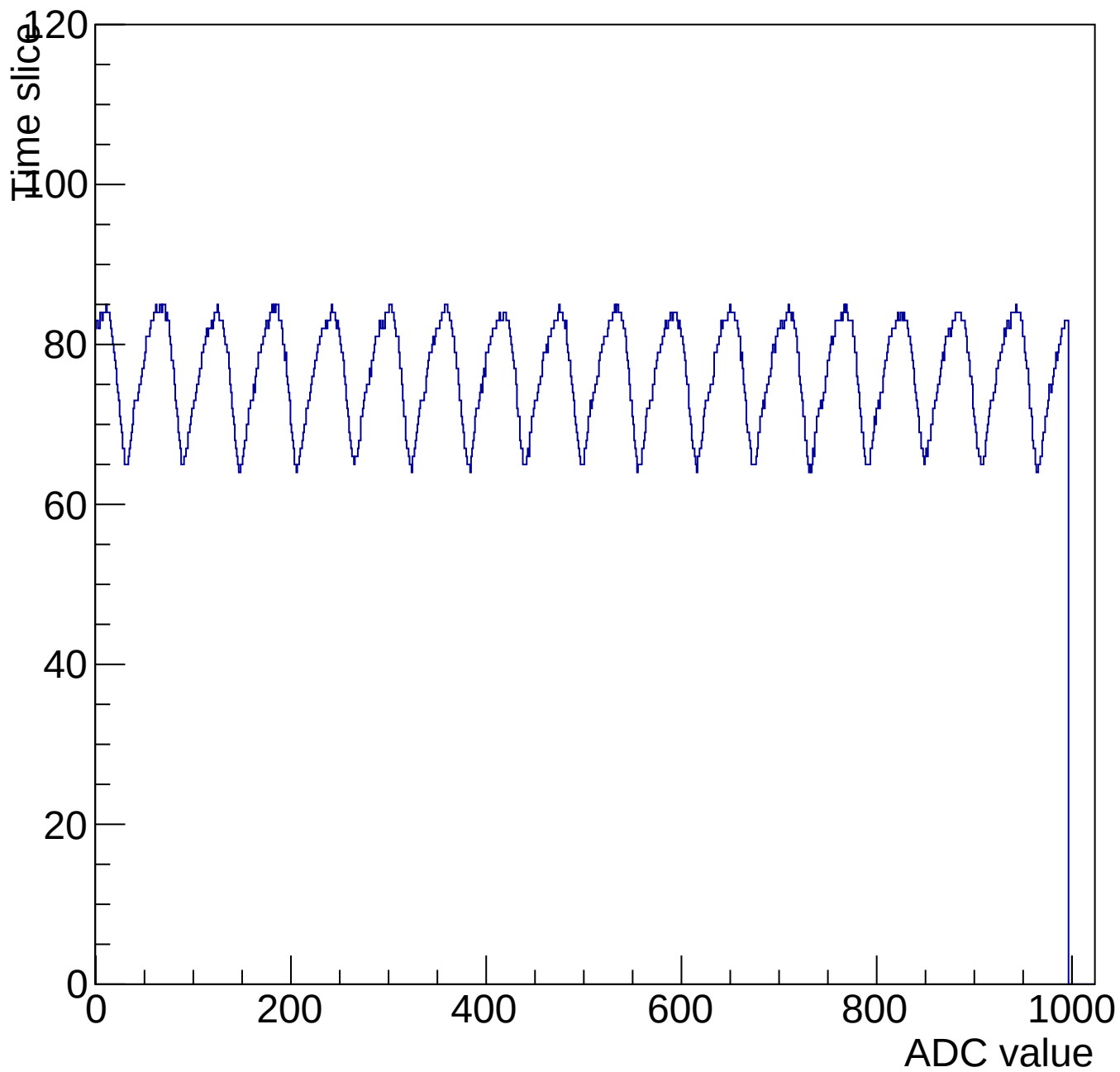
Evt 10 Time mcm 3002 chip 2 chan 10 1000-shift-gain0-shaper0
