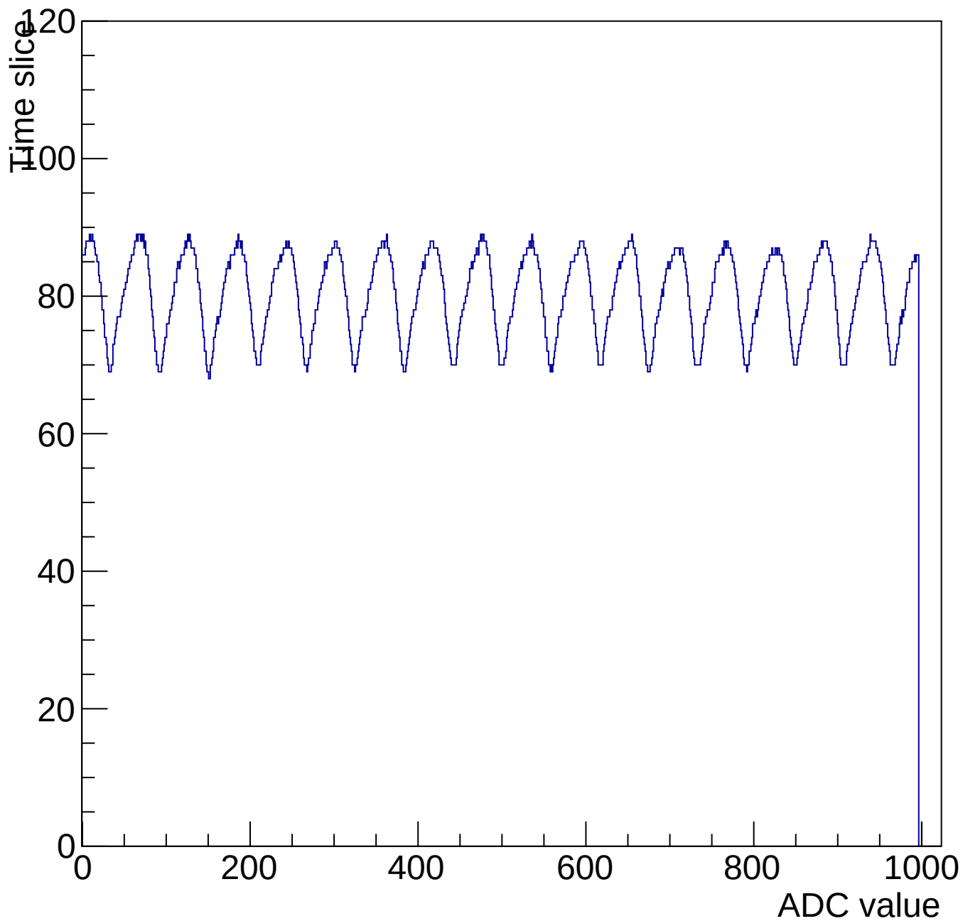
Evt 10 Time mcm 3002 chip 2 chan 7 1000-shift-gain0-shaper0
