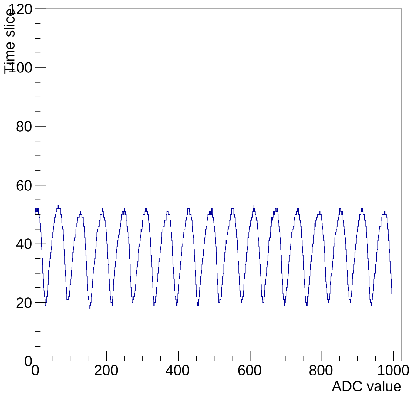
Evt 10 Time mcm 3002 chip 2 chan 7 1000-shift-gain3-shaper0
