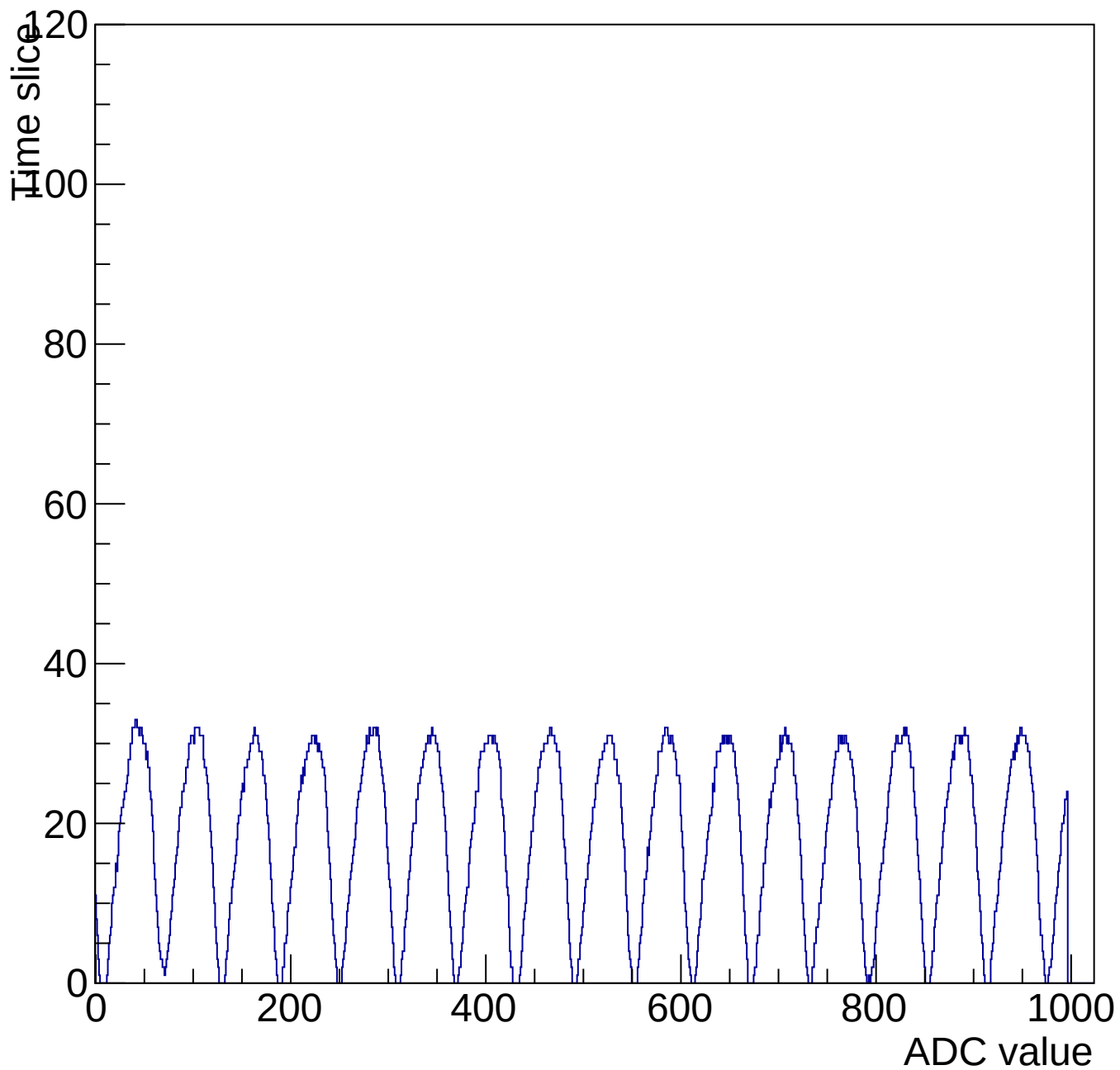
Evt 10 Time mcm 3002 chip 2 chan 8 1000-shift-gain3-shaper0
