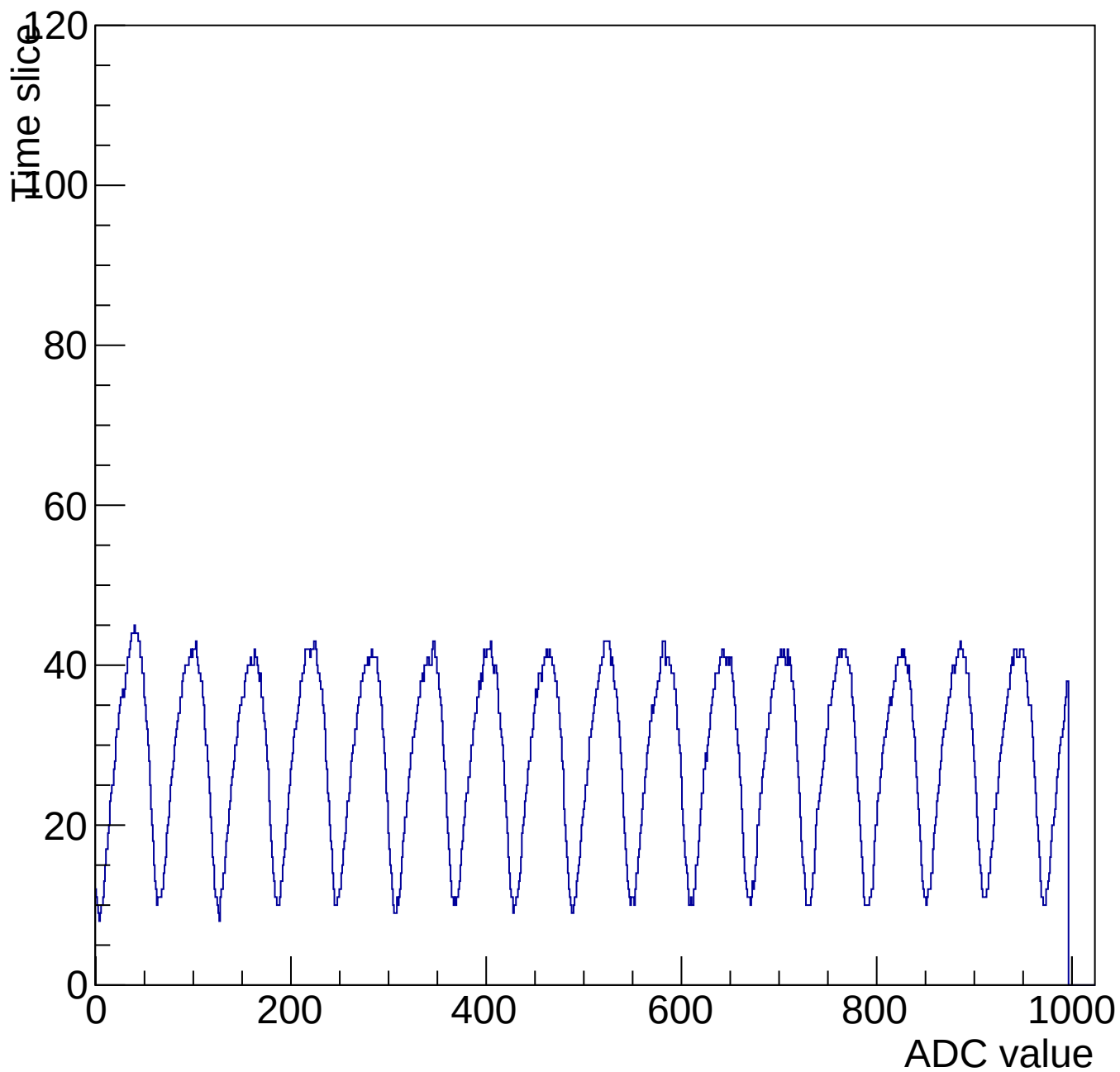
Evt 10 Time mcm 3002 chip 2 chan 12 1000-shift-gain3-shaper0
