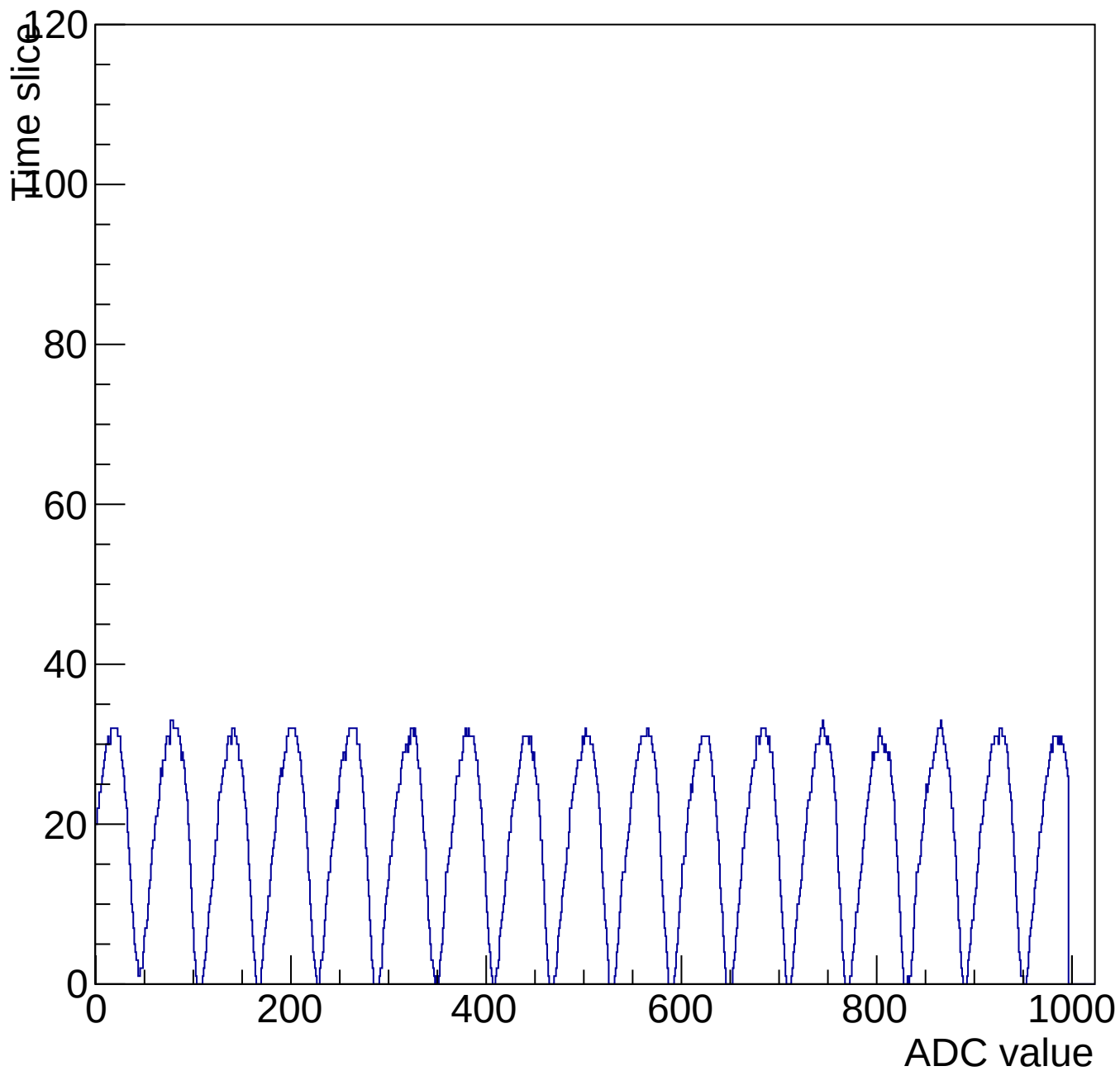
Evt 10 Time mcm 3002 chip 2 chan 5 1000-shift-gain3-shaper0
