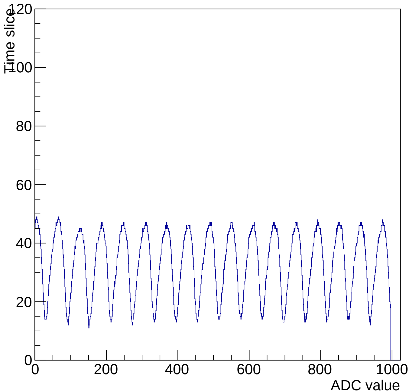
Evt 10 Time mcm 3002 chip 2 chan 6 1000-shift-gain3-shaper0
