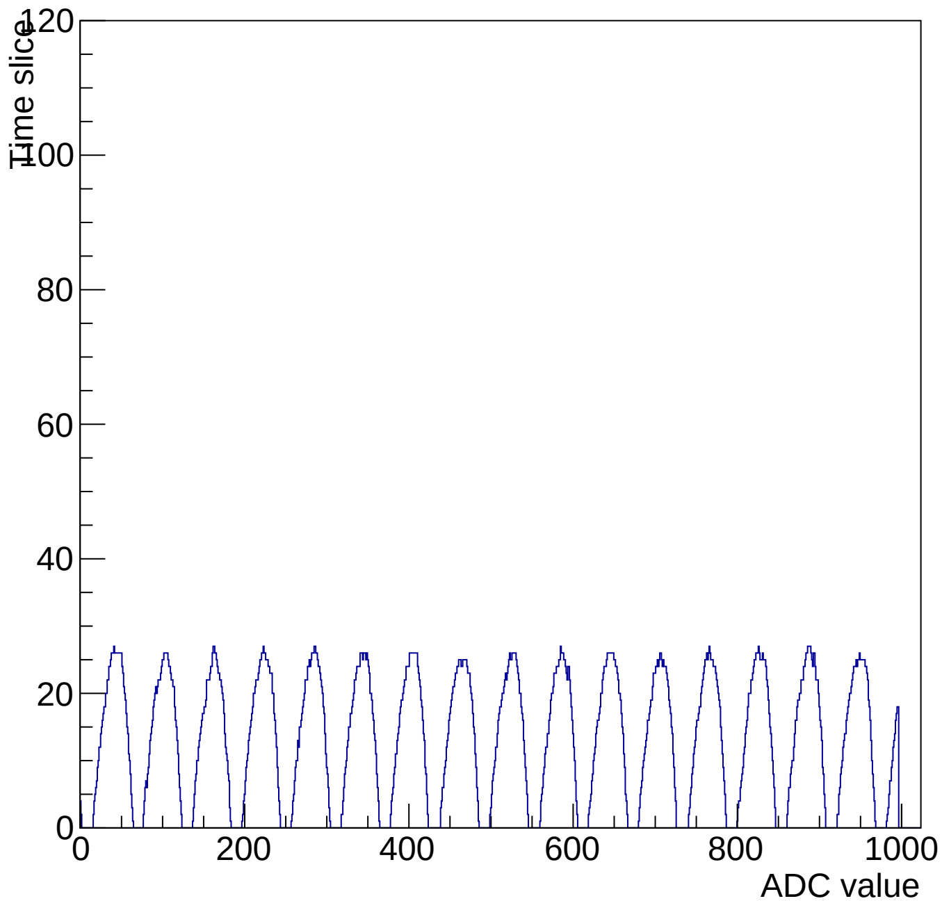
Evt 10 Time mcm 3002 chip 2 chan 9 1000-shift-gain3-shaper0
