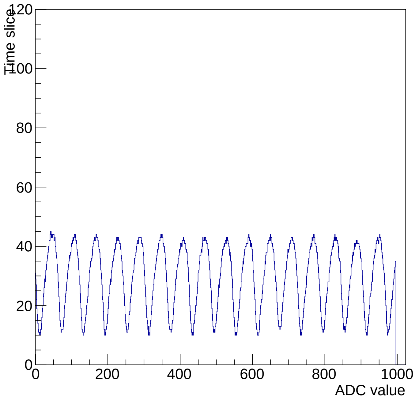
Evt 10 Time mcm 3002 chip 2 chan 11 1000-shift-gain3-shaper0
