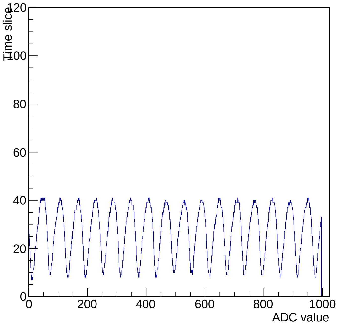
Evt 10 Time mcm 3002 chip 2 chan 10 1000-shift-gain3-shaper0
