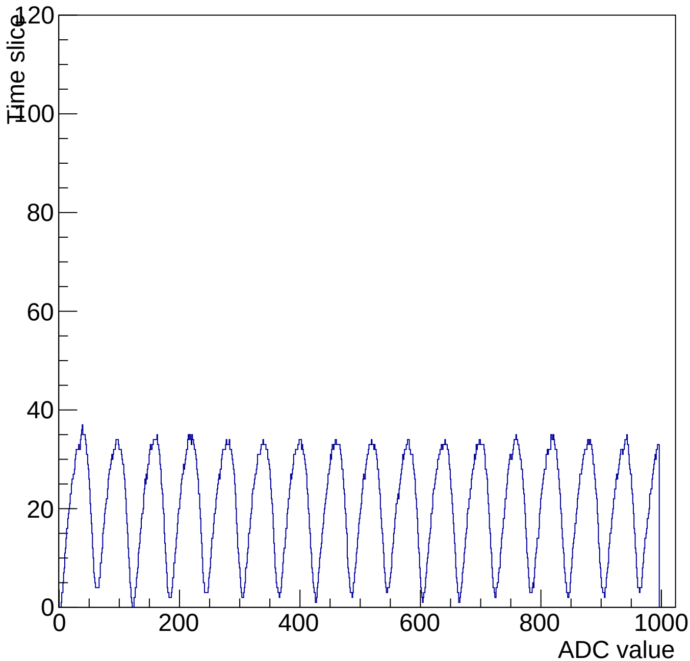
Evt 10 Time mcm 3002 chip 2 chan 14 1000-shift-gain3-shaper0
