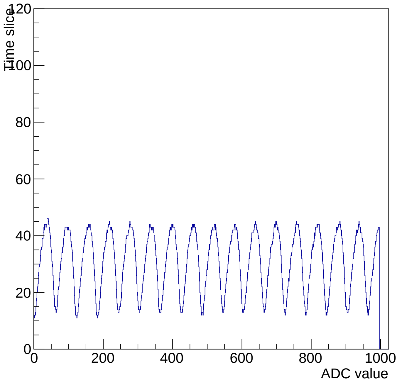
Evt 10 Time mcm 3002 chip 2 chan 15 1000-shift-gain3-shaper0
