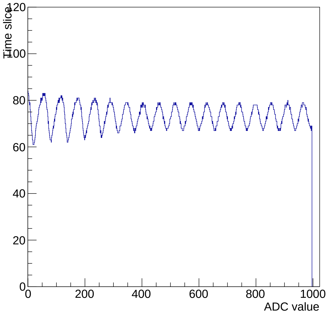
Evt 10 Time mcm 3002 chip 2 chan 13 1000-shift-gain0-shaper7
