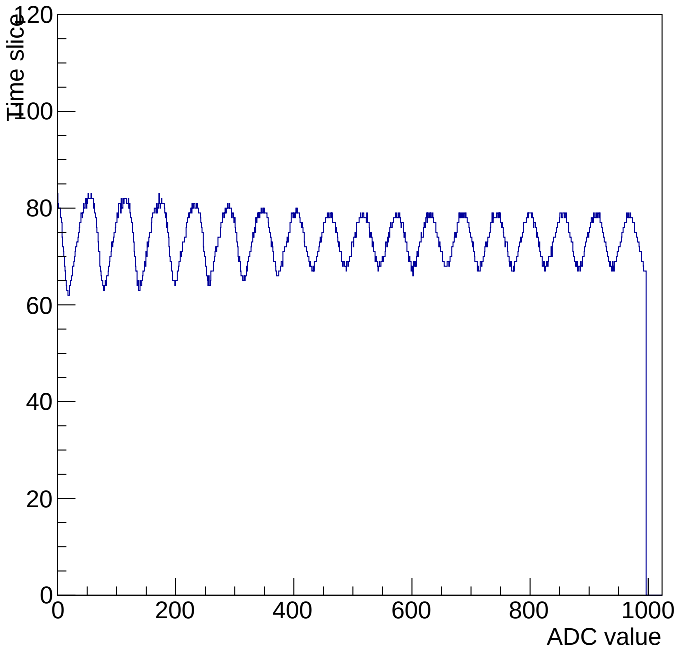
Evt 10 Time mcm 3002 chip 2 chan 1 1000-shift-gain0-shaper7
