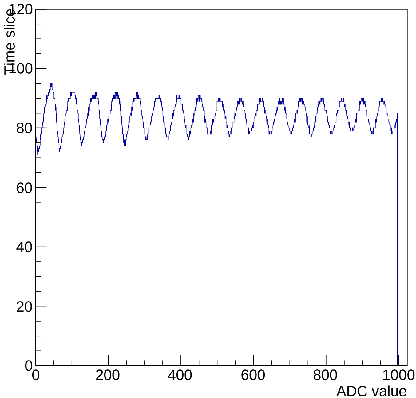
Evt 10 Time mcm 3002 chip 2 chan 2 1000-shift-gain0-shaper7
