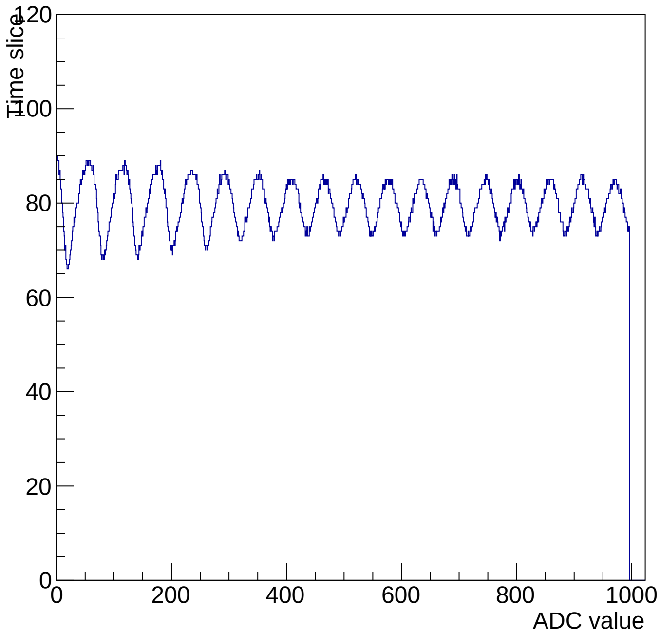
Evt 10 Time mcm 3002 chip 2 chan 11 1000-shift-gain0-shaper7
