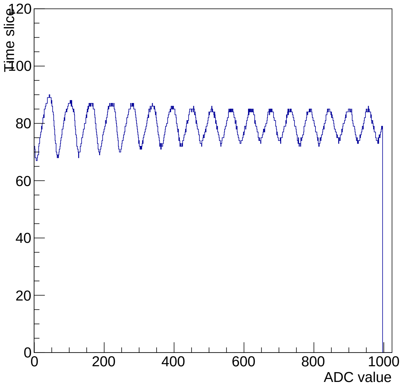
Evt 10 Time mcm 3002 chip 2 chan 3 1000-shift-gain0-shaper7
