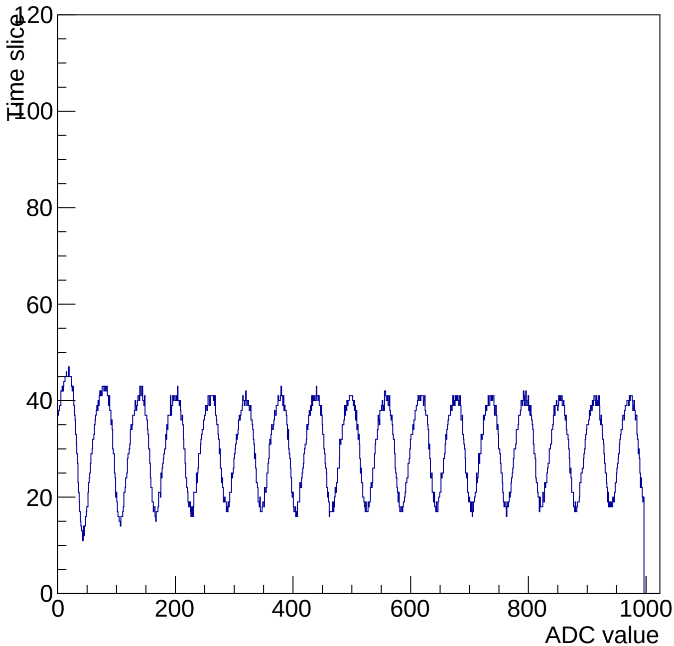
Evt 10 Time mcm 3002 chip 2 chan 1 1000-shift-gain3-shaper7
