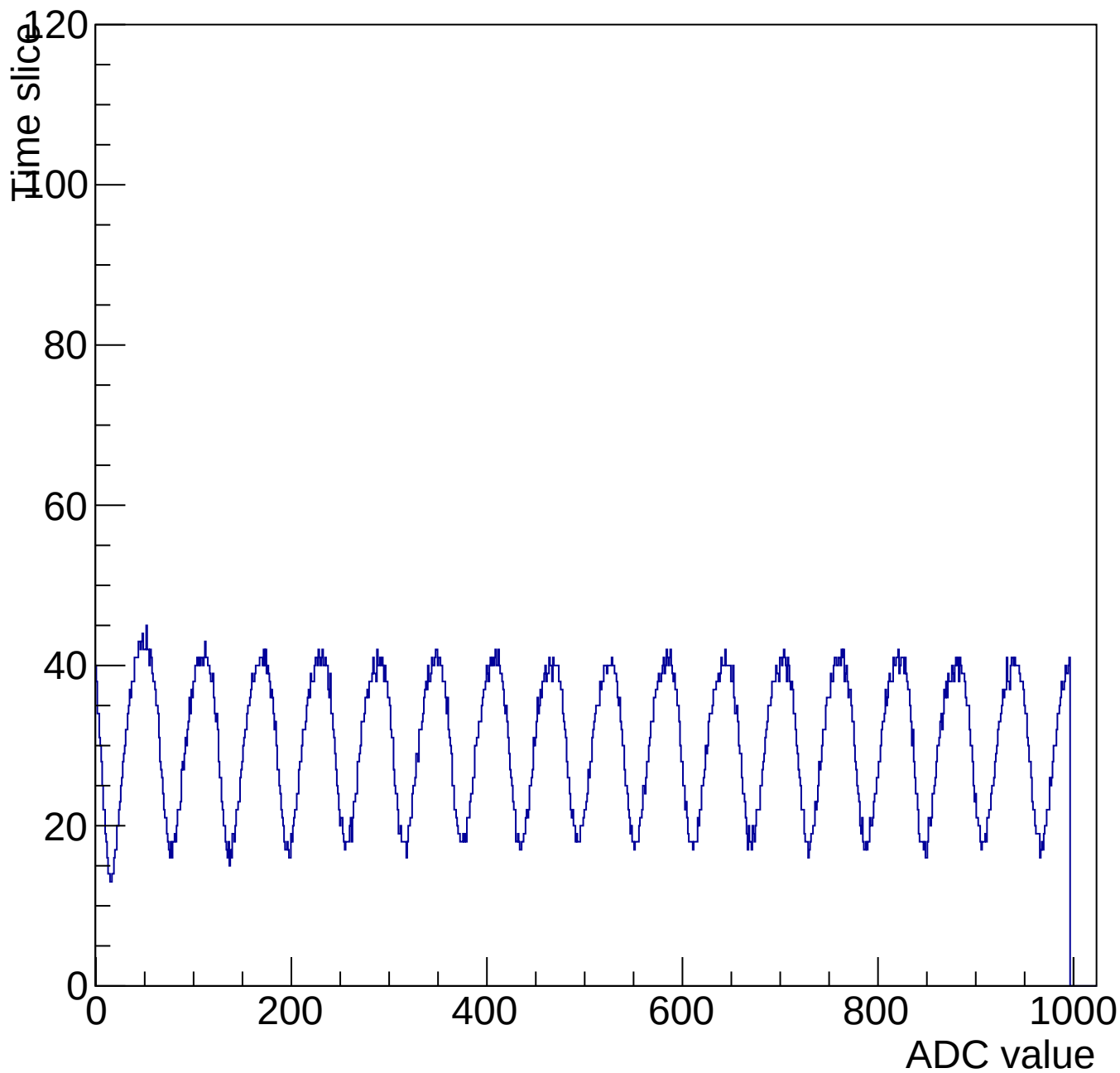
Evt 10 Time mcm 3002 chip 2 chan 4 1000-shift-gain3-shaper7
