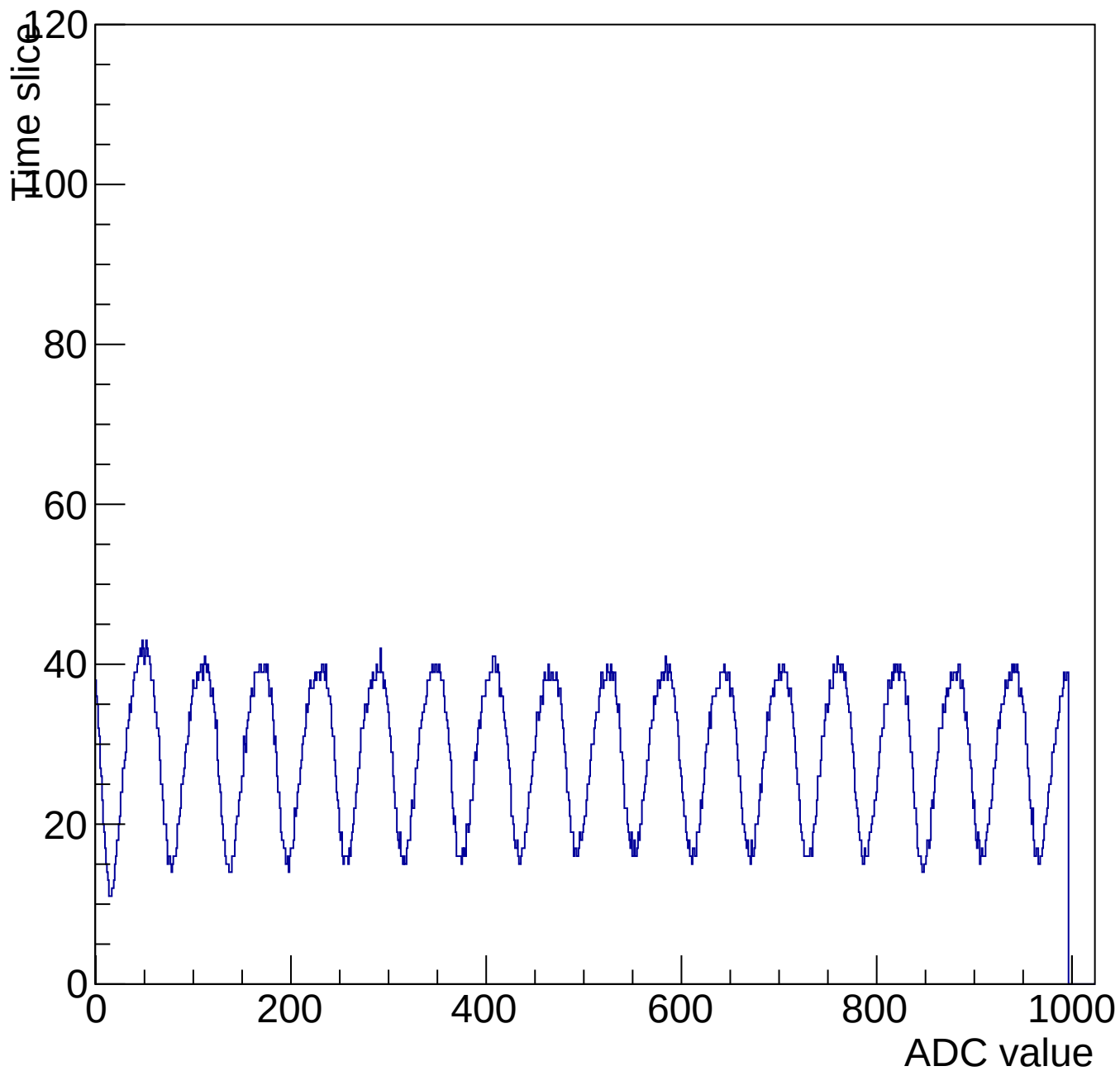
Evt 10 Time mcm 3002 chip 2 chan 5 1000-shift-gain3-shaper7
