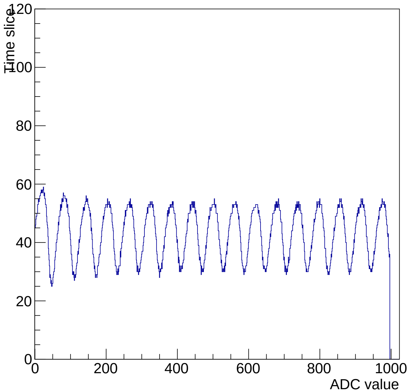
Evt 10 Time mcm 3002 chip 2 chan 2 1000-shift-gain3-shaper7
