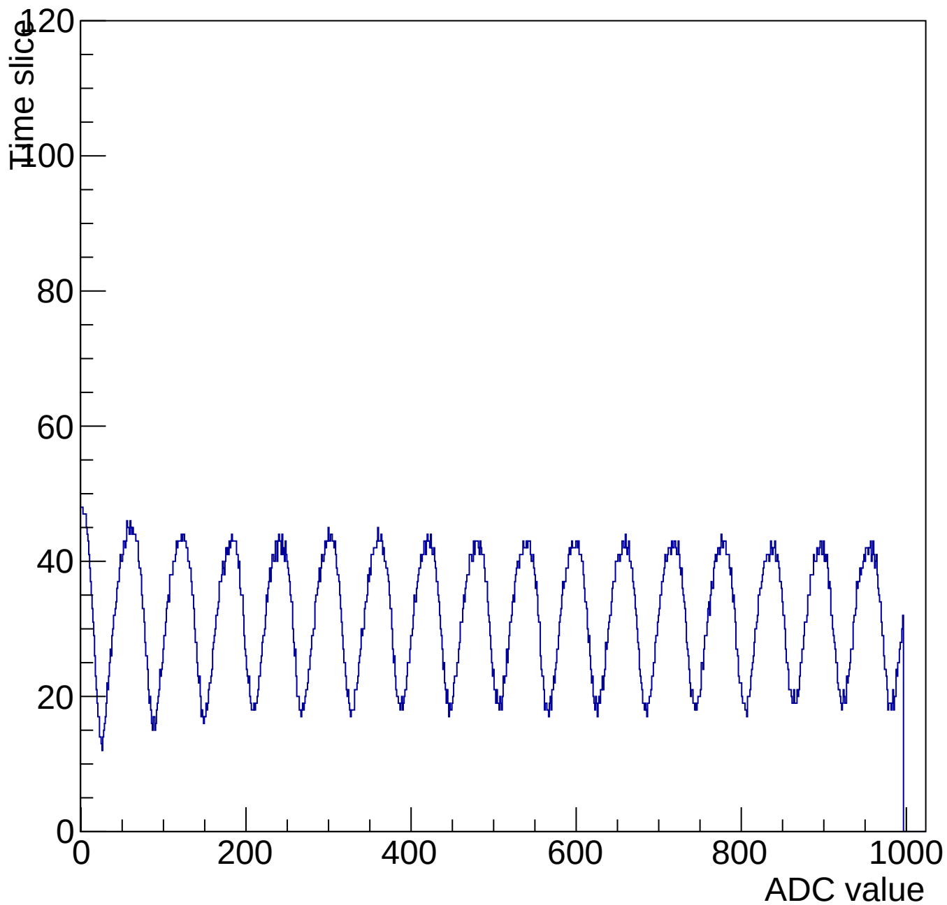
Evt 10 Time mcm 3002 chip 2 chan 10 1000-shift-gain3-shaper7
