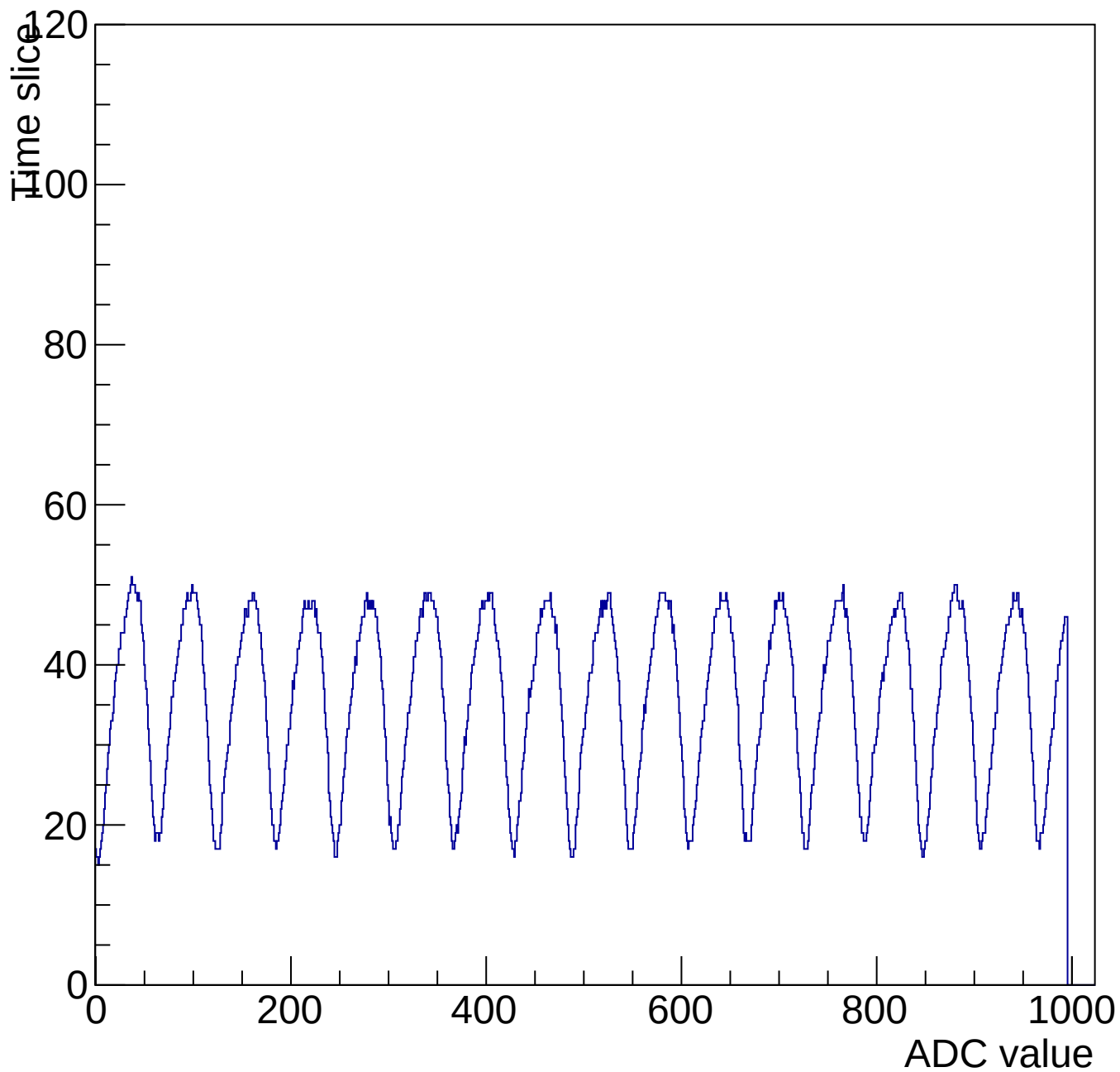
Evt 10 Time mcm 3003 chip 3 chan 10 1000-shift-gain3-shaper0
