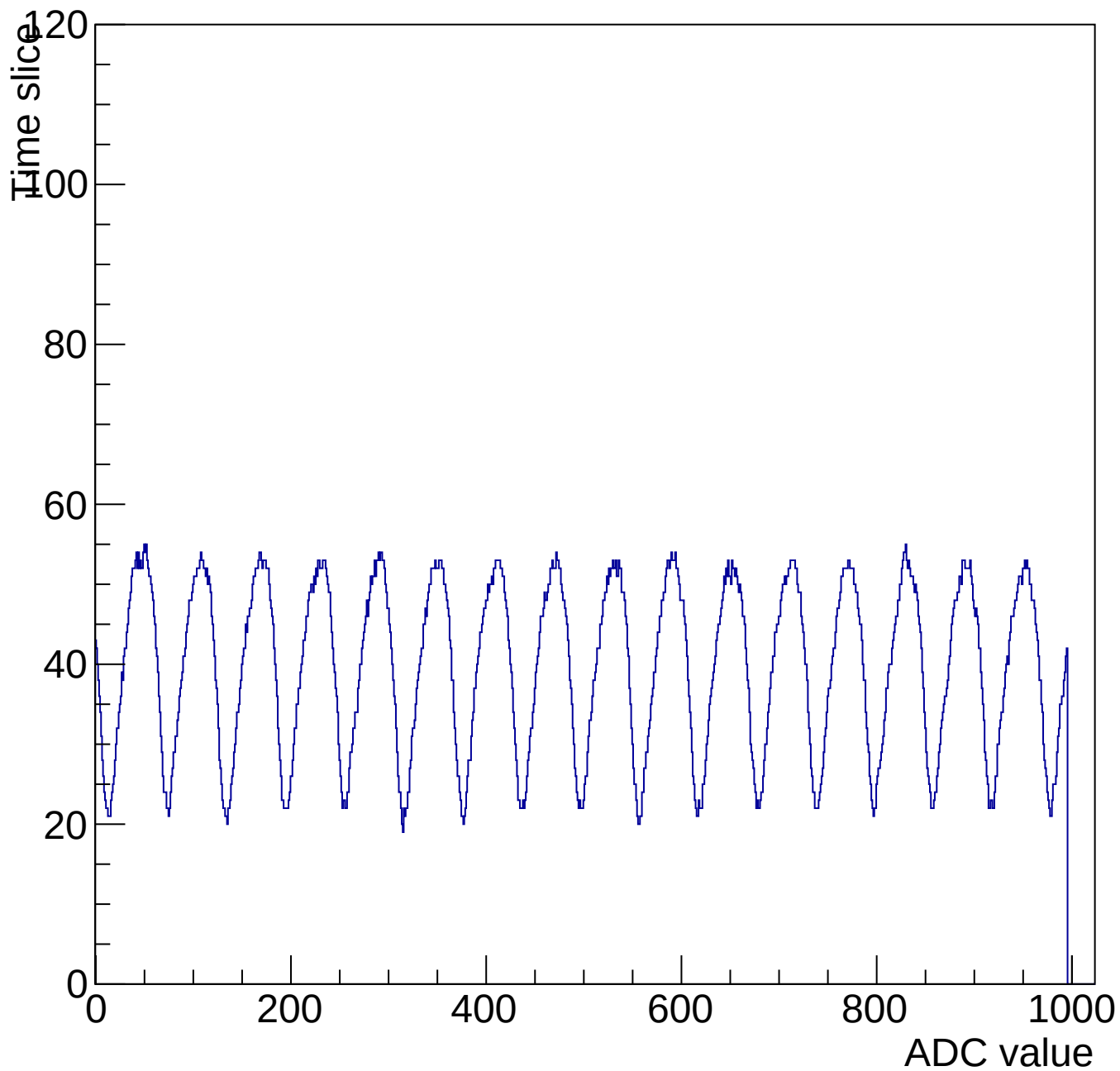
Evt 10 Time mcm 3003 chip 3 chan 4 1000-shift-gain3-shaper0
