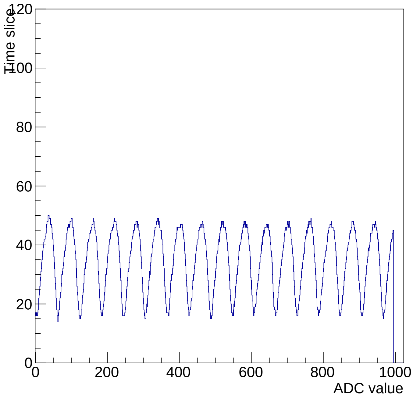
Evt 10 Time mcm 3003 chip 3 chan 11 1000-shift-gain3-shaper0
