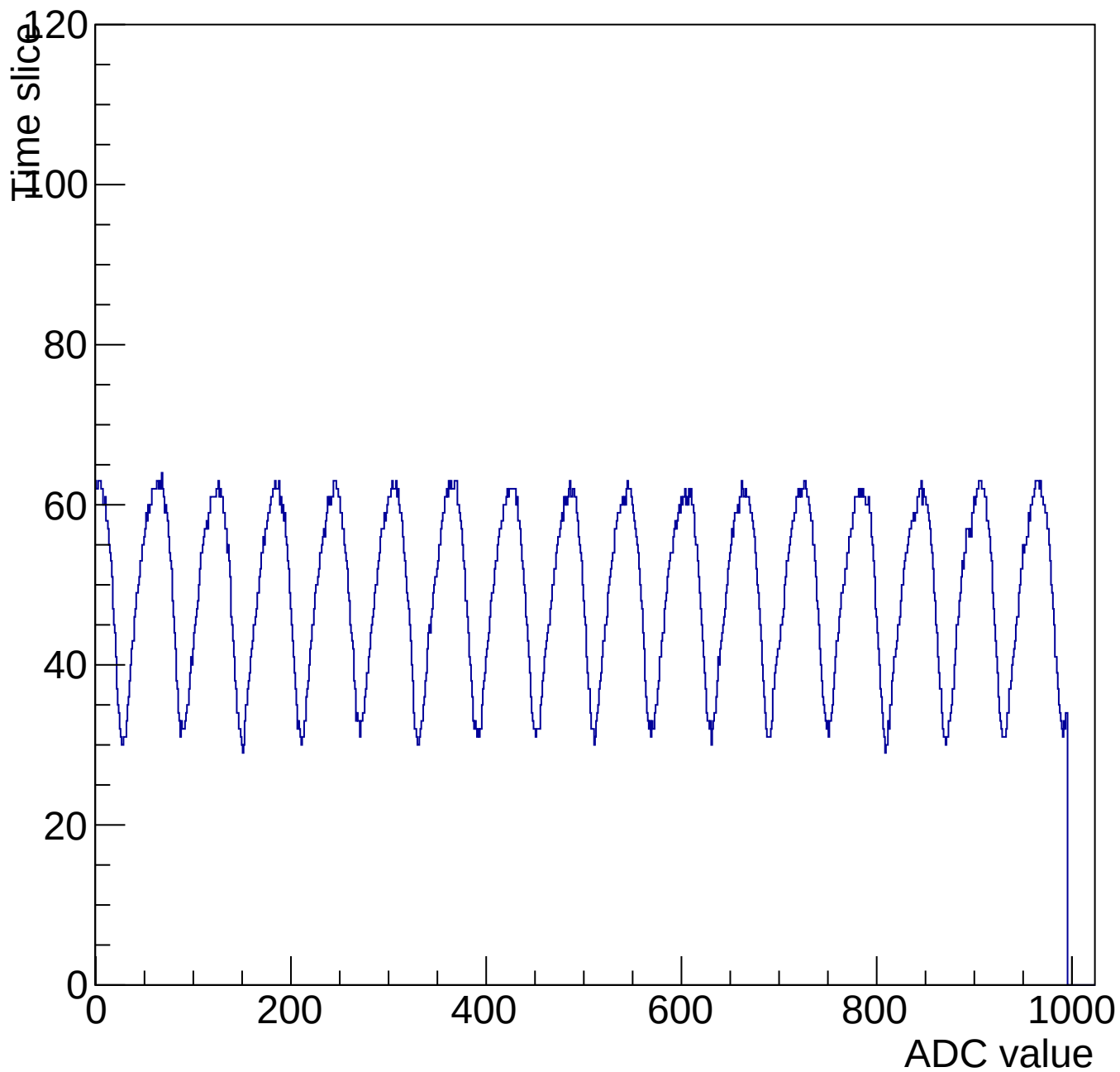
Evt 10 Time mcm 3003 chip 3 chan 12 1000-shift-gain3-shaper0
