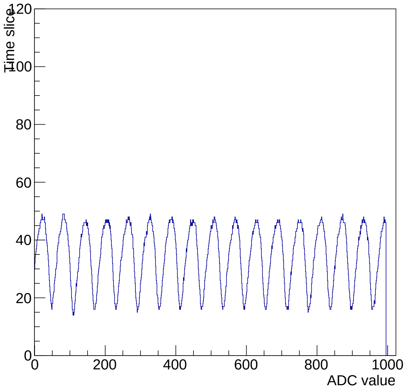
Evt 10 Time mcm 3003 chip 3 chan 3 1000-shift-gain3-shaper0
