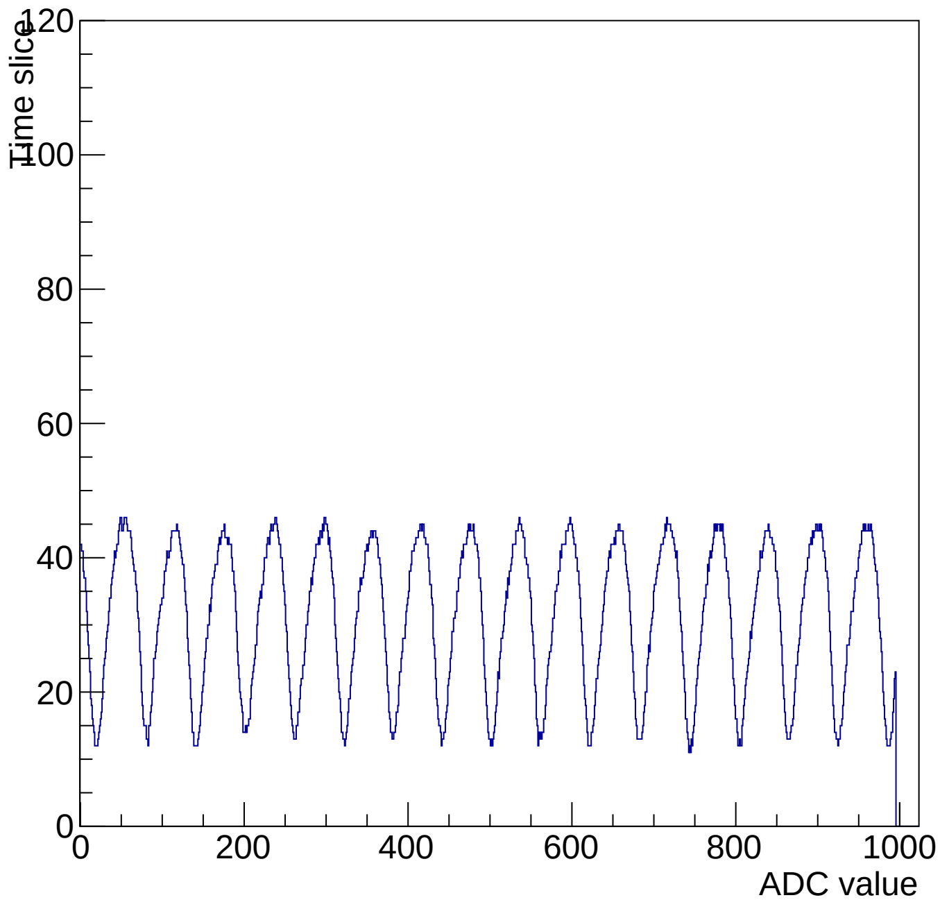
Evt 10 Time mcm 3003 chip 3 chan 8 1000-shift-gain3-shaper0
