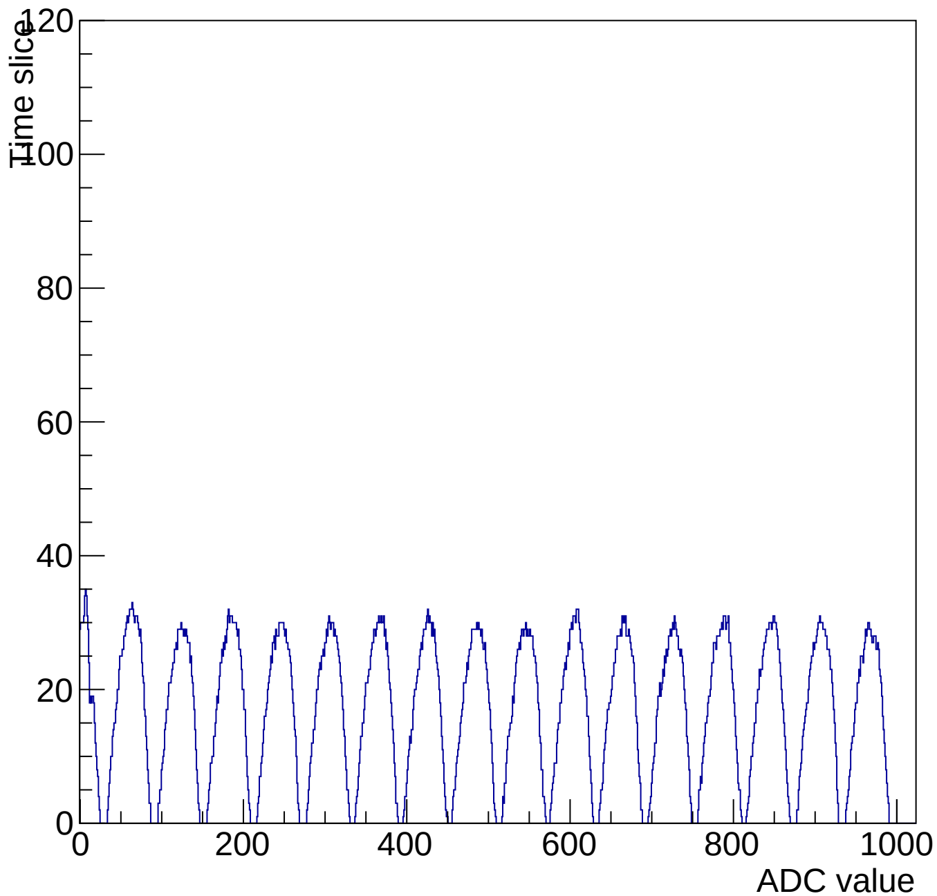
Evt 10 Time mcm 3003 chip 3 chan 0 1000-shift-gain3-shaper0
