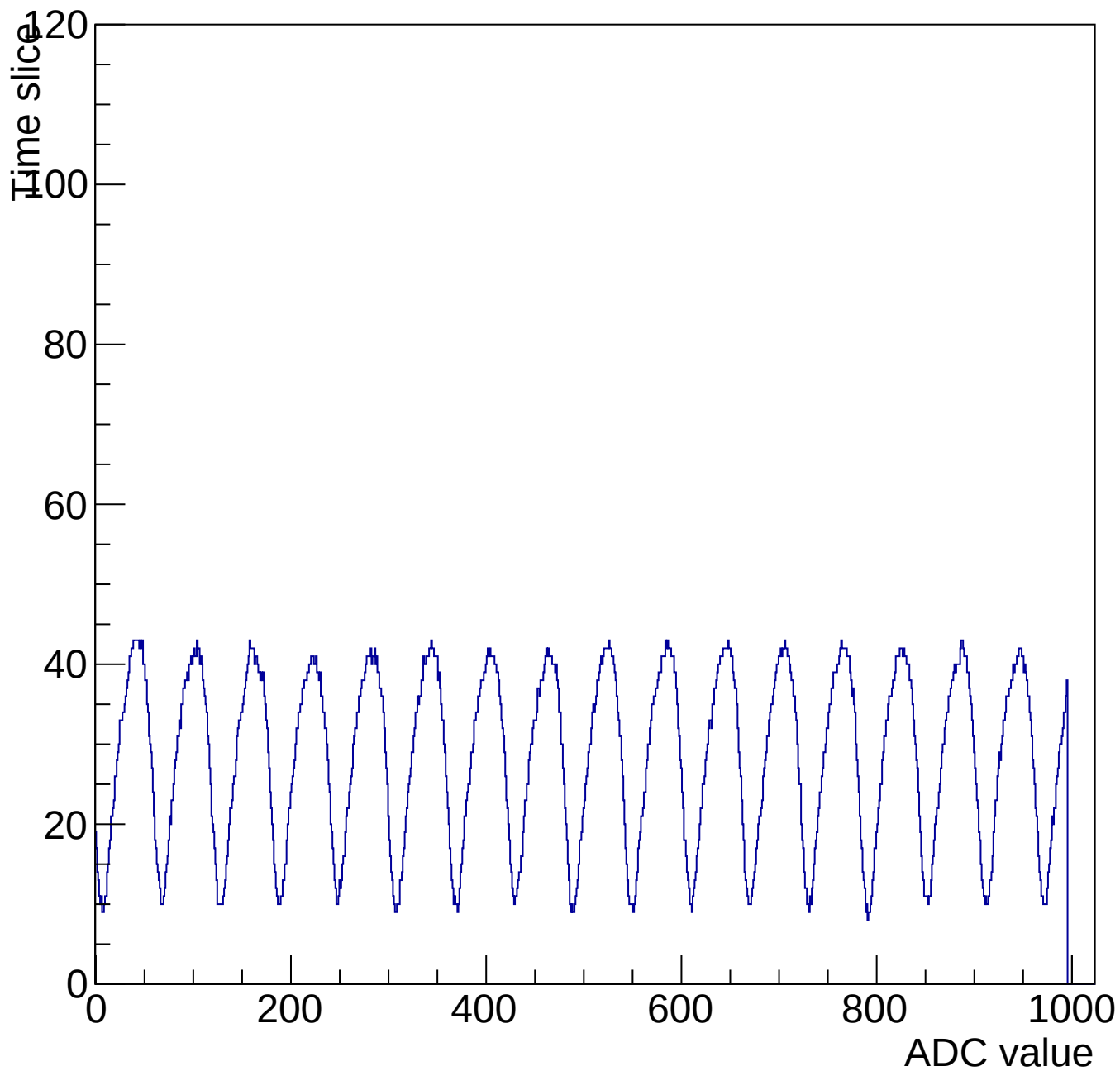
Evt 10 Time mcm 3003 chip 3 chan 6 1000-shift-gain3-shaper0
