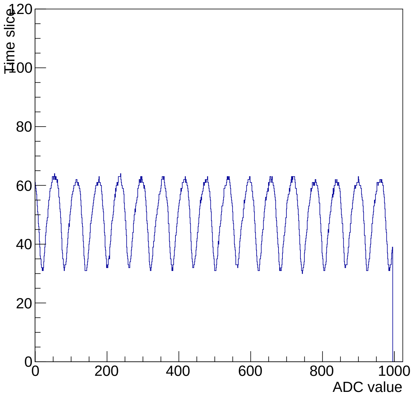
Evt 10 Time mcm 3003 chip 3 chan 9 1000-shift-gain3-shaper0
