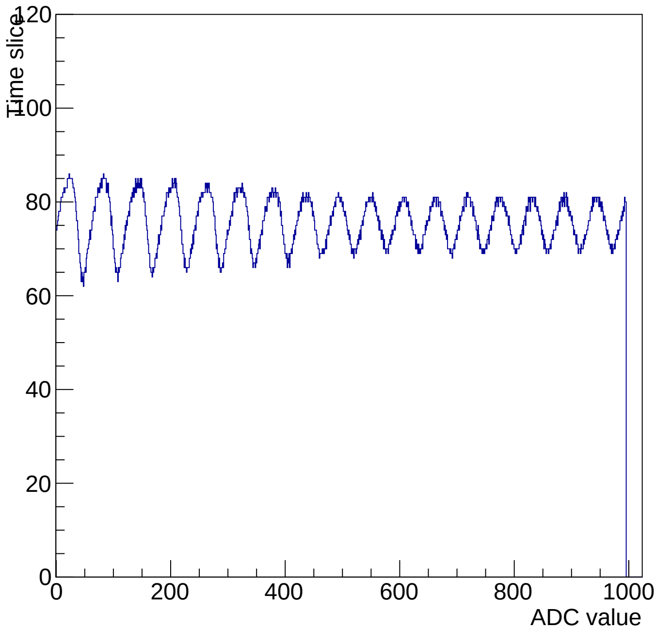
Evt 10 Time mcm 3003 chip 3 chan 7 1000-shift-gain0-shaper7
