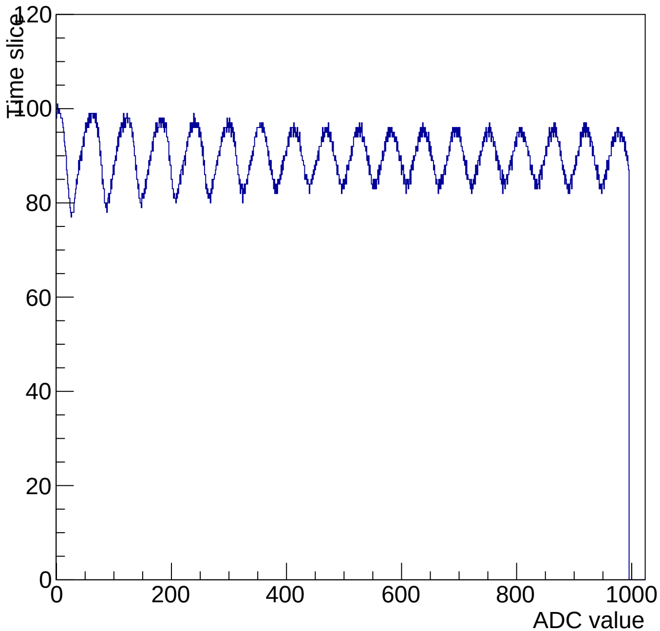
Evt 10 Time mcm 3003 chip 3 chan 4 1000-shift-gain0-shaper7
