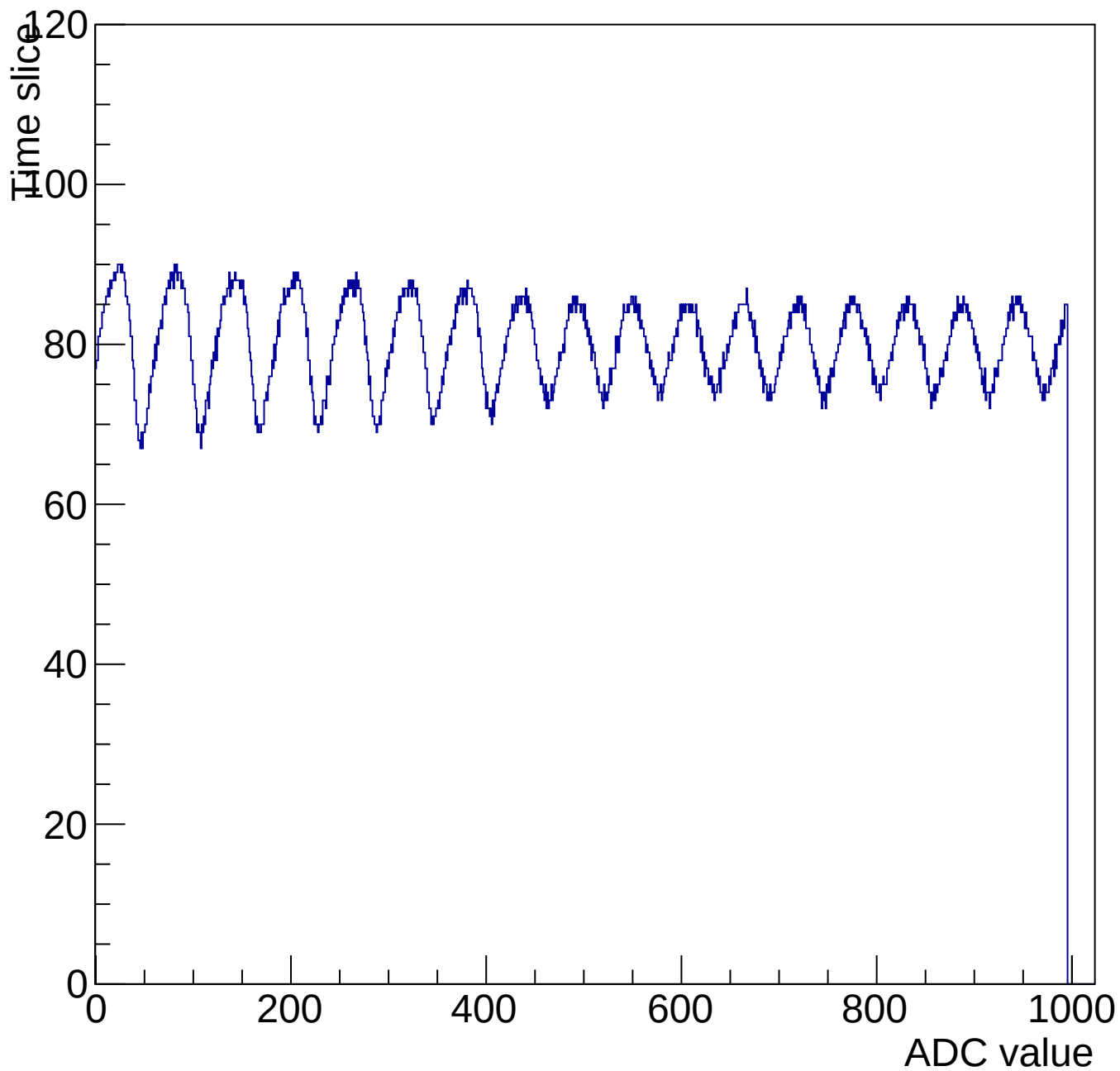
Evt 10 Time mcm 3003 chip 3 chan 6 1000-shift-gain0-shaper7
