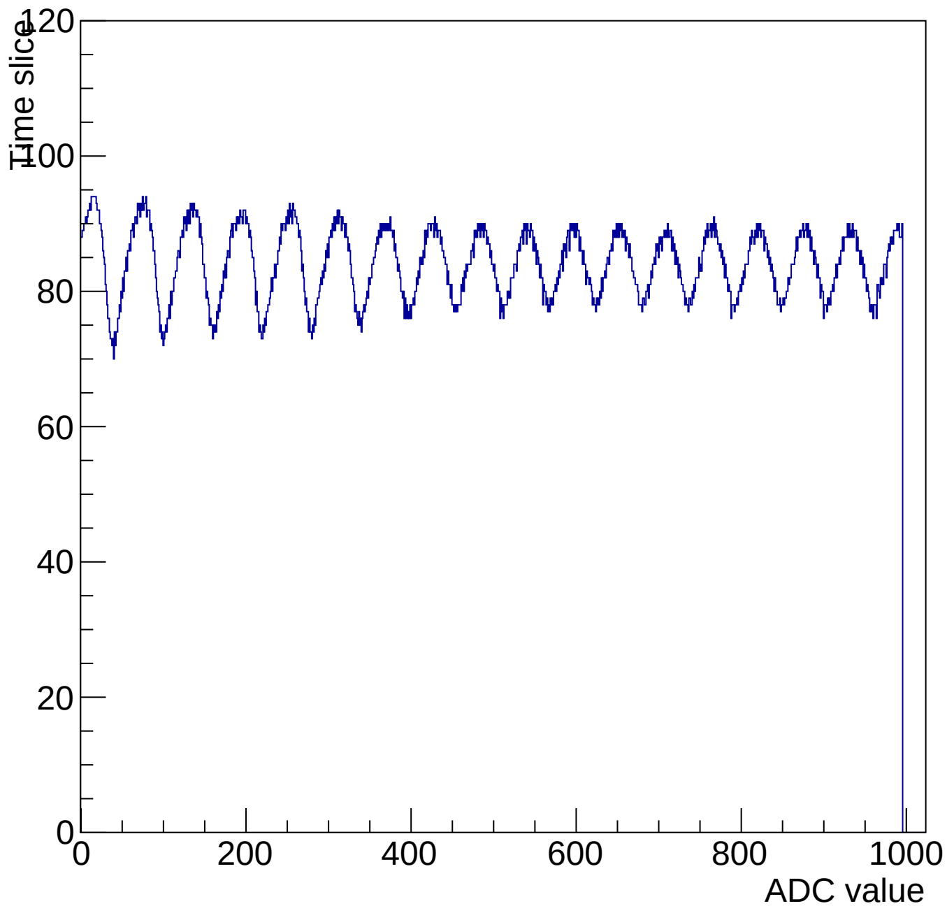
Evt 10 Time mcm 3003 chip 3 chan 8 1000-shift-gain0-shaper7
