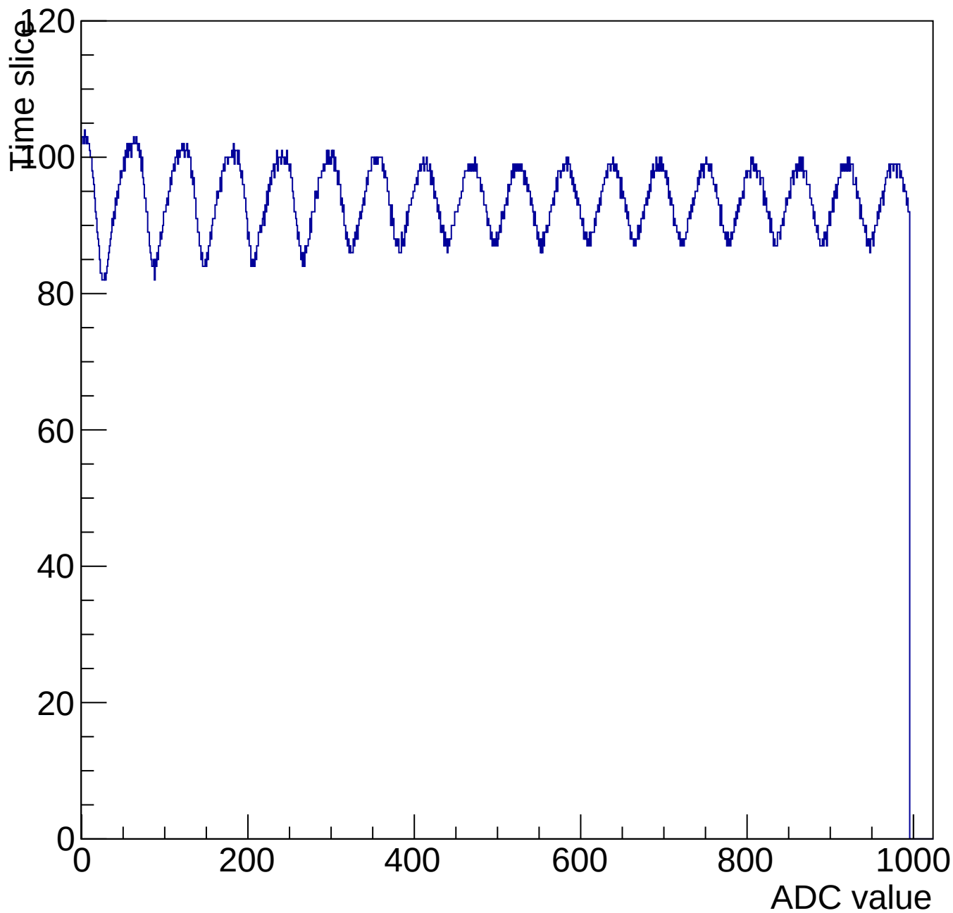
Evt 10 Time mcm 3003 chip 3 chan 5 1000-shift-gain0-shaper7
