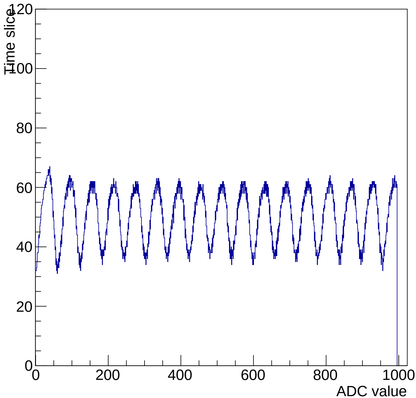
Evt 10 Time mcm 3003 chip 3 chan 4 1000-shift-gain3-shaper7
