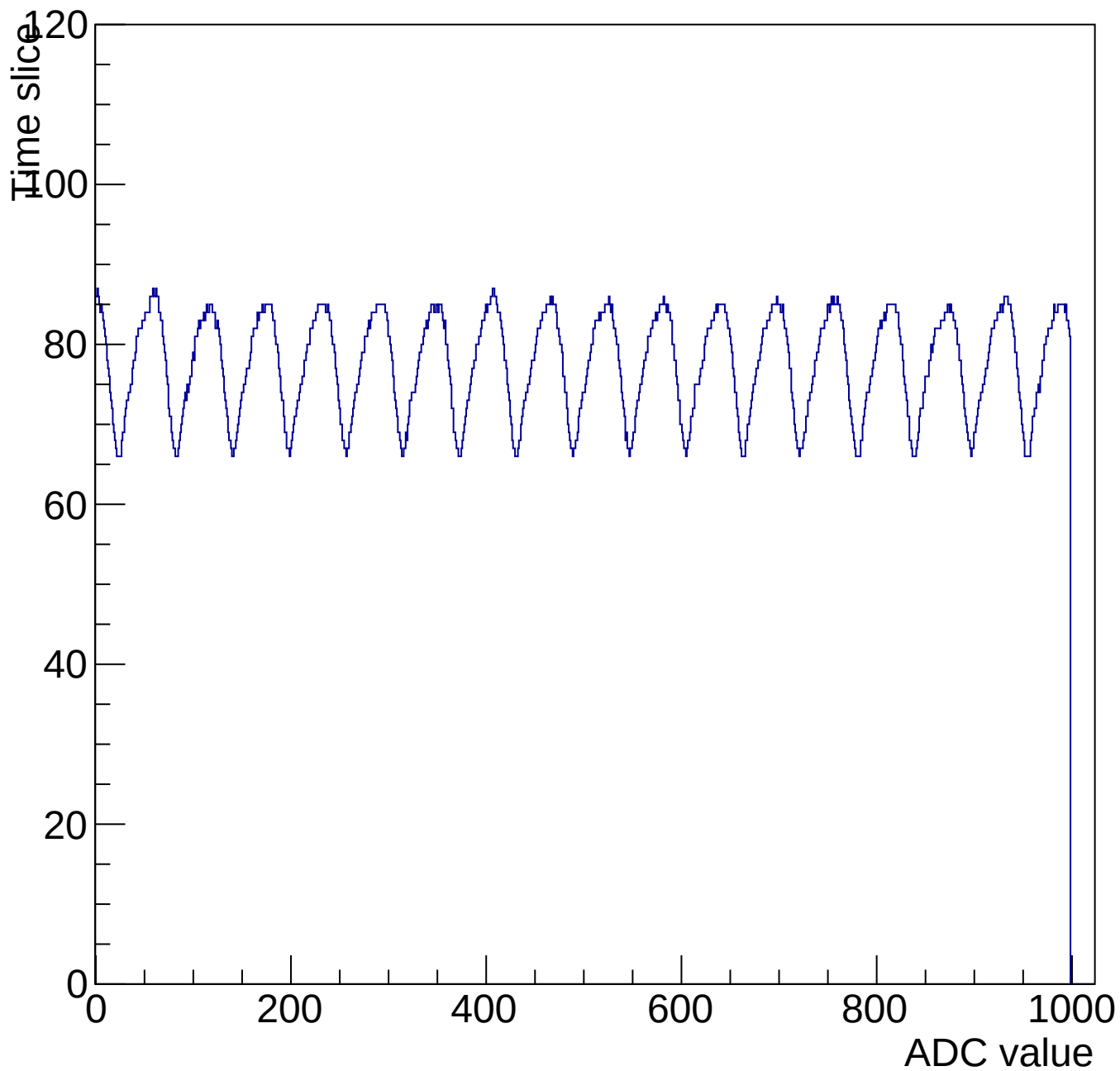
Evt 10 Time mcm 3004 chip 4 chan 7 1000-shift-gain0-shaper0
