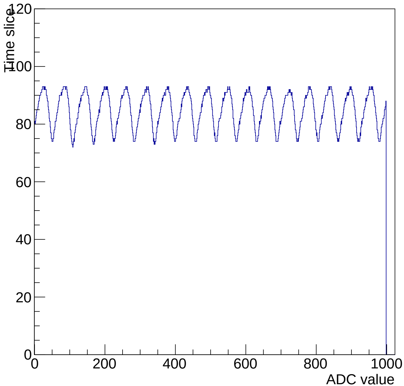
Evt 10 Time mcm 3004 chip 4 chan 5 1000-shift-gain0-shaper0
