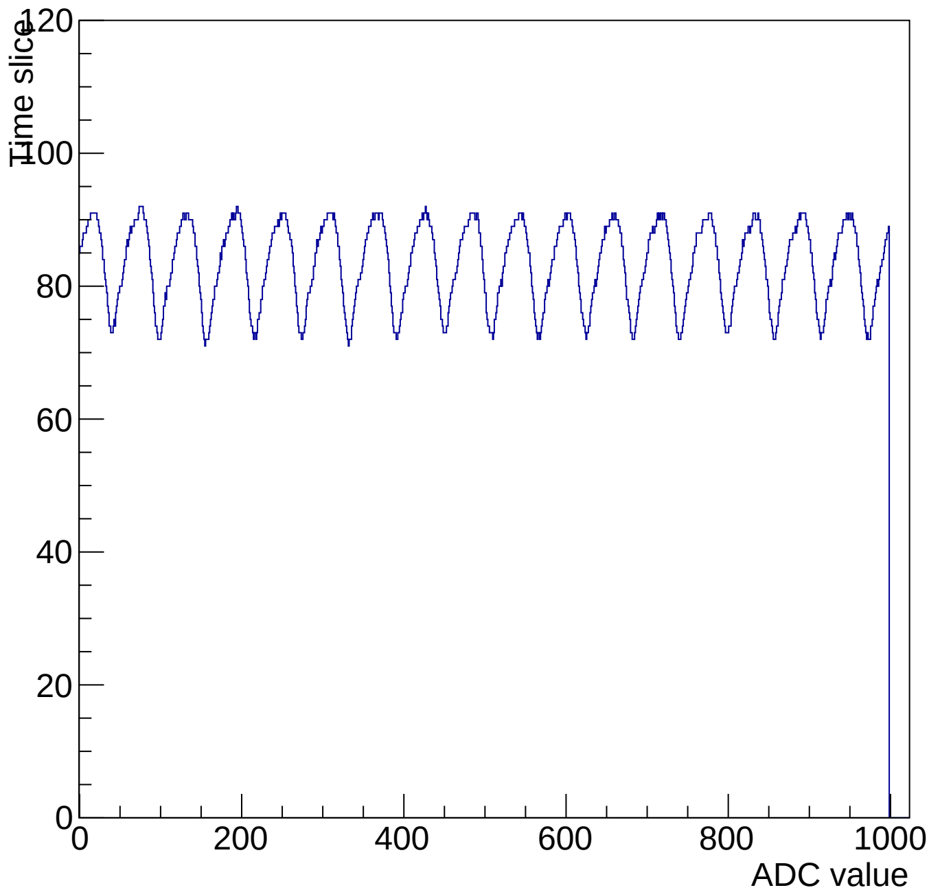
Evt 10 Time mcm 3004 chip 4 chan 10 1000-shift-gain0-shaper0
