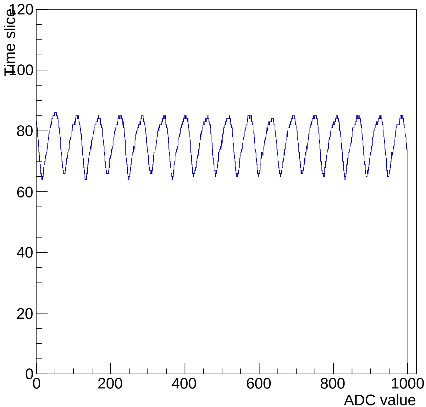
Evt 10 Time mcm 3004 chip 4 chan 0 1000-shift-gain0-shaper0
