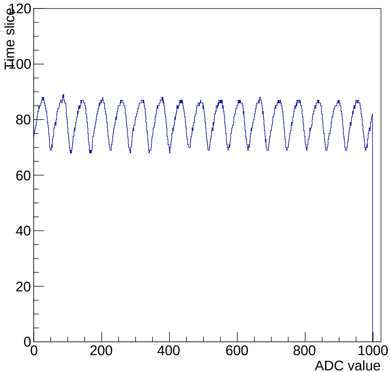
Evt 10 Time mcm 3004 chip 4 chan 4 1000-shift-gain0-shaper0
