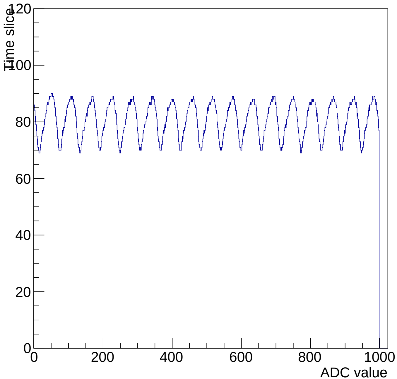
Evt 10 Time mcm 3004 chip 4 chan 1 1000-shift-gain0-shaper0
