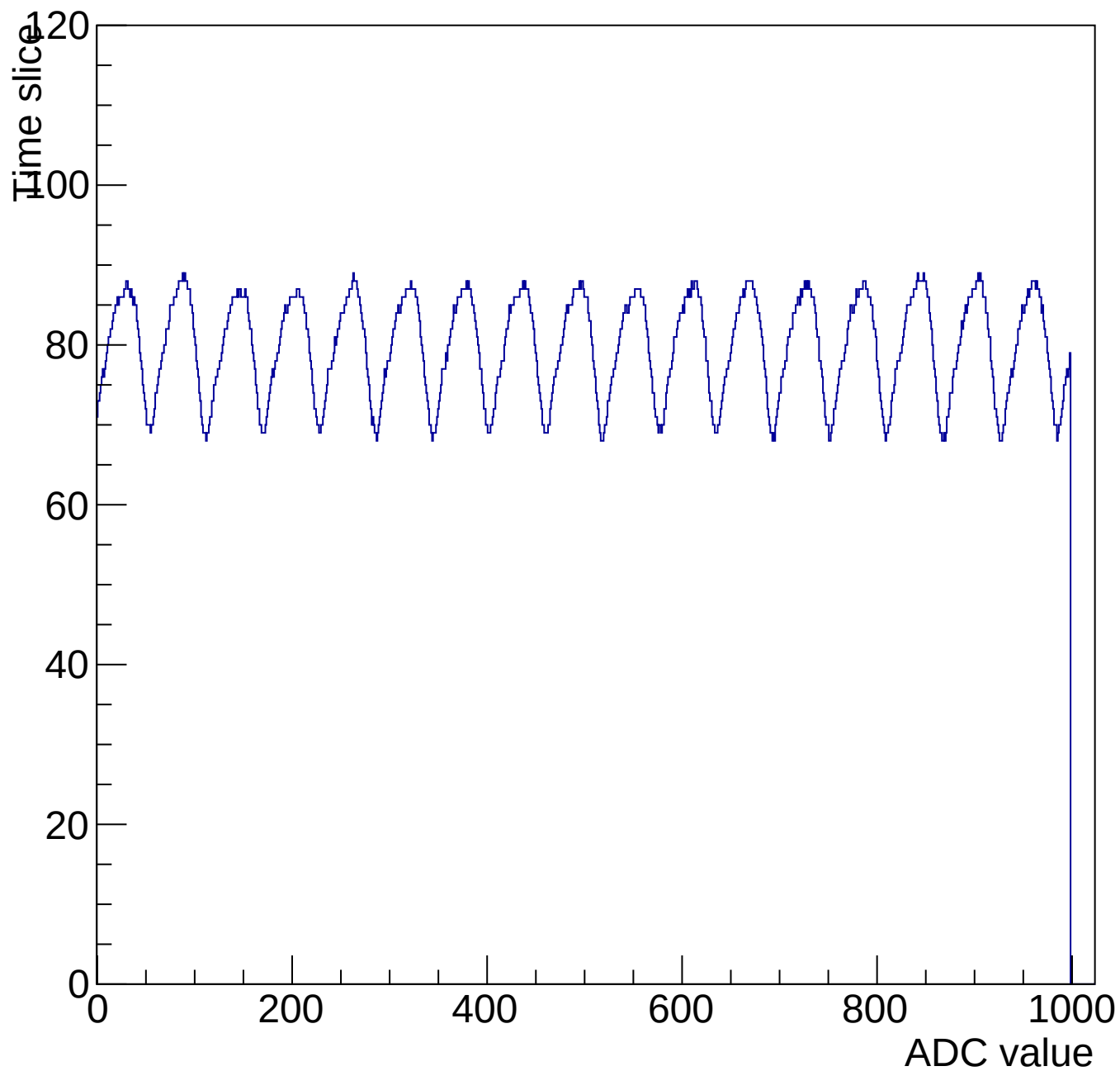
Evt 10 Time mcm 3004 chip 4 chan 8 1000-shift-gain0-shaper0
