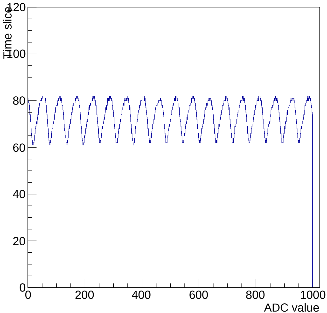
Evt 10 Time mcm 3004 chip 4 chan 14 1000-shift-gain0-shaper0
