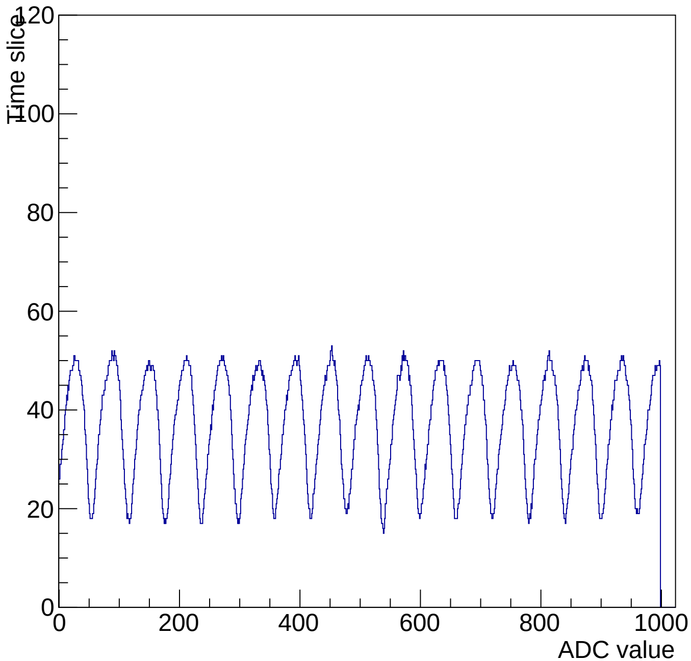
Evt 10 Time mcm 3004 chip 4 chan 5 1000-shift-gain3-shaper0
