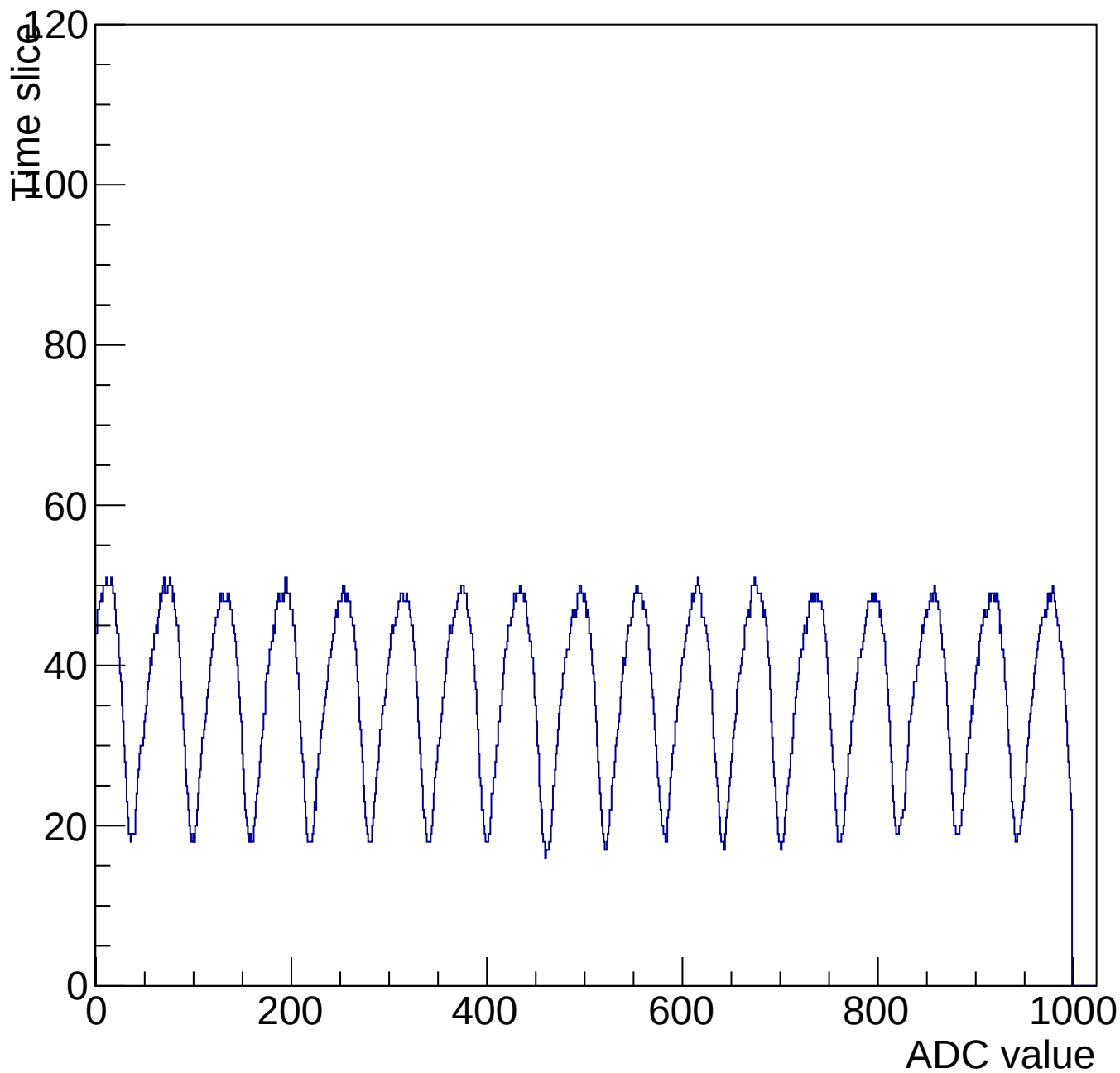
Evt 10 Time mcm 3004 chip 4 chan 1 1000-shift-gain3-shaper0
