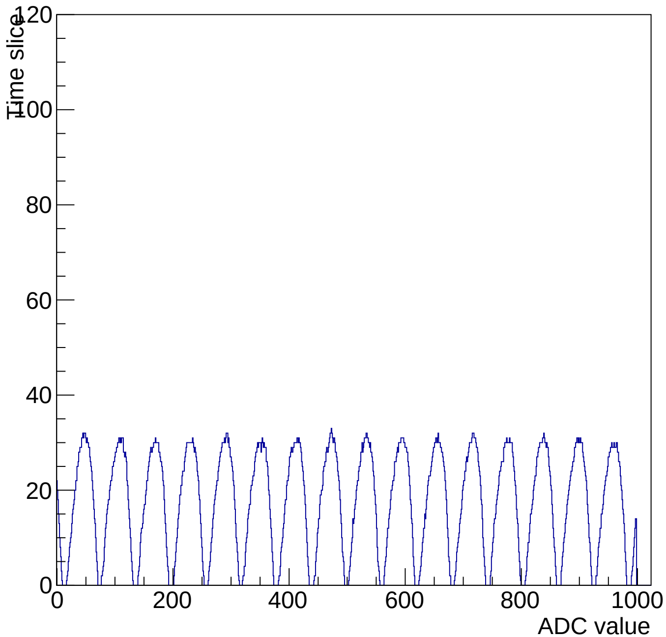
Evt 10 Time mcm 3004 chip 4 chan 2 1000-shift-gain3-shaper0
