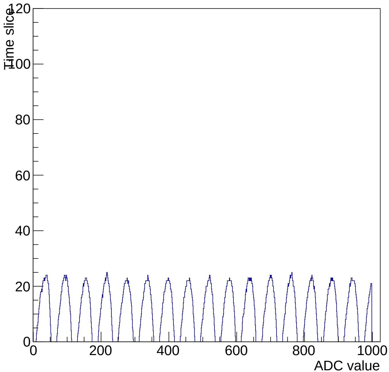
Evt 10 Time mcm 3004 chip 4 chan 6 1000-shift-gain3-shaper0
