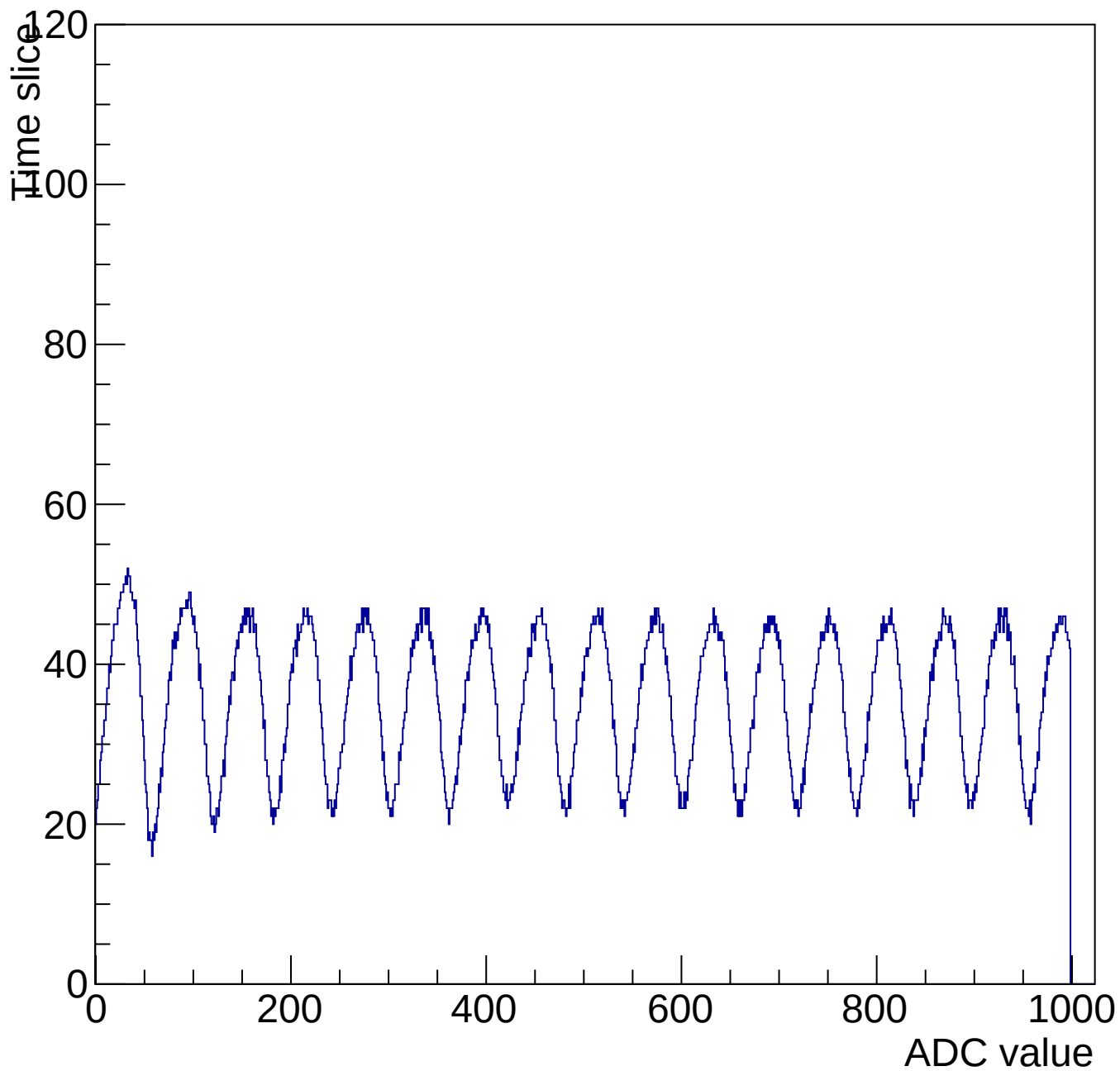
Evt 10 Time mcm 3004 chip 4 chan 12 1000-shift-gain3-shaper7
