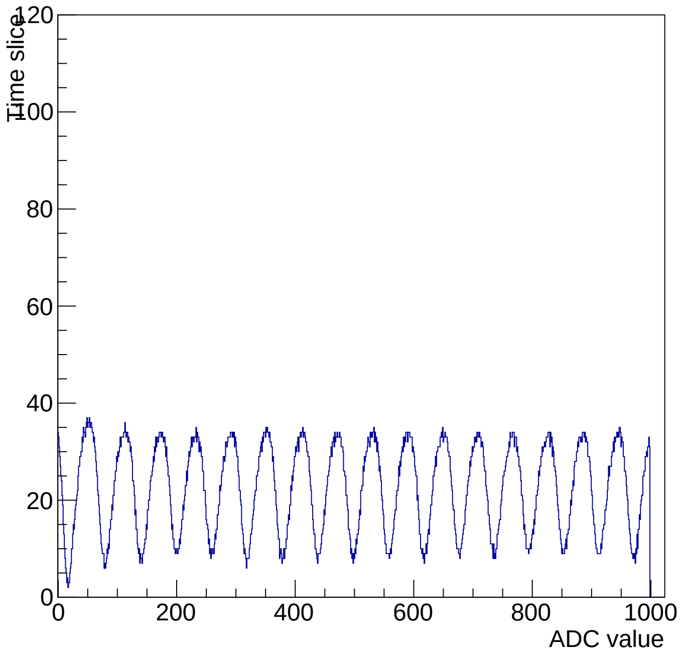
Evt 10 Time mcm 3004 chip 4 chan 3 1000-shift-gain3-shaper7
