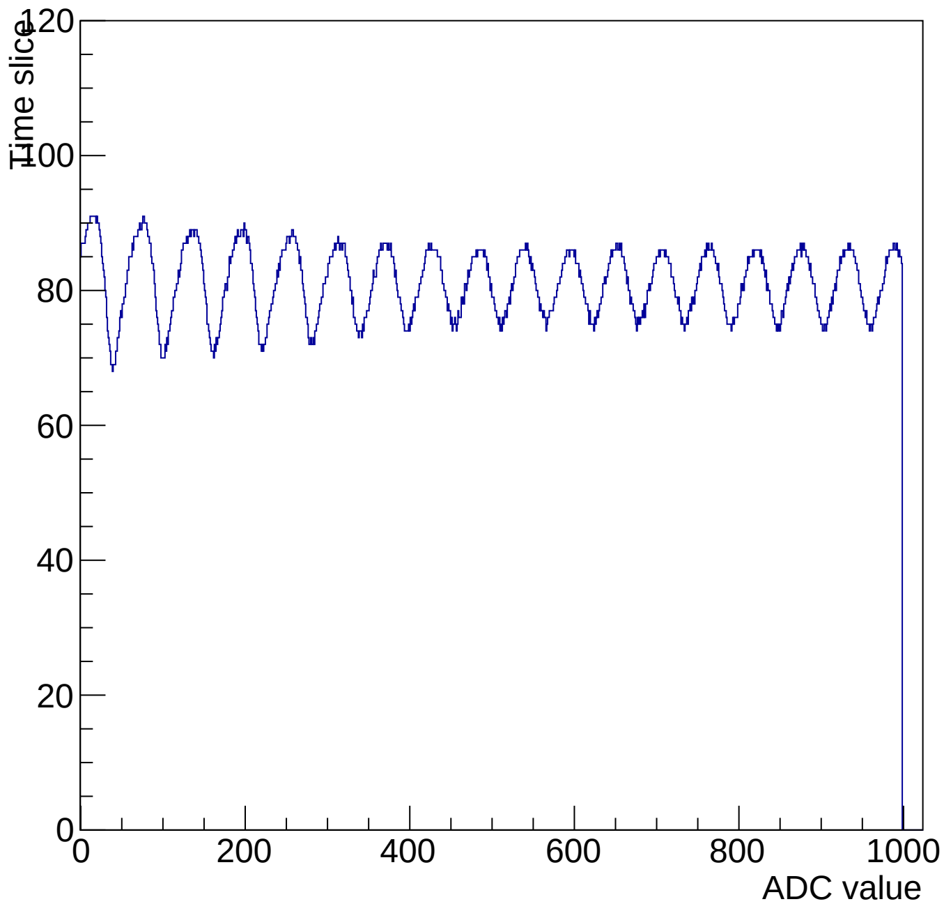
Evt 11 Time mcm 3004 chip 4 chan 10 1000-shift-gain0-shaper7
