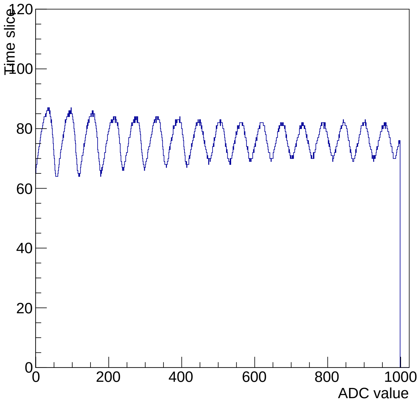
Evt 11 Time mcm 3004 chip 4 chan 7 1000-shift-gain0-shaper7
