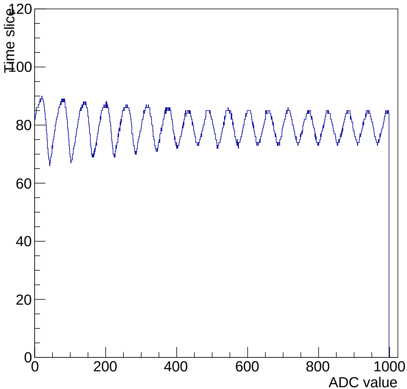
Evt 11 Time mcm 3004 chip 4 chan 8 1000-shift-gain0-shaper7
