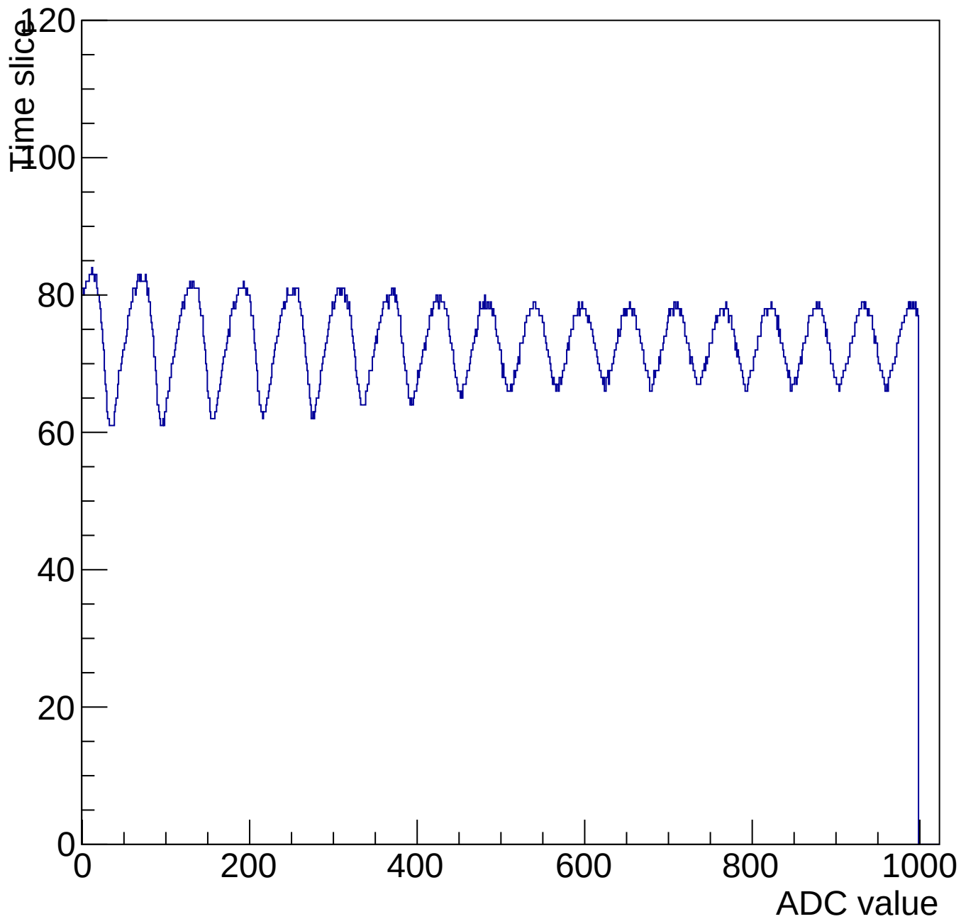
Evt 11 Time mcm 3004 chip 4 chan 3 1000-shift-gain0-shaper7
