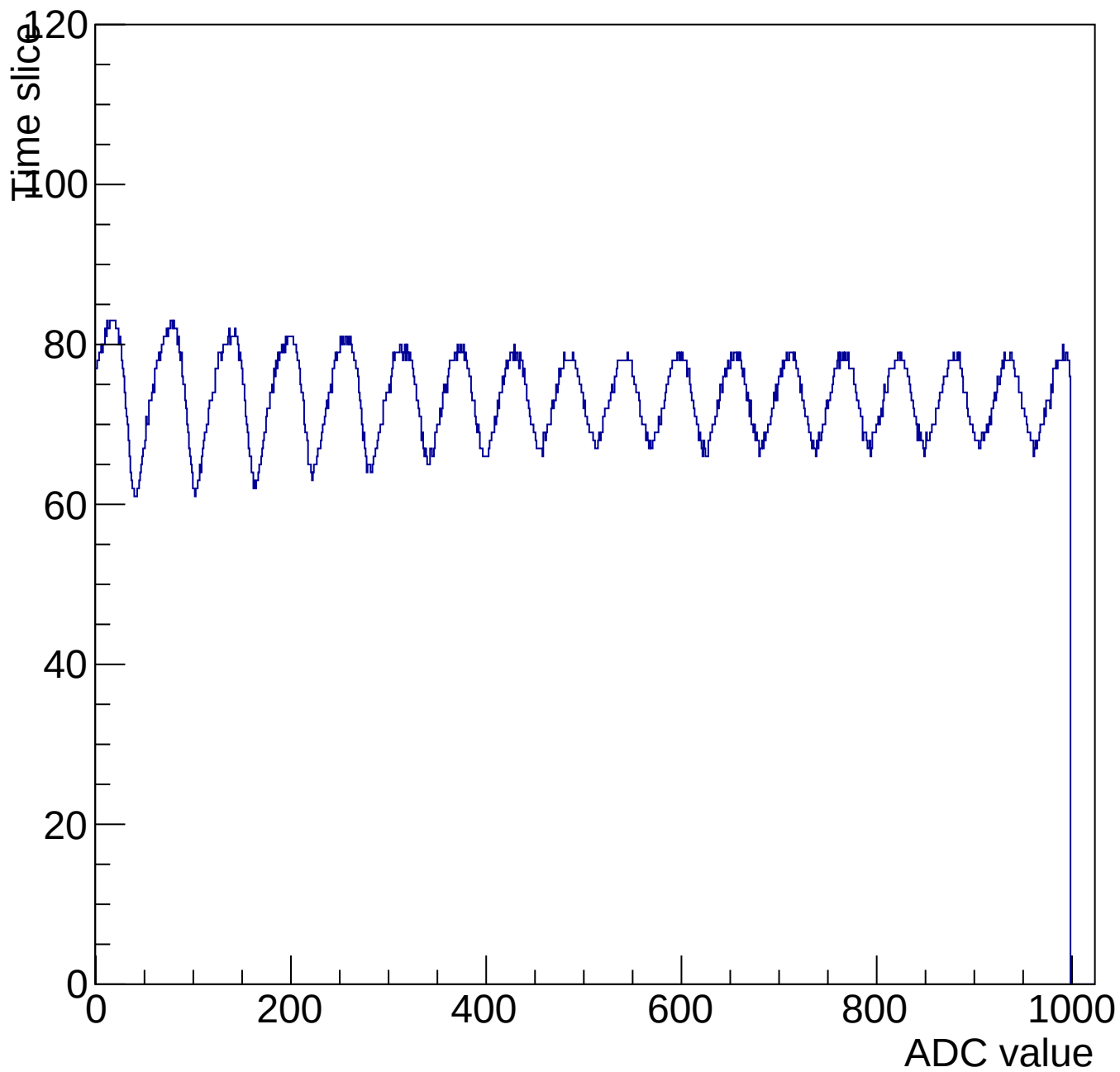
Evt 11 Time mcm 3004 chip 4 chan 13 1000-shift-gain0-shaper7
