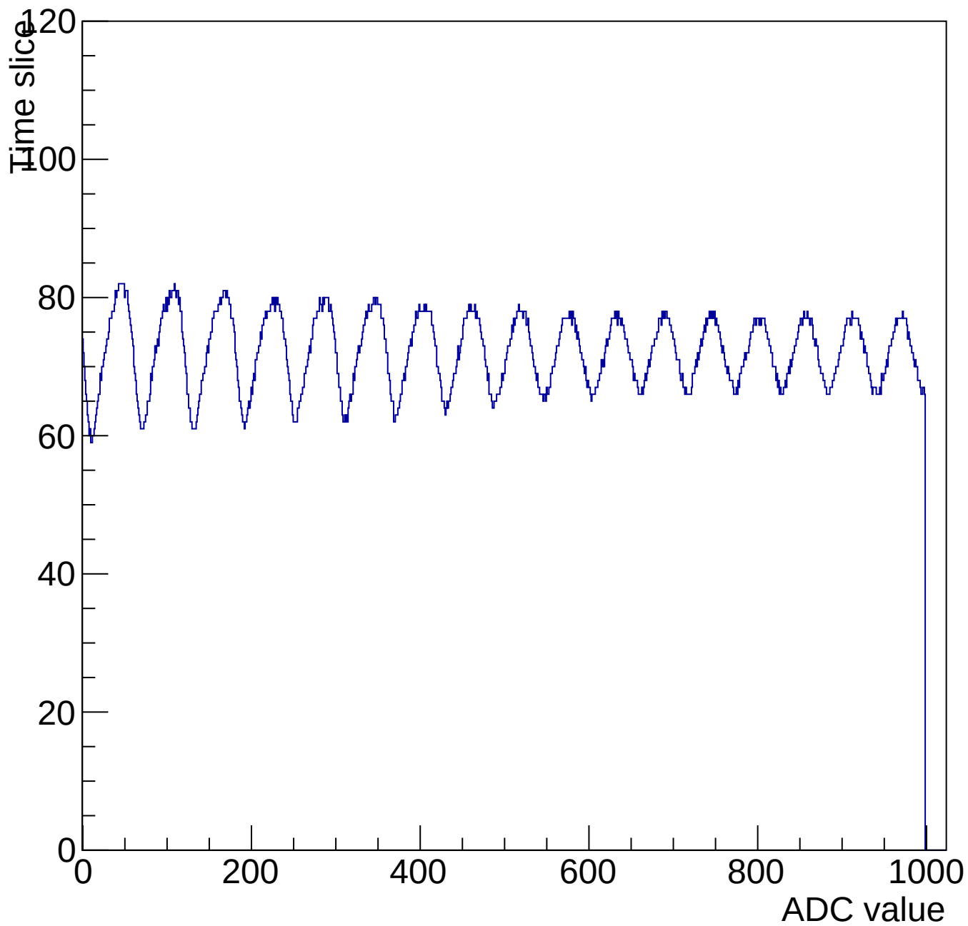
Evt 11 Time mcm 3004 chip 4 chan 15 1000-shift-gain0-shaper7
