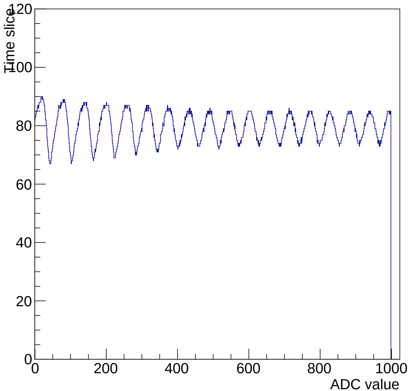
Evt 11 Time mcm 3004 chip 4 chan 9 1000-shift-gain0-shaper7
