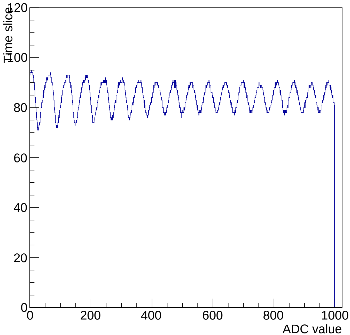
Evt 11 Time mcm 3004 chip 4 chan 5 1000-shift-gain0-shaper7
