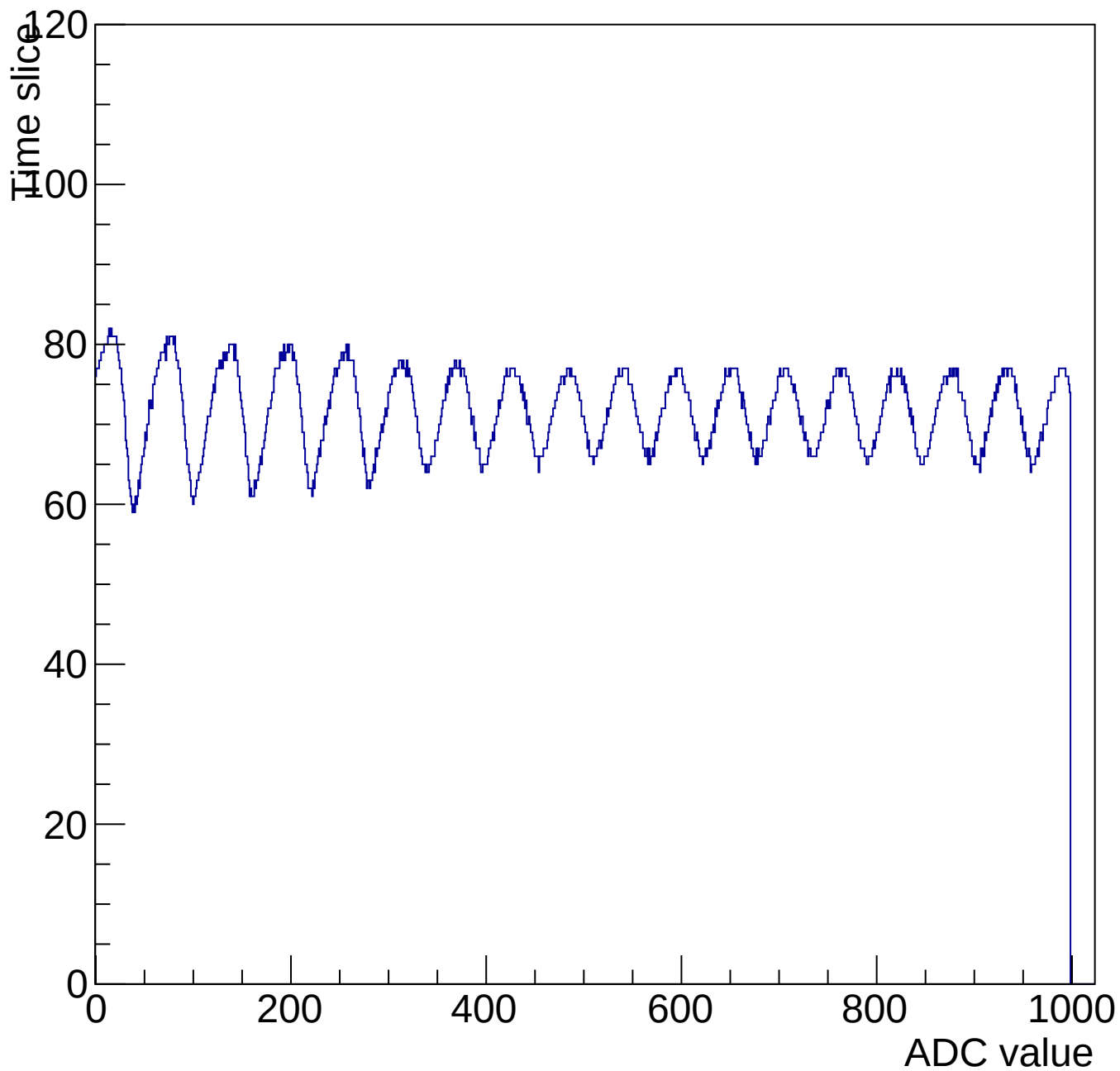
Evt 11 Time mcm 3004 chip 4 chan 11 1000-shift-gain0-shaper7
