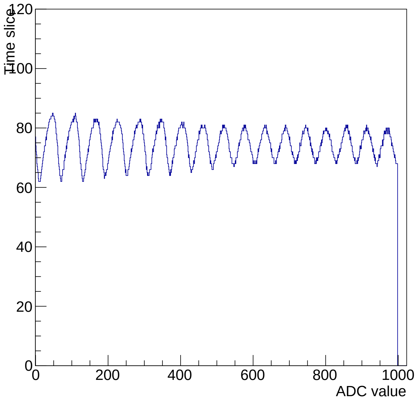
Evt 11 Time mcm 3004 chip 4 chan 14 1000-shift-gain0-shaper7
