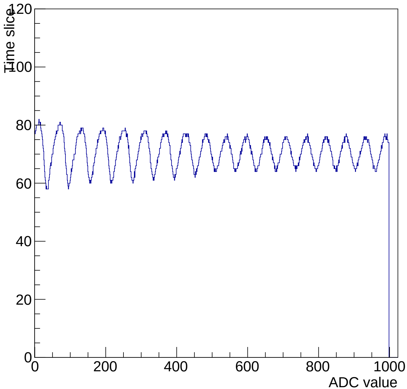
Evt 11 Time mcm 3004 chip 4 chan 2 1000-shift-gain0-shaper7
