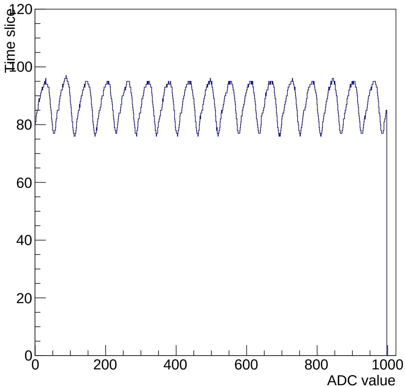
Evt 10 Time mcm 3005 chip 5 chan 11 1000-shift-gain0-shaper0
