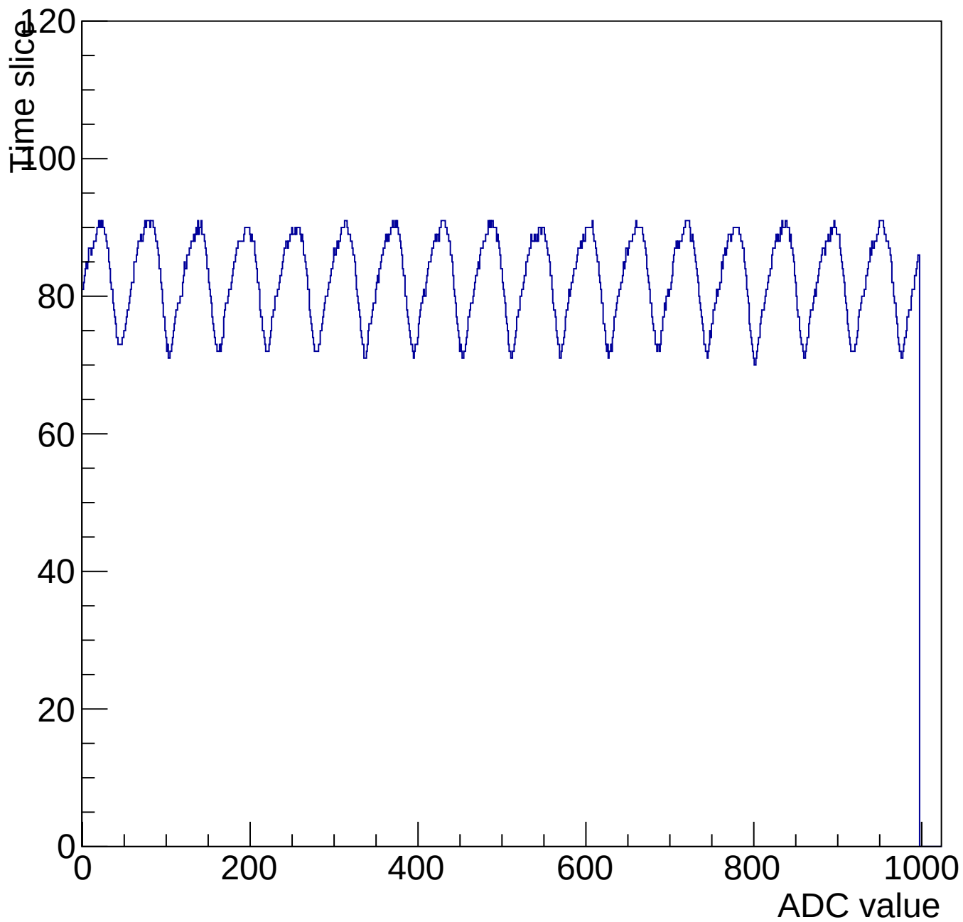
Evt 10 Time mcm 3005 chip 5 chan 15 1000-shift-gain0-shaper0
