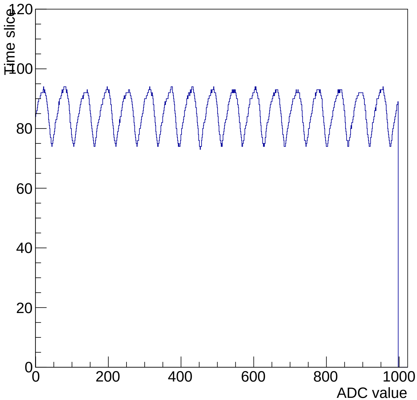
Evt 10 Time mcm 3005 chip 5 chan 14 1000-shift-gain0-shaper0
