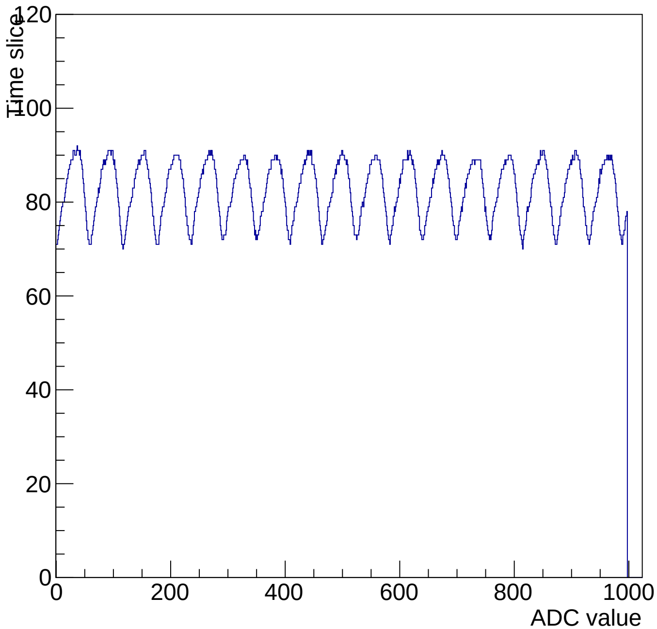
Evt 10 Time mcm 3005 chip 5 chan 13 1000-shift-gain0-shaper0
