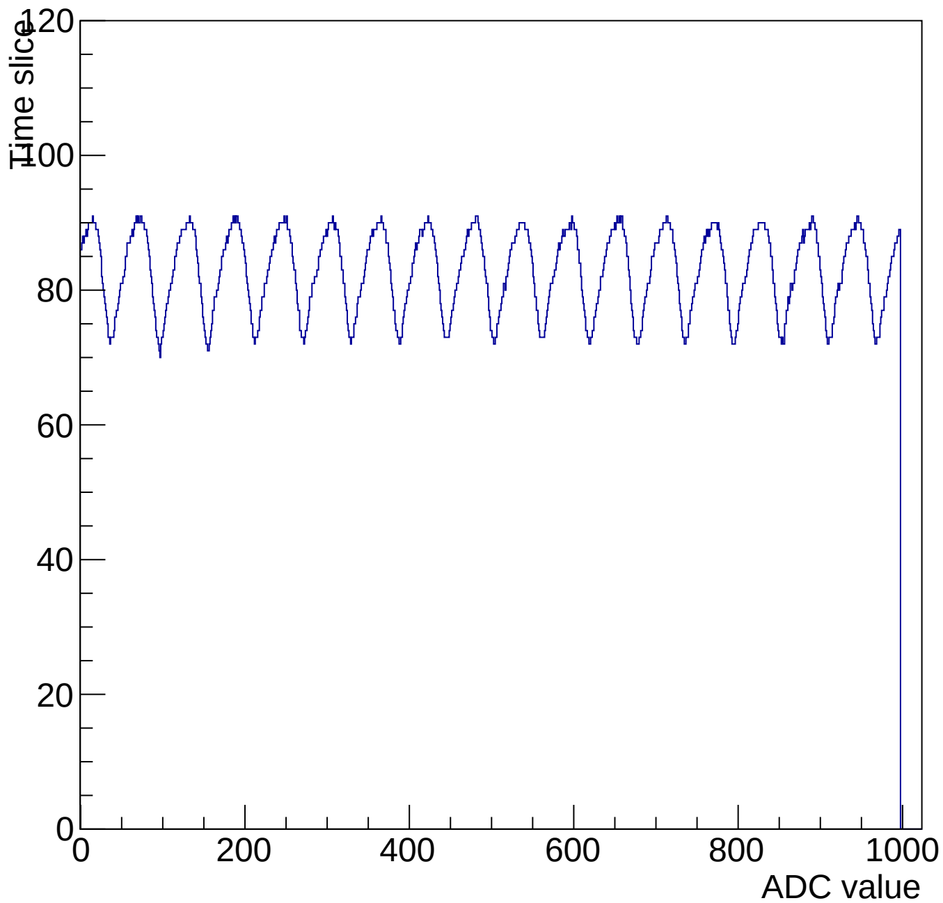
Evt 10 Time mcm 3005 chip 5 chan 5 1000-shift-gain0-shaper0
