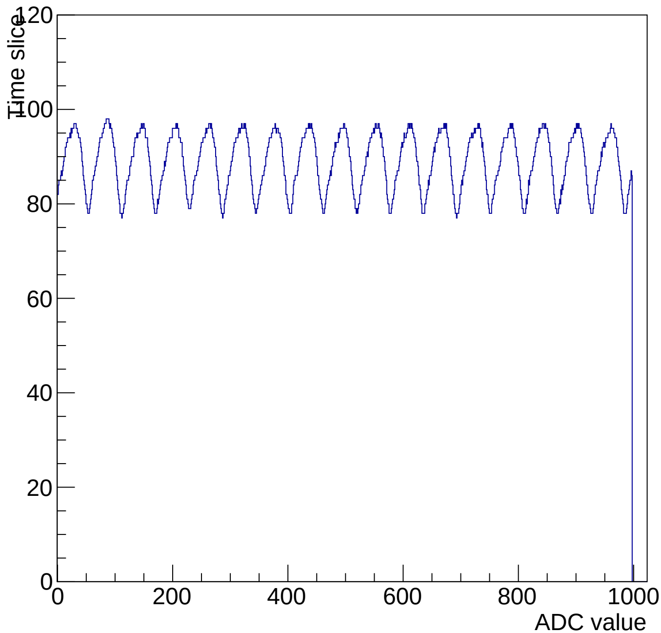
Evt 10 Time mcm 3005 chip 5 chan 10 1000-shift-gain0-shaper0
