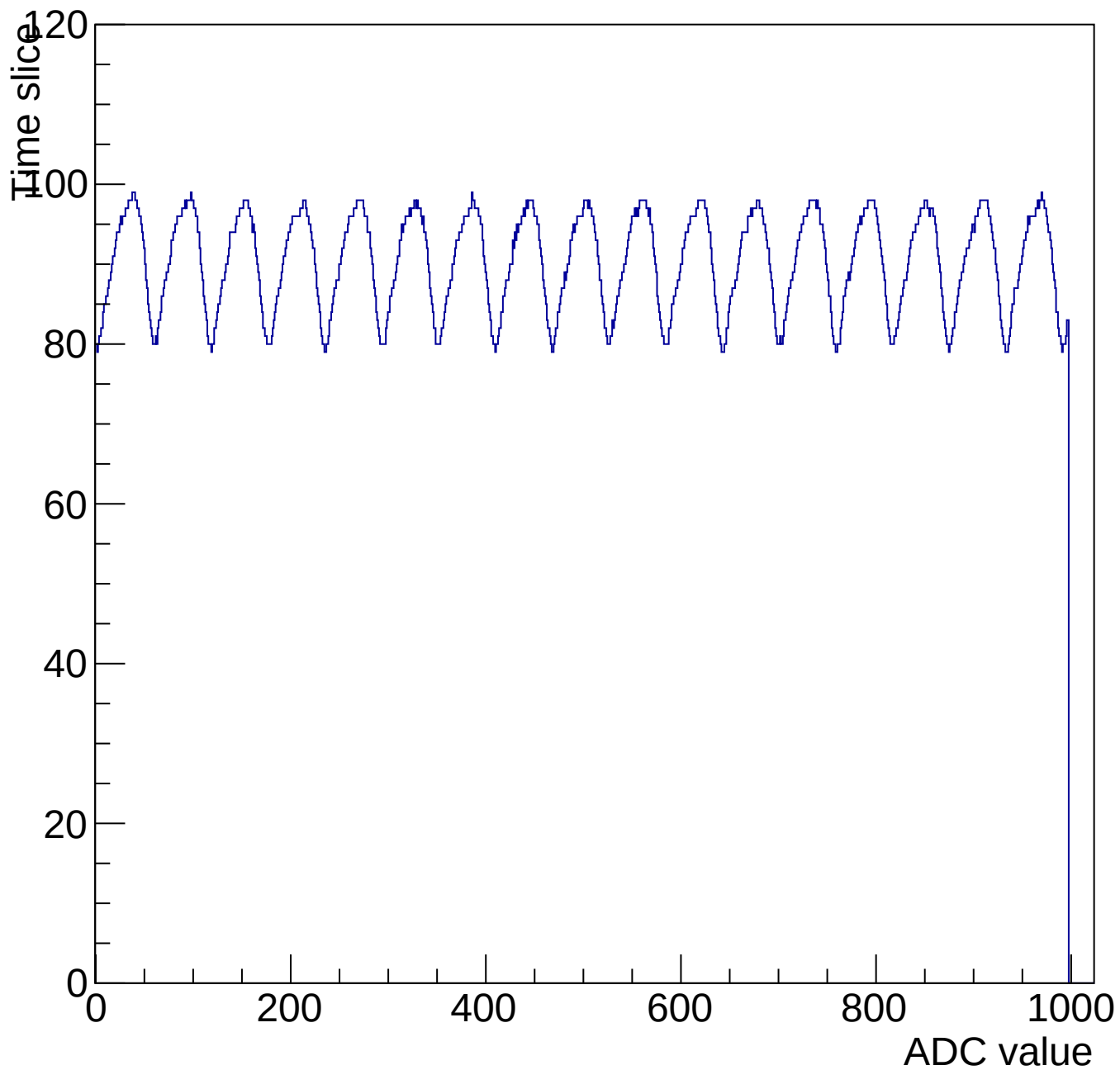
Evt 10 Time mcm 3005 chip 5 chan 1 1000-shift-gain0-shaper0
