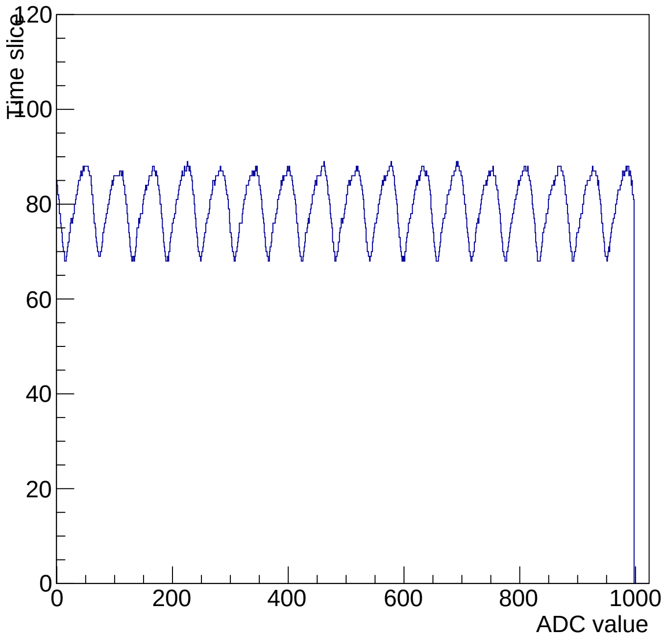
Evt 10 Time mcm 3005 chip 5 chan 2 1000-shift-gain0-shaper0
