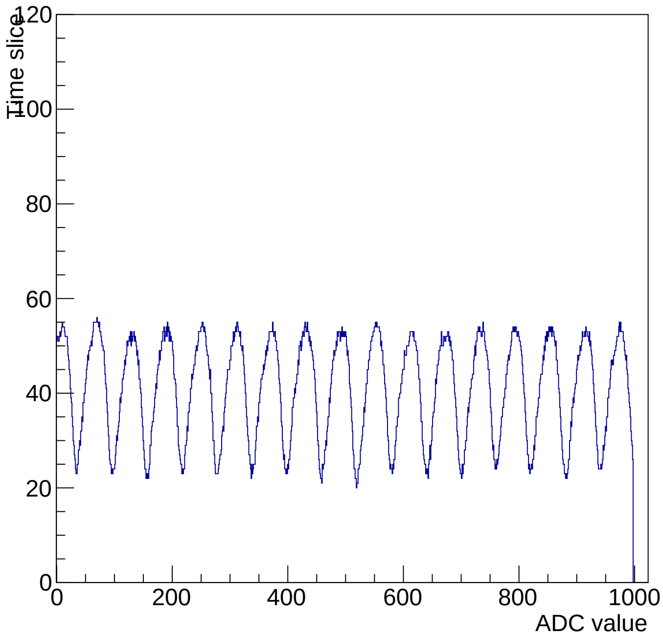
Evt 10 Time mcm 3005 chip 5 chan 0 1000-shift-gain3-shaper0
