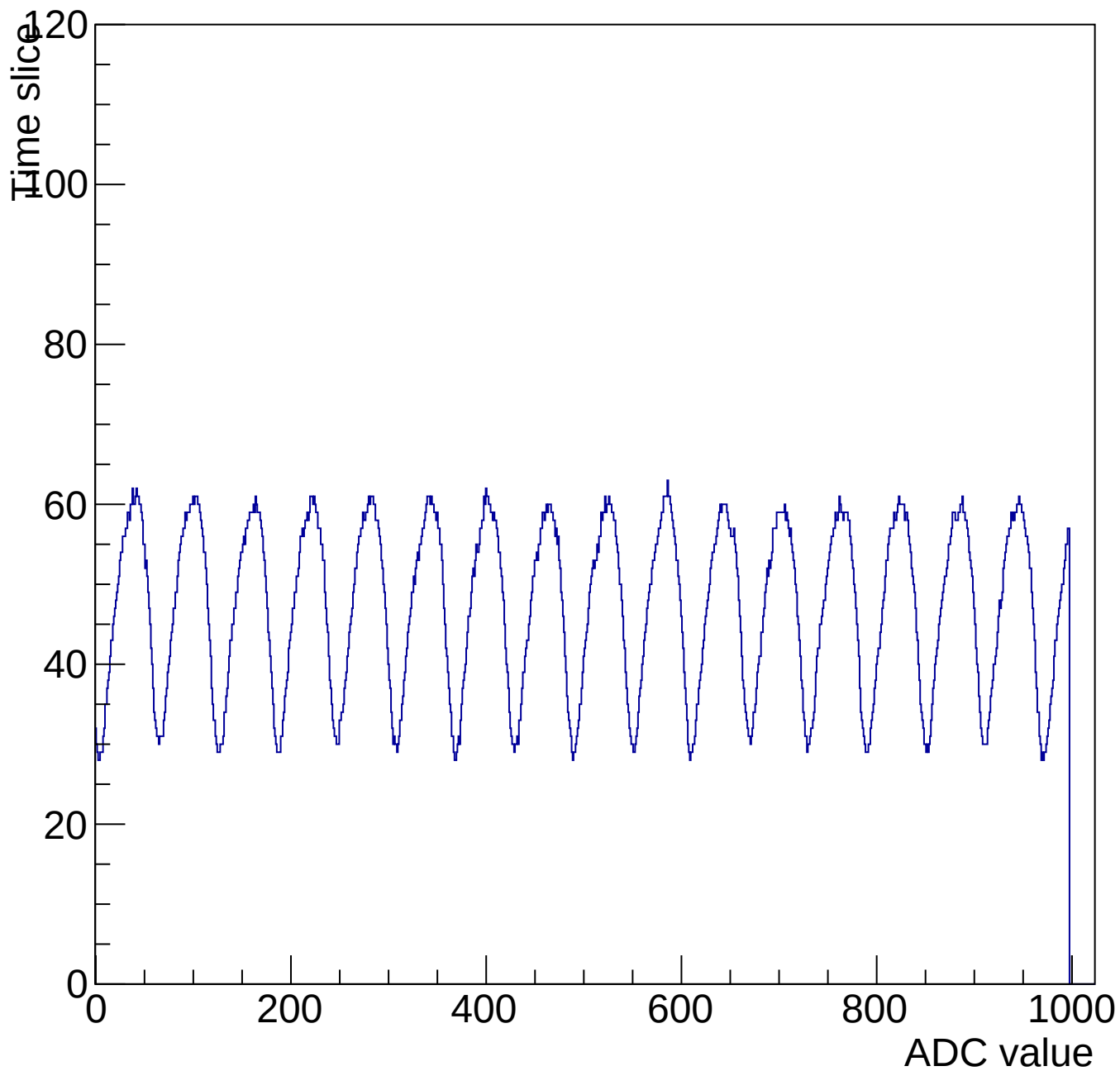
Evt 10 Time mcm 3005 chip 5 chan 12 1000-shift-gain3-shaper0
