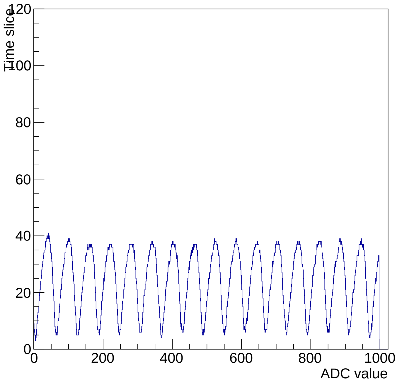
Evt 10 Time mcm 3005 chip 5 chan 13 1000-shift-gain3-shaper0
