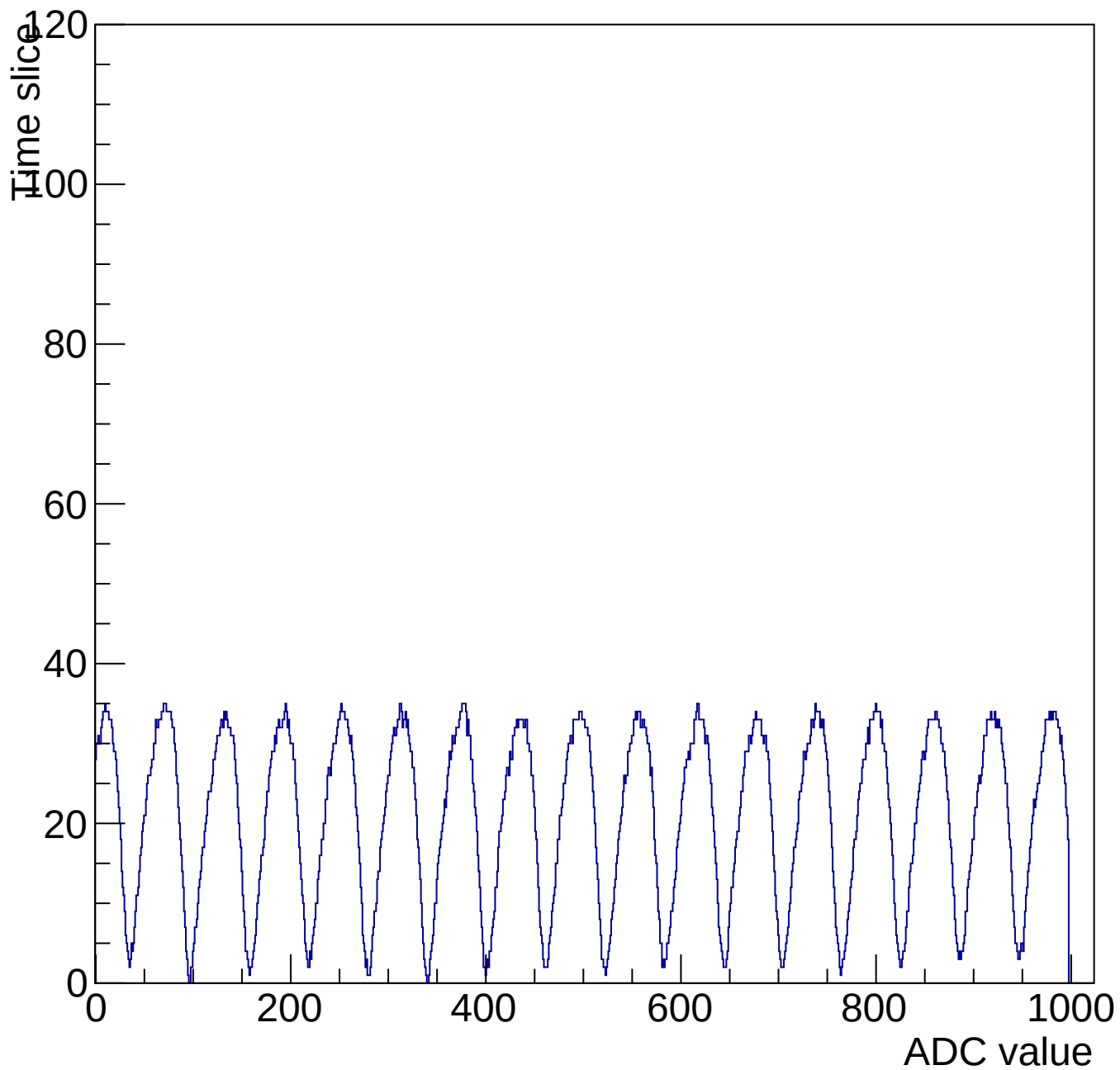
Evt 10 Time mcm 3005 chip 5 chan 6 1000-shift-gain3-shaper0
