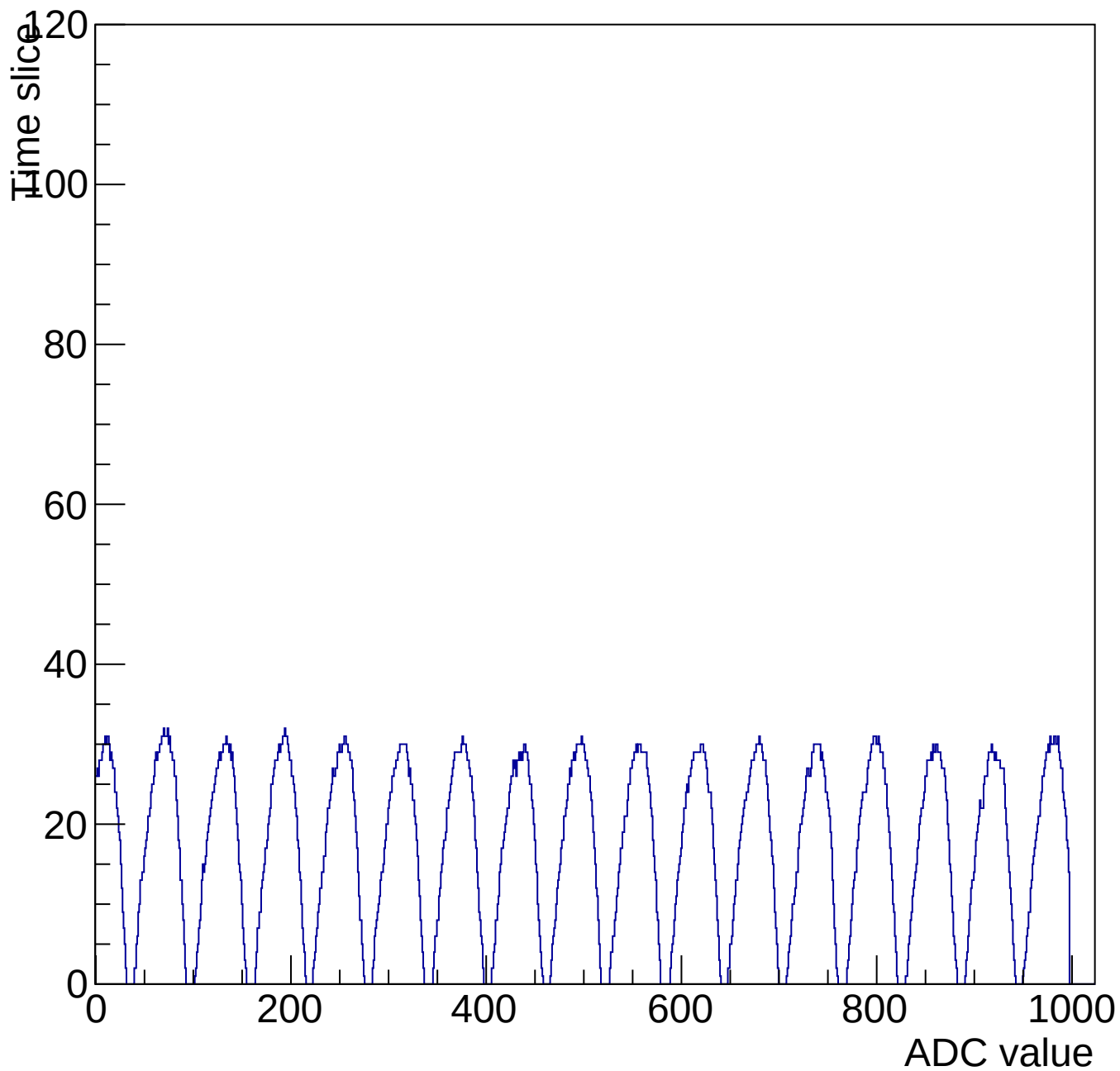
Evt 10 Time mcm 3005 chip 5 chan 7 1000-shift-gain3-shaper0
