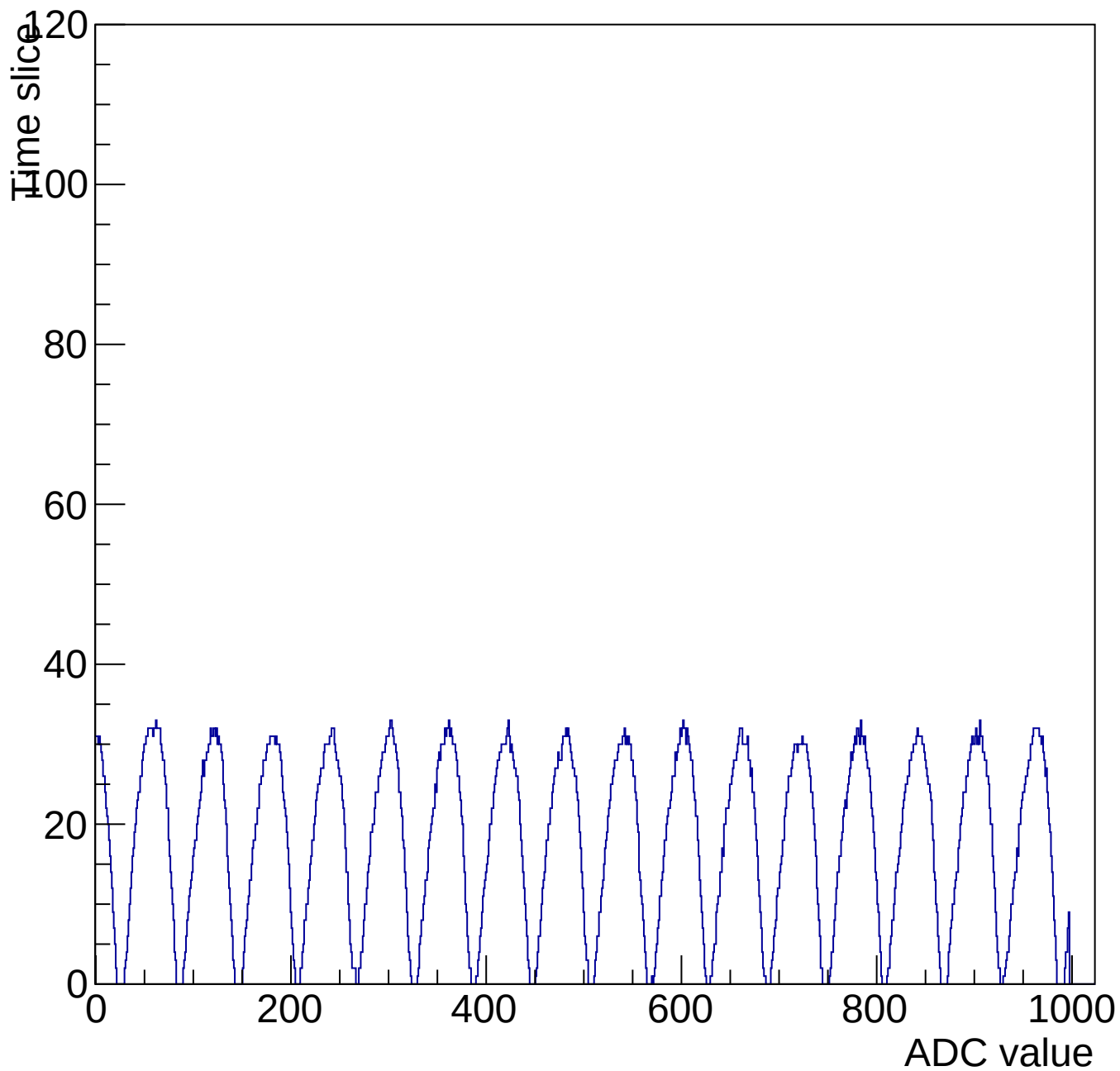
Evt 10 Time mcm 3005 chip 5 chan 2 1000-shift-gain3-shaper0
