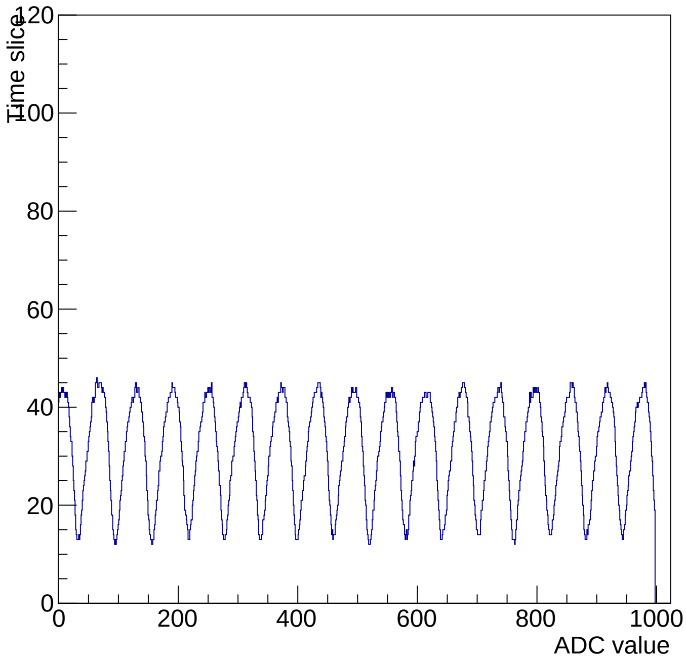
Evt 10 Time mcm 3005 chip 5 chan 5 1000-shift-gain3-shaper0
