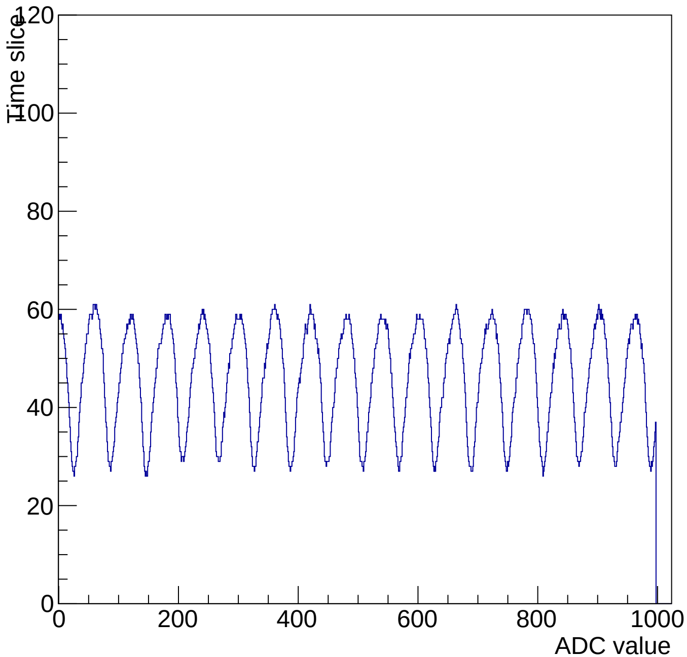
Evt 10 Time mcm 3005 chip 5 chan 3 1000-shift-gain3-shaper0
