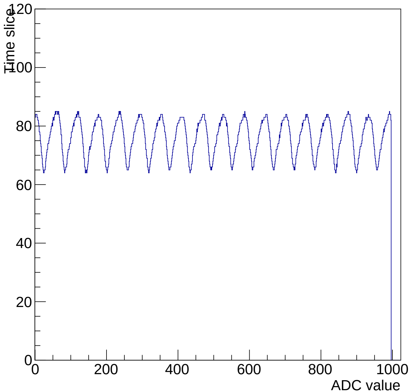
Evt 10 Time mcm 3006 chip 6 chan 5 1000-shift-gain0-shaper0
