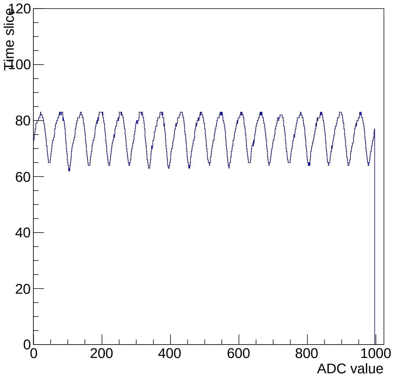
Evt 10 Time mcm 3006 chip 6 chan 6 1000-shift-gain0-shaper0
