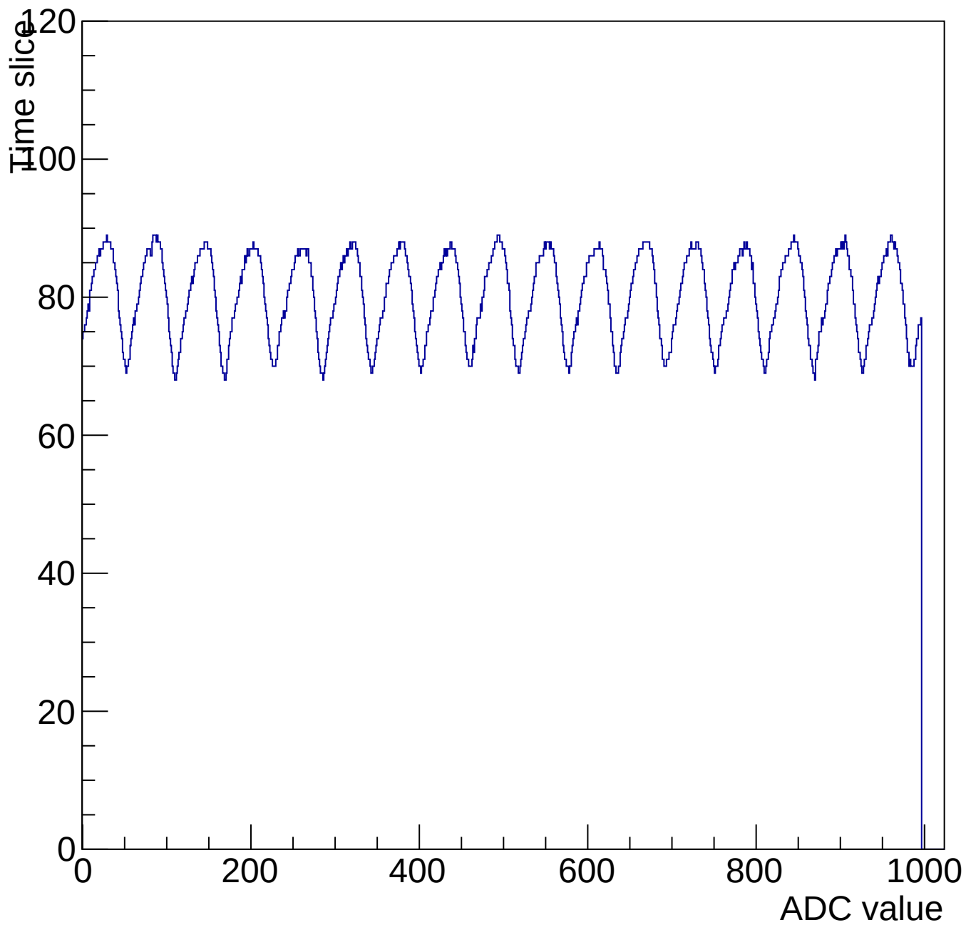
Evt 10 Time mcm 3006 chip 6 chan 15 1000-shift-gain0-shaper0
