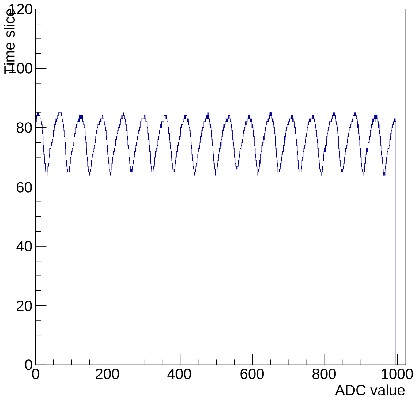
Evt 10 Time mcm 3006 chip 6 chan 0 1000-shift-gain0-shaper0
