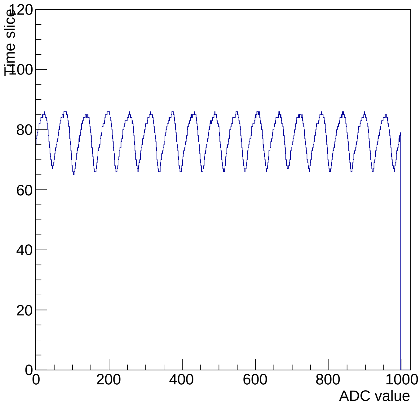
Evt 10 Time mcm 3006 chip 6 chan 7 1000-shift-gain0-shaper0
