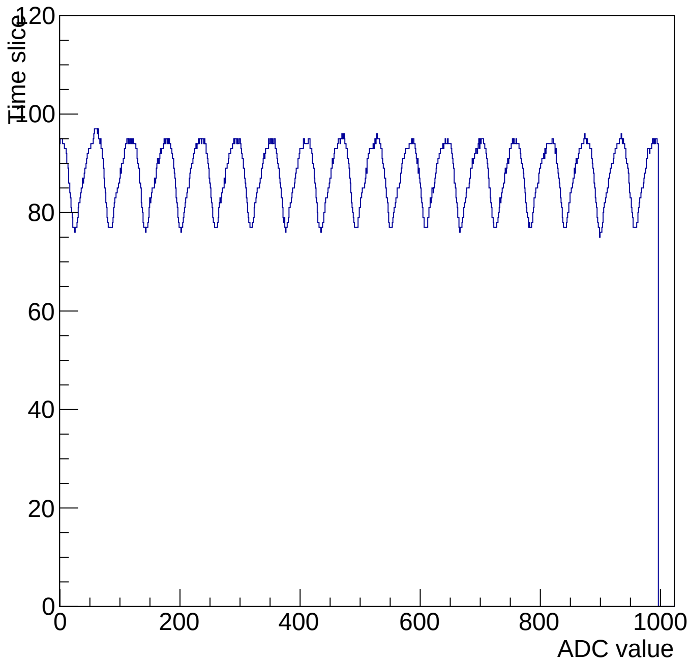
Evt 10 Time mcm 3006 chip 6 chan 4 1000-shift-gain0-shaper0
