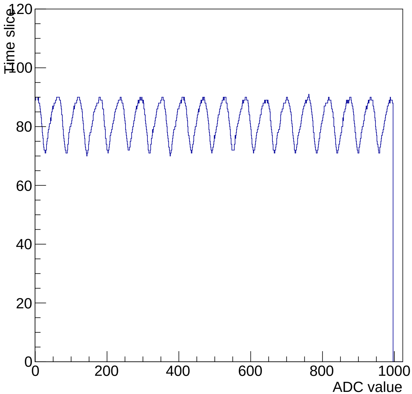
Evt 10 Time mcm 3006 chip 6 chan 9 1000-shift-gain0-shaper0
