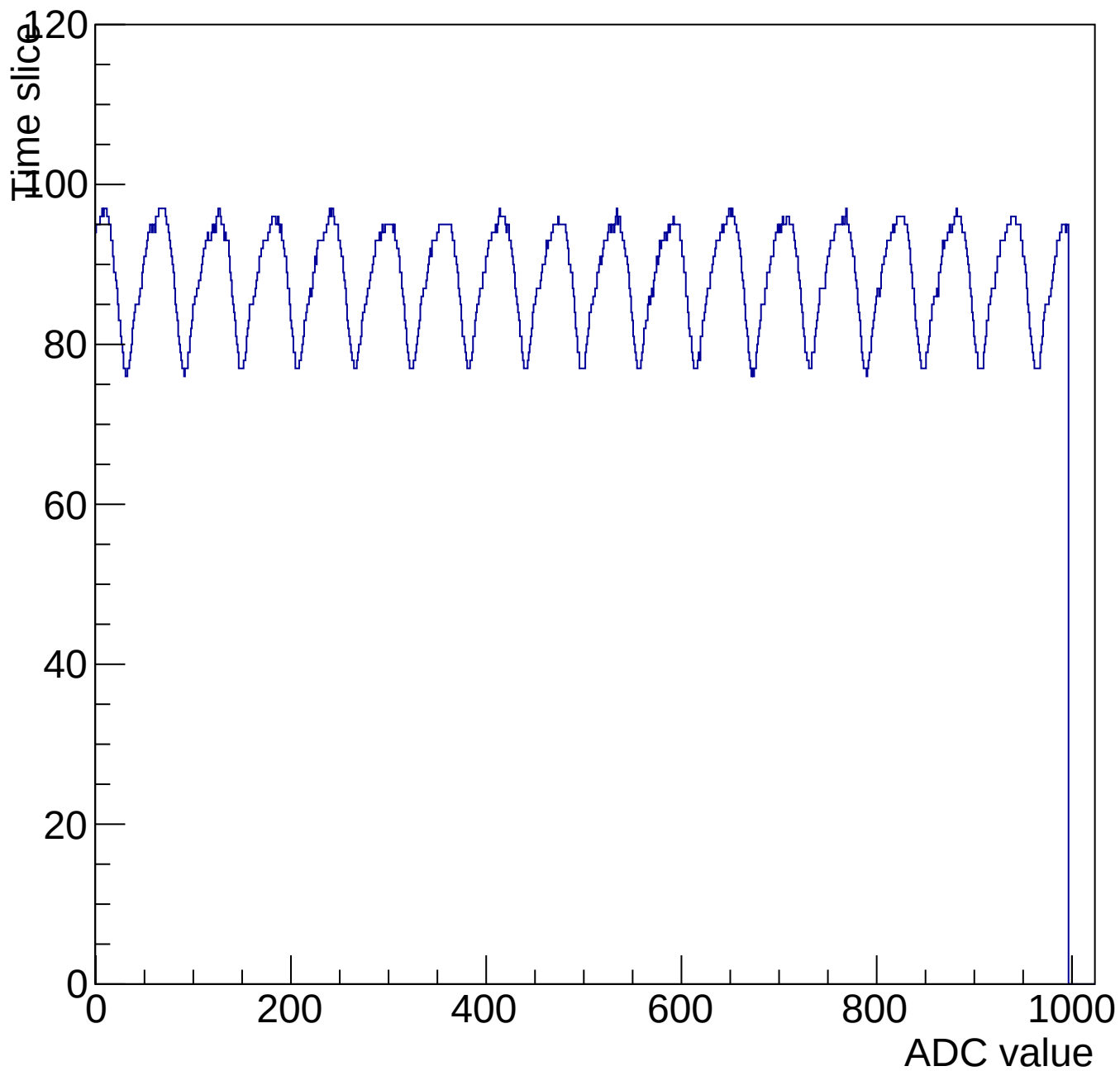
Evt 10 Time mcm 3006 chip 6 chan 1 1000-shift-gain0-shaper0
