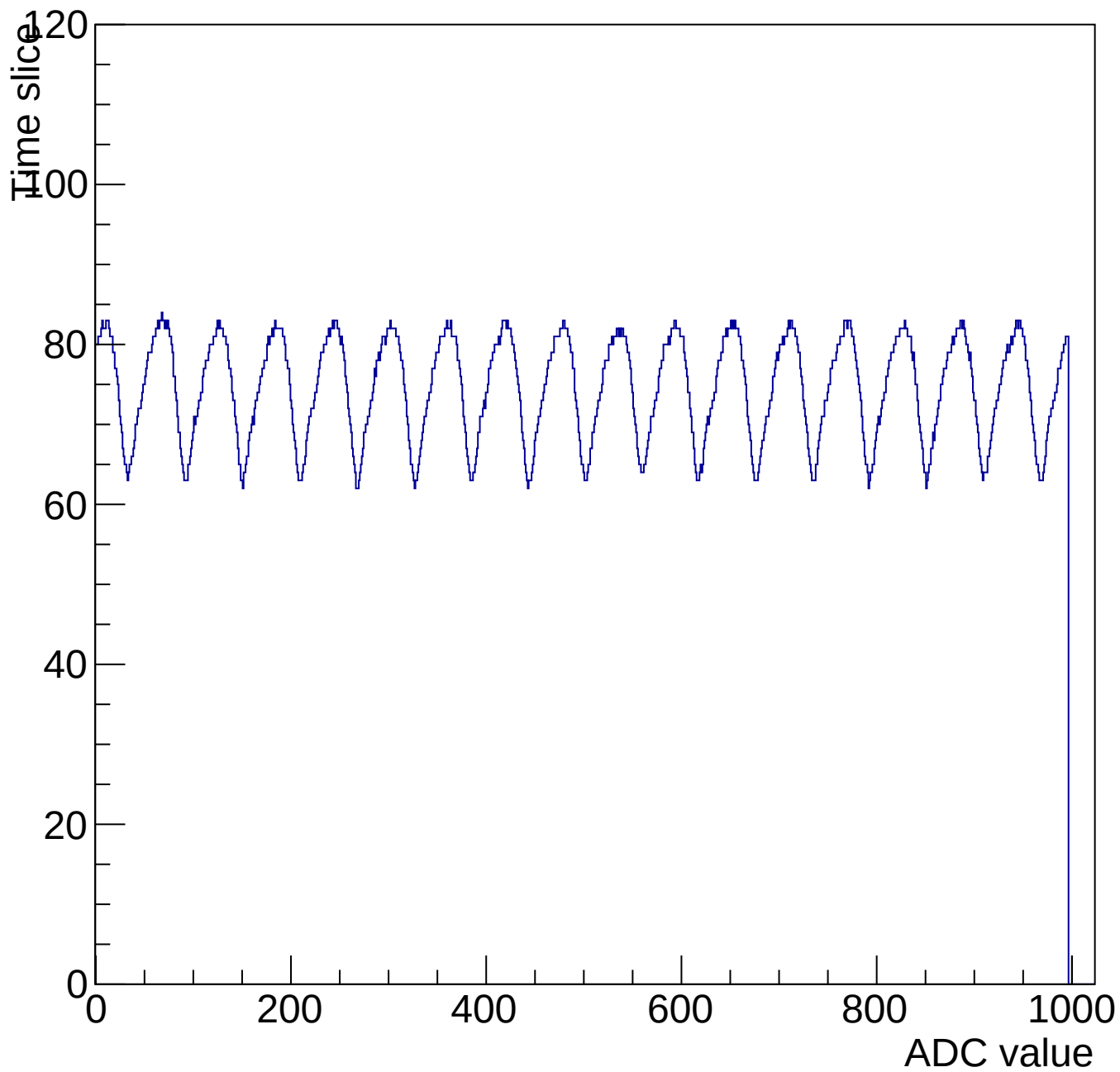
Evt 10 Time mcm 3006 chip 6 chan 11 1000-shift-gain0-shaper0
