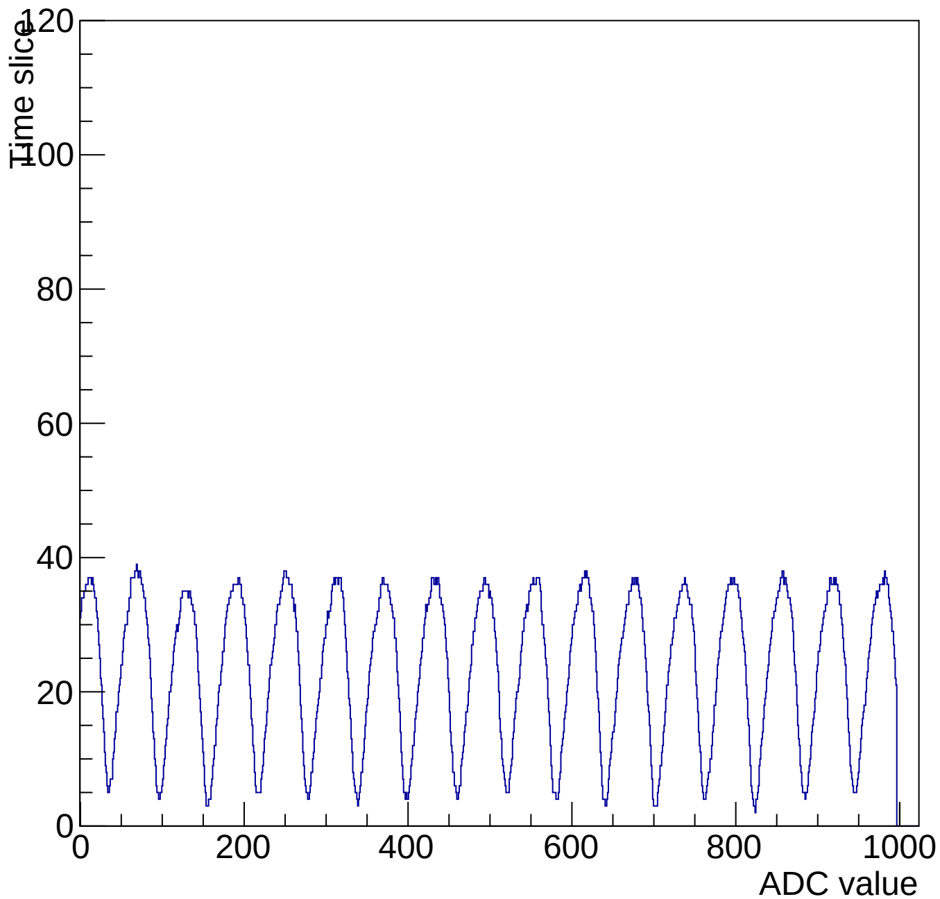
Evt 10 Time mcm 3006 chip 6 chan 0 1000-shift-gain3-shaper0
