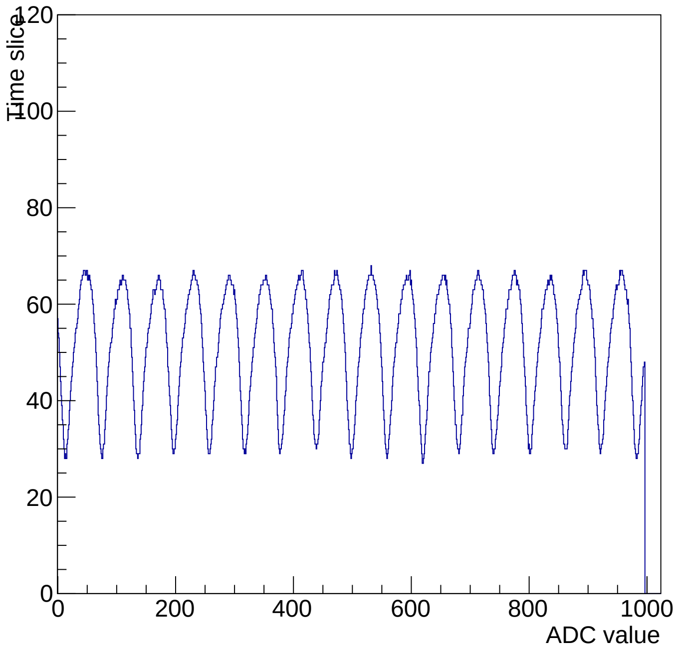
Evt 10 Time mcm 3006 chip 6 chan 2 1000-shift-gain3-shaper0
