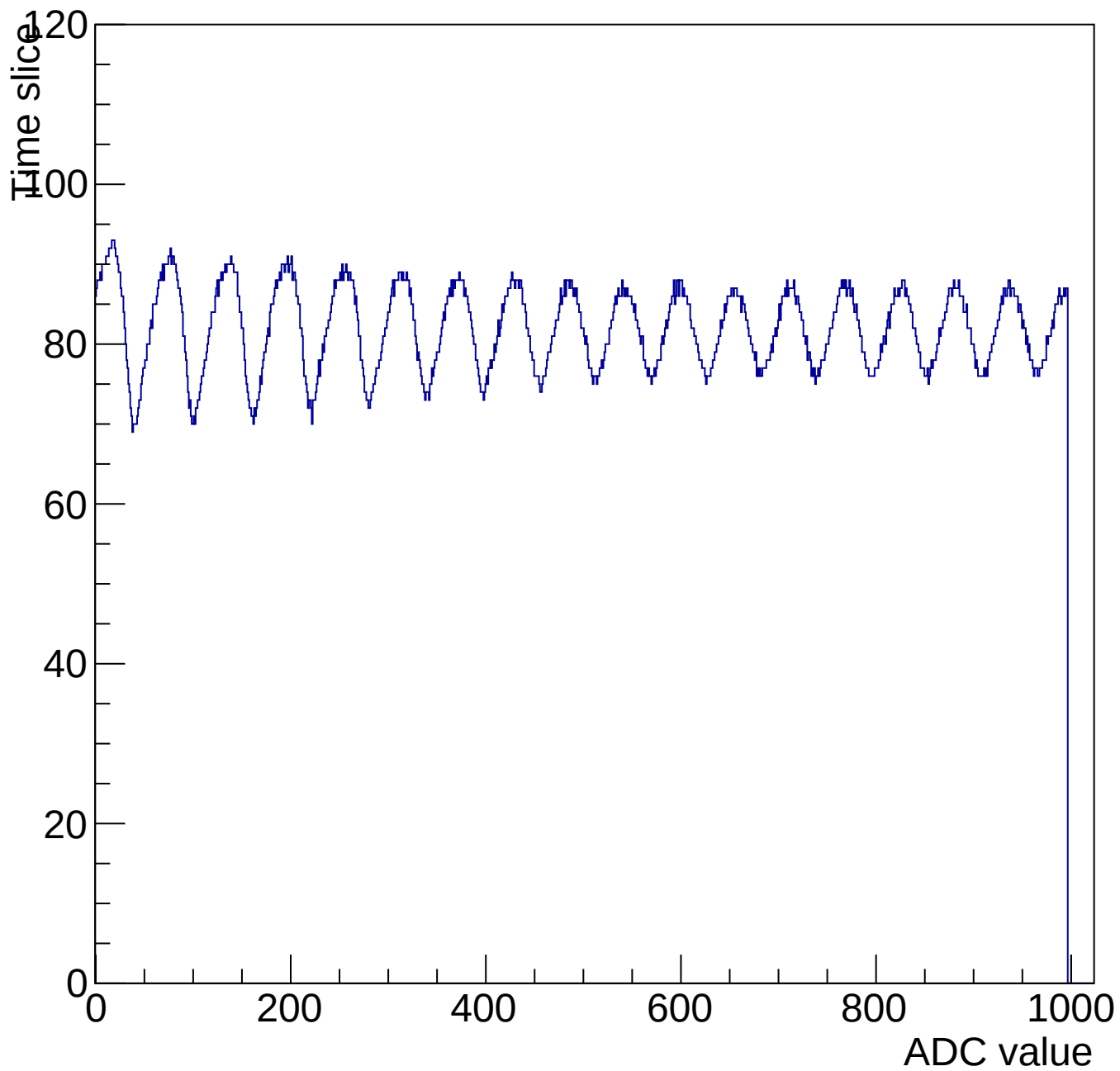
Evt 10 Time mcm 3006 chip 6 chan 14 1000-shift-gain0-shaper7
