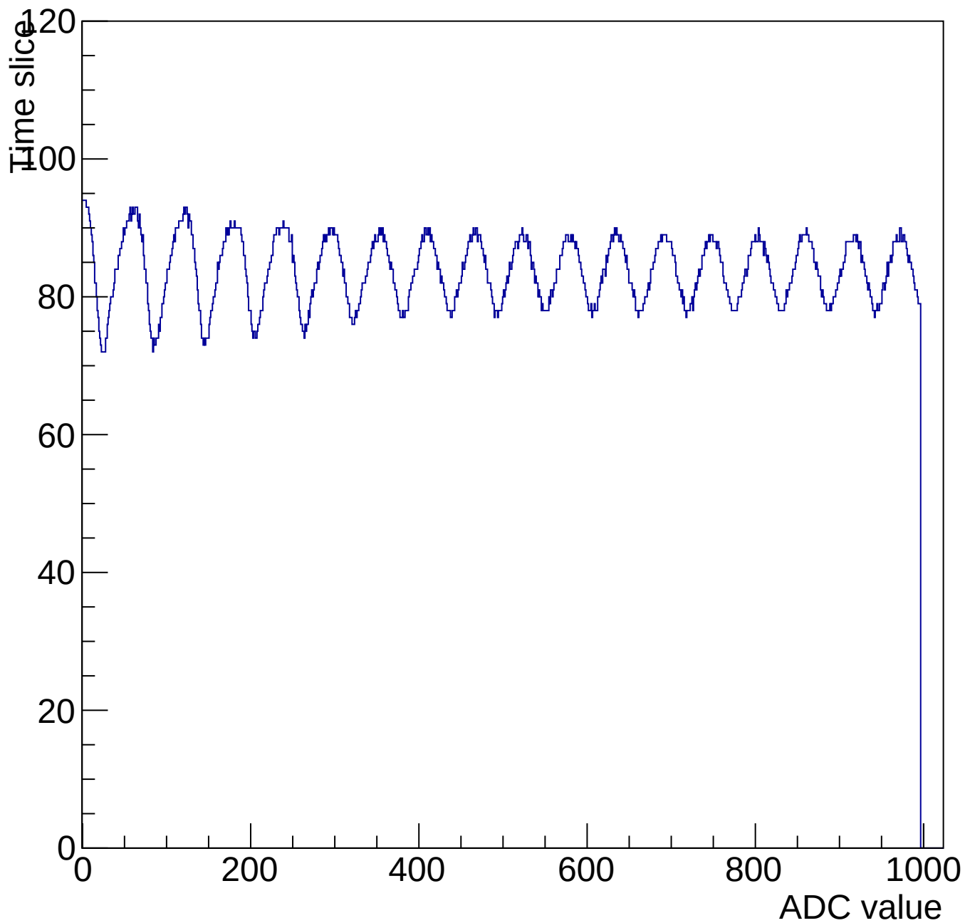
Evt 10 Time mcm 3006 chip 6 chan 13 1000-shift-gain0-shaper7
