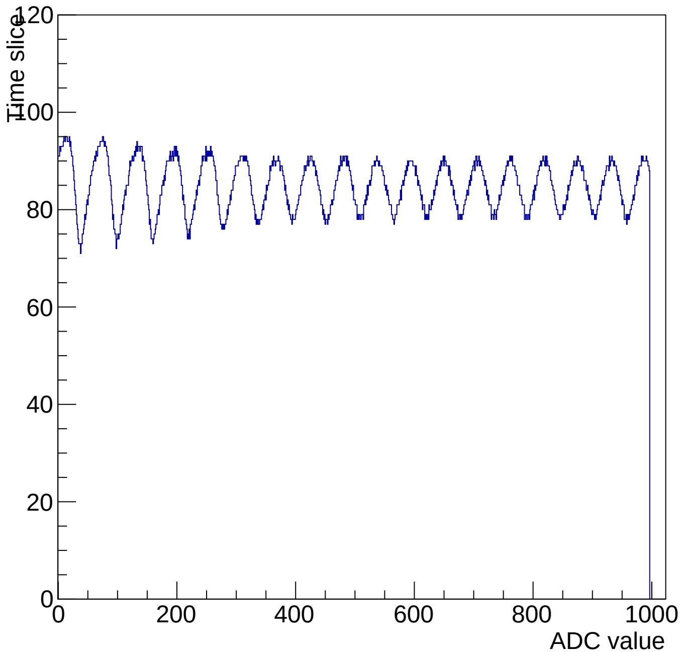
Evt 10 Time mcm 3006 chip 6 chan 4 1000-shift-gain0-shaper7
