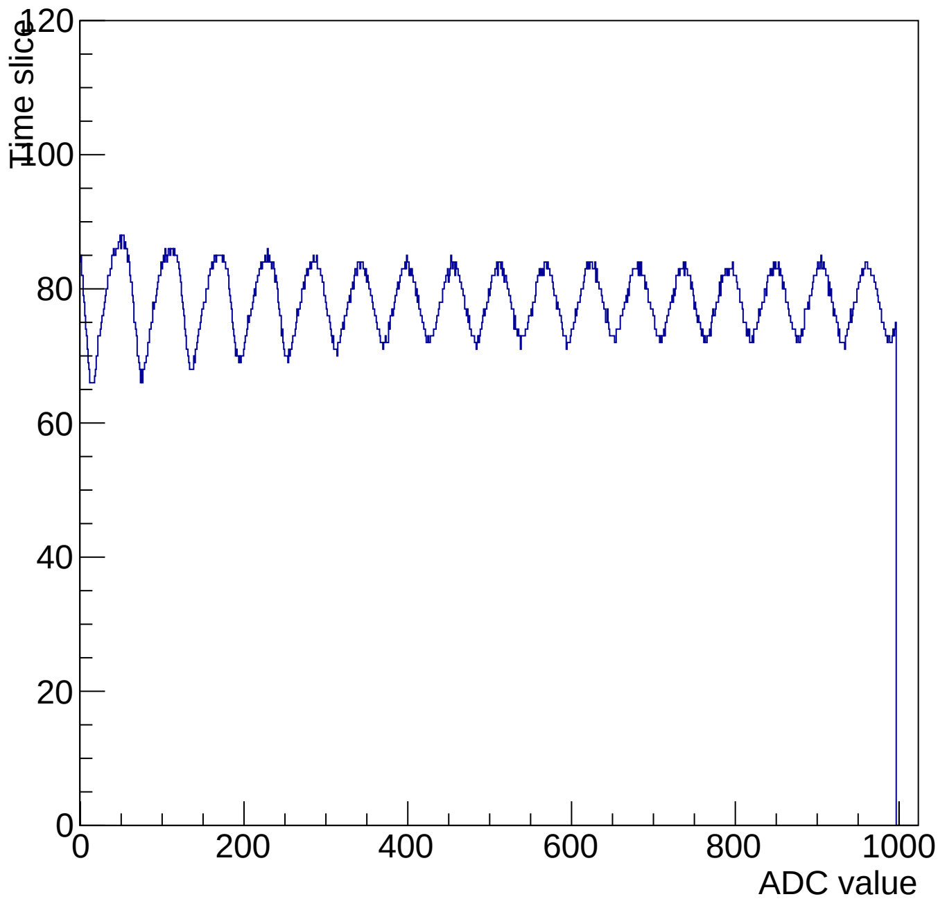
Evt 10 Time mcm 3006 chip 6 chan 7 1000-shift-gain0-shaper7
