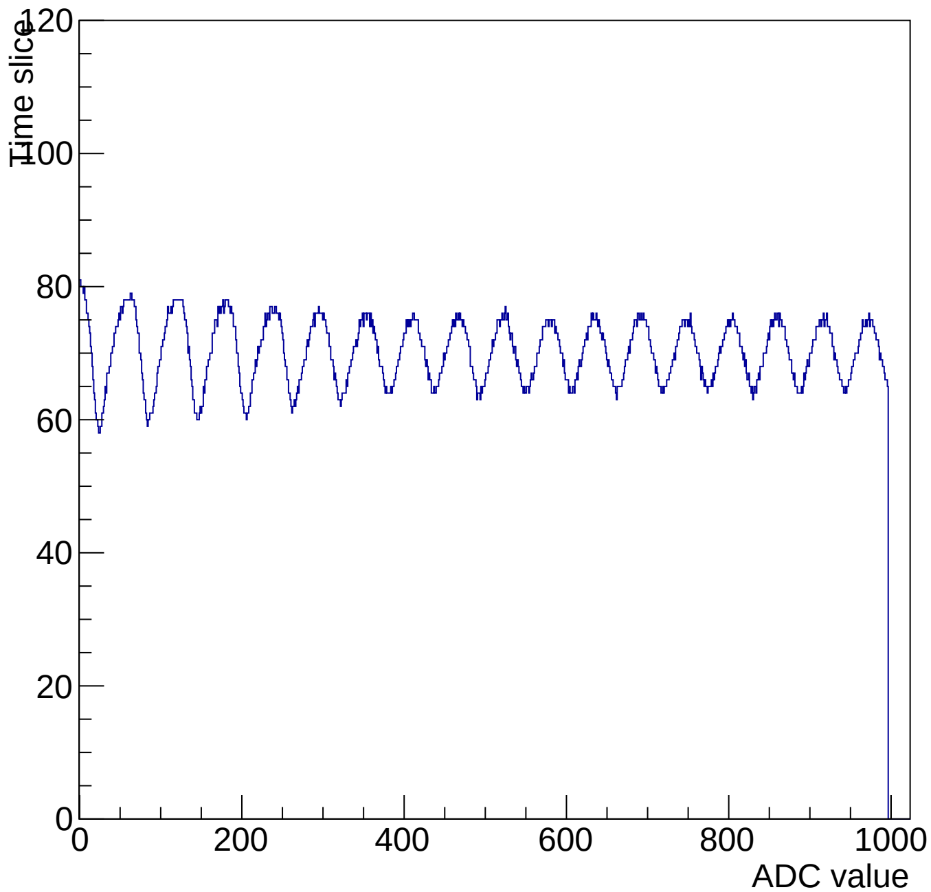
Evt 10 Time mcm 3006 chip 6 chan 12 1000-shift-gain0-shaper7
