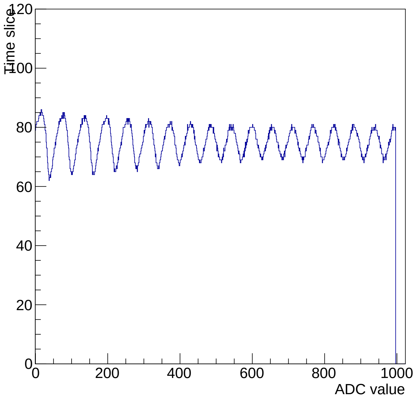
Evt 10 Time mcm 3006 chip 6 chan 15 1000-shift-gain0-shaper7
