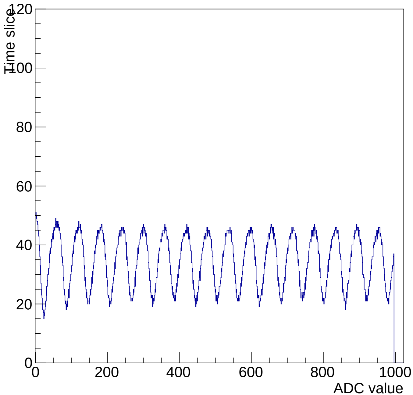
Evt 10 Time mcm 3006 chip 6 chan 3 1000-shift-gain3-shaper7
