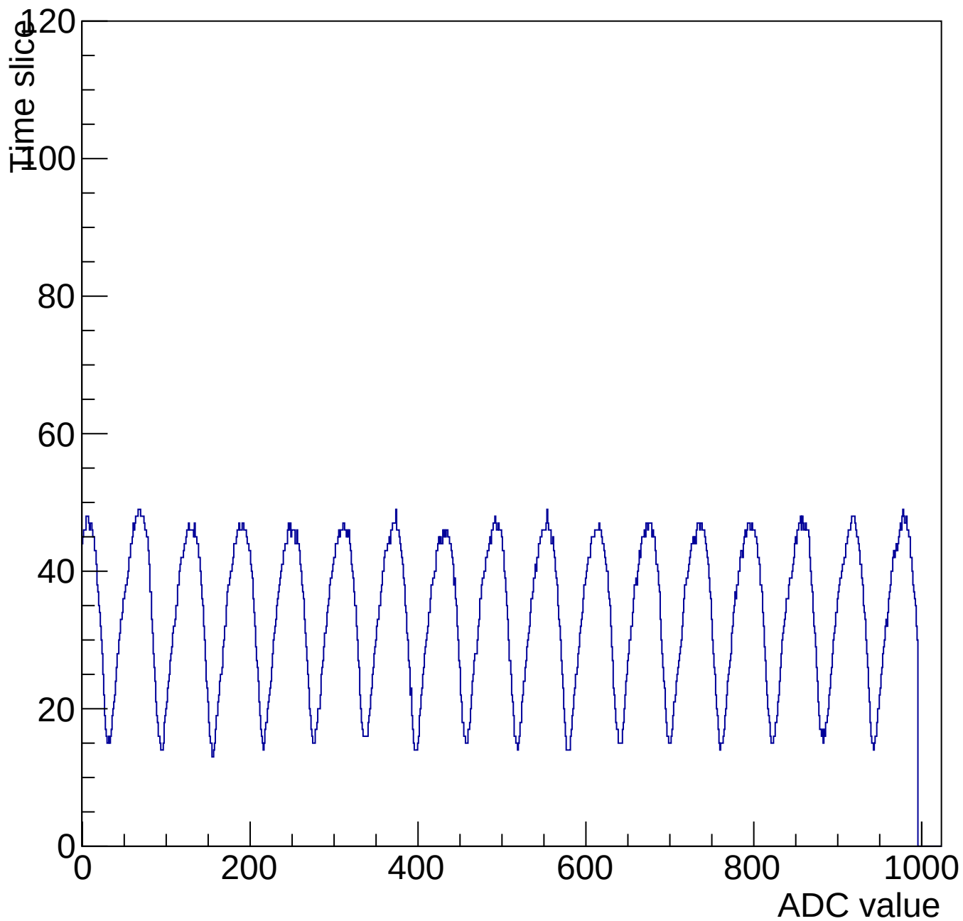
Evt 10 Time mcm 3007 chip 7 chan 5 1000-shift-gain3-shaper0
