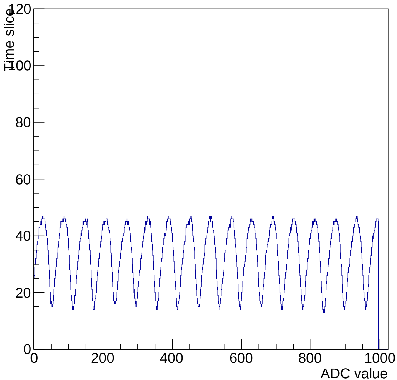
Evt 10 Time mcm 3007 chip 7 chan 13 1000-shift-gain3-shaper0
