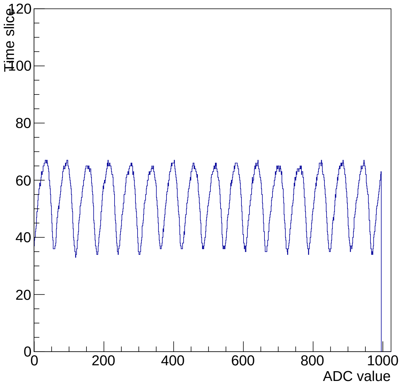
Evt 10 Time mcm 3007 chip 7 chan 15 1000-shift-gain3-shaper0
