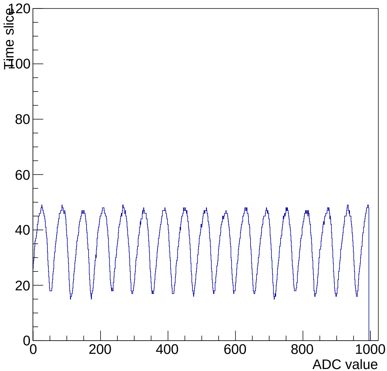
Evt 10 Time mcm 3007 chip 7 chan 12 1000-shift-gain3-shaper0
