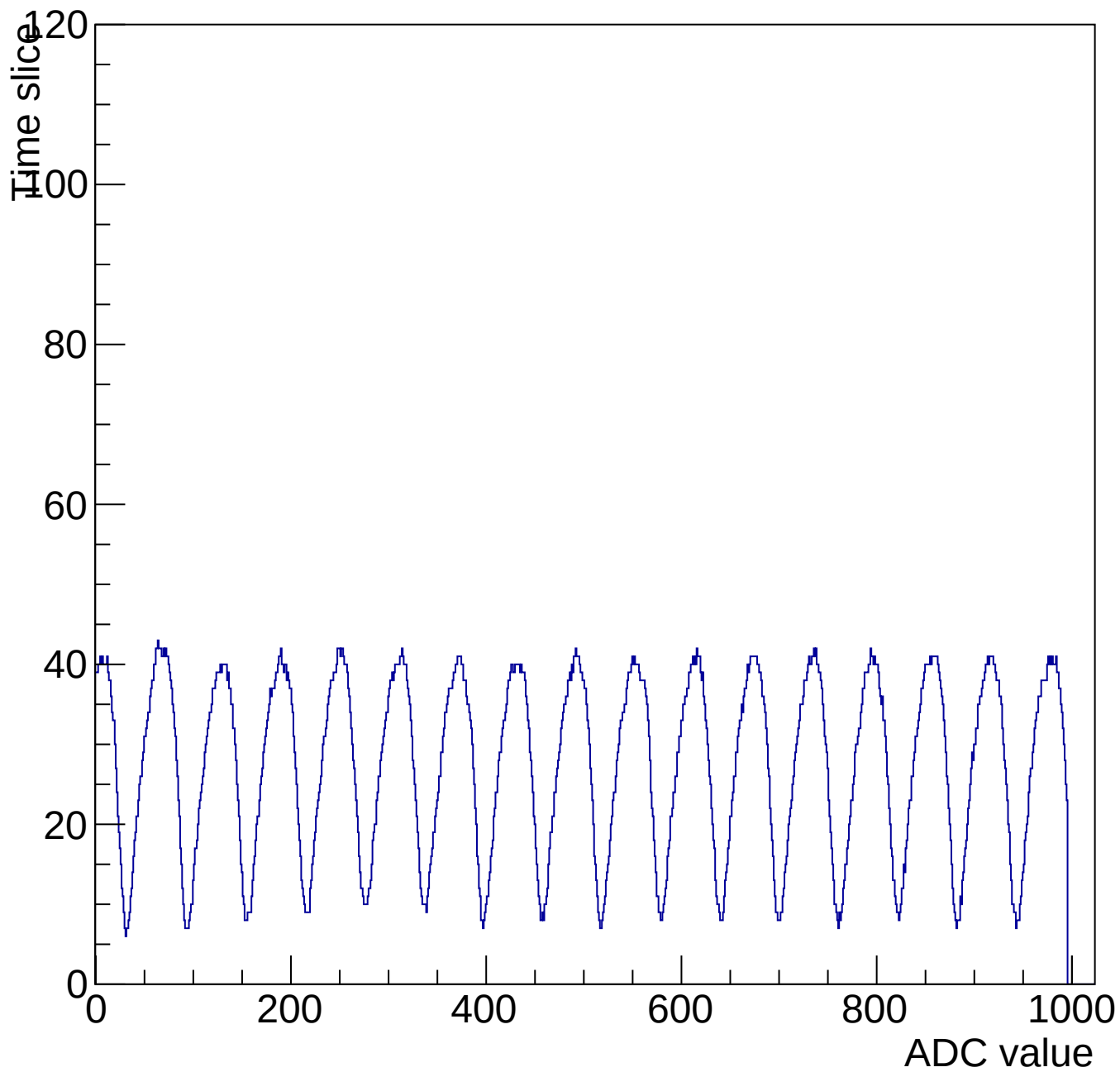
Evt 10 Time mcm 3007 chip 7 chan 4 1000-shift-gain3-shaper0
