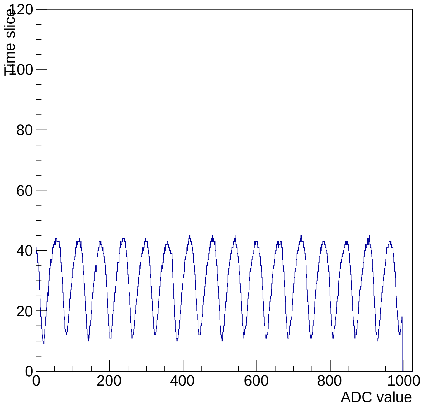
Evt 10 Time mcm 3007 chip 7 chan 2 1000-shift-gain3-shaper0
