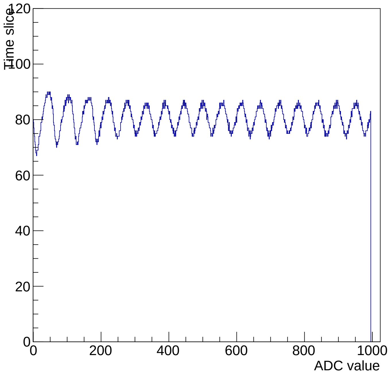
Evt 10 Time mcm 3007 chip 7 chan 7 1000-shift-gain0-shaper7
