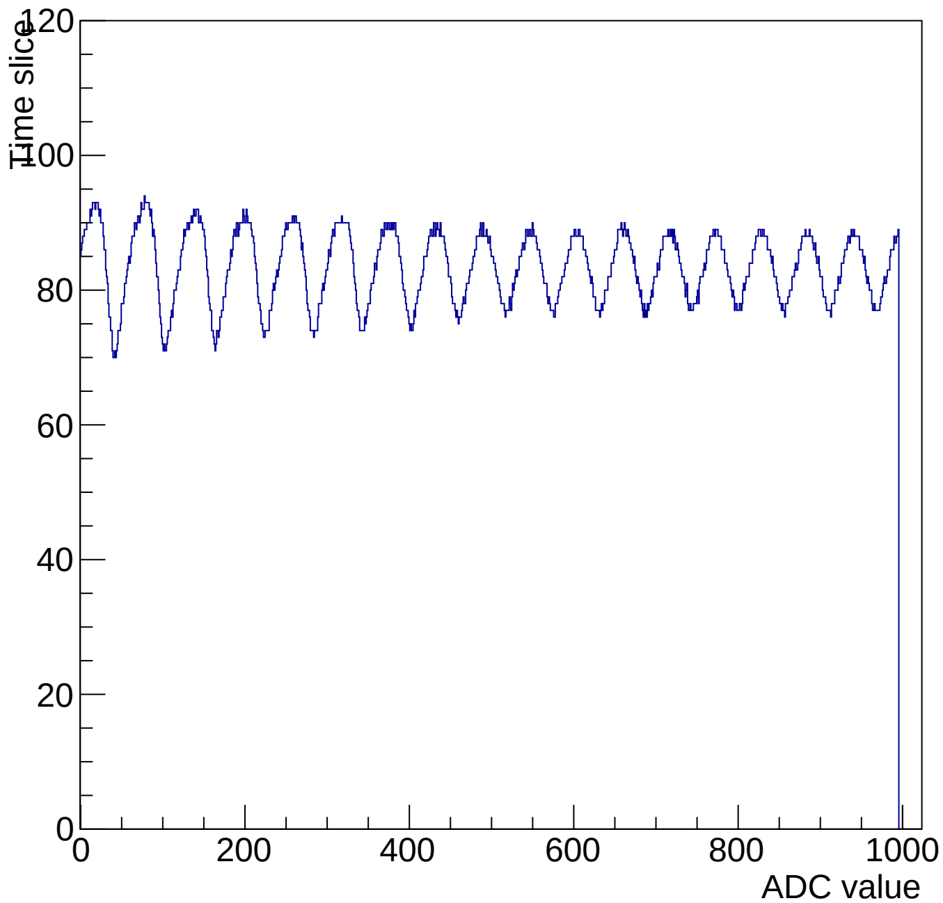
Evt 10 Time mcm 3007 chip 7 chan 11 1000-shift-gain0-shaper7
