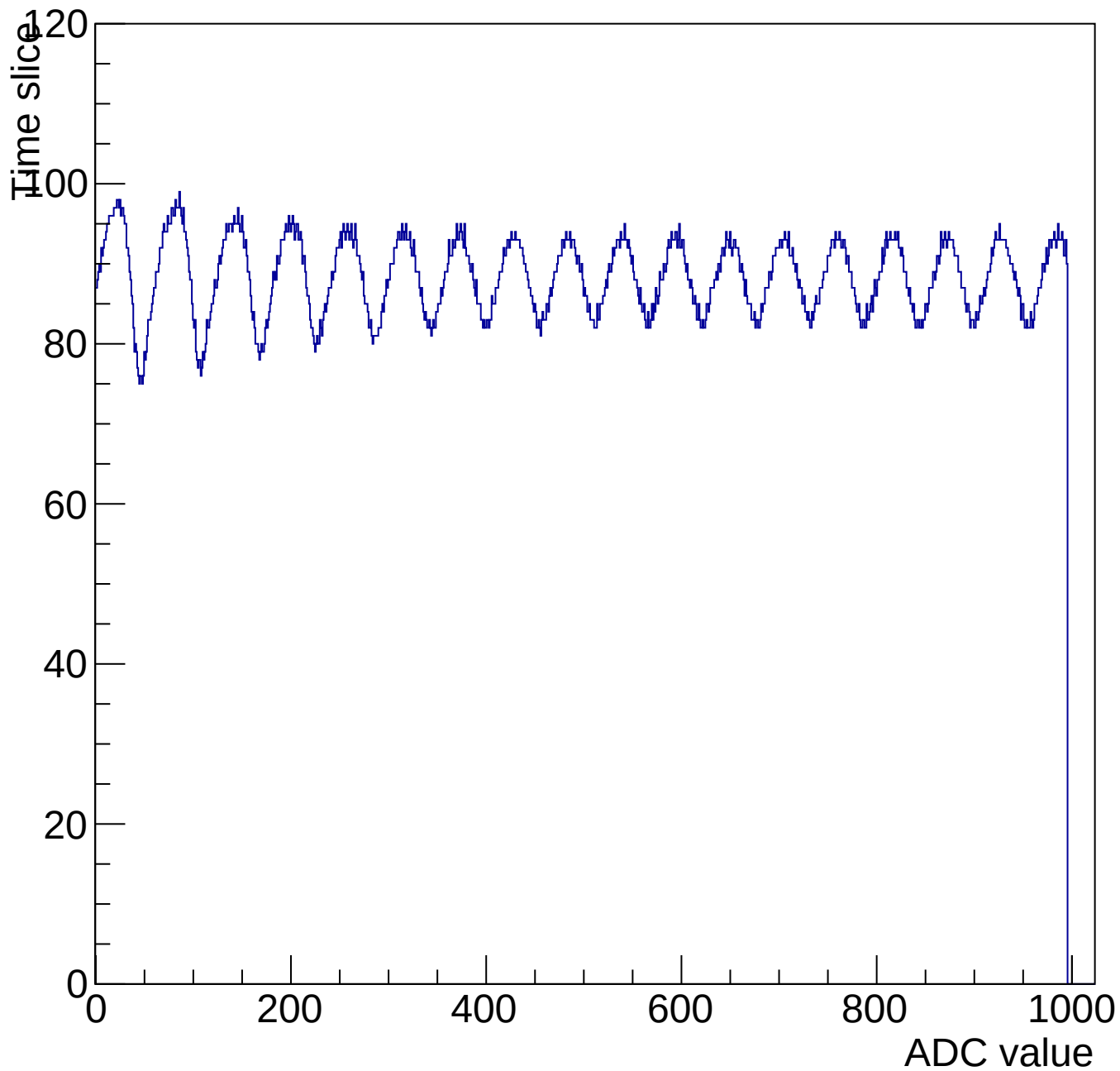
Evt 10 Time mcm 3007 chip 7 chan 3 1000-shift-gain0-shaper7
