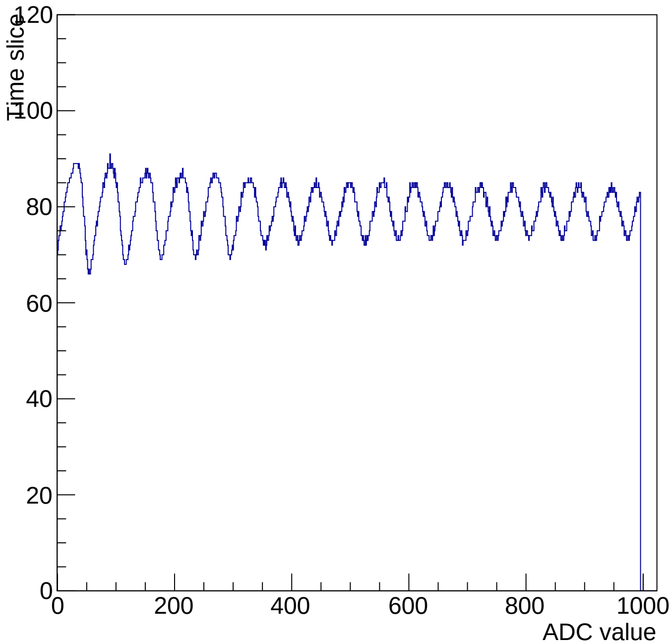
Evt 10 Time mcm 3007 chip 7 chan 12 1000-shift-gain0-shaper7
