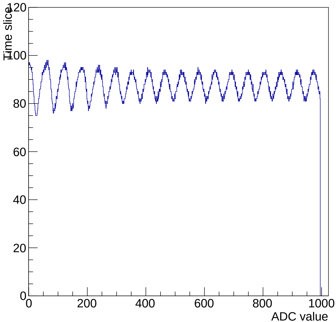
Evt 10 Time mcm 3007 chip 7 chan 1 1000-shift-gain0-shaper7
