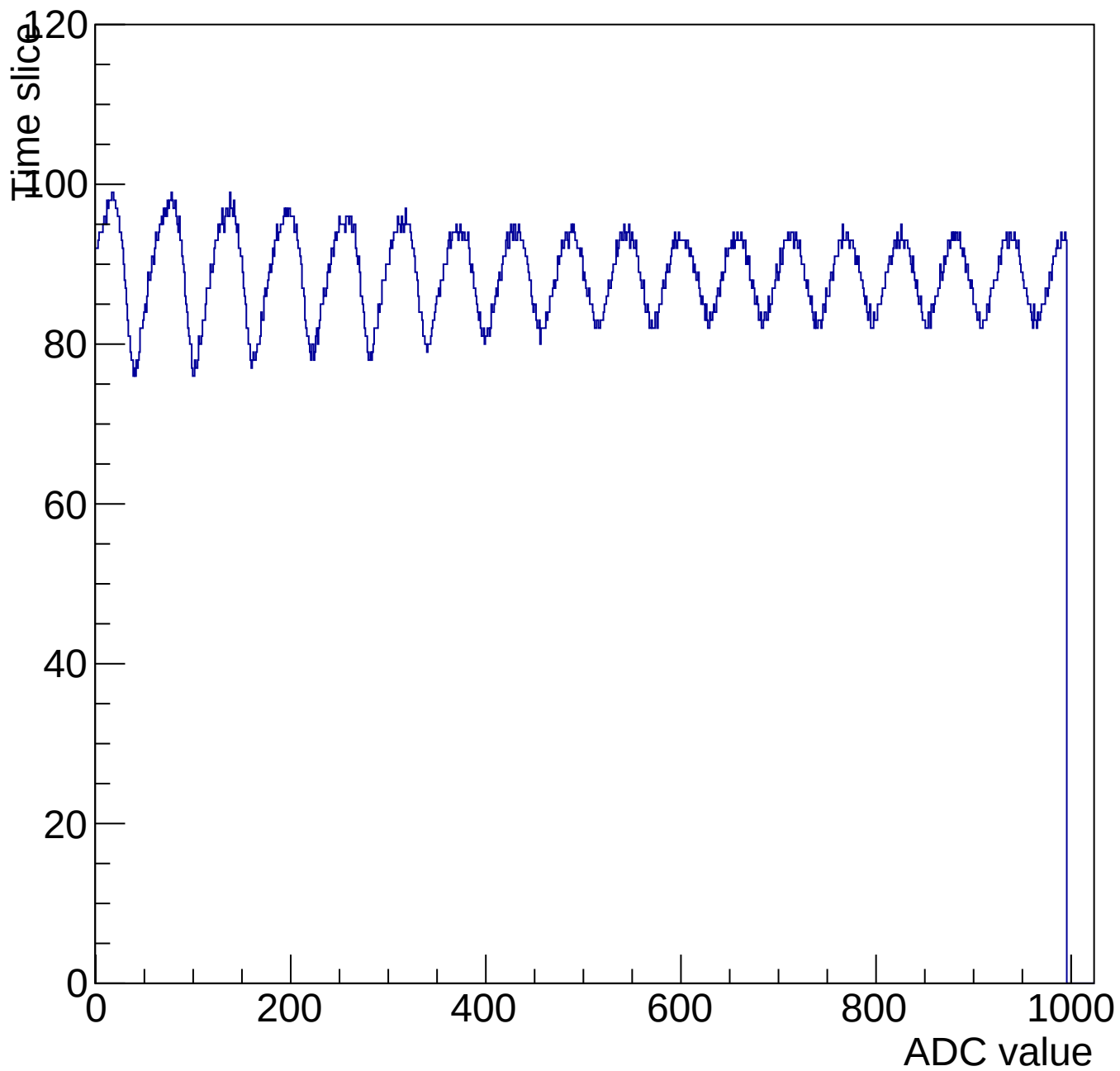
Evt 10 Time mcm 3007 chip 7 chan 15 1000-shift-gain0-shaper7
