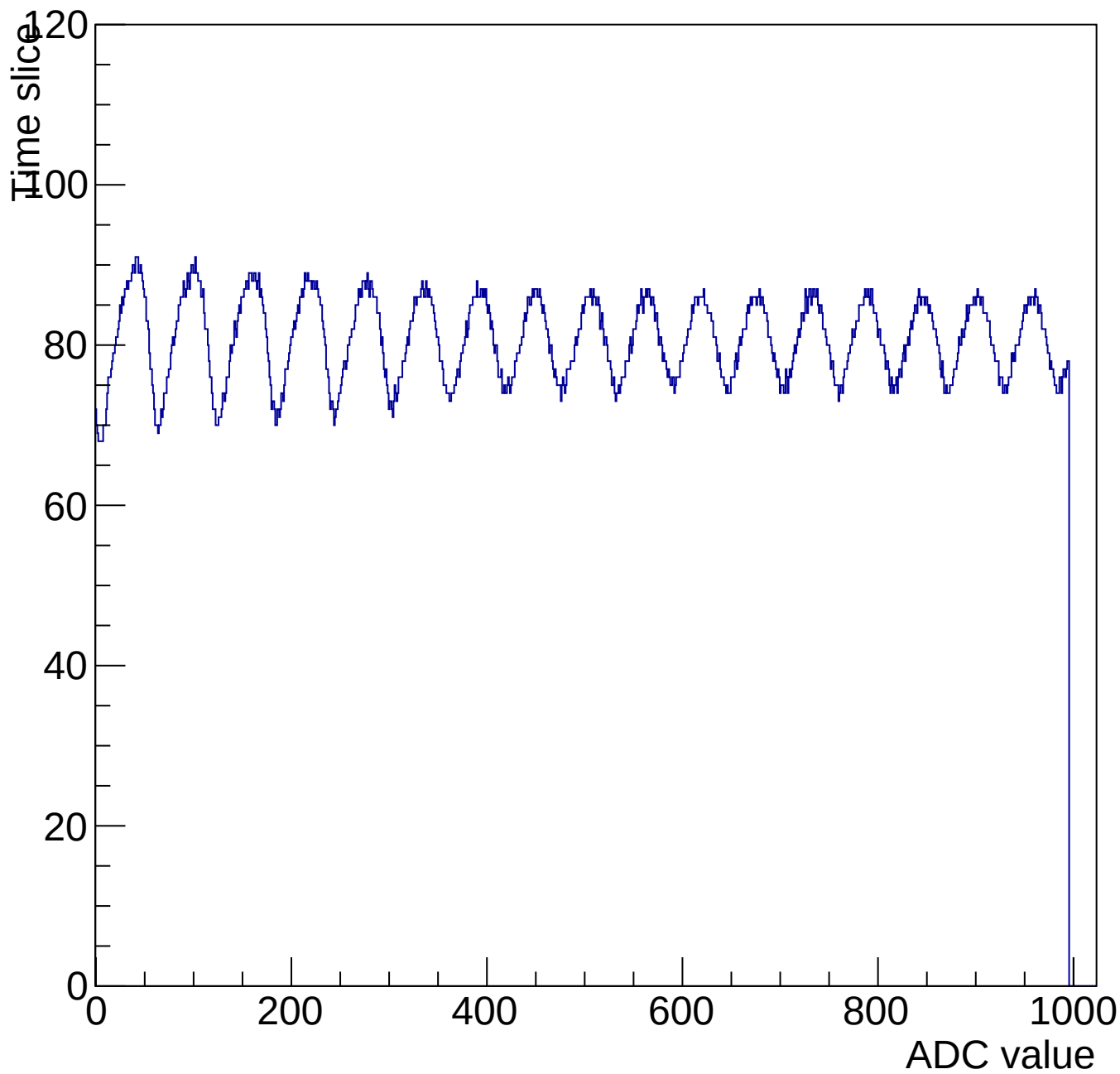
Evt 10 Time mcm 3007 chip 7 chan 5 1000-shift-gain0-shaper7
