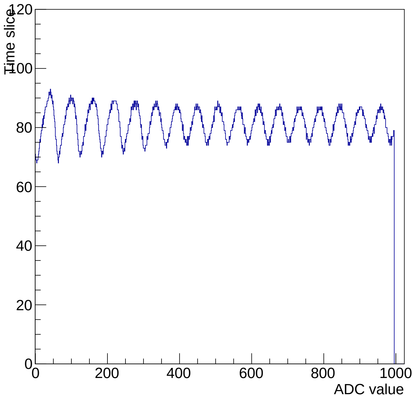
Evt 10 Time mcm 3007 chip 7 chan 4 1000-shift-gain0-shaper7
