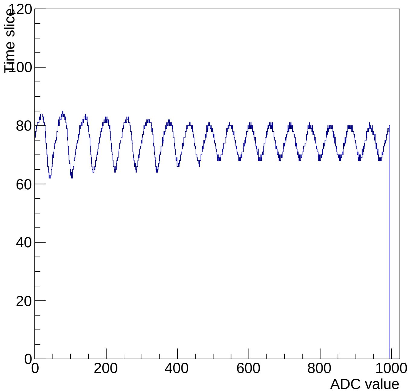
Evt 10 Time mcm 3007 chip 7 chan 10 1000-shift-gain0-shaper7
