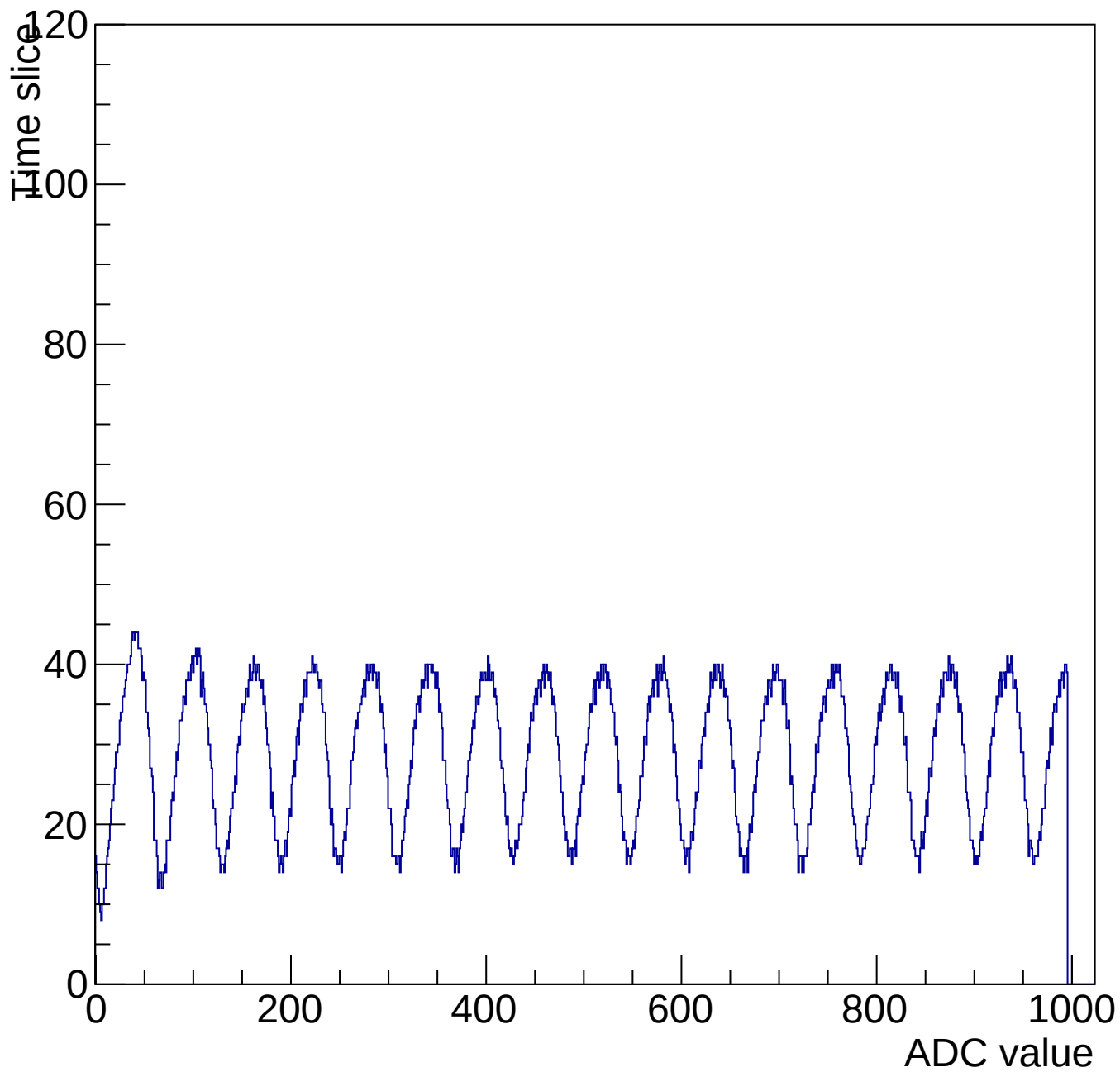
Evt 10 Time mcm 3007 chip 7 chan 10 1000-shift-gain3-shaper7
