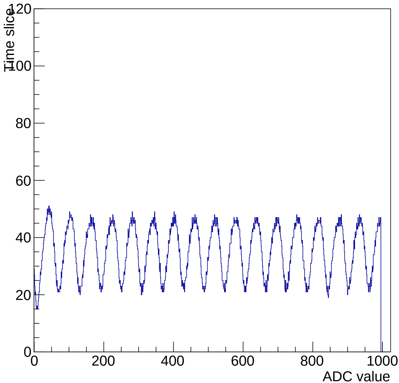
Evt 10 Time mcm 3007 chip 7 chan 2 1000-shift-gain3-shaper7
