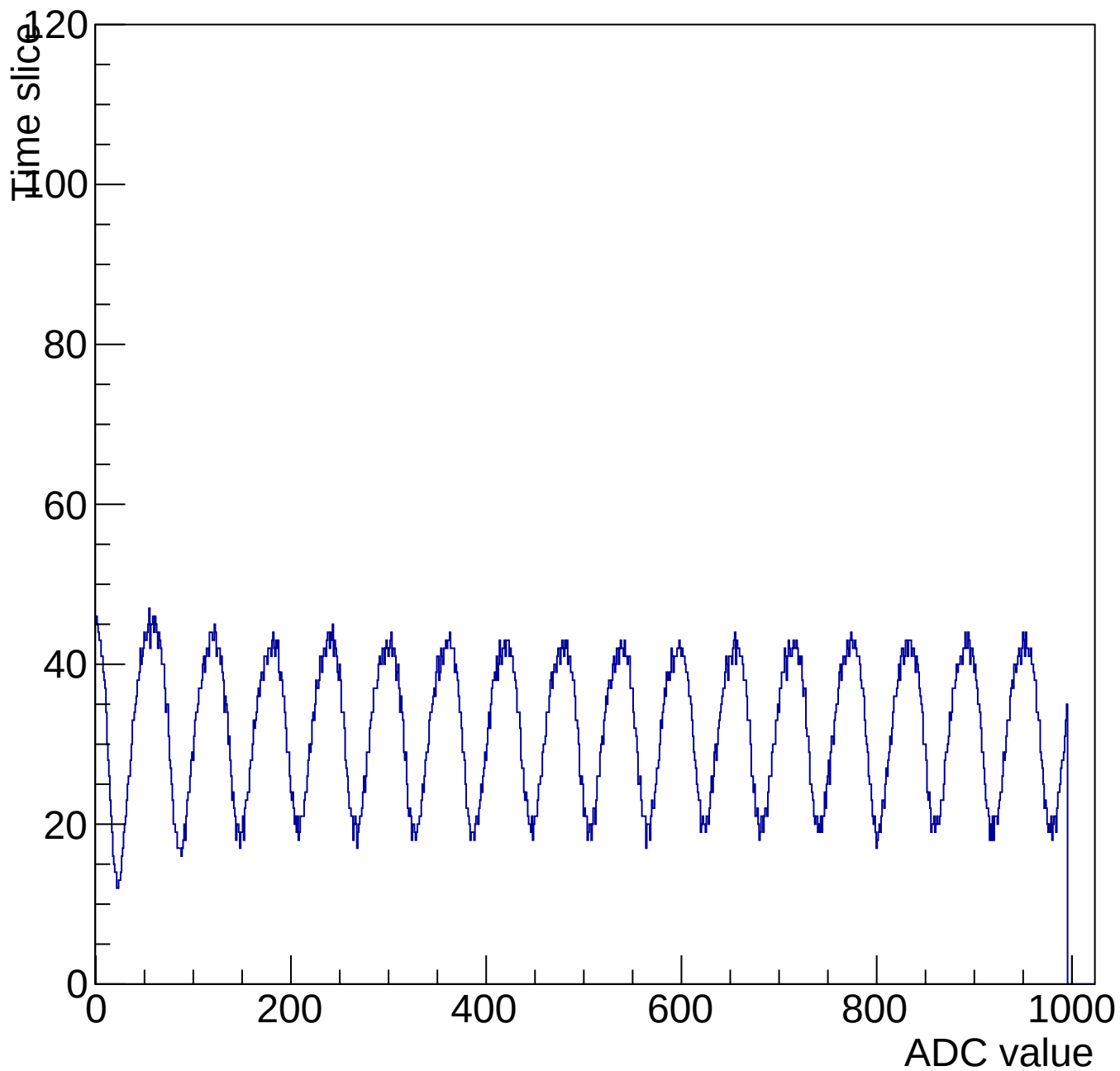
Evt 10 Time mcm 3007 chip 7 chan 9 1000-shift-gain3-shaper7
