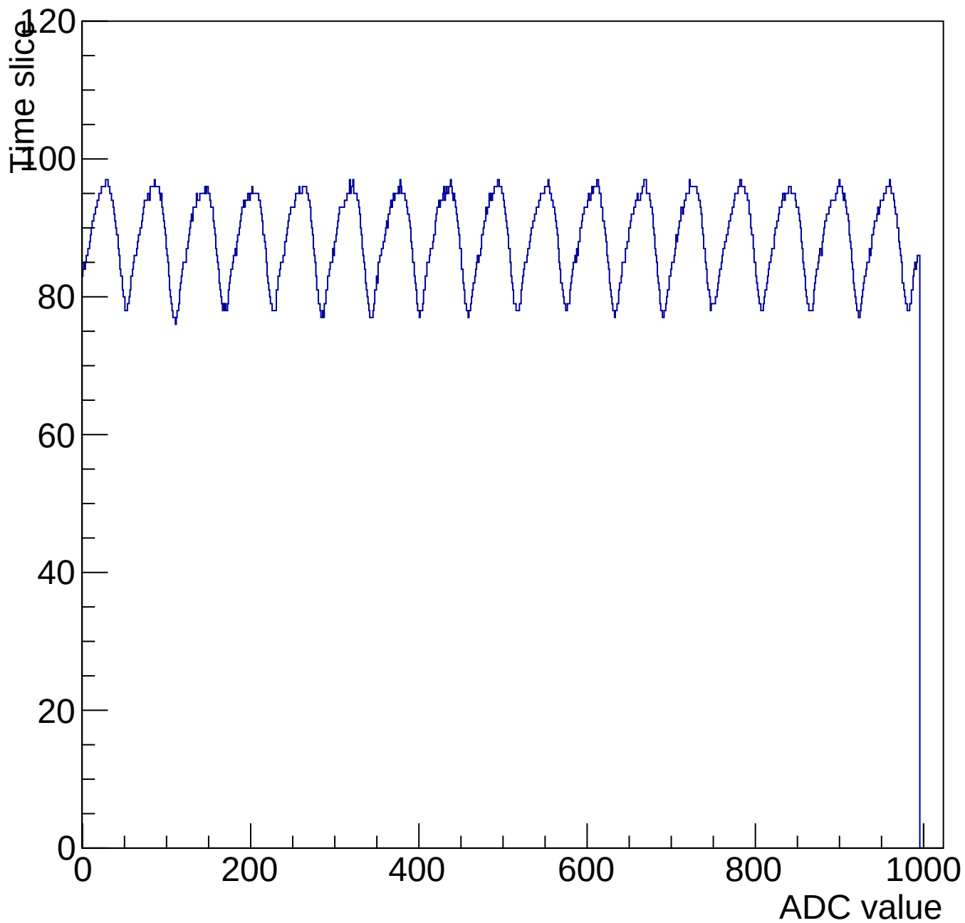
Evt 10 Time mcm 3007 chip 7 chan 6 1000-shift-gain0-shaper0
