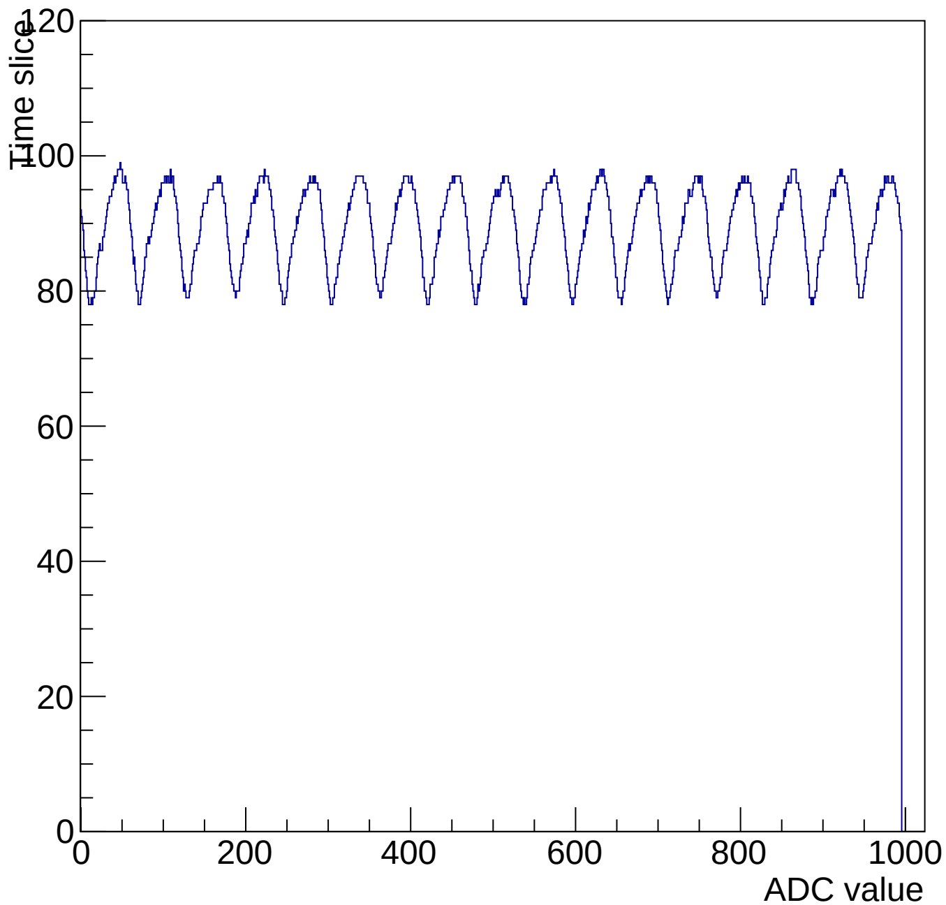
Evt 10 Time mcm 3007 chip 7 chan 15 1000-shift-gain0-shaper0
