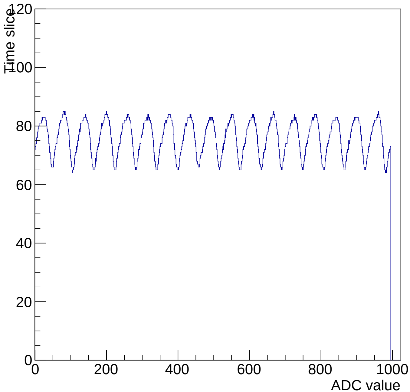
Evt 10 Time mcm 3007 chip 7 chan 9 1000-shift-gain0-shaper0
