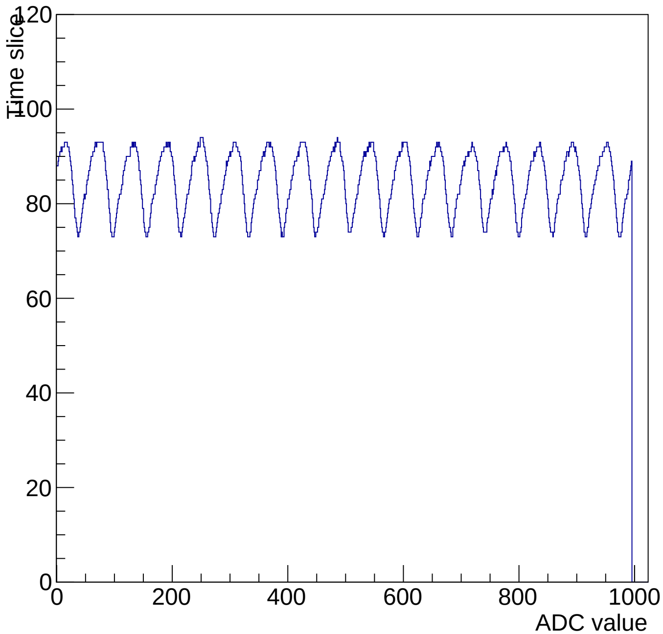
Evt 10 Time mcm 3007 chip 7 chan 1 1000-shift-gain0-shaper0
