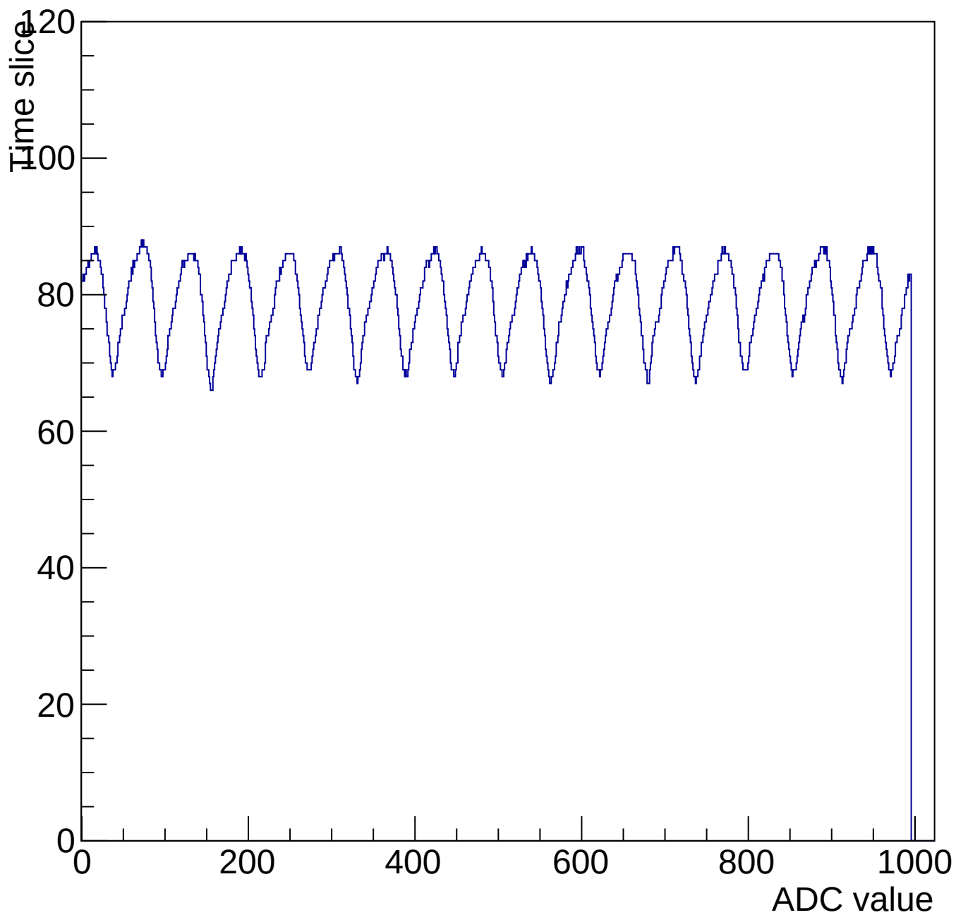
Evt 10 Time mcm 3007 chip 7 chan 12 1000-shift-gain0-shaper0
