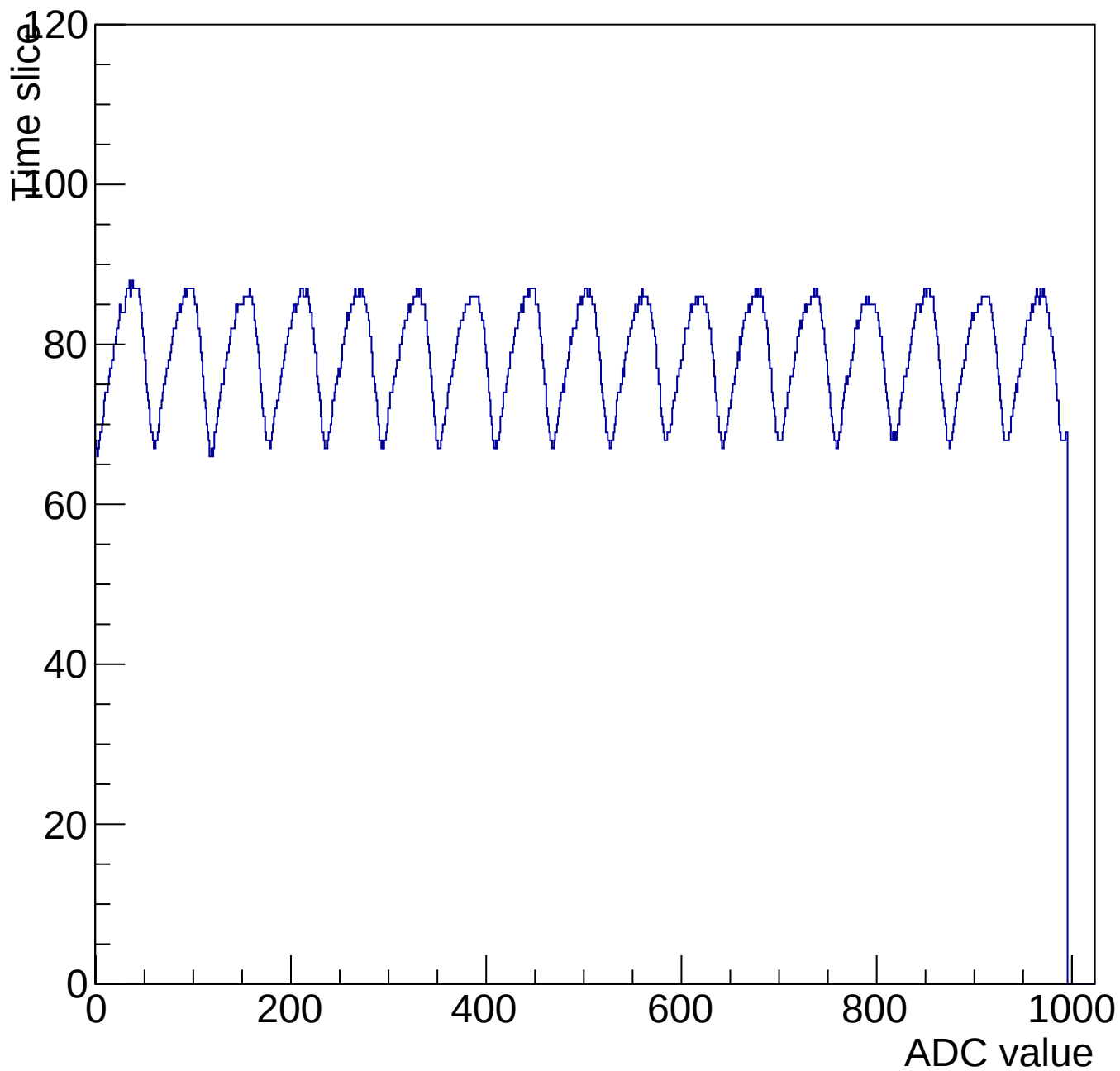
Evt 10 Time mcm 3007 chip 7 chan 4 1000-shift-gain0-shaper0
