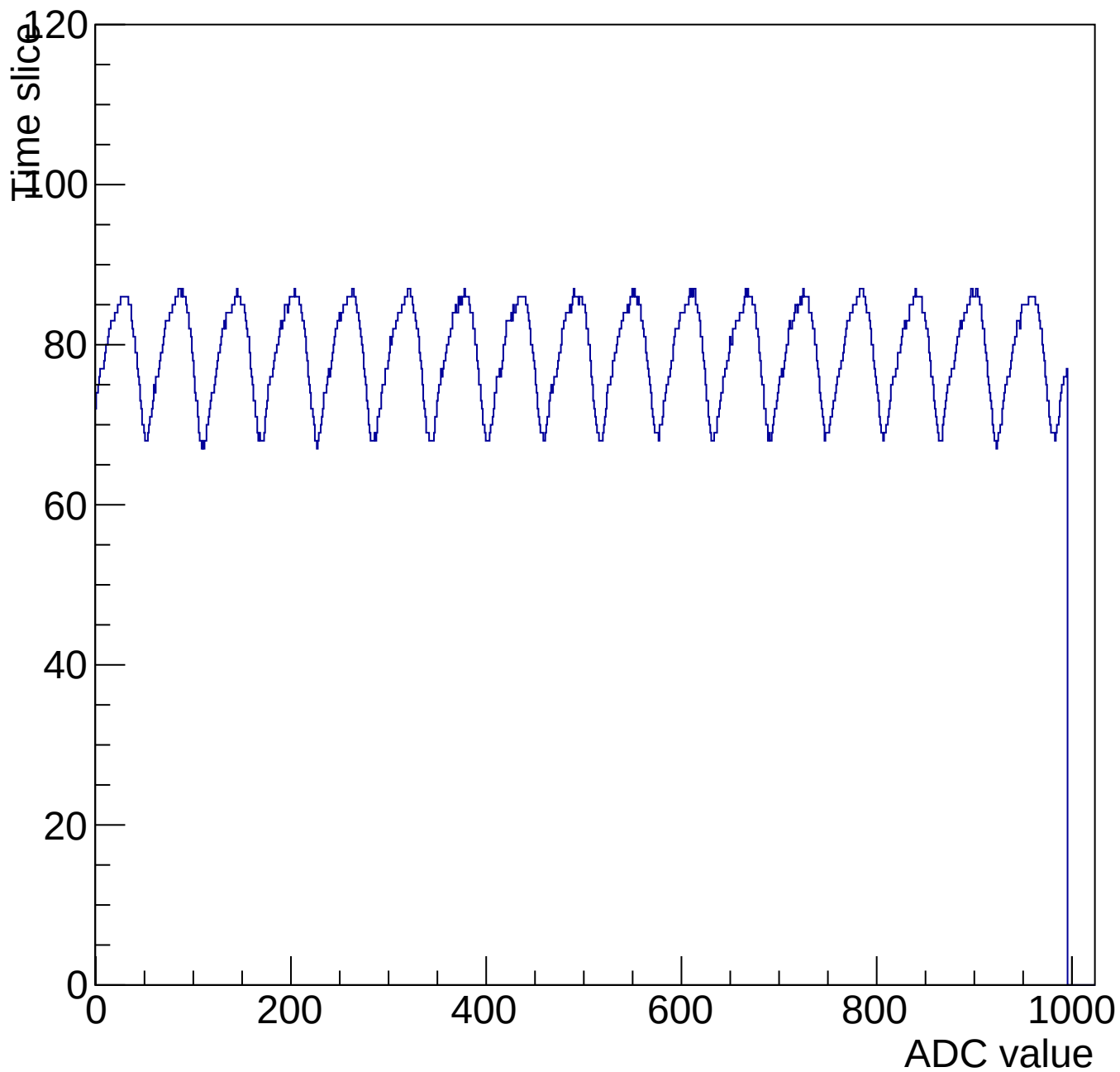
Evt 10 Time mcm 3007 chip 7 chan 7 1000-shift-gain0-shaper0
