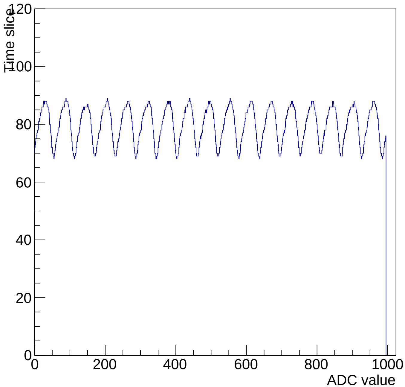
Evt 10 Time mcm 3007 chip 7 chan 11 1000-shift-gain0-shaper0
