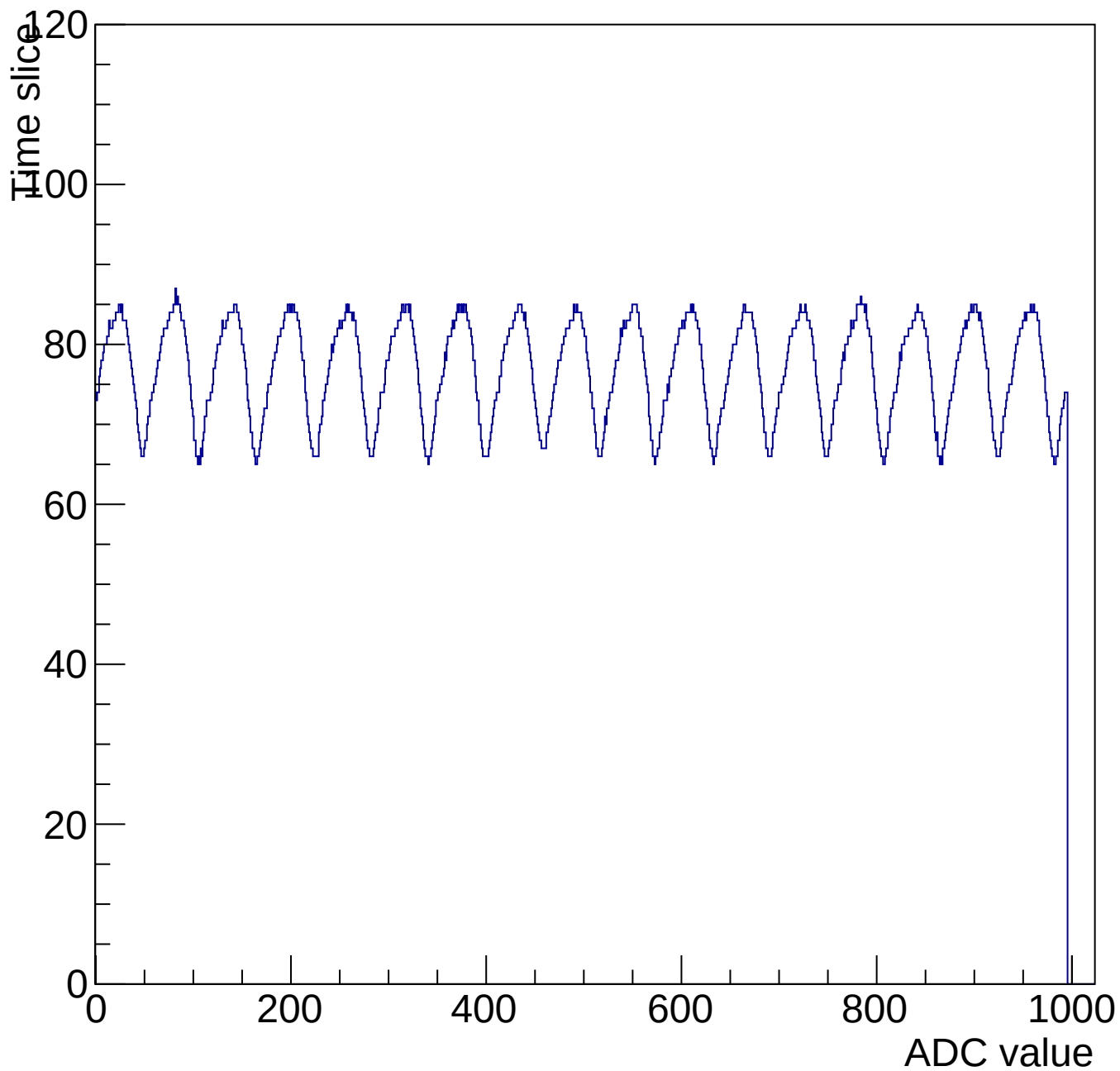
Evt 10 Time mcm 3007 chip 7 chan 8 1000-shift-gain0-shaper0
