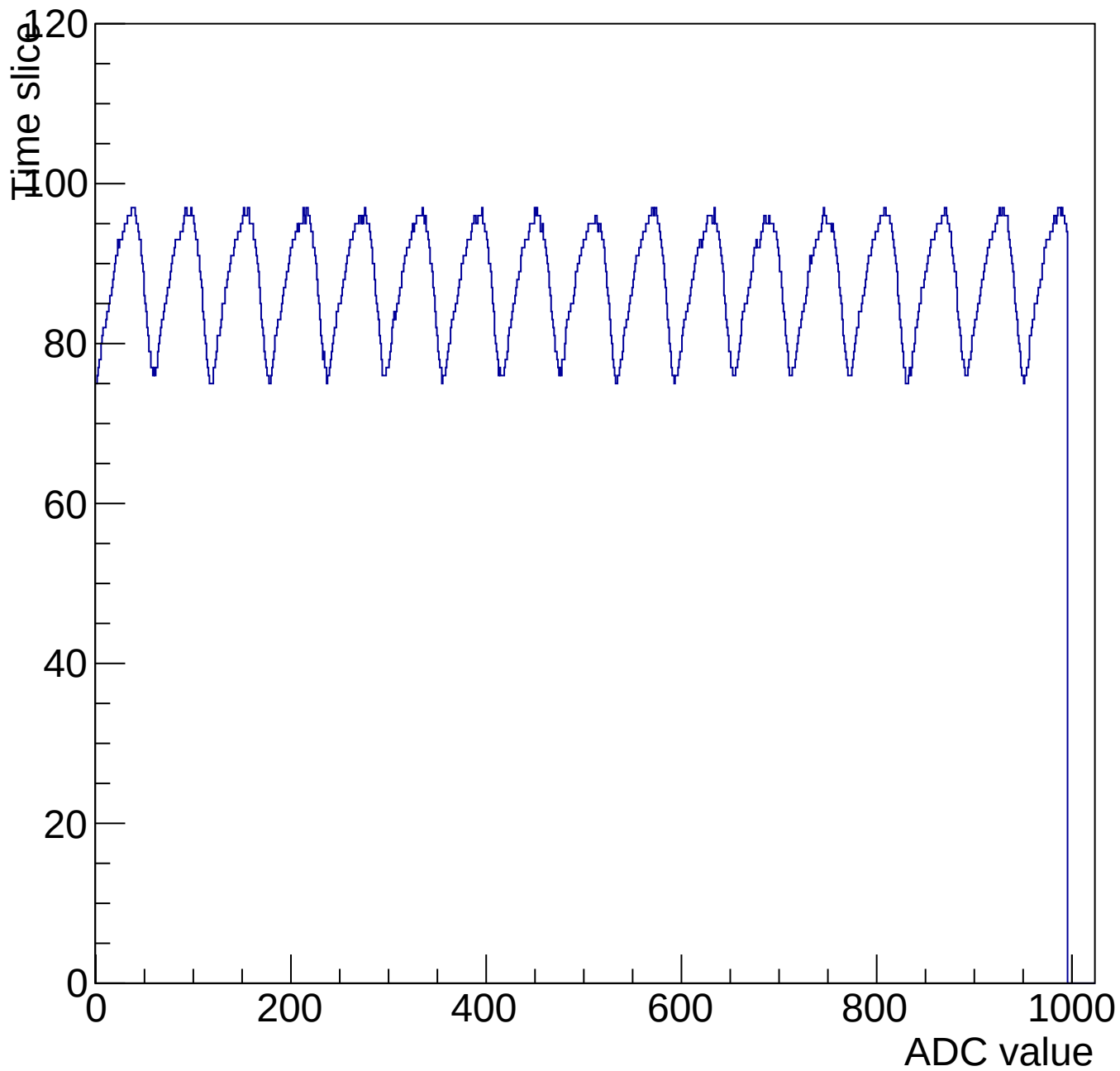
Evt 10 Time mcm 3007 chip 7 chan 6 1000-shift-gain0-shaper1
