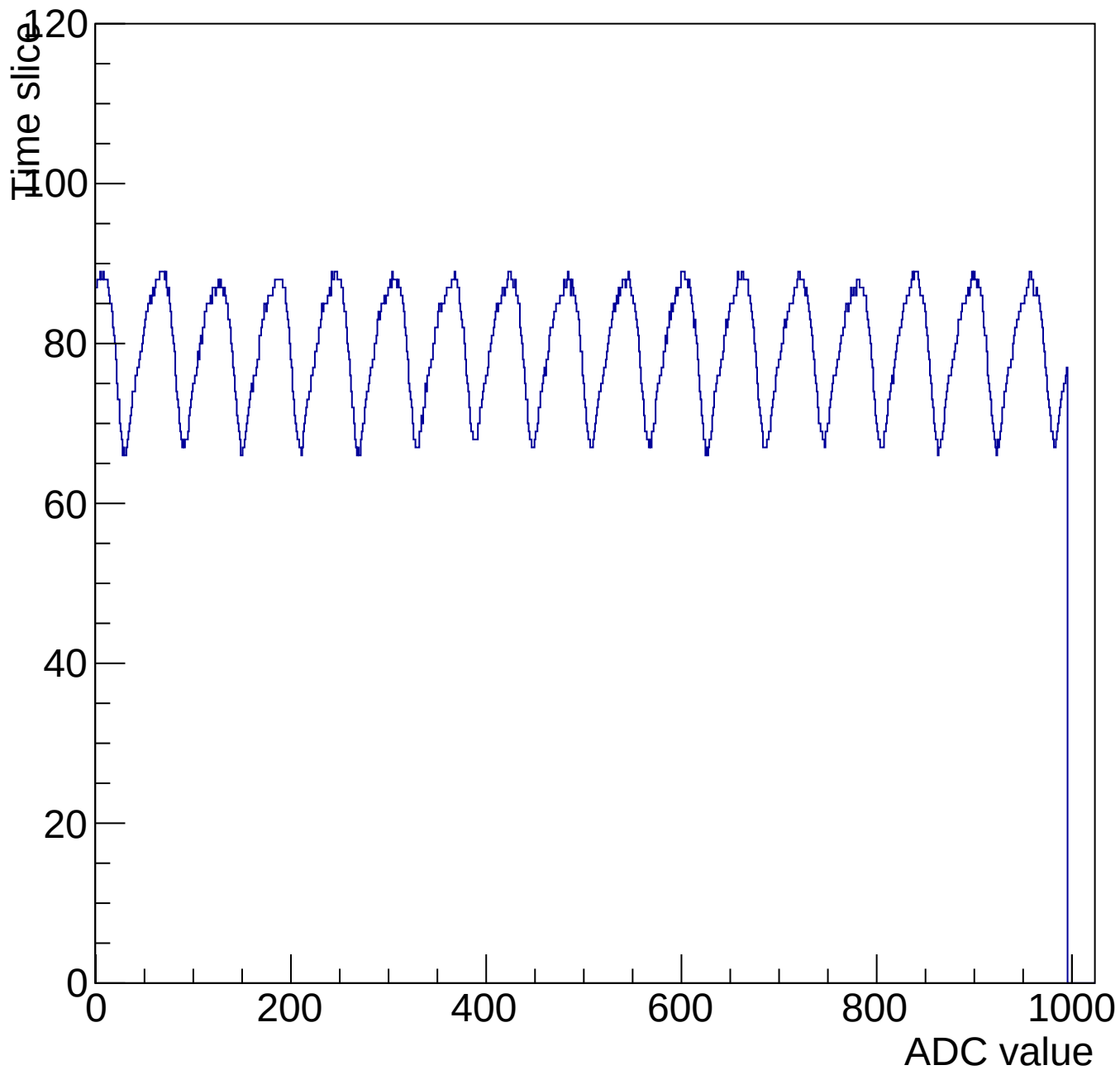
Evt 10 Time mcm 3007 chip 7 chan 4 1000-shift-gain0-shaper1
