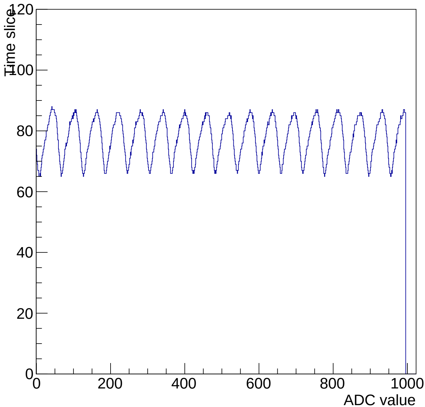
Evt 10 Time mcm 3007 chip 7 chan 8 1000-shift-gain0-shaper1
