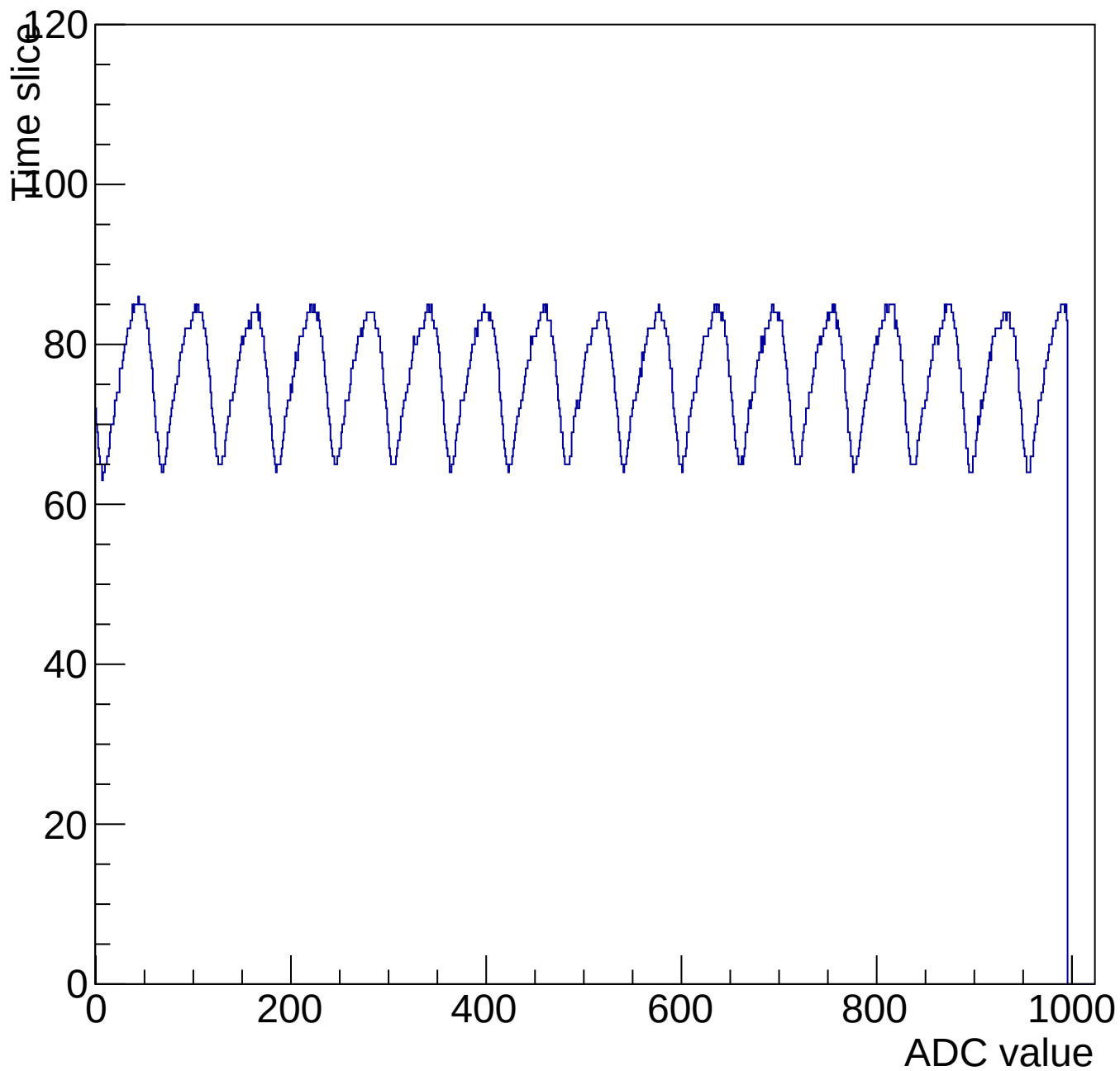
Evt 10 Time mcm 3007 chip 7 chan 9 1000-shift-gain0-shaper1
