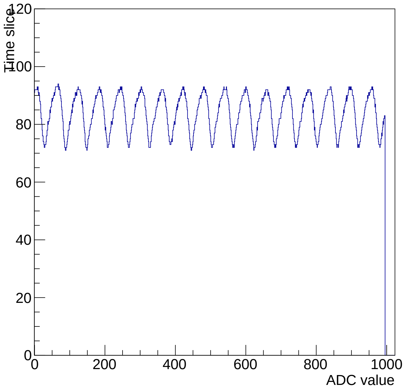
Evt 10 Time mcm 3007 chip 7 chan 0 1000-shift-gain0-shaper1
