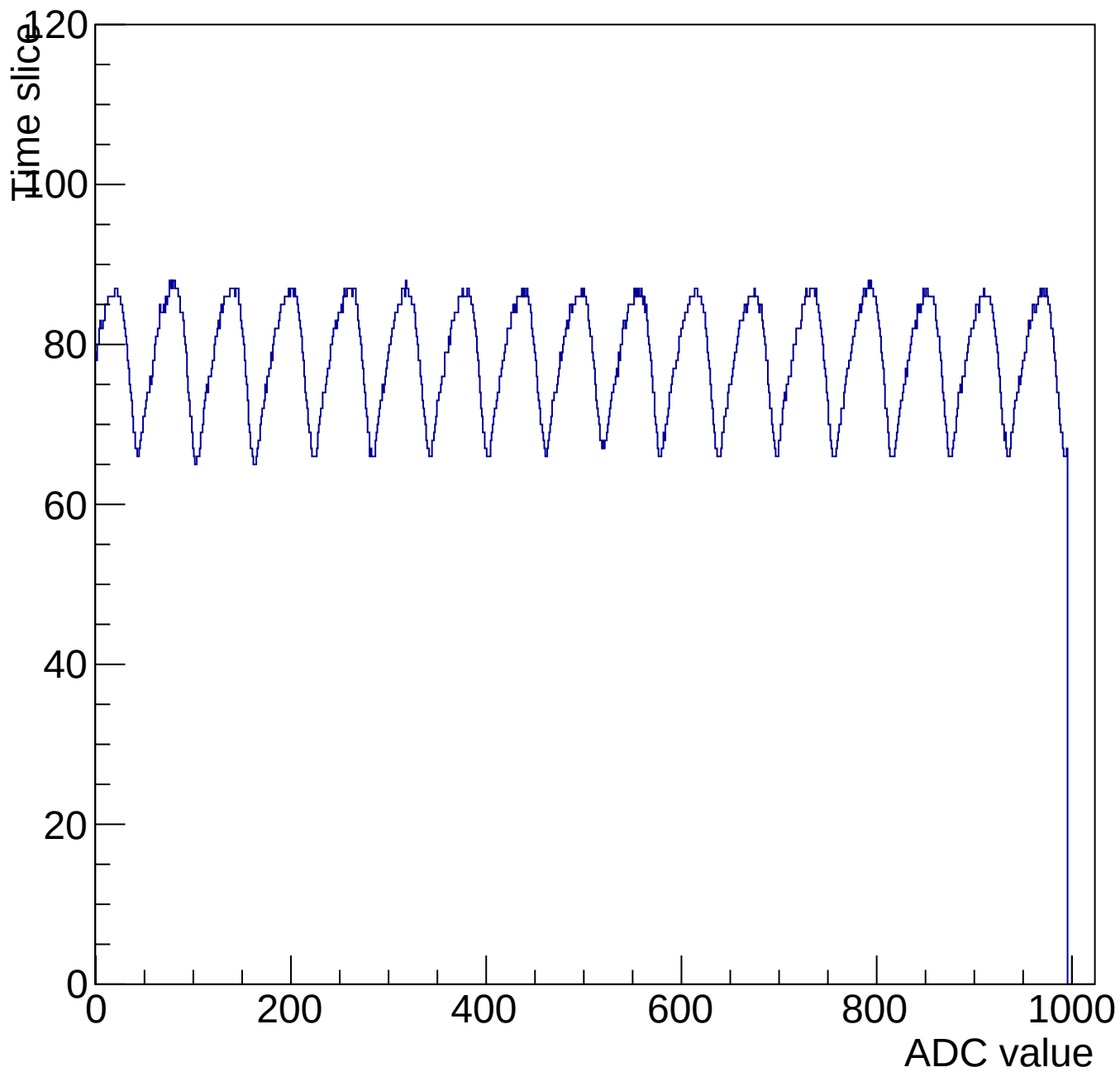
Evt 10 Time mcm 3007 chip 7 chan 14 1000-shift-gain0-shaper1
