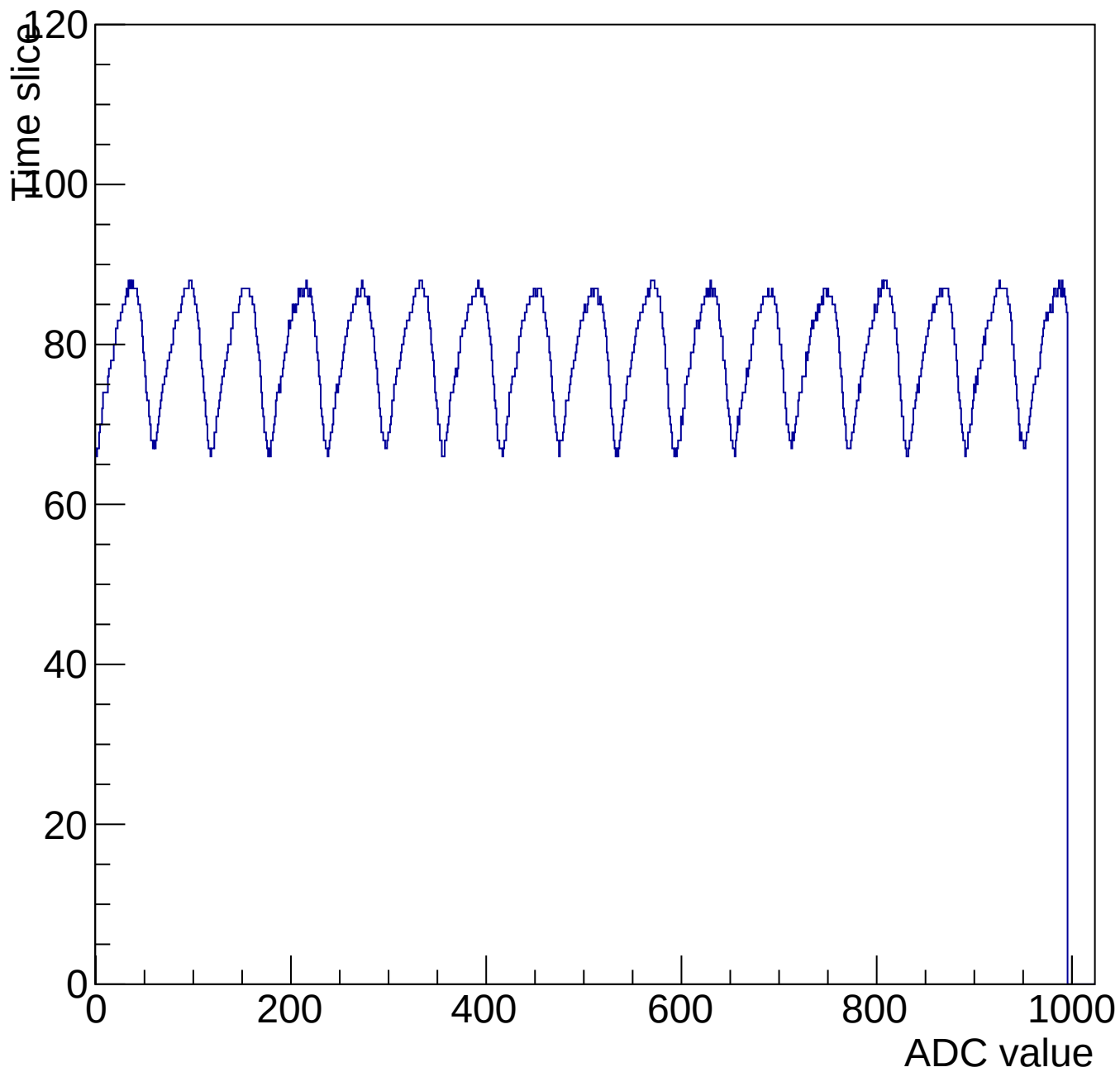
Evt 10 Time mcm 3007 chip 7 chan 7 1000-shift-gain0-shaper1
