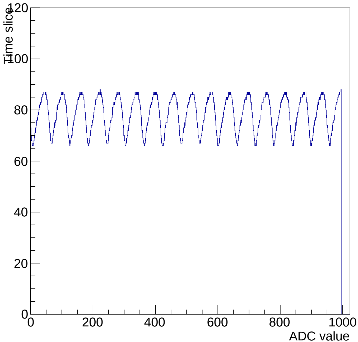
Evt 10 Time mcm 3007 chip 7 chan 13 1000-shift-gain0-shaper1
