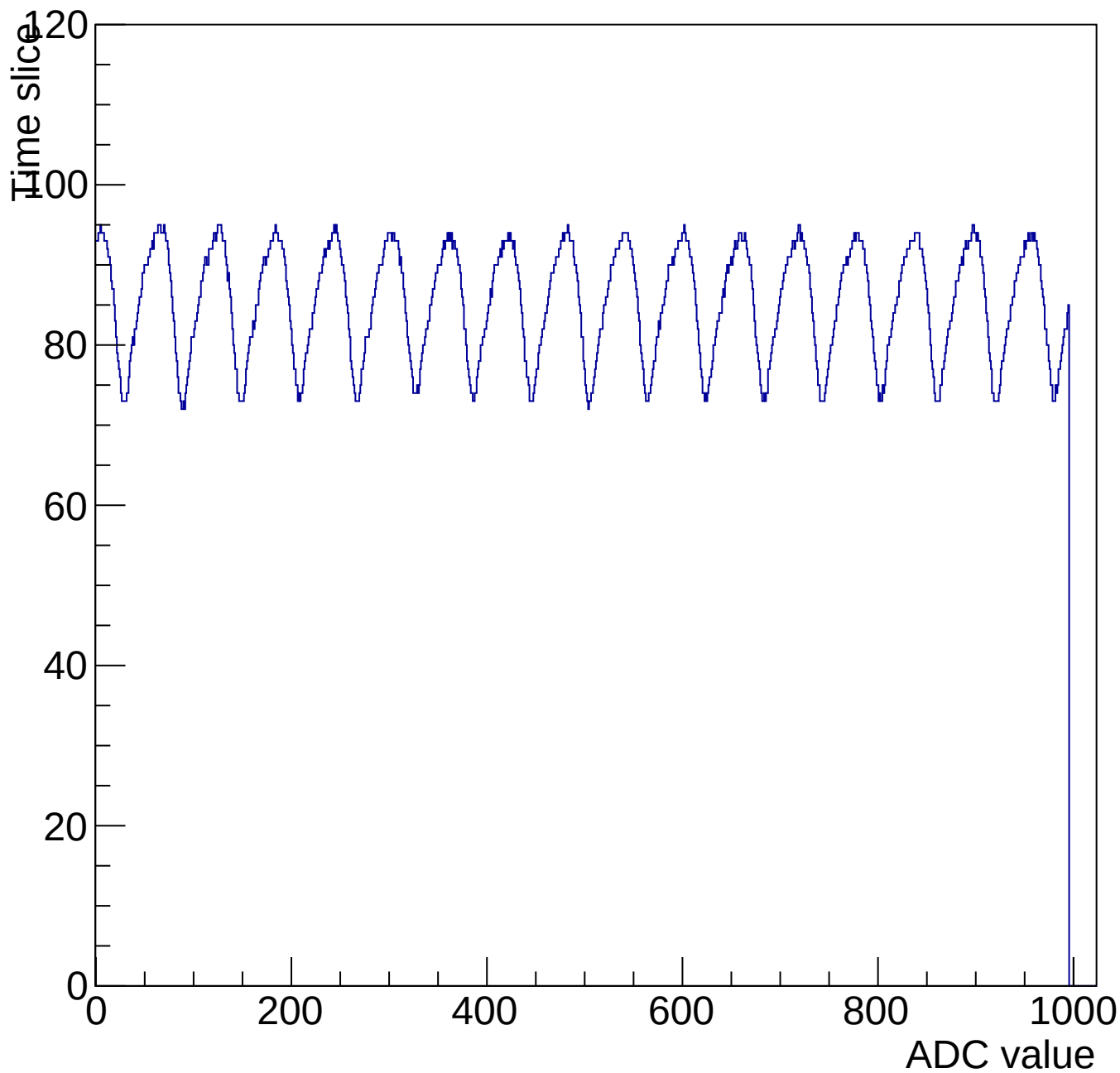
Evt 10 Time mcm 3007 chip 7 chan 1 1000-shift-gain0-shaper1
