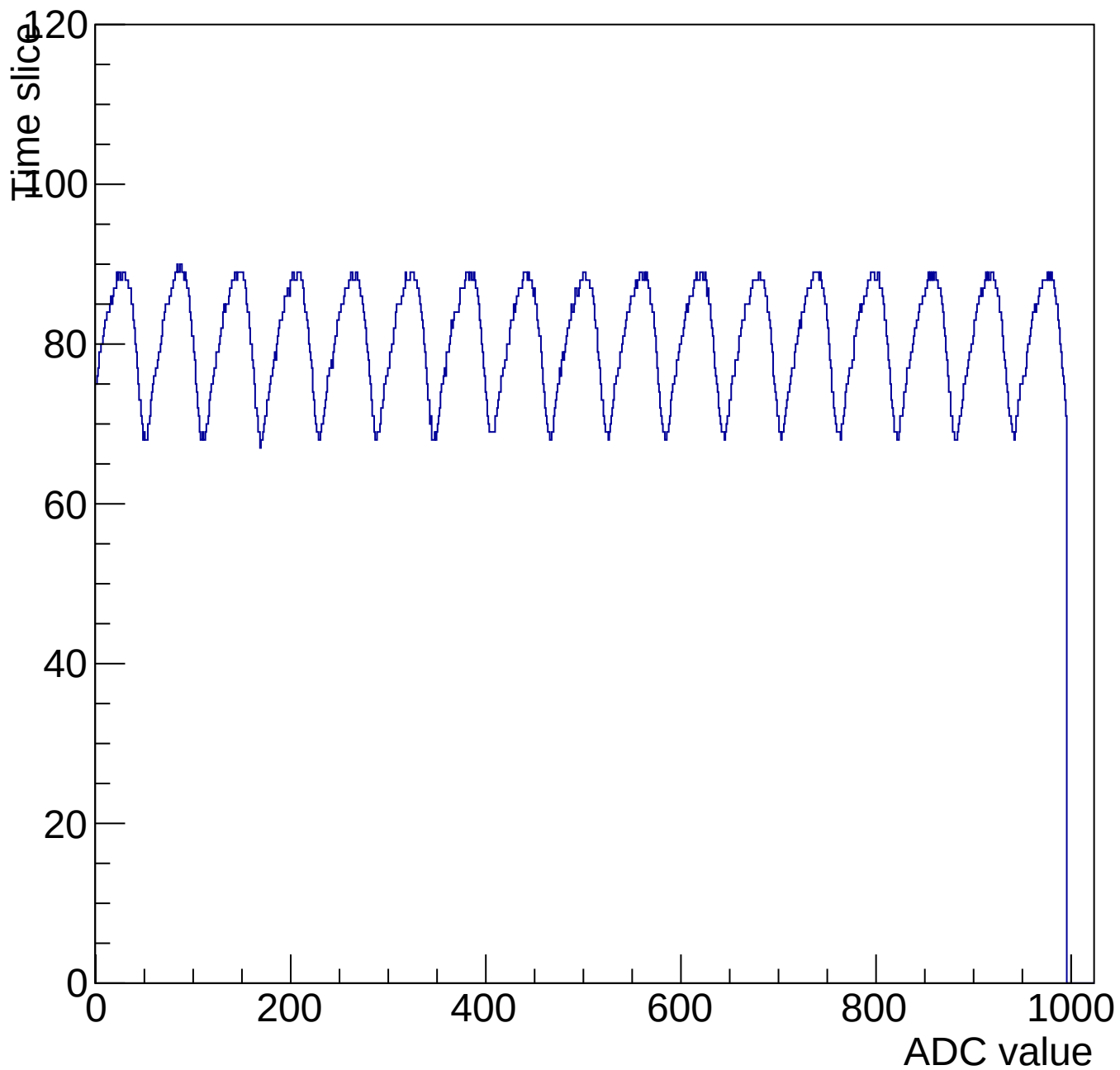
Evt 10 Time mcm 3007 chip 7 chan 2 1000-shift-gain0-shaper1
