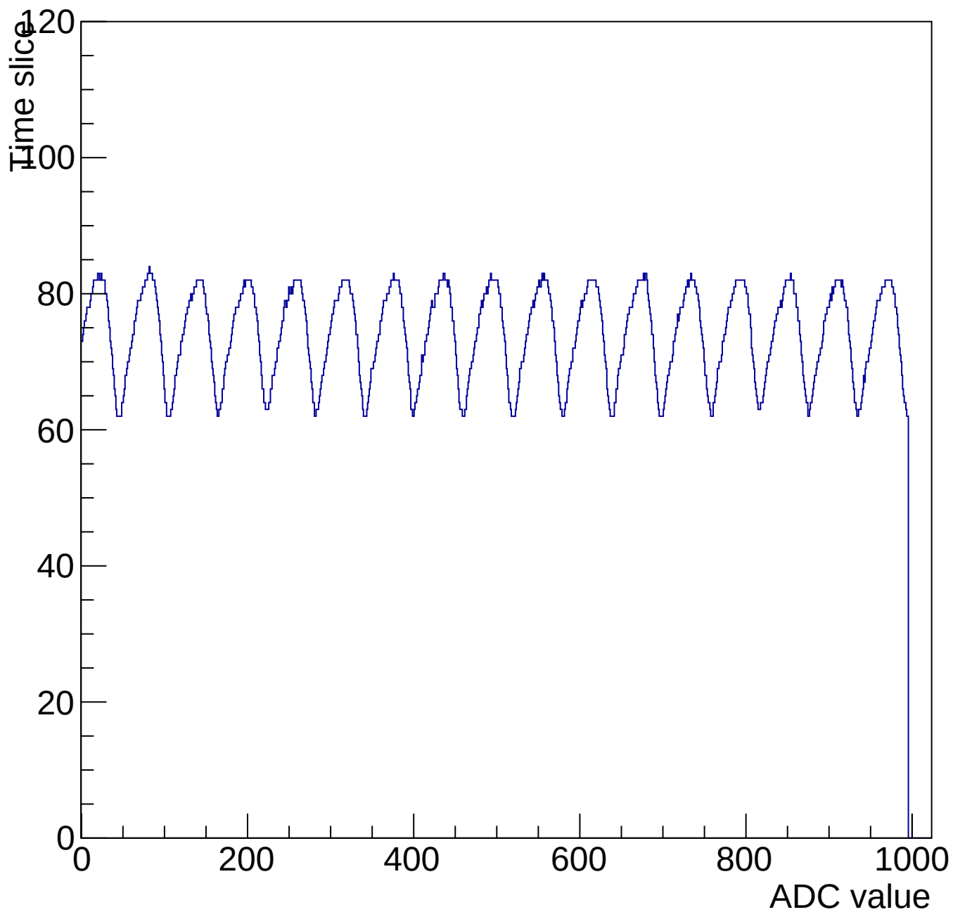
Evt 10 Time mcm 3007 chip 7 chan 10 1000-shift-gain0-shaper1
