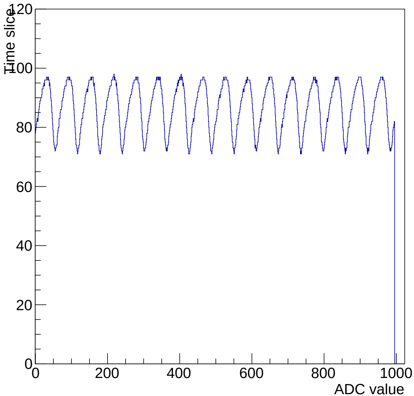
Evt 10 Time mcm 3007 chip 7 chan 1 1000-shift-gain0-shaper3
