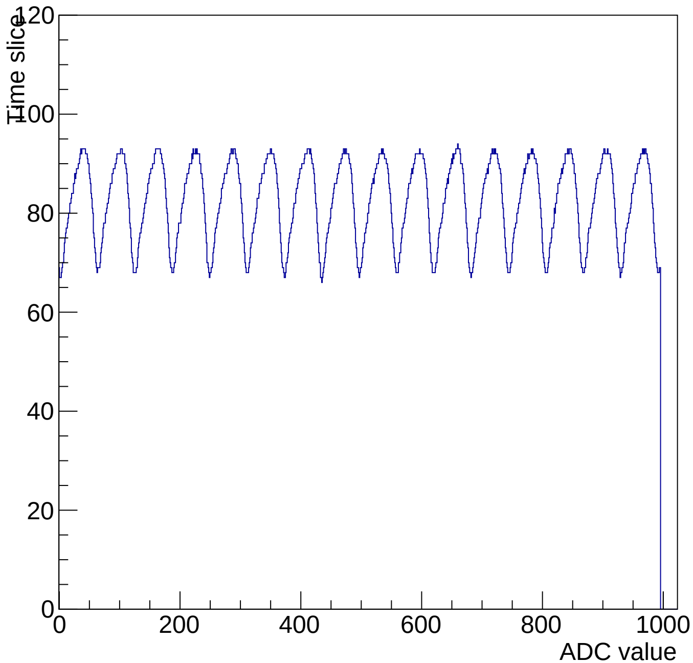
Evt 10 Time mcm 3007 chip 7 chan 11 1000-shift-gain0-shaper3
