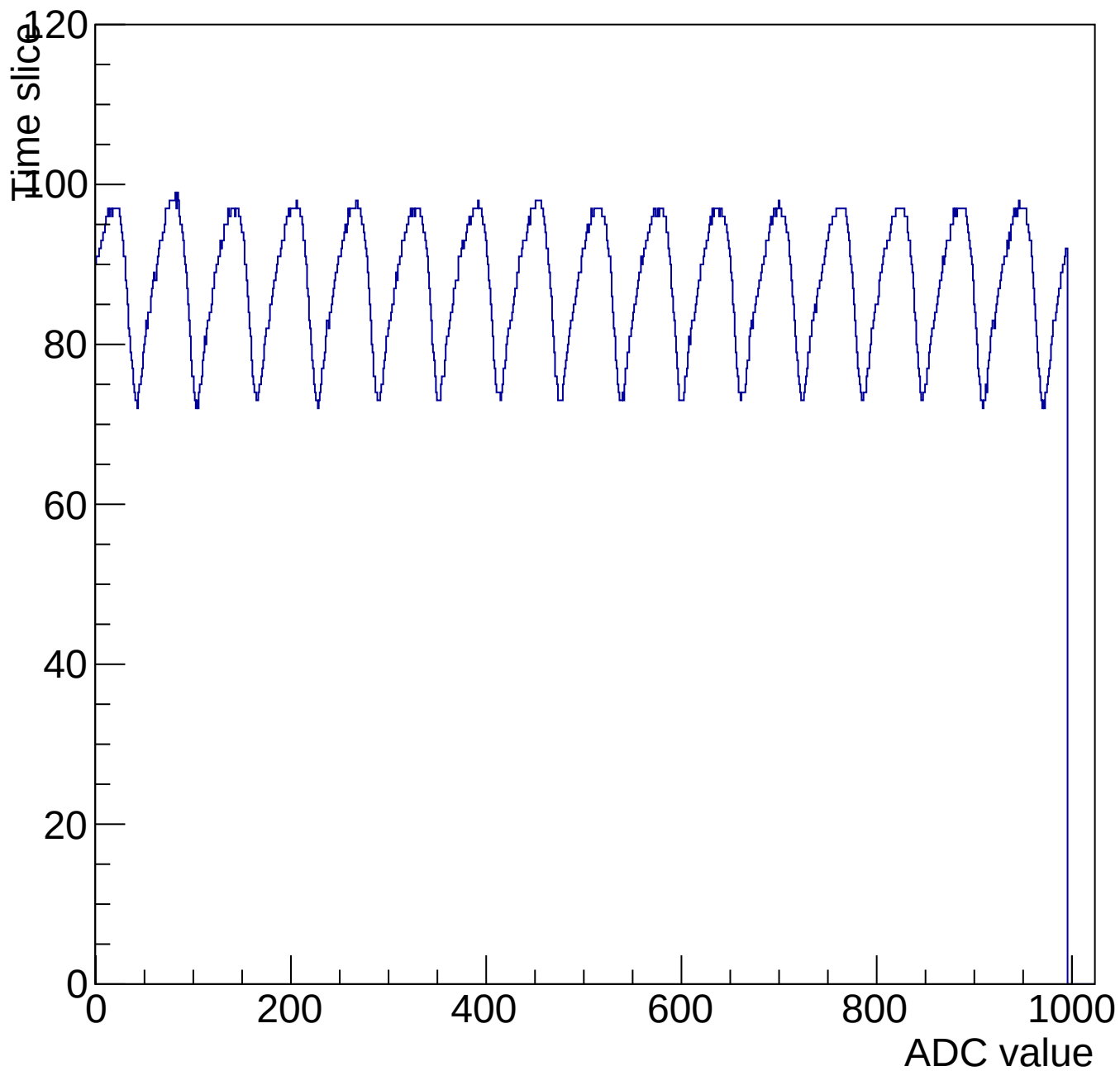
Evt 10 Time mcm 3007 chip 7 chan 3 1000-shift-gain0-shaper3
