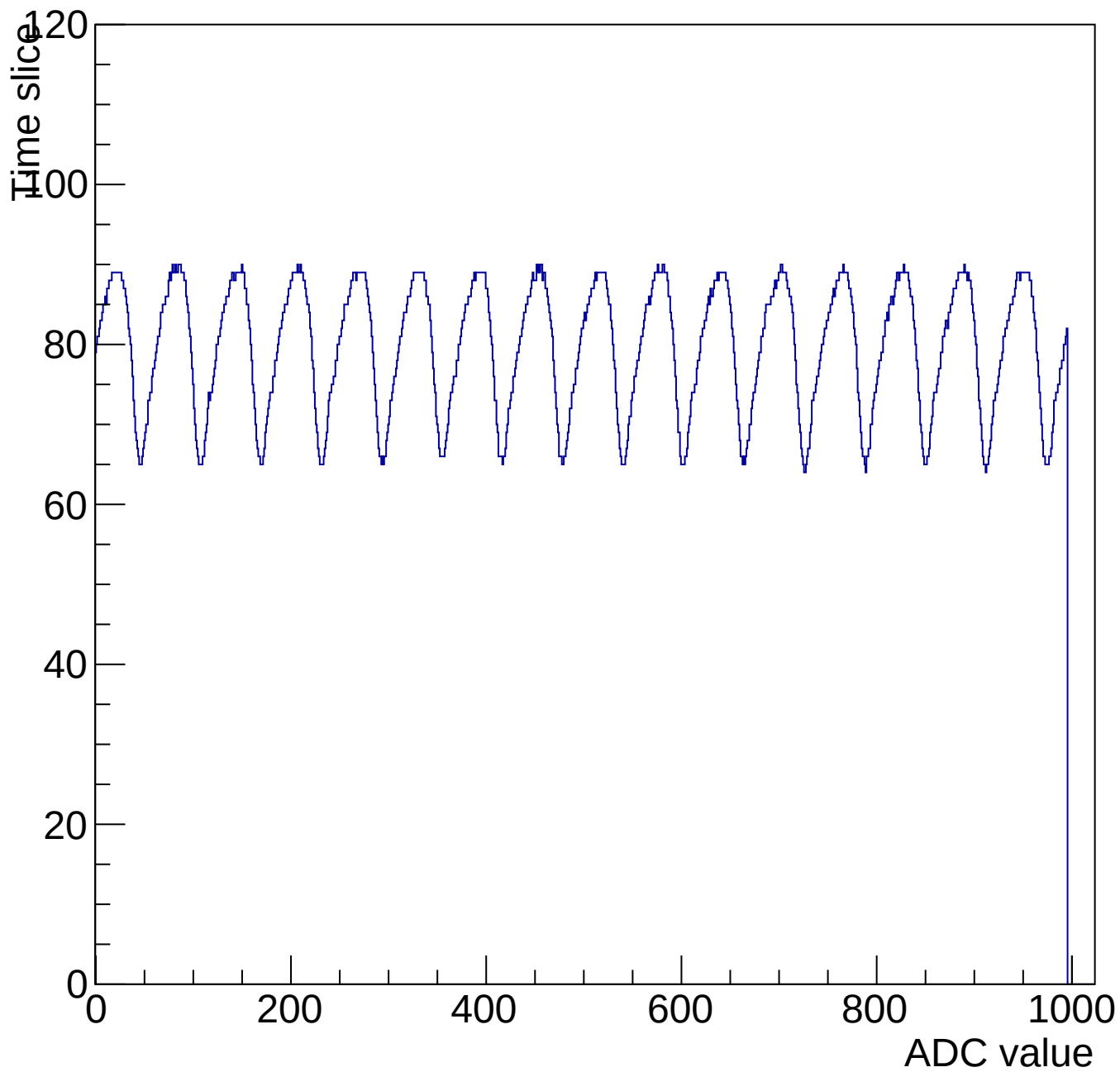
Evt 10 Time mcm 3007 chip 7 chan 12 1000-shift-gain0-shaper3
