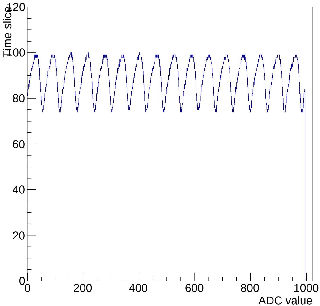
Evt 10 Time mcm 3007 chip 7 chan 15 1000-shift-gain0-shaper3
