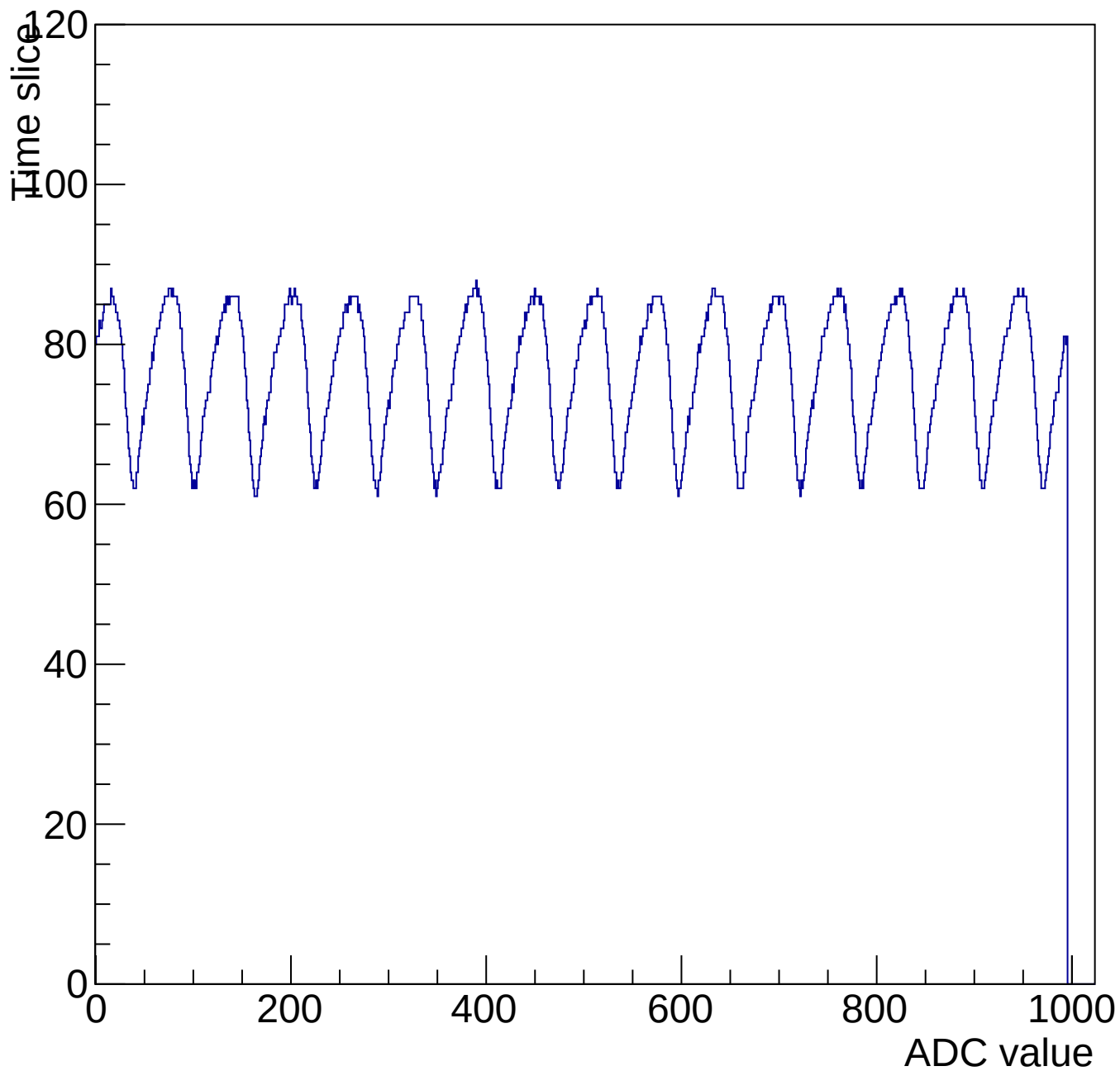
Evt 10 Time mcm 3007 chip 7 chan 9 1000-shift-gain0-shaper3
