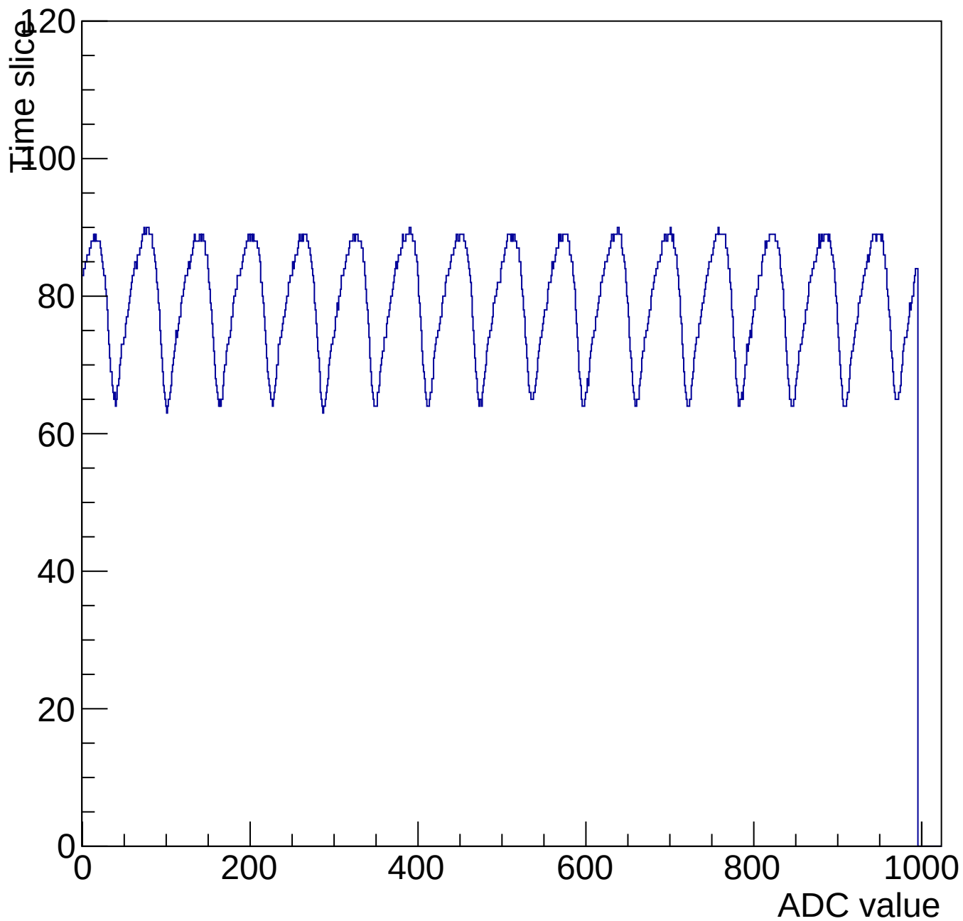
Evt 10 Time mcm 3007 chip 7 chan 8 1000-shift-gain0-shaper3
