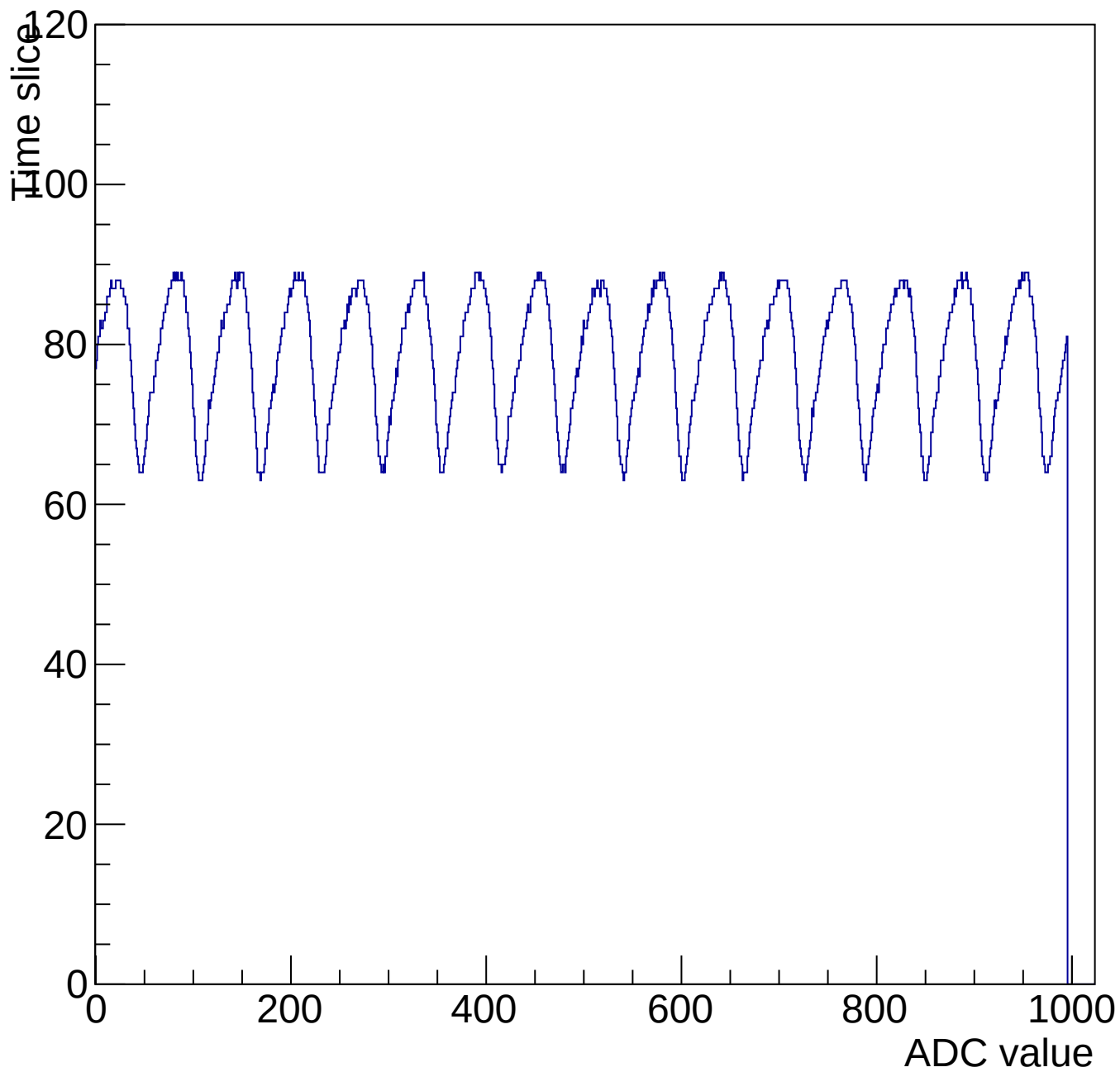
Evt 10 Time mcm 3007 chip 7 chan 13 1000-shift-gain0-shaper3
