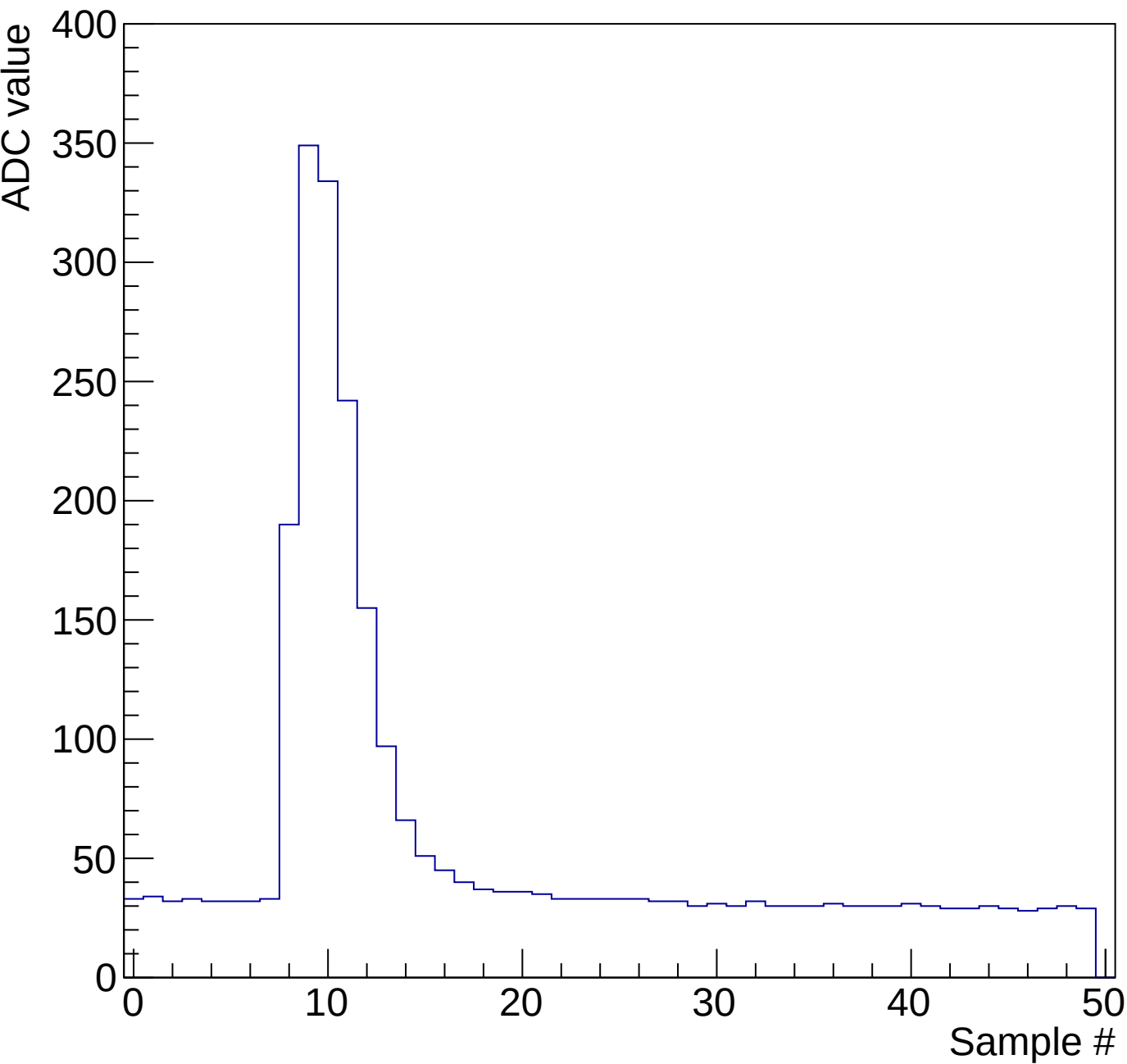
Run 34977 Event 1 Chip 2000 Channel_0_1
