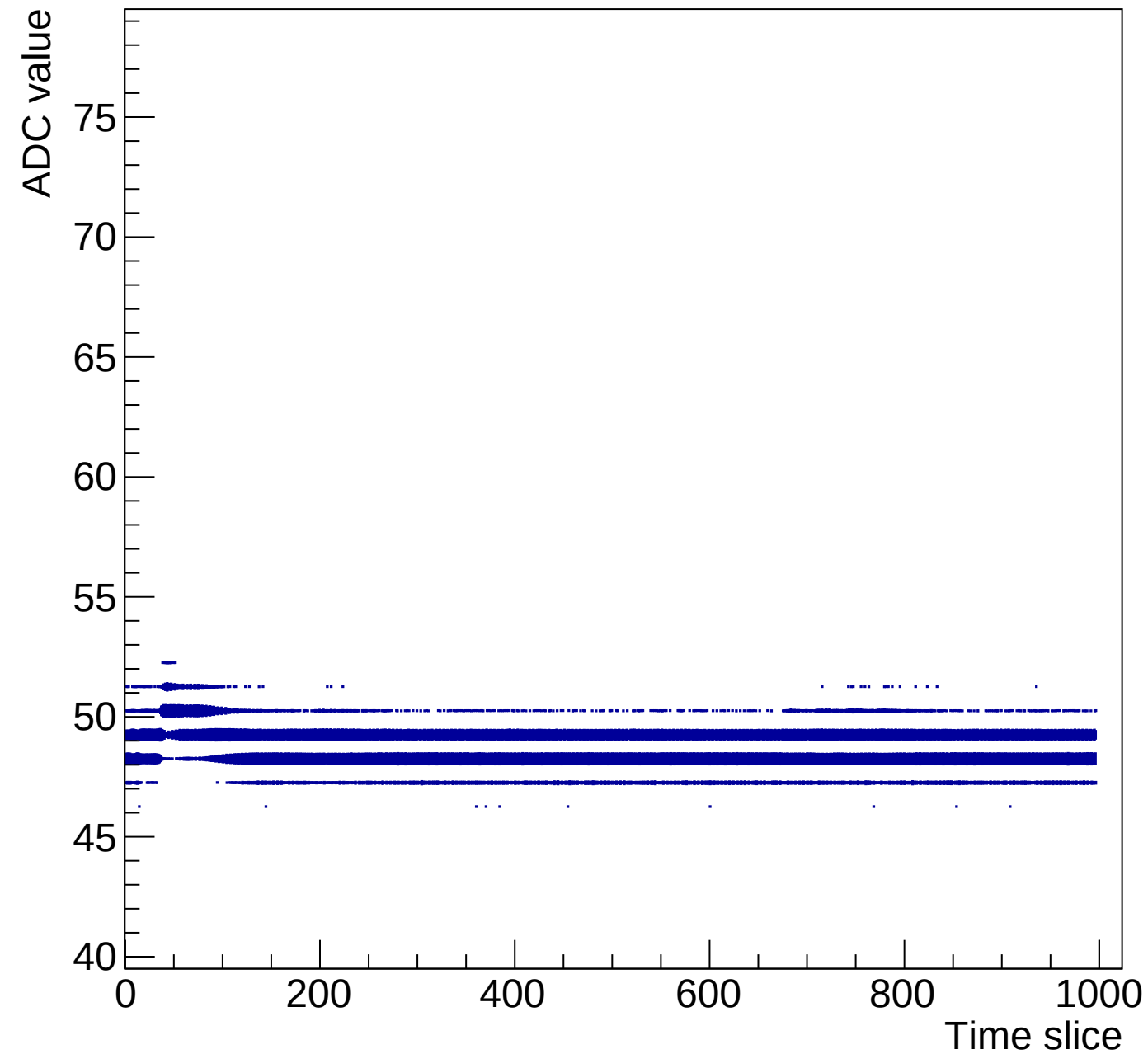
Time mcm 2007 chip 7 chan 0 gain0-shaper0
