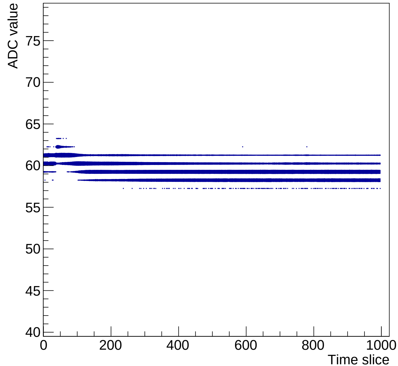
Time mcm 2007 chip 7 chan 15 gain0-shaper0
