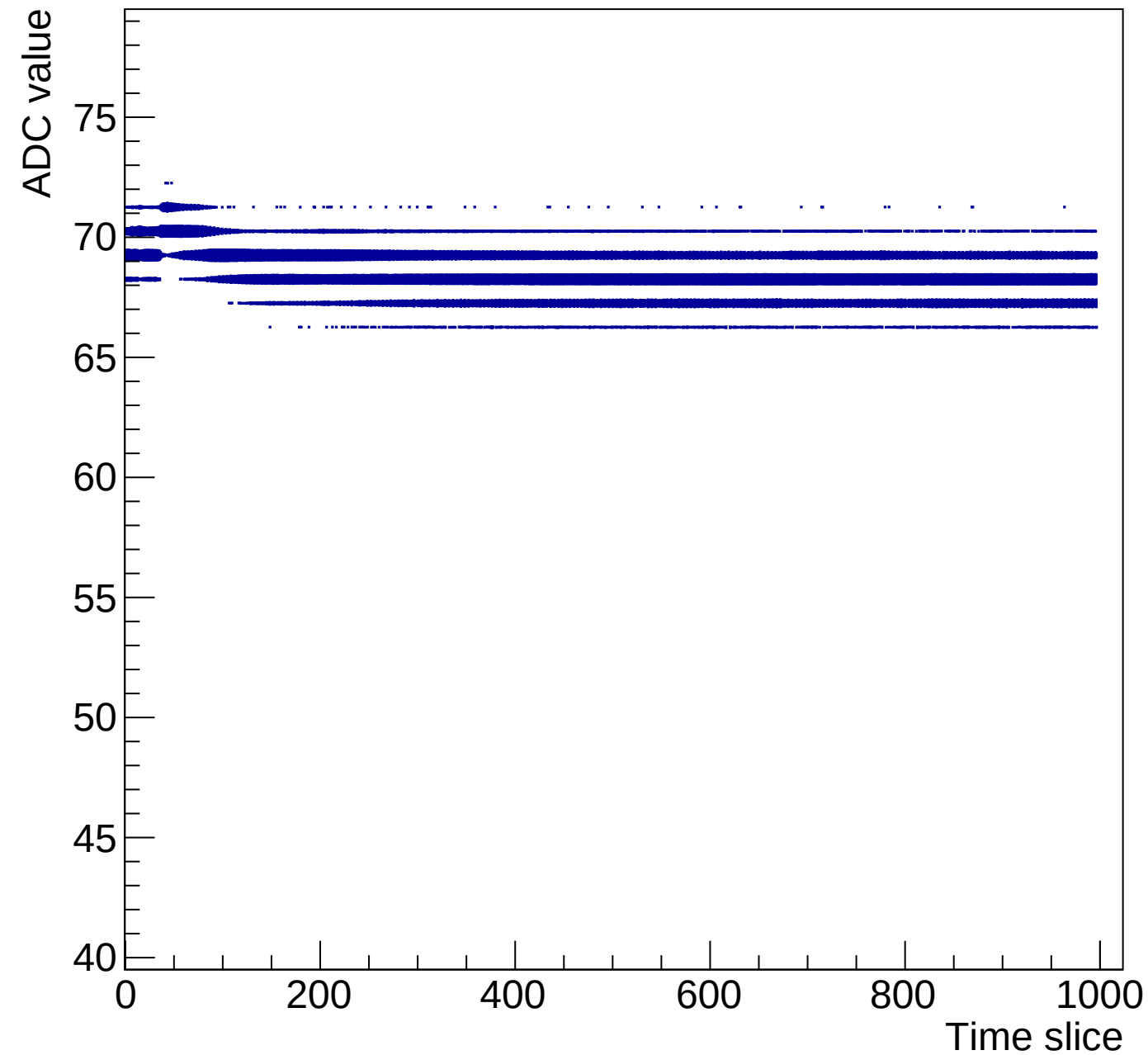
Time mcm 2007 chip 7 chan 14 gain0-shaper0
