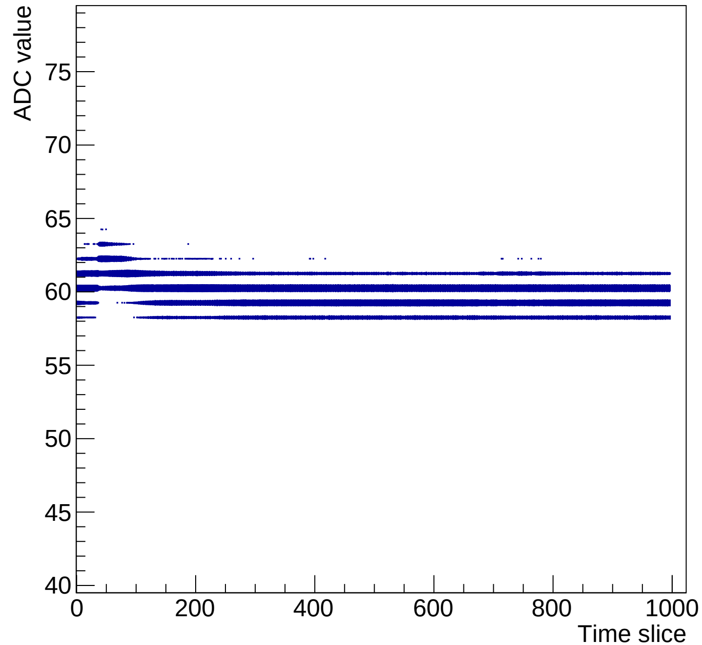
Time mcm 2007 chip 7 chan 4 gain0-shaper0
