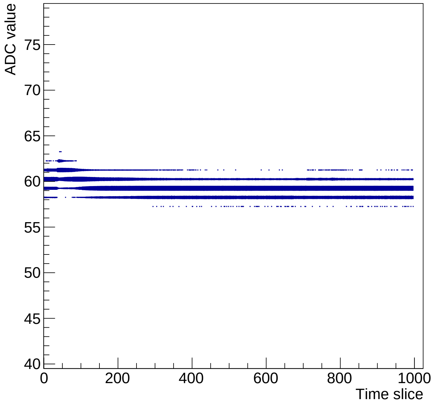
Time mcm 2007 chip 7 chan 9 gain0-shaper0
