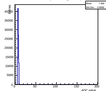
Pedestals ch 4 chip 2000 shift-gain0-shaper0
