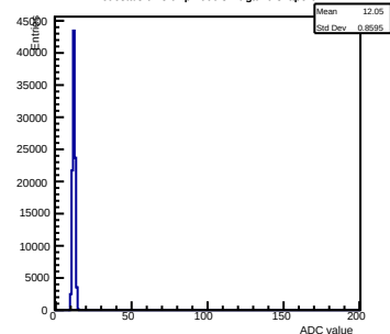
Pedestals ch 8 chip 2000 shift-gain0-shaper0
