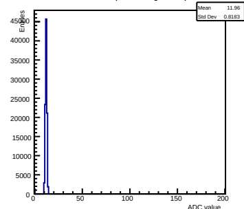
Pedestals ch 12 chip 2000 shift-gain0-shaper0
