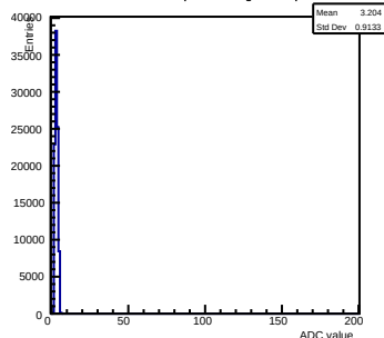
Pedestals ch 15 chip 2000 shift-gain0-shaper0
