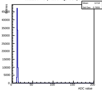
Pedestals ch 1 chip 2000 shift-gain0-shaper0
