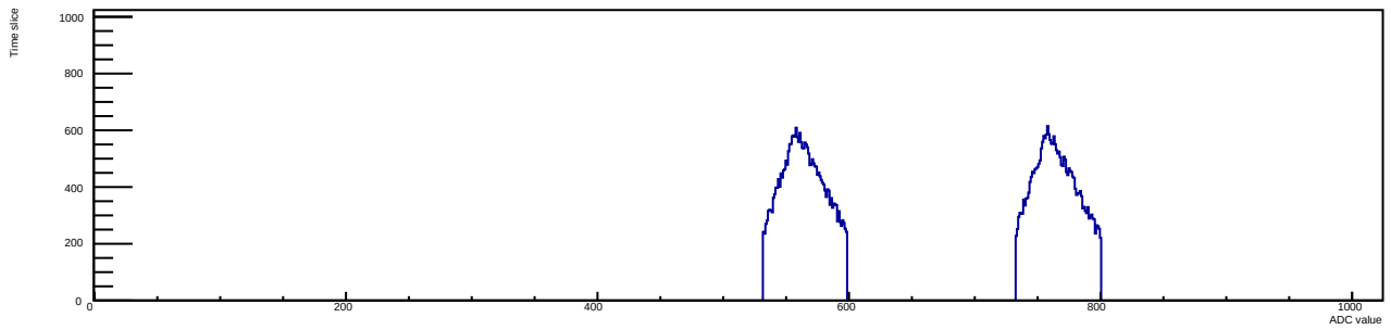
Run 36521 Evt 797 Time mcm 2 chip 3 chan 9 pulses
