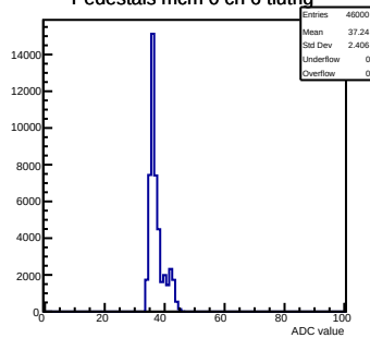
Pedestals mcm 0 ch 6 tlutrig
