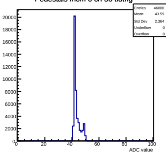
Pedestals mcm 0 ch 56 tlutrig
