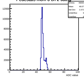
Pedestals mcm 0 ch 2 tlutrig
