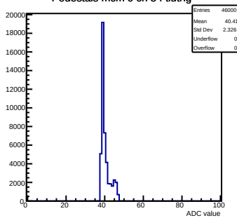
Pedestals mcm 0 ch 54 tlutrig
