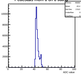
Pedestals mcm 0 ch 0 tlutrig
