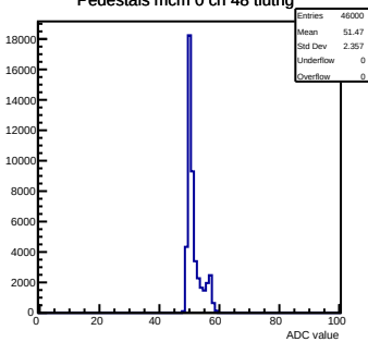
Pedestals mcm 0 ch 48 tlutrig
