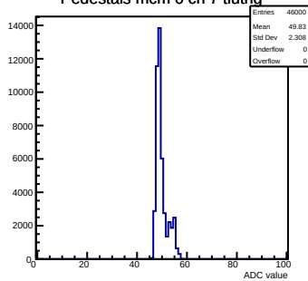
Pedestals mcm 0 ch 7 tlutrig
