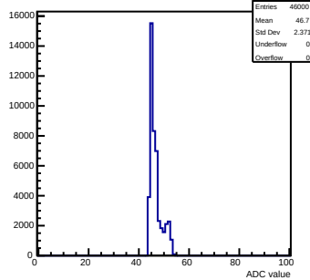
Pedestals mcm 0 ch 115 tlutrig
