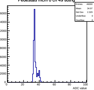
Pedestals mcm 0 ch 49 tlutrig
