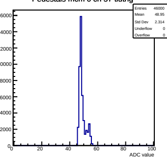
Pedestals mcm 0 ch 57 tlutrig
