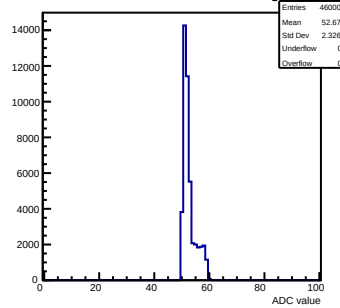
Pedestals mcm 0 ch 83 tlutrig
