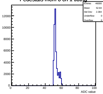
Pedestals mcm 0 ch 1 tlutrig
