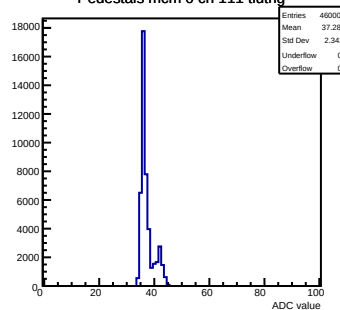
Pedestals mcm 0 ch 111 tlutrig
