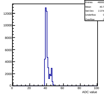
Pedestals mcm 0 ch 114 tlutrig
