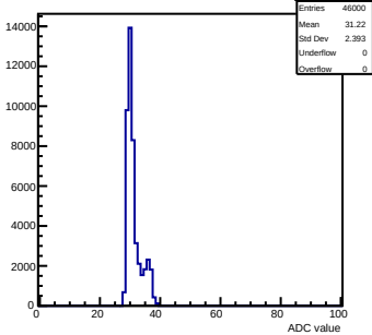
Pedestals mcm 0 ch 112 tlutrig
