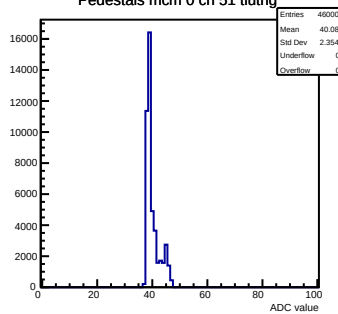
Pedestals mcm 0 ch 51 tlutrig
