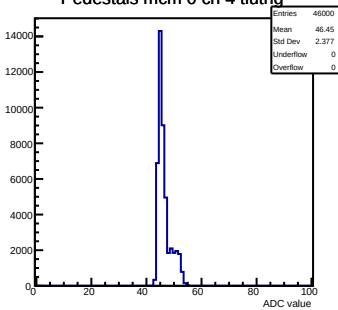
Pedestals mcm 0 ch 4 tlutrig
