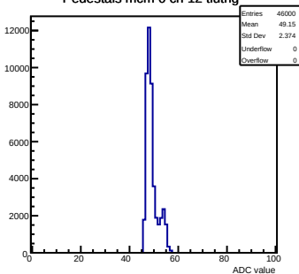
Pedestals mcm 0 ch 12 tlutrig
