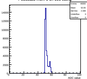
Pedestals mcm 0 ch 101 tlutrig
