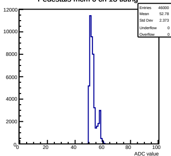
Pedestals mcm 0 ch 13 tlutrig
