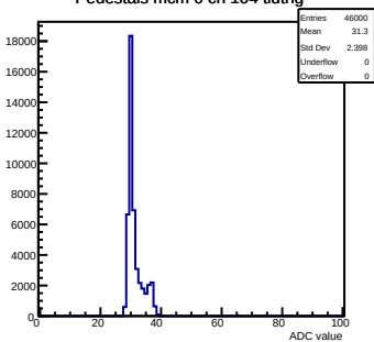
Pedestals mcm 0 ch 104 tlutrig
