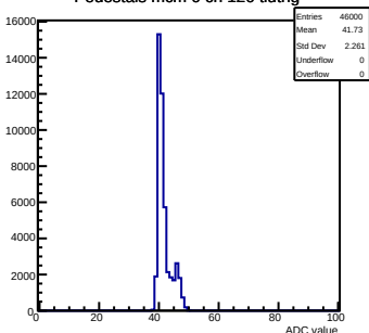
Pedestals mcm 0 ch 120 tlutrig
