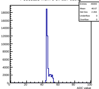
Pedestals mcm 0 ch 117 tlutrig
