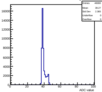
Pedestals mcm 0 ch 84 tlutrig
