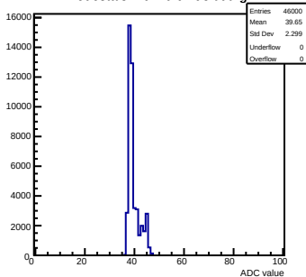
Pedestals mcm 0 ch 93 tlutrig
