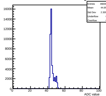
Pedestals mcm 0 ch 90 tlutrig
