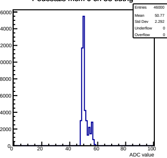
Pedestals mcm 0 ch 53 tlutrig
