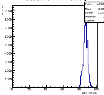
Pedestals mcm 1 ch 118 swt1rg
