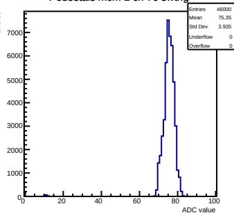
Pedestals mcm 1 ch 76 swtrig
