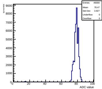
Pedestals mcm 1 ch 85 swrig
