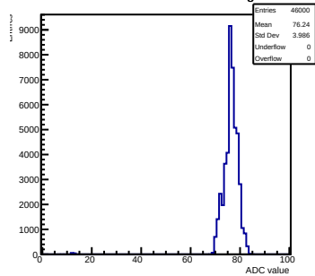
Pedestals mcm 1 ch 38 swtrig
