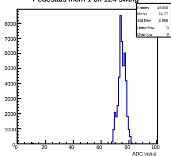
Pedestals mcm 1 ch 124 swt1rg
