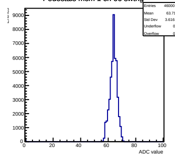
Pedestals mcm 1 ch 66 swtrig
