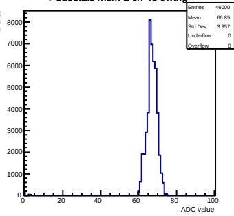
Pedestals mcm 1 ch 48 swtrig
