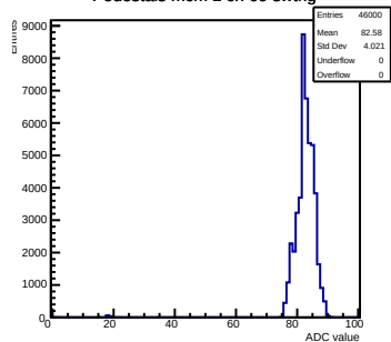
Pedestals mcm 1 ch 69 swtrig
