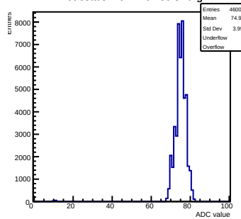
Pedestals mcm 1 ch 59 swtrig
