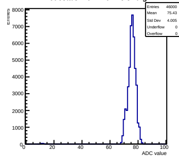
Pedestals mcm 1 ch 43 swtrig
