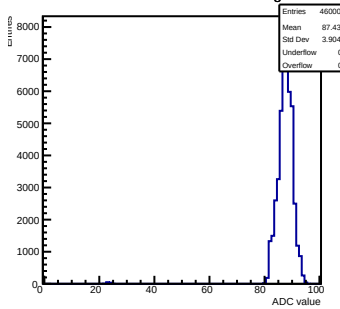
Pedestals mcm 1 ch 53 swtrig
