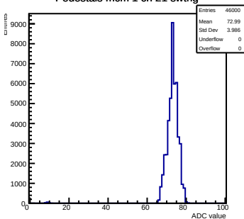
Pedestals mcm 1 ch 21 swtrig
