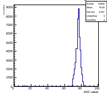
Pedestals mcm 1 ch 89 swrig
