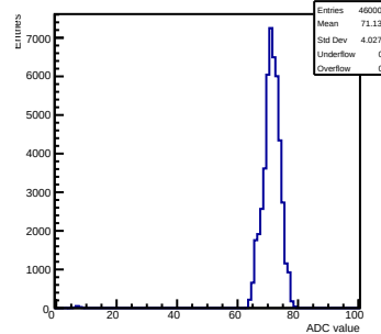
Pedestals mcm 1 ch 11 swtrig
