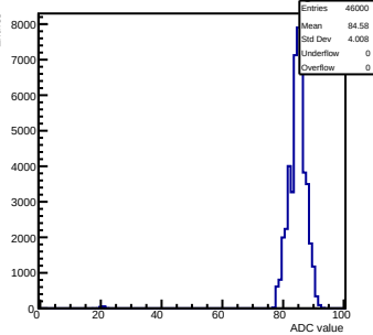
Pedestals mcm 1 ch 4 swtrig
