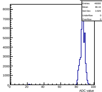
Pedestals mcm 1 ch 92 swrig
