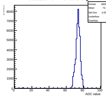
Pedestals mcm 1 ch 58 swtrig
