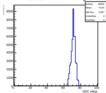
Pedestals mcm 1 ch 42 swtrig
