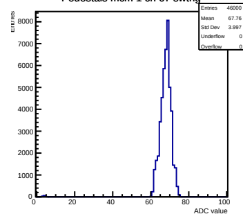
Pedestals mcm 1 ch 67 swtrig
