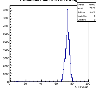
Pedestals mcm 1 ch 24 swtrig
