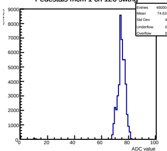
Pedestals mcm 1 ch 126 swt1rg
