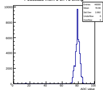
Pedestals mcm 1 ch 73 swtrig
