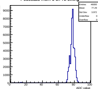
Pedestals mcm 1 ch 72 swtrig
