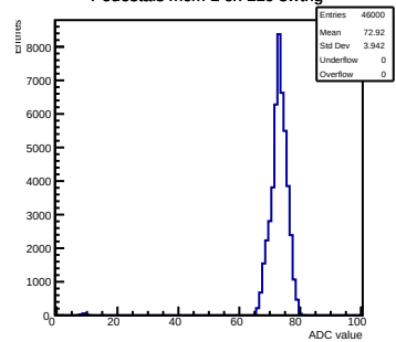
Pedestals mcm 1 ch 119 swt1rg
