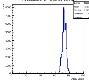
Pedestals mcm 1 ch 19 swtrig
