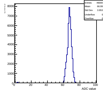
Pedestals mcm 1 ch 14 swtrig
