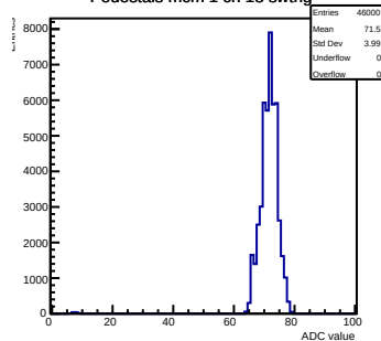
Pedestals mcm 1 ch 18 swtrig
