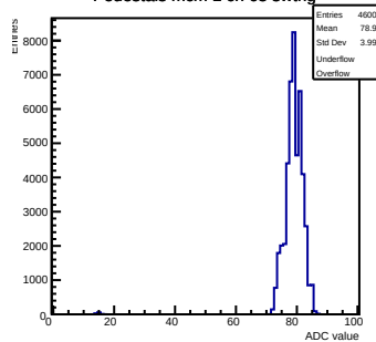
Pedestals mcm 1 ch 63 swtrig
