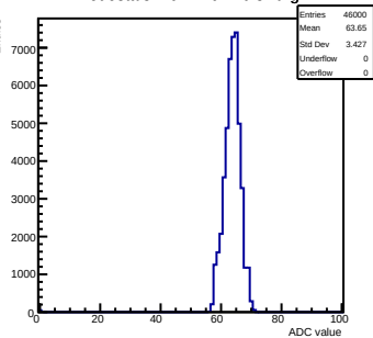
Pedestals mcm 1 ch 40 swtrig
