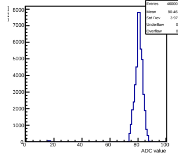
Pedestals mcm 1 ch 6 swtrig
