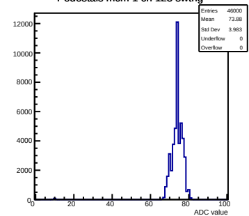
Pedestals mcm 1 ch 123 swt1rg
