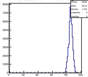
Pedestals mcm 1 ch 0 swtrig
