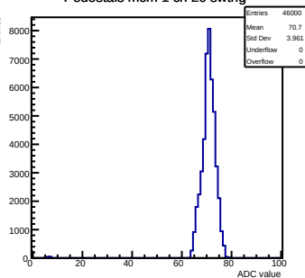
Pedestals mcm 1 ch 20 swtrig
