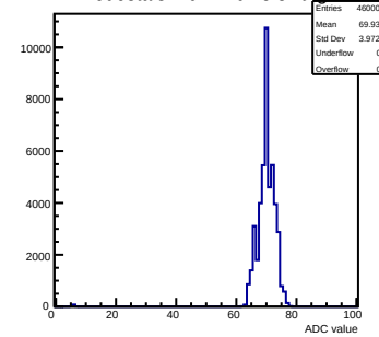
Pedestals mcm 1 ch 3 swtrig
