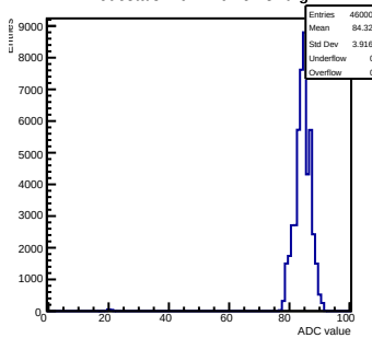
Pedestals mcm 1 ch 57 swtrig
