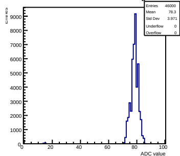
Pedestals mcm 1 ch 93 swrig
