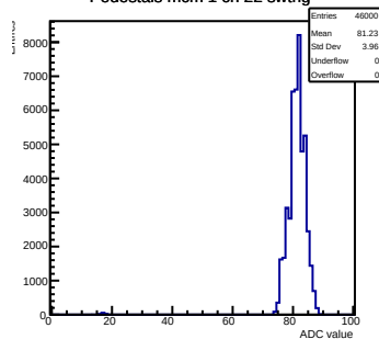
Pedestals mcm 1 ch 22 swtrig
