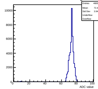
Pedestals mcm 1 ch 55 swtrig
