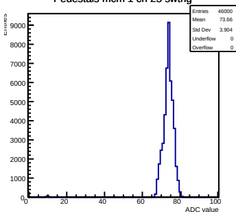
Pedestals mcm 1 ch 25 swtrig
