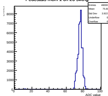
Pedestals mcm 1 ch 26 swtrig
