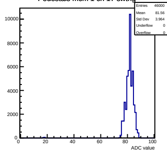
Pedestals mcm 1 ch 17 swtrig
