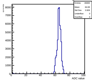
Pedestals mcm 1 ch 37 swtrig
