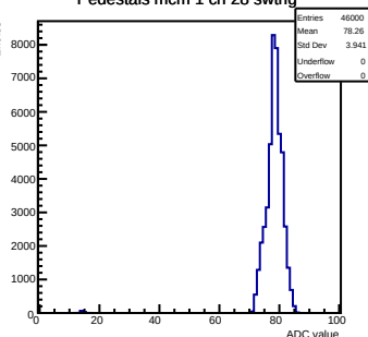
Pedestals mcm 1 ch 28 swtrig
