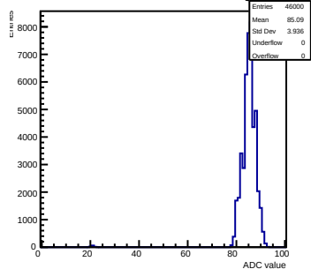
Pedestals mcm 1 ch 81 swrig
