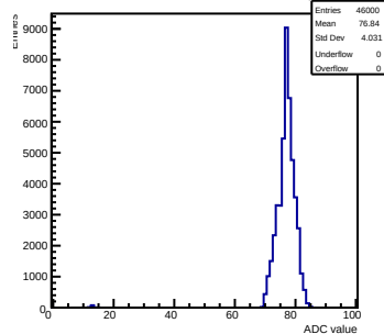
Pedestals mcm 1 ch 13 swtrig
