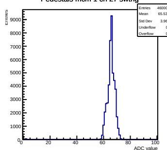
Pedestals mcm 1 ch 27 swtrig
