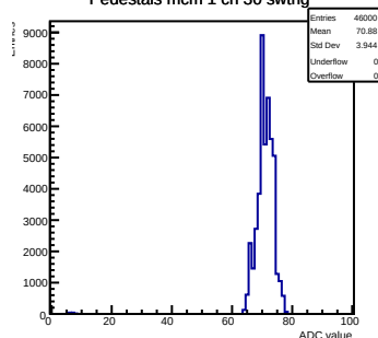
Pedestals mcm 1 ch 30 swtrig
