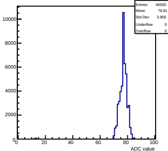
Pedestals mcm 1 ch 12 swtrig
