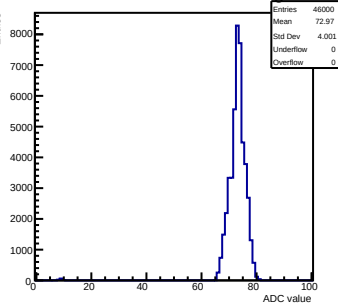
Pedestals mcm 1 ch 8 swtrig
