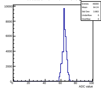
Pedestals mcm 1 ch 41 swtrig
