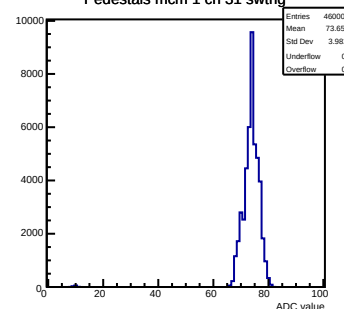
Pedestals mcm 1 ch 31 swtrig
