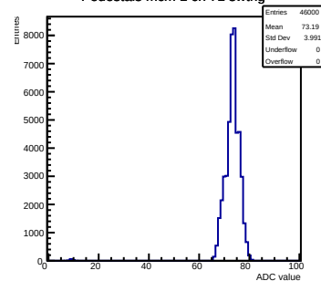
Pedestals mcm 1 ch 71 swtrig
