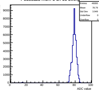
Pedestals mcm 1 ch 16 swtrig
