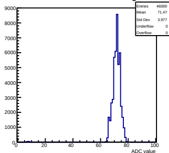
Pedestals mcm 1 ch 88 swrig
