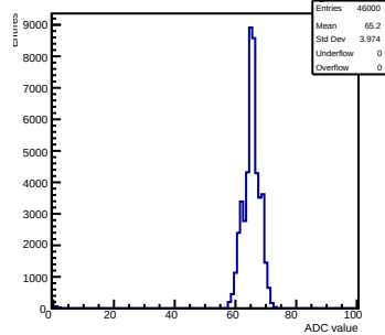
Pedestals mcm 1 ch 5 swtrig
