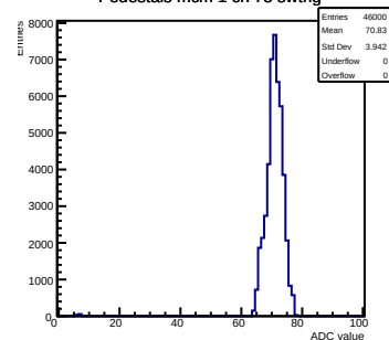
Pedestals mcm 1 ch 75 swtrig
