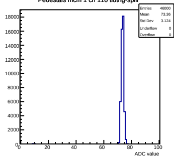
Pedestals mcm 1 ch 110 lutrig-spill
