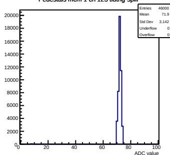
Pedestals mcm 1 ch 123 lutrig-spill
