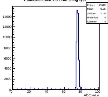
Pedestals mcm 1 ch 105 lutrig-spill
