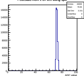
Pedestals mcm 1 ch 121 lutrig-spill
