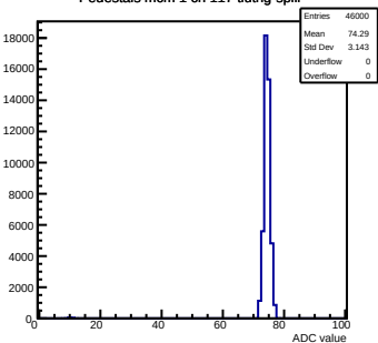
Pedestals mcm 1 ch 117 lutrig-spill
