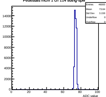
Pedestals mcm 1 ch 114 lutrig-spill
