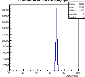
Pedestals mcm 1 ch 108 lutrig-spill
