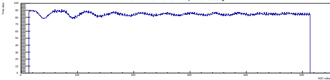
Run 12 Evt 3 Time mcm 1 chip 0 chan 0 30deg
