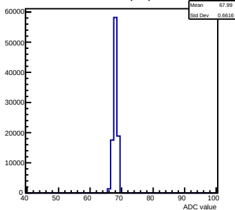
Pedestals ch 0 chip 7 protomcm
