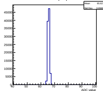
Pedestals ch 6 chip 7 protomcm
