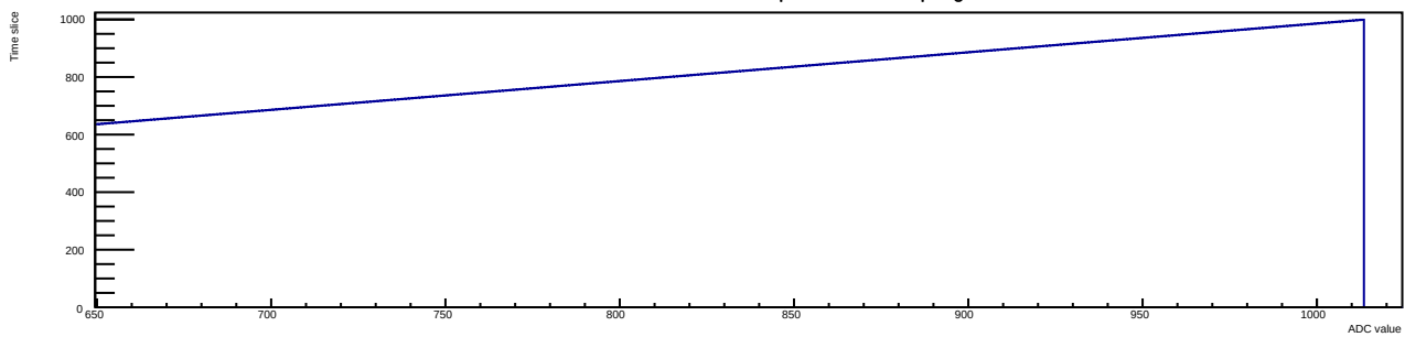
Run 15 Evt 2 Time mcm 0 chip 2 chan 15 ramp-high
