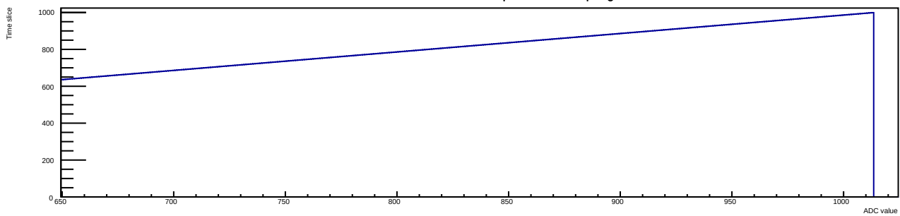
Run 15 Evt 2 Time mcm 0 chip 4 chan 3 ramp-high
