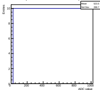
Ramp mcm 0 channel 56 run 18 ramps-1
