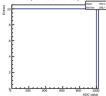
Ramp mcm 1 channel 110 run 19 ramps-2
