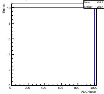
Ramp mcm 1 channel 64 run 19 ramps-2
